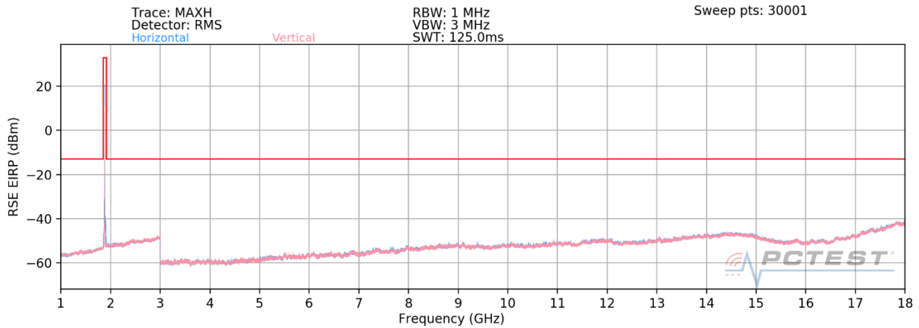
Plot 7-34. Ant 1 - n261 Radiated Spurious Plot– Anchor Band 2
