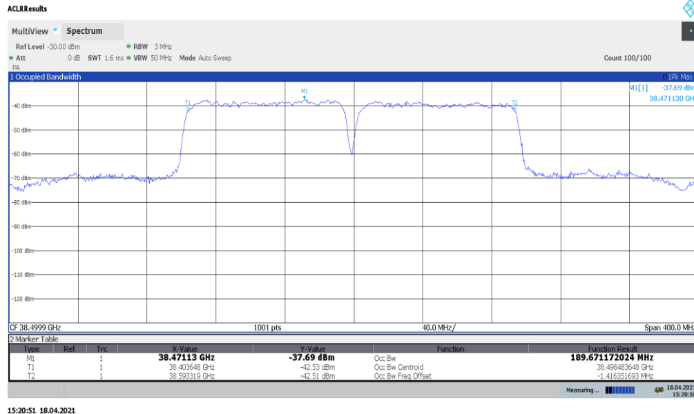
Plot 7-22. Ant 1 Occupied Bandwidth Plot (100MHz-2CC – pi/2-BPSK – Mid Channel)
