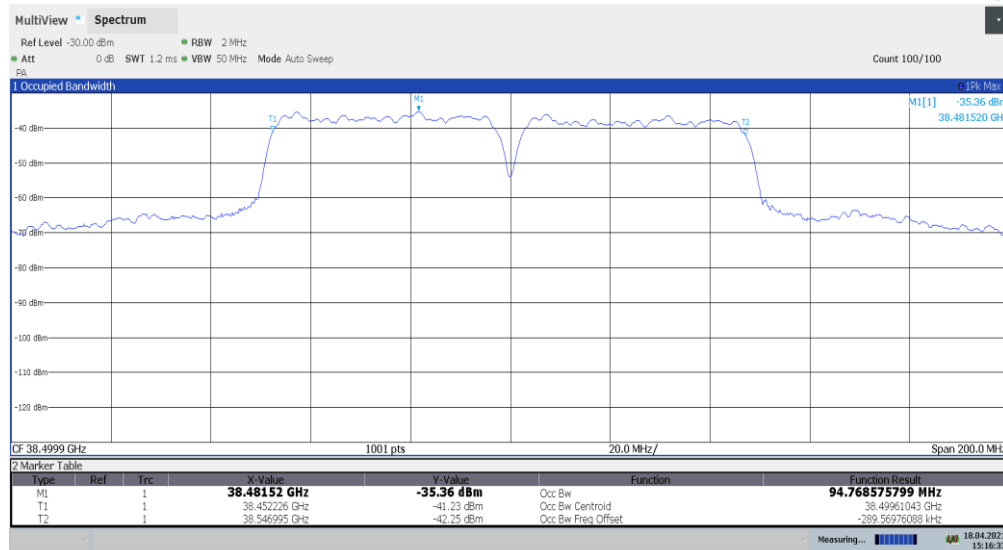
Plot 7-29. Ant 1 Occupied Bandwidth Plot (50MHz-2CC – QPSK – Mid Channel)
