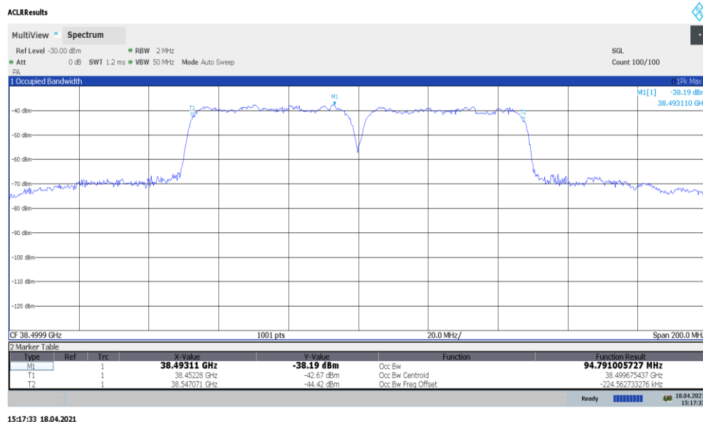
Plot 7-31. Ant 1 Occupied Bandwidth Plot (50MHz-2CC – 16QAM – Mid Channel)
