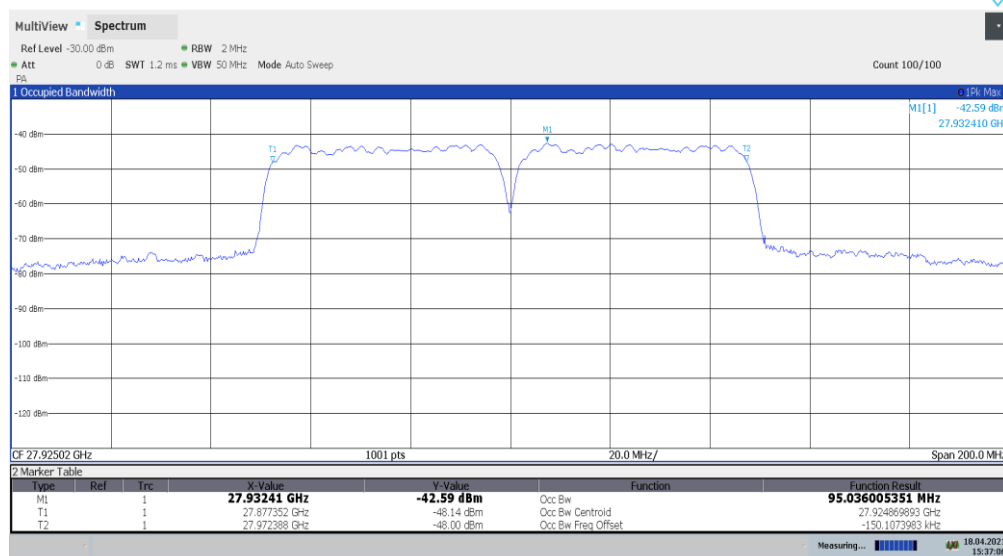
Plot 7-13. Ant 1 Occupied Bandwidth Plot (50MHz-2CC – QPSK – Mid Channel)
