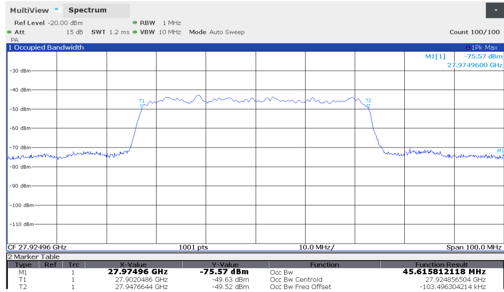
Plot 7-10. Ant 1 Occupied Bandwidth Plot (50MHz-1CC – pi/2-BPSK – Mid Channel)
