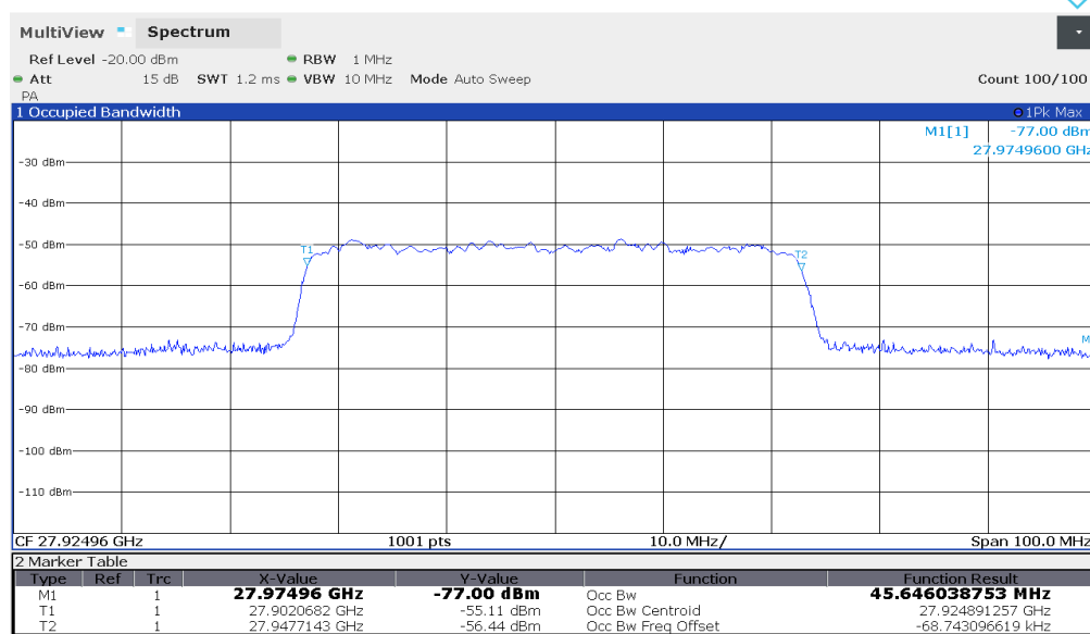
Plot 7-12. Ant 1 Occupied Bandwidth Plot (50MHz-1CC – 64QAM – Mid Channel)
