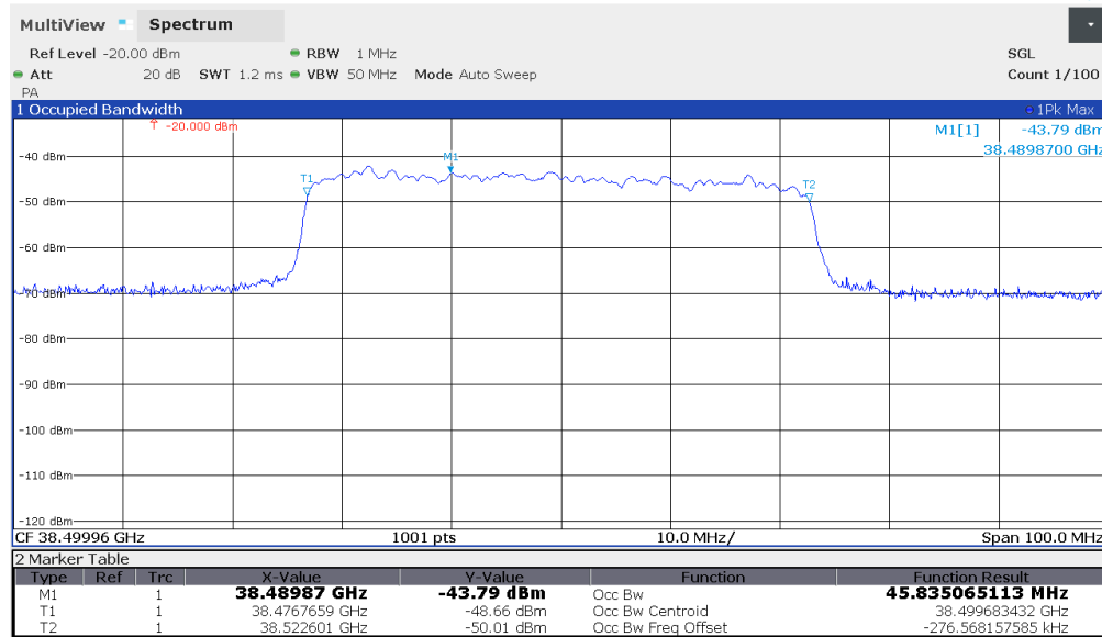
Plot 7-28. Ant 1 Occupied Bandwidth Plot (50MHz-1CC – 64QAM – Mid Channel)
