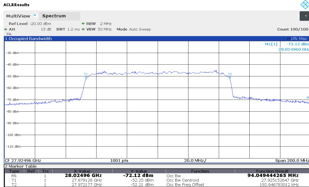
Plot 7-1. Ant 1 Occupied Bandwidth Plot (100MHz-1CC – QPSK – Mid Channel)
