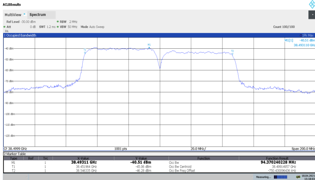
Plot 7-32. Ant 1 Occupied Bandwidth Plot (50MHz-2CC – 64QAM – Mid Channel)
