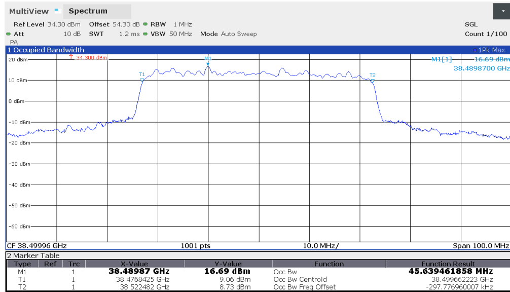
Plot 7-26. Ant 1 Occupied Bandwidth Plot (50MHz-1CC – pi/2-BPSK – Mid Channel)
