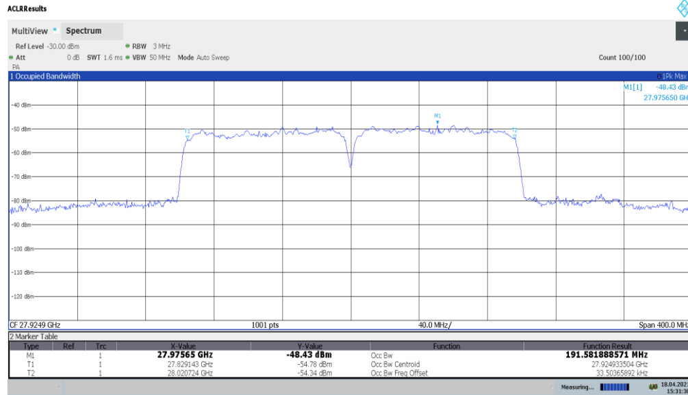
Plot 7-8. Ant 1 Occupied Bandwidth Plot (100MHz-2CC – 64QAM – Mid Channel)
