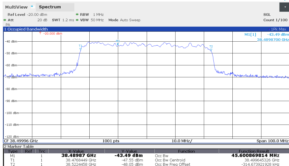
Plot 7-27. Ant 1 Occupied Bandwidth Plot (50MHz-1CC – 16QAM – Mid Channel)
