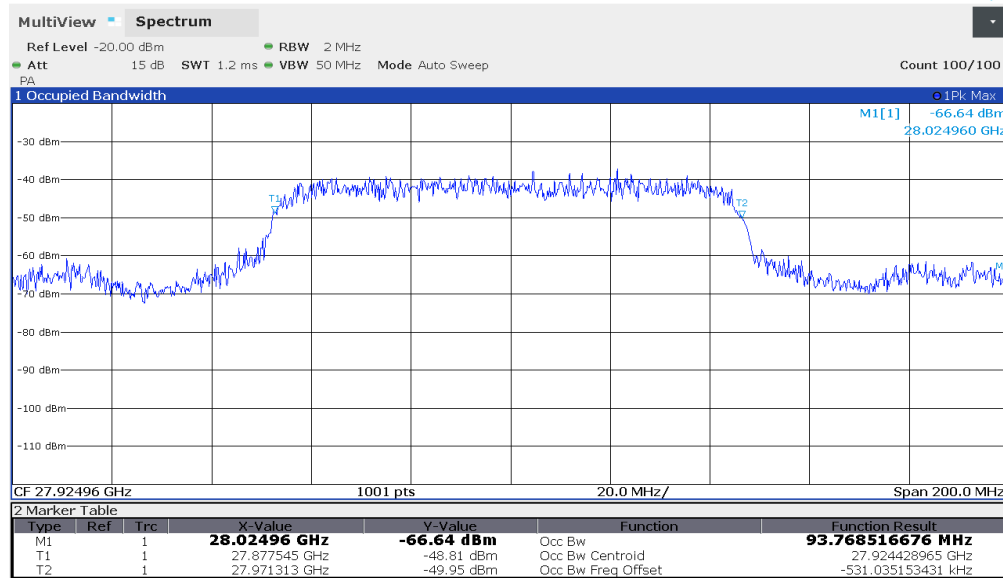
Plot 7-2. Ant 1 Occupied Bandwidth Plot (100MHz-1CC – pi/2-BPSK – Mid Channel)
