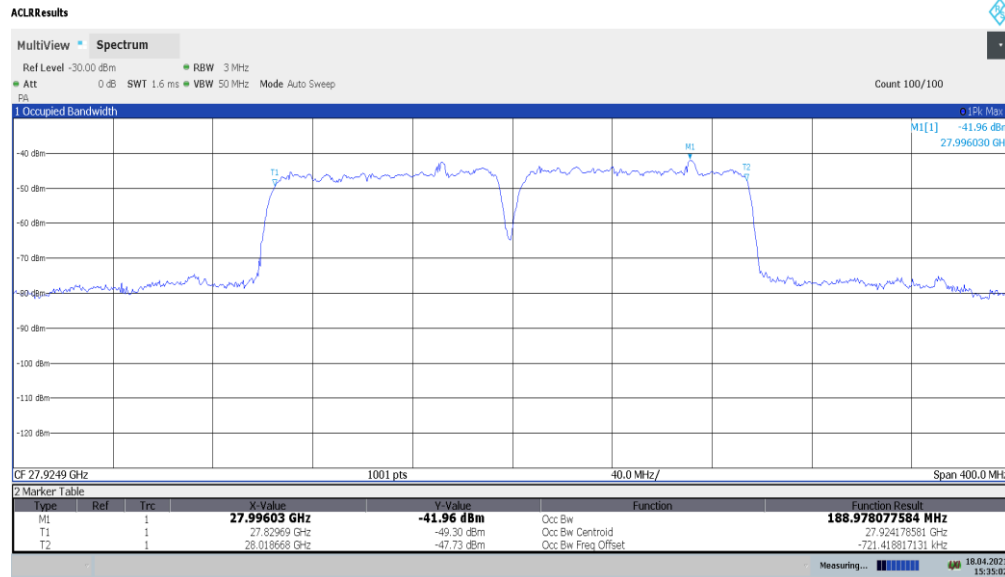
Plot 7-6. Ant 1 Occupied Bandwidth Plot (100MHz-2CC – pi/2-BPSK – Mid Channel)
