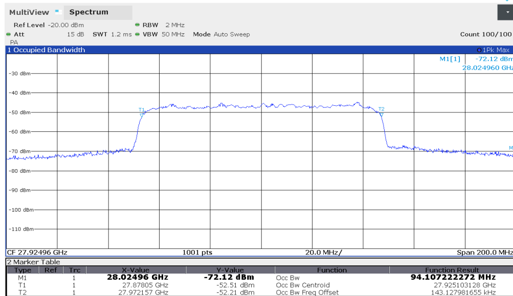
Plot 7-3. Ant 1 Occupied Bandwidth Plot (100MHz-1CC – 16QAM – Mid Channel)
