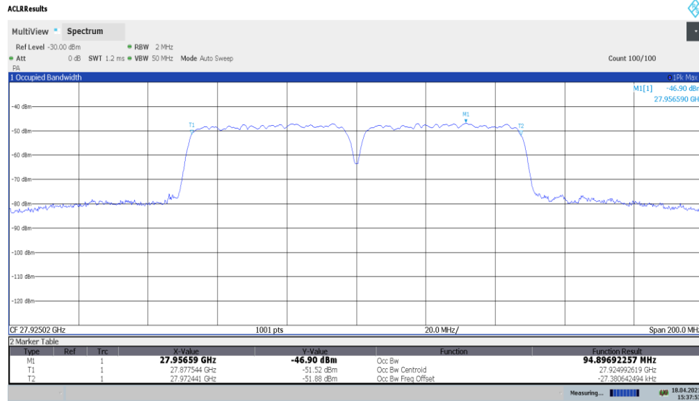
Plot 7-16. Ant 1 Occupied Bandwidth Plot (50MHz-2CC – 64QAM – Mid Channel)
