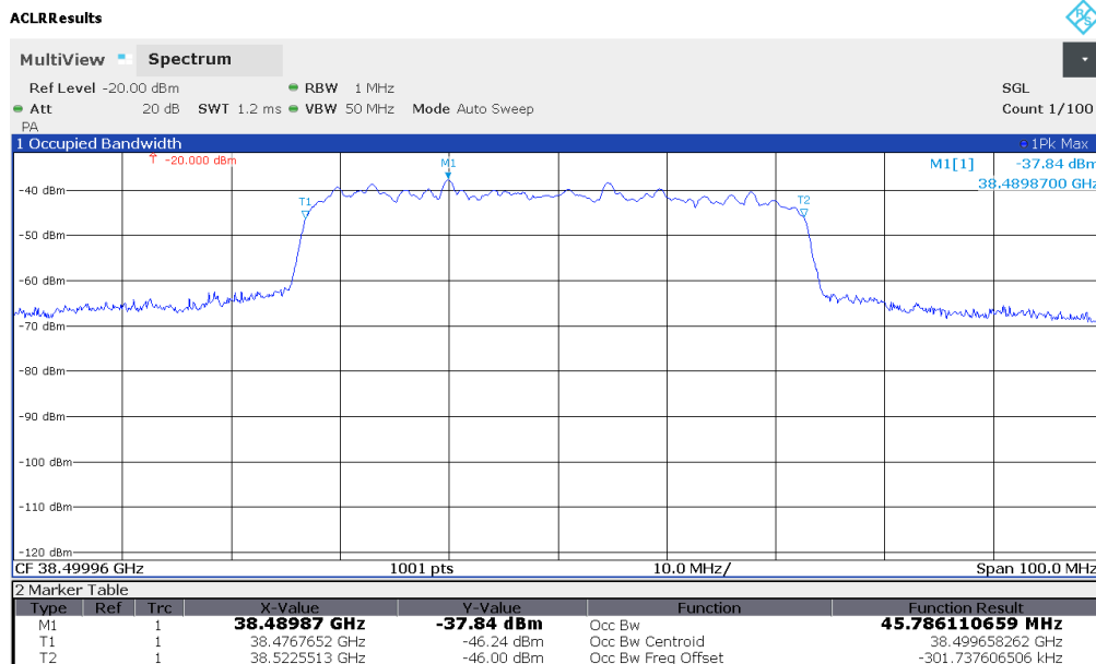
Plot 7-25. Ant 1 Occupied Bandwidth Plot (50MHz-1CC – QPSK – Mid Channel)
