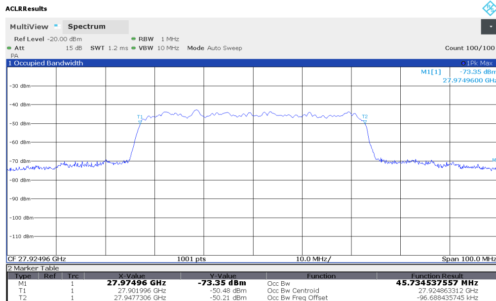
Plot 7-9. Ant 1 Occupied Bandwidth Plot (50MHz-1CC – QPSK – Mid Channel)
