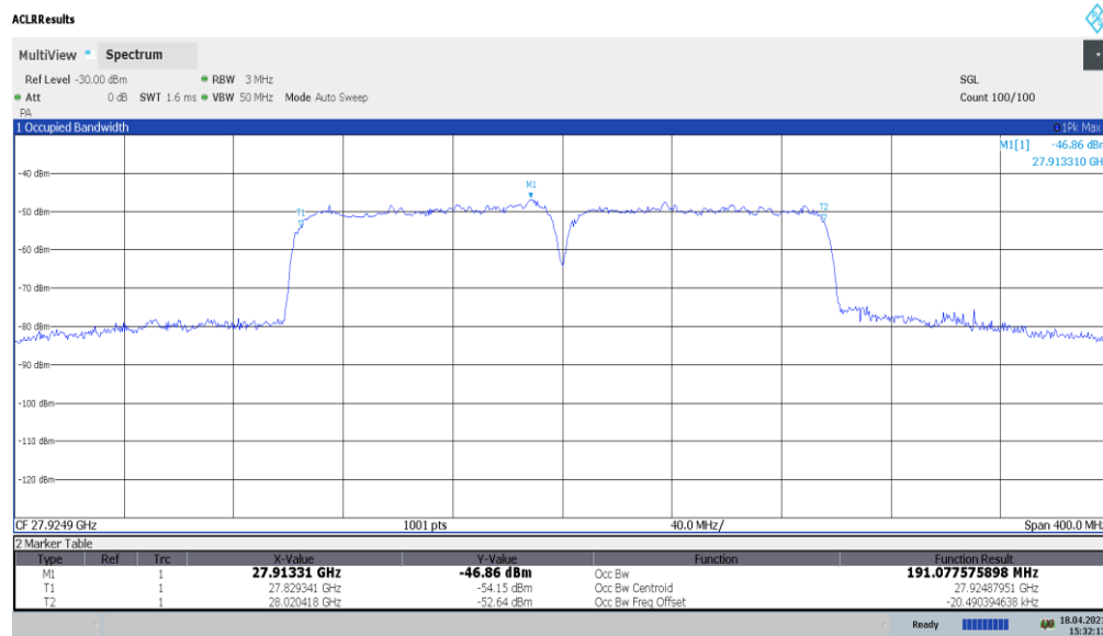
Plot 7-7. Ant 1 Occupied Bandwidth Plot (100MHz-2CC – 16QAM – Mid Channel)
