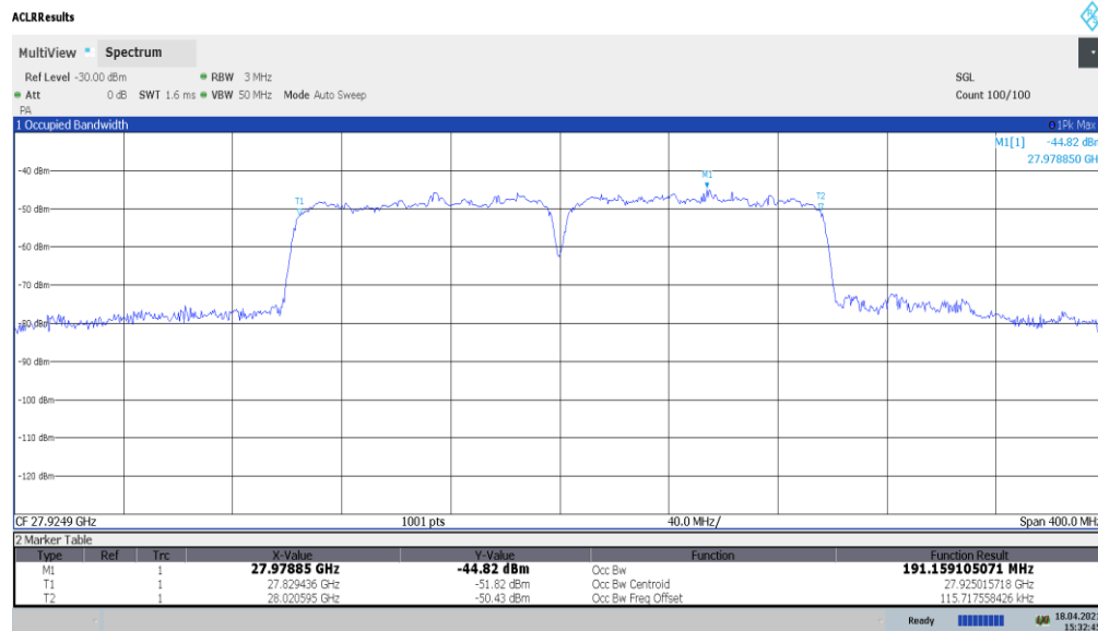
Plot 7-5. Ant 1 Occupied Bandwidth Plot (100MHz-2CC – QPSK – Mid Channel)
