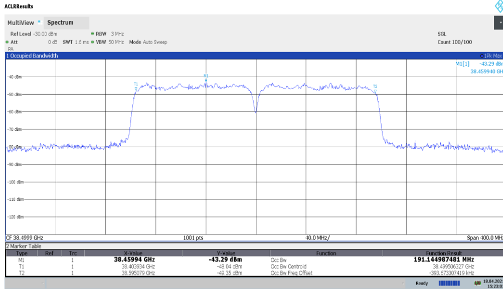
Plot 7-24. Ant 1 Occupied Bandwidth Plot (100MHz-2CC – 64QAM – Mid Channel)
