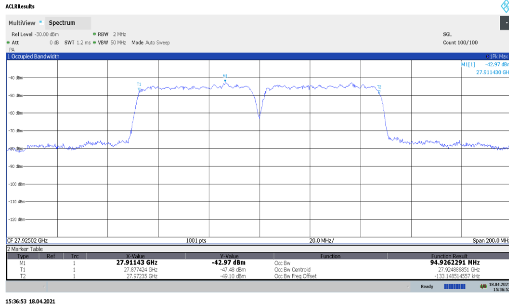
Plot 7-14. Ant 1 Occupied Bandwidth Plot (50MHz-2CC – pi/2-BPSK – Mid Channel)
