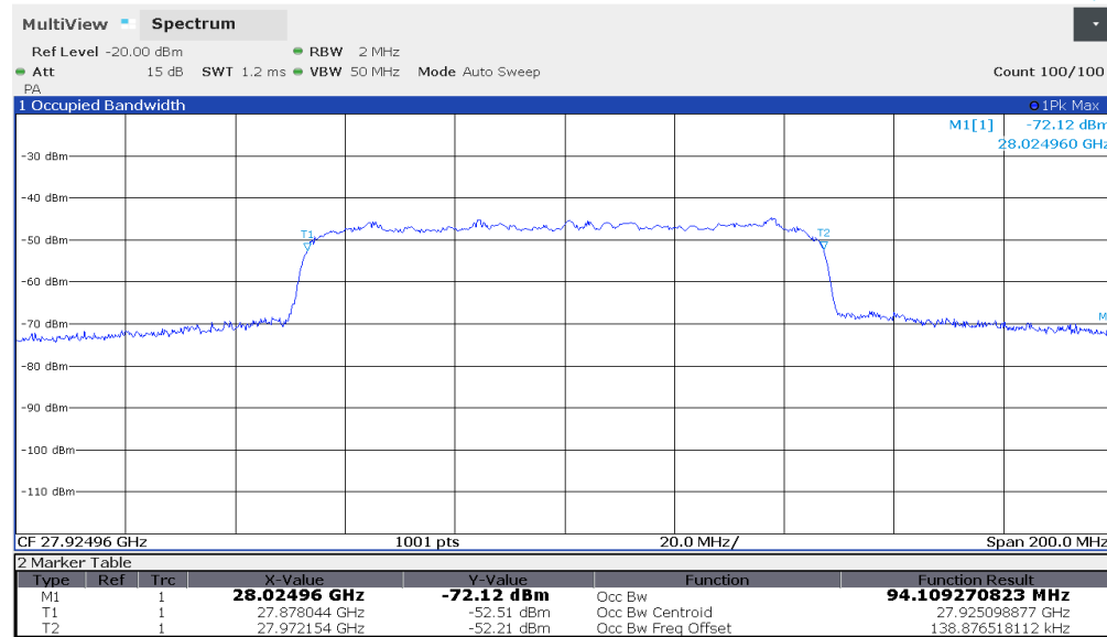
Plot 7-4. Ant 1 Occupied Bandwidth Plot (100MHz-1CC – 64QAM – Mid Channel)
