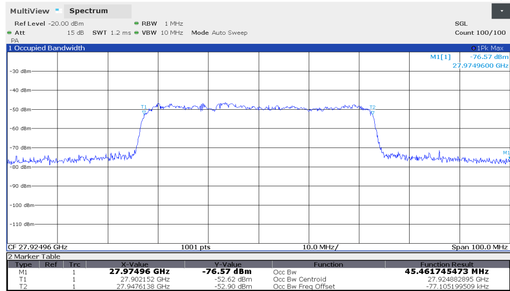
Plot 7-11. Ant 1 Occupied Bandwidth Plot (50MHz-1CC – 16QAM – Mid Channel)
