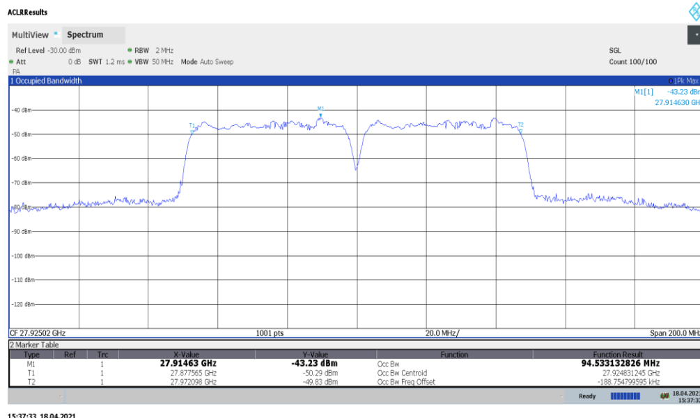
Plot 7-15. Ant 1 Occupied Bandwidth Plot (50MHz-2CC – 16QAM – Mid Channel)
