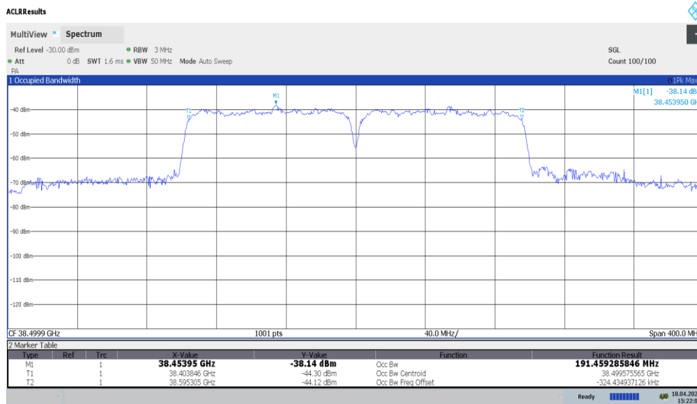
Plot 7-21. Ant 1 Occupied Bandwidth Plot (100MHz-2CC – QPSK – Mid Channel)
