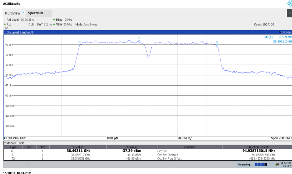
Plot 7-30. Ant 1 Occupied Bandwidth Plot (50MHz-2CC – pi/2-BPSK – Mid Channel)
