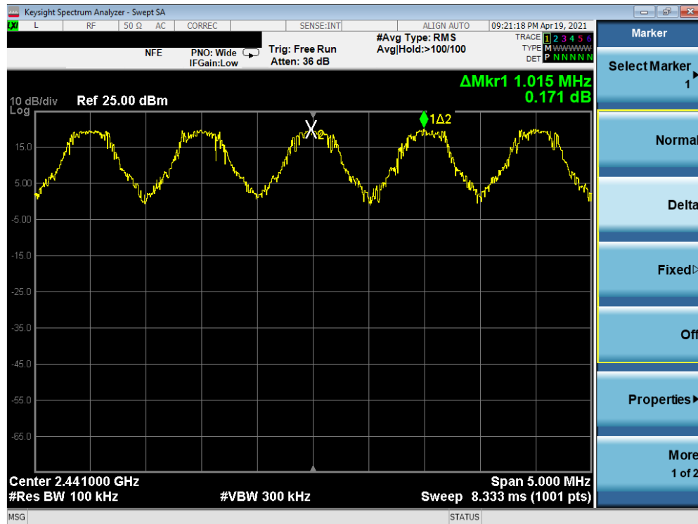
Plot 7-99. Channel Spacing Plot (Bluetooth)
