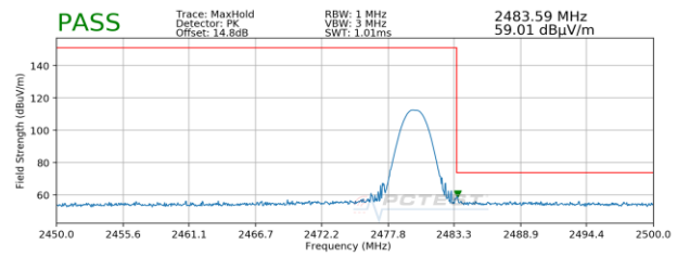
Plot 7-119. Radiated Restricted Upper Band Edge Measurement (Peak)
