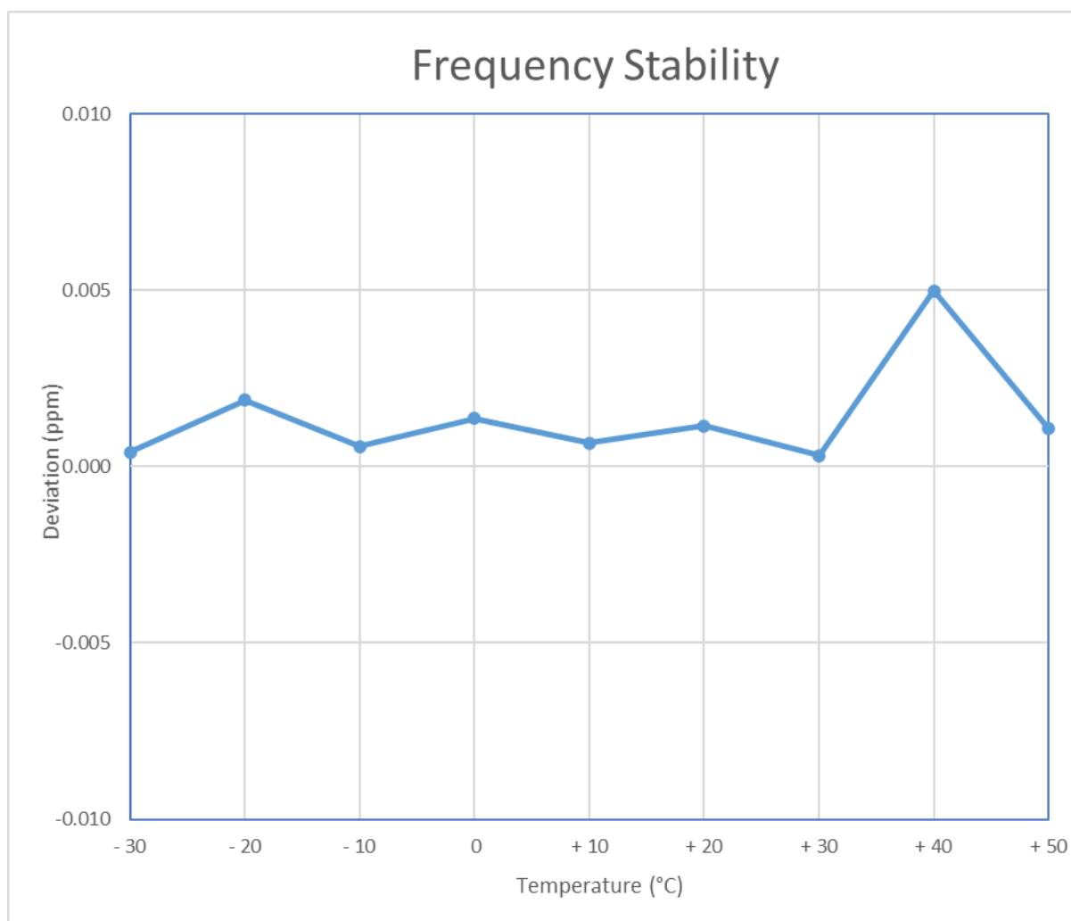
Figure 7-1. Frequency Stability Graph (n261)
