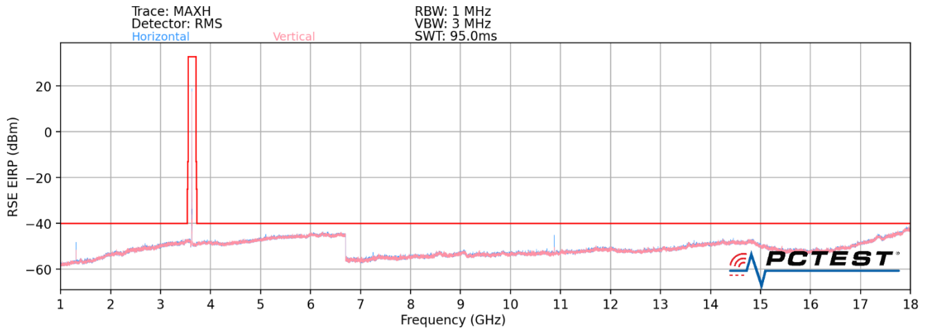
Plot 7-58. Radiated Spurious Plot (LTE Band 48) – CLOSED
