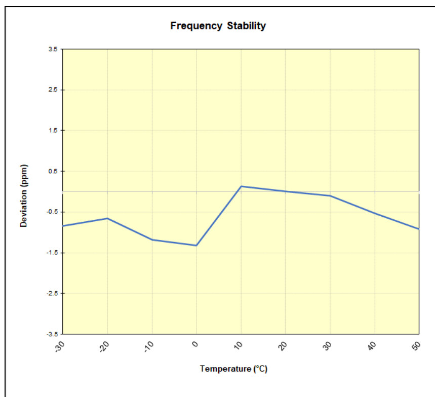
Plot 7-67. LTE Band 48 Frequency Stability Chart
