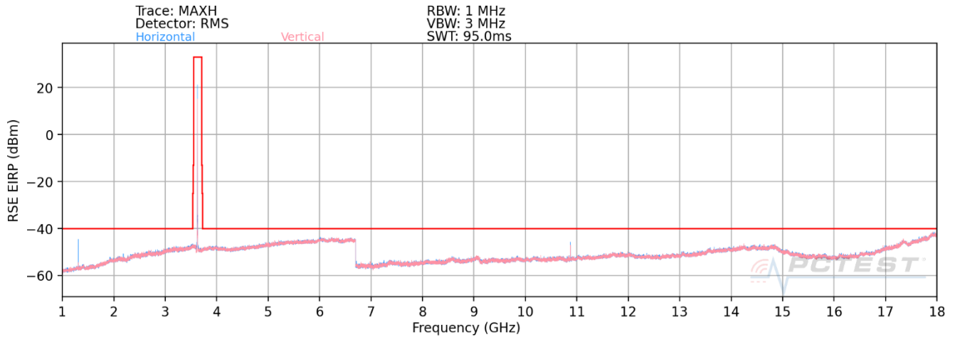
Plot 7-55. Radiated Spurious Plot (LTE Band 48) – OPEN
