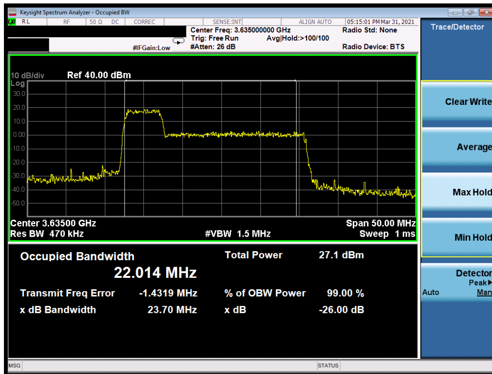
Plot 7-16. Occupied Bandwidth Plot (ULCA LB48 - 20+5MHz 16-QAM - Full RB Configuration)
