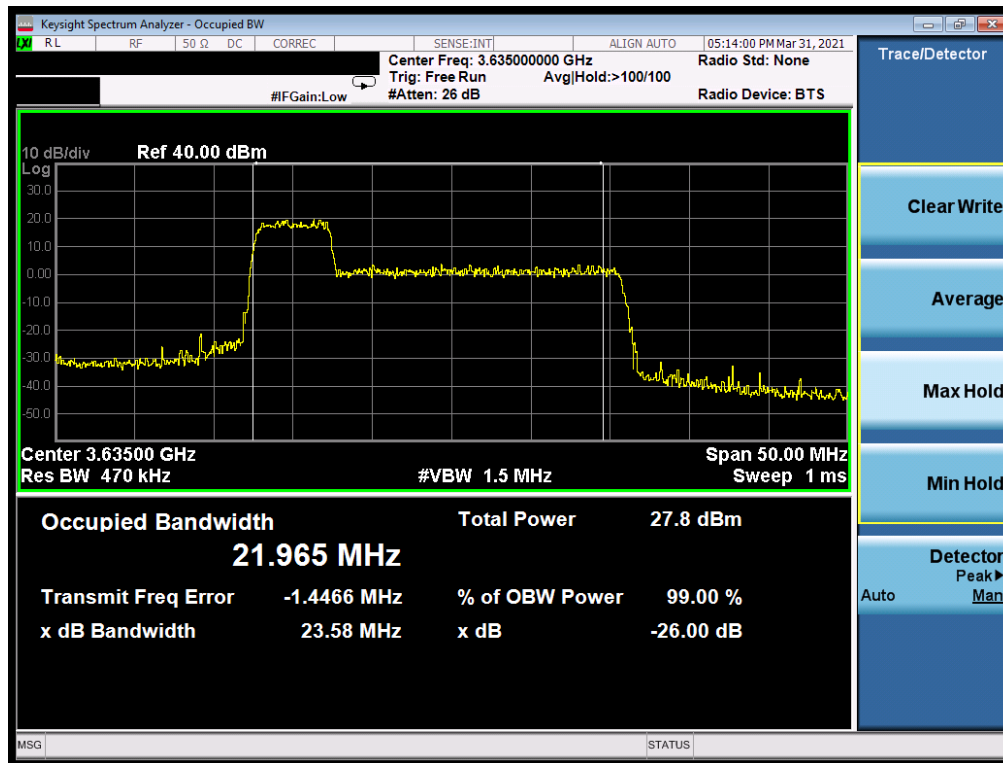
Plot 7-15. Occupied Bandwidth Plot (ULCA LB48 - 20+5MHz QPSK - Full RB Configuration)
