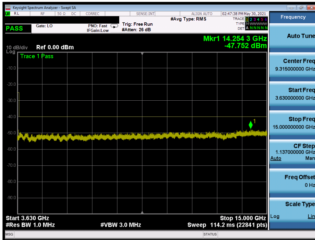
Plot 7-42. Conducted Spurious Plot (ULCA LB48 - 20+20MHz QPSK - Low Channel)
