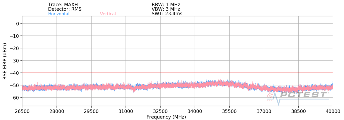
Plot 7-60. Radiated Spurious Plot (LTE Band 48) – CLOSED
