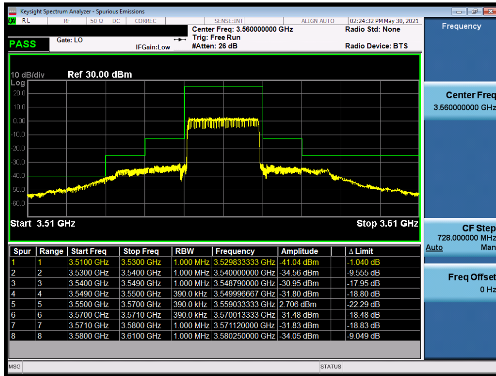
Plot 7-29. Channel Edge Plot (LTE Band 48 - 20MHz QPSK - Low Channel)
