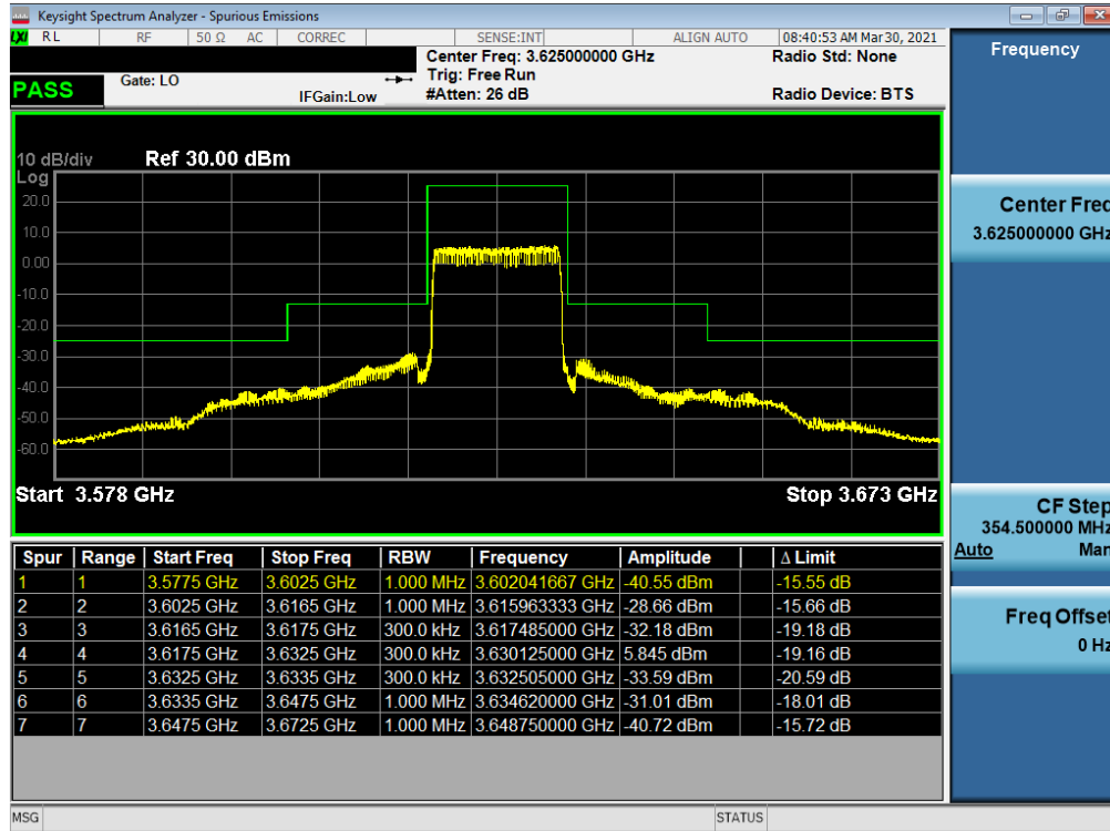
Plot 7-33. Channel Edge Plot (LTE Band 48 - 15MHz QPSK - Mid Channel)
