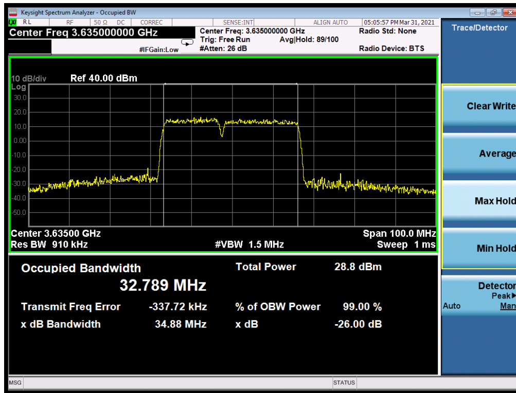
Plot 7-11. Occupied Bandwidth Plot (ULCA LB48 - 20+15MHz QPSK - Full RB Configuration)
