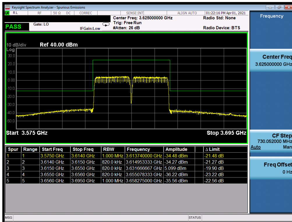
Plot 7-53. Channel Edge Plot (LTE Band 48 – 20+20MHz QPSK - Mid Channel)
