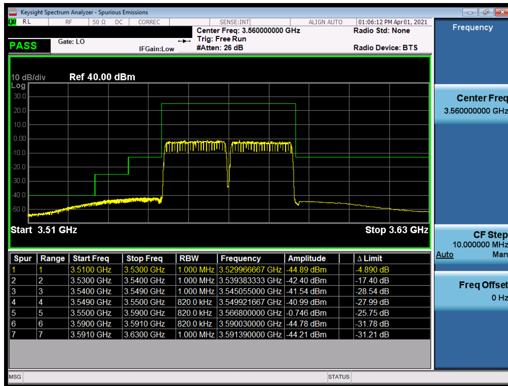
Plot 7-52. Channel Edge Plot (LTE Band 48 – 20+20MHz QPSK - Low Channel)
