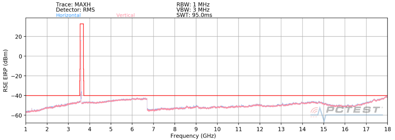
Plot 7-61. Radiated Spurious Plot (ULCA LB48) Low Channel – OPEN
