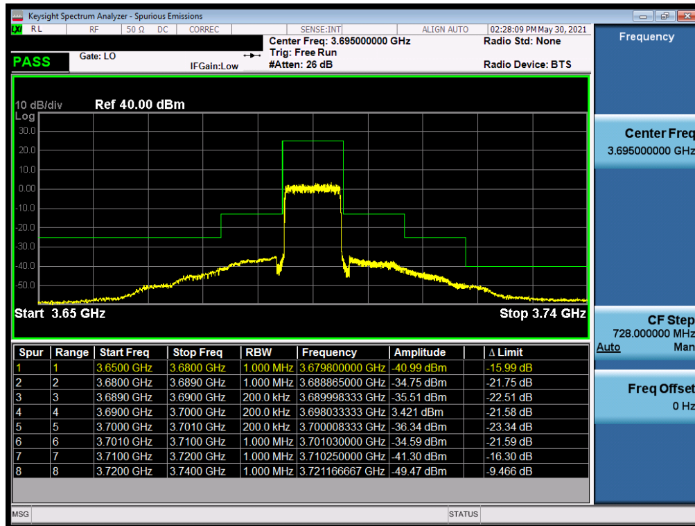
Plot 7-37. Channel Edge Plot (LTE Band 48 - 10MHz QPSK - High Channel)
