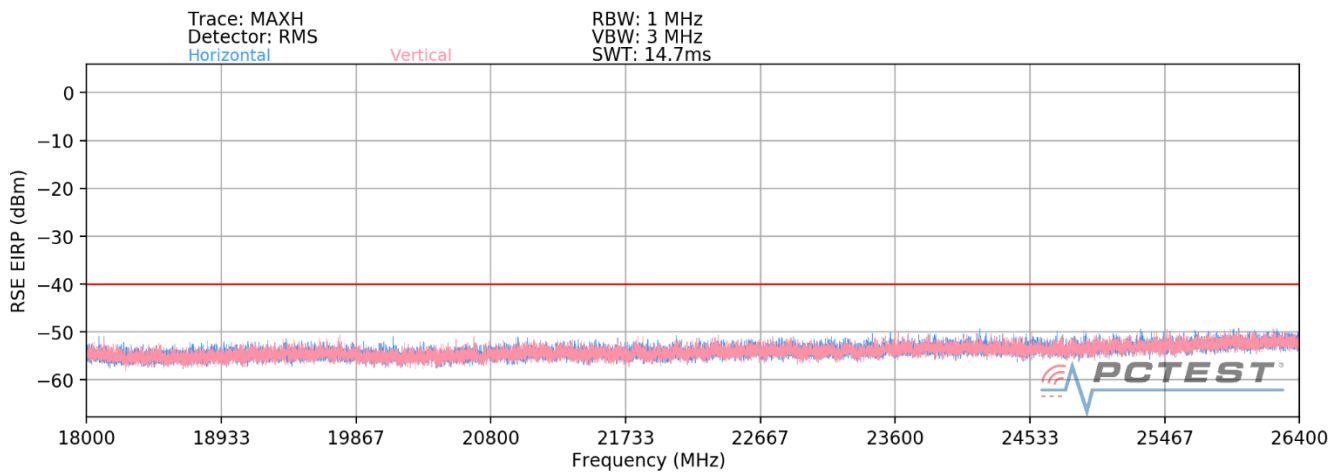
Plot 7-56. Radiated Spurious Plot (LTE Band 48) – OPEN
