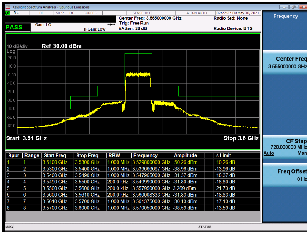
Plot 7-35. Channel Edge Plot (LTE Band 48 - 10MHz QPSK - Low Channel)
