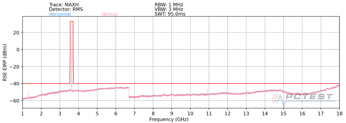
Plot 7-62. Radiated Spurious Plot (ULCA LB48) Mid Channel – OPEN
