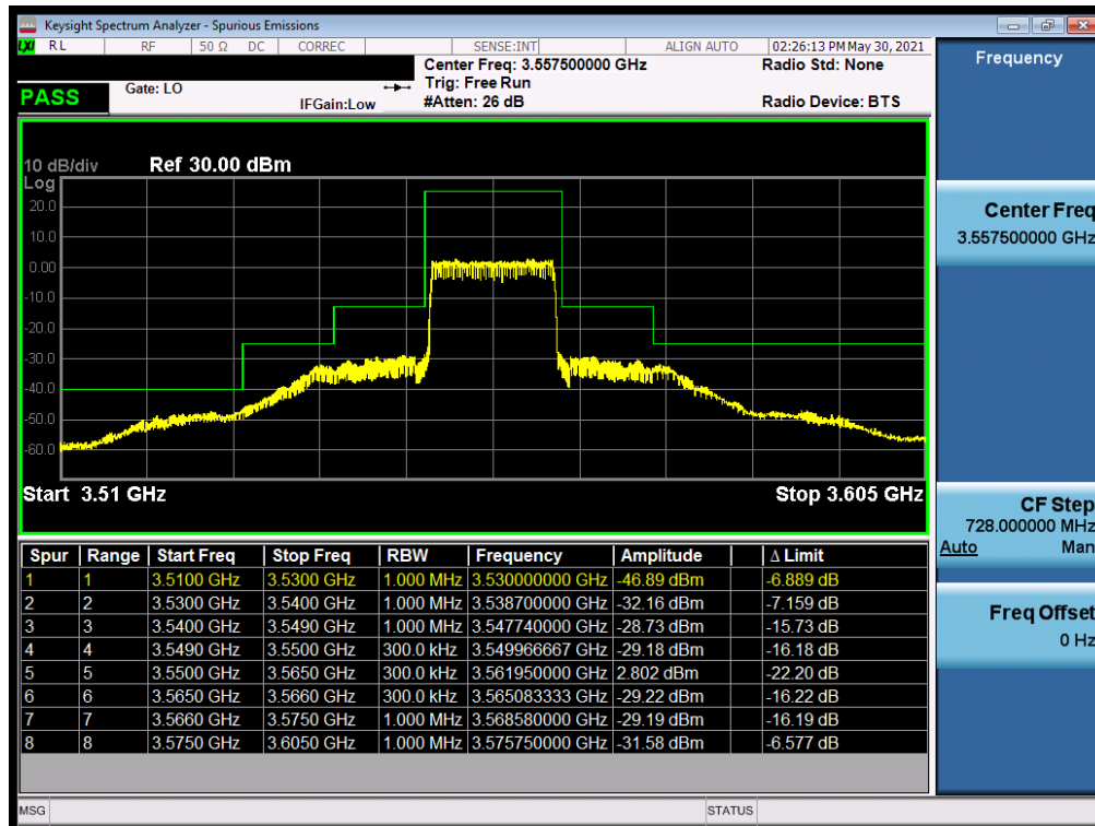
Plot 7-32. Channel Edge Plot (LTE Band 48 - 15MHz QPSK - Low Channel)
