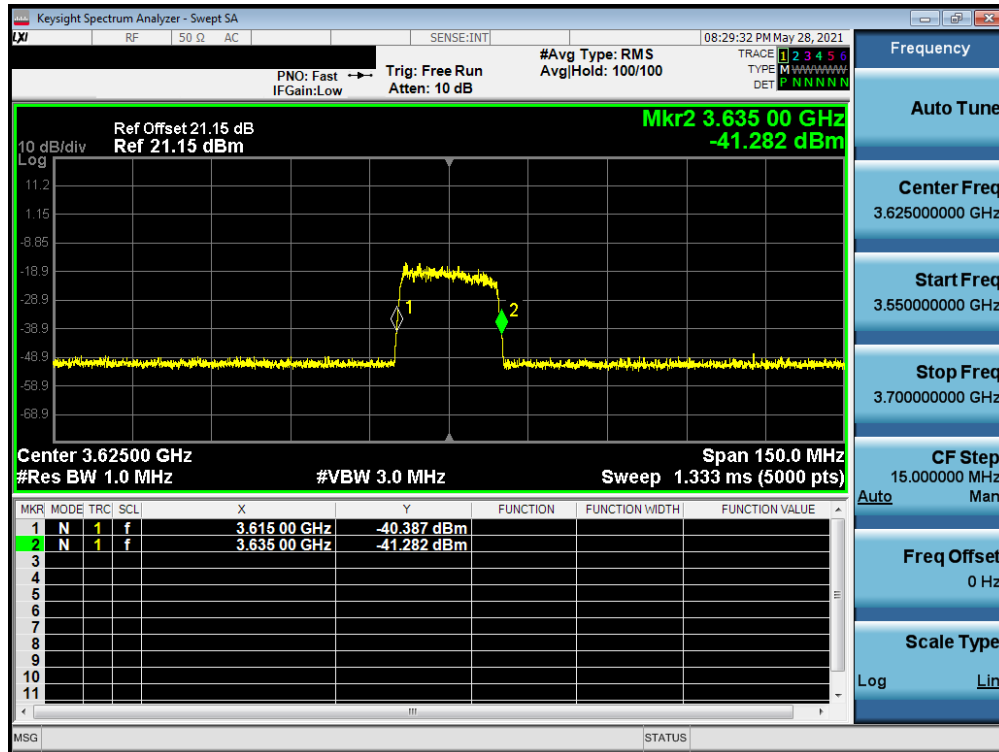
Plot 7-68. Run#1 End User Device Frequency of Operations
