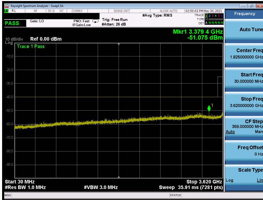
Plot 7-48. Conducted Spurious Plot (ULCA LB48 - 20+20MHz QPSK - High Channel)
