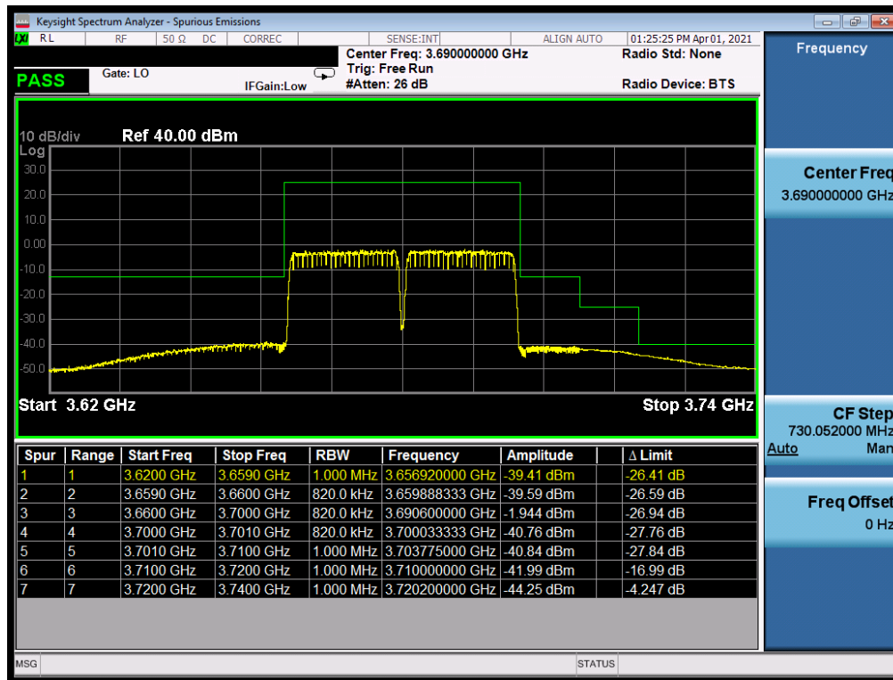
Plot 7-54. Channel Edge Plot (LTE Band 48 – 20+20MHz QPSK - High Channel)
