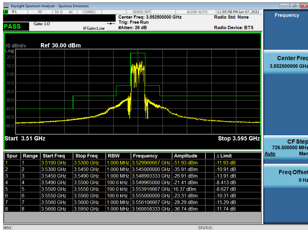
Plot 7-38. Channel Edge Plot (LTE Band 48 - 5MHz QPSK - Low Channel)
