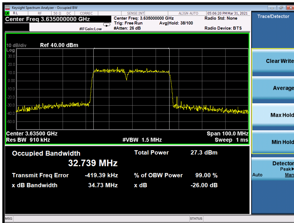
Plot 7-12. Occupied Bandwidth Plot (ULCA LB48 - 20+15MHz 16-QAM - Full RB Configuration)
