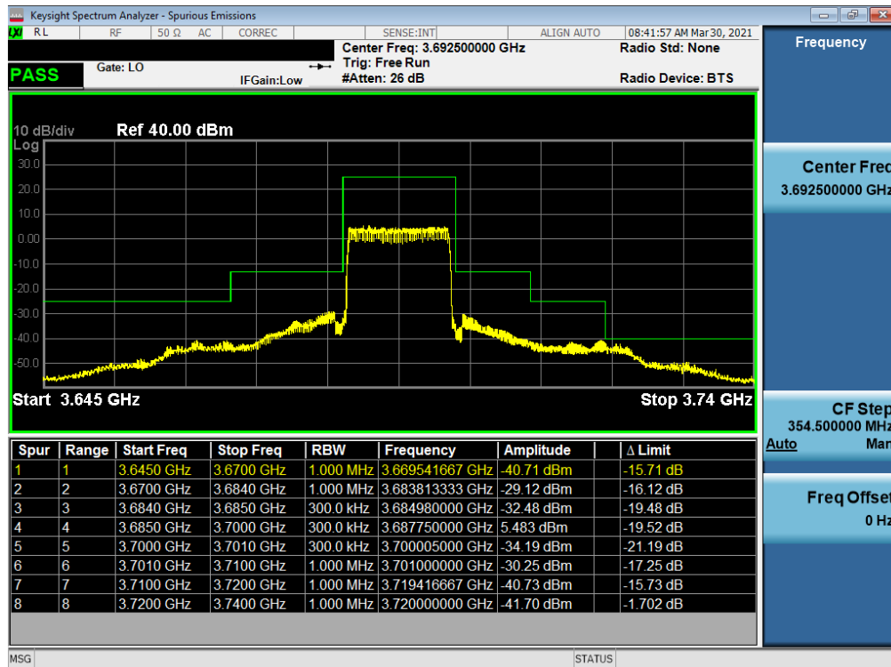
Plot 7-34. Channel Edge Plot (LTE Band 48 - 15MHz QPSK - High Channel)
