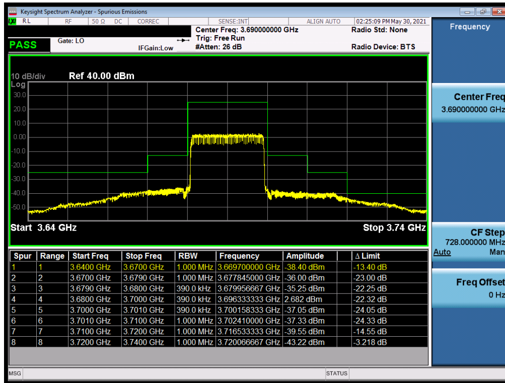
Plot 7-31. Channel Edge Plot (LTE Band 48 - 20MHz QPSK - High Channel)
