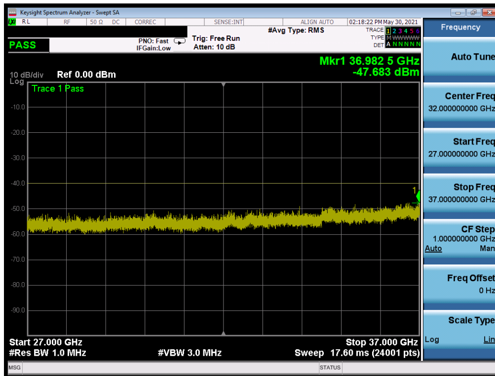
Plot 7-20. Conducted Spurious Plot (LTE Band 48 - 20MHz QPSK - Low Channel)
