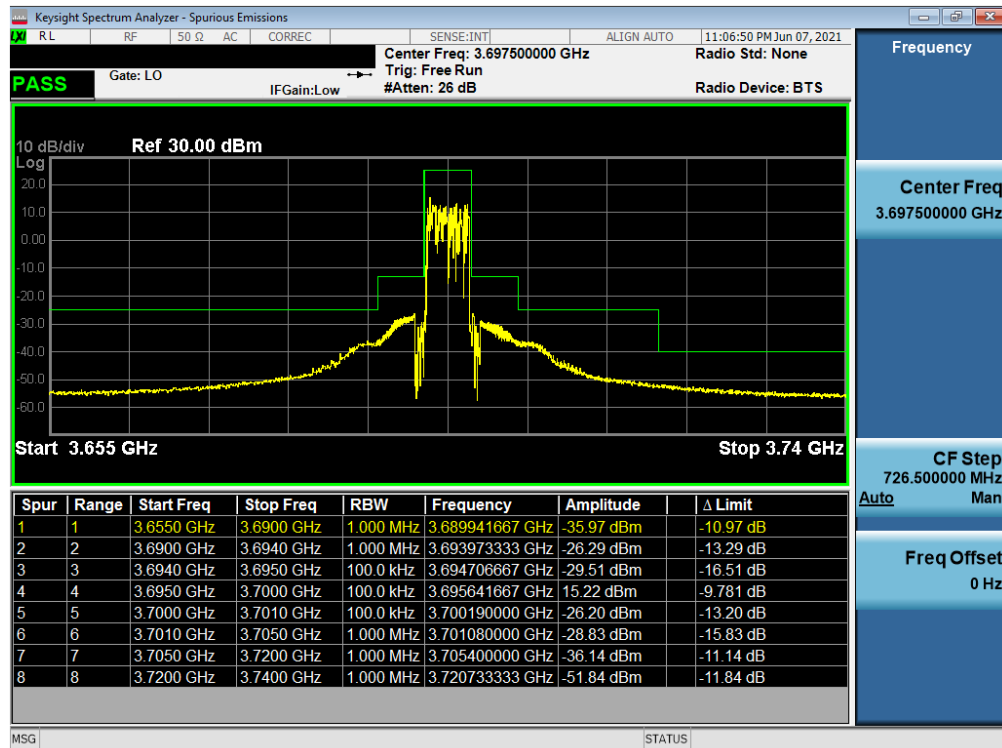
Plot 7-40. Channel Edge Plot (LTE Band 48 - 5MHz QPSK - High Channel)
