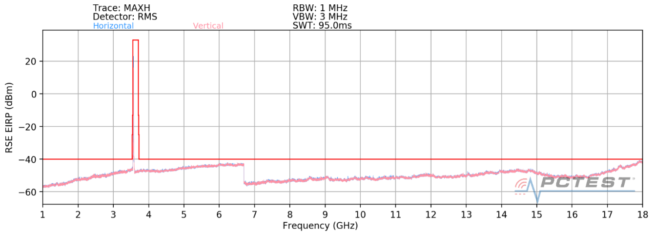
Plot 7-64. Radiated Spurious Plot (ULCA LB48) Low Channel – CLOSED
