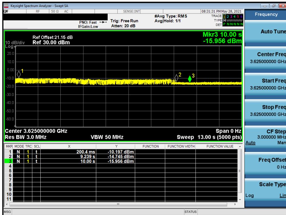
Plot 7-69. Run#1 End User Device Discontinues Operations within 10s
