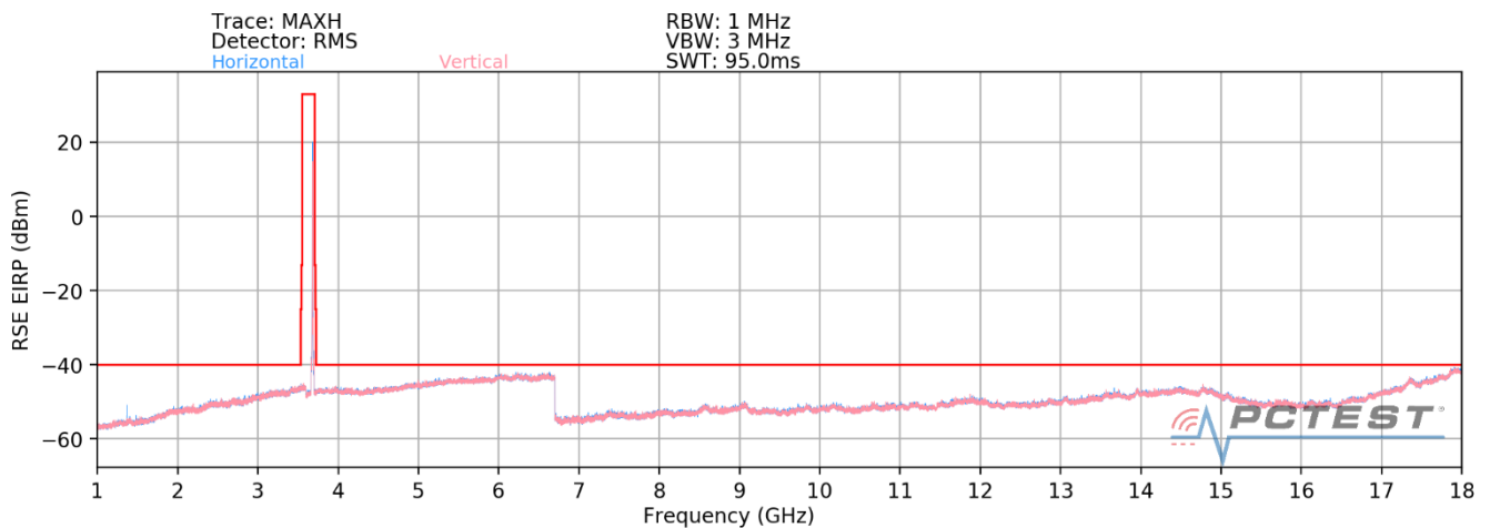
Plot 7-66. Radiated Spurious Plot (ULCA LB48) High Channel - CLOSED
