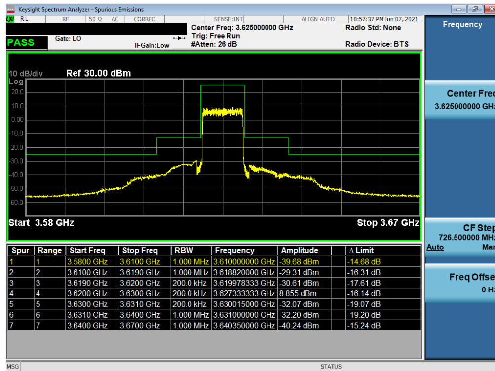
Plot 7-36. Channel Edge Plot (LTE Band 48 - 10MHz QPSK - Mid Channel)
