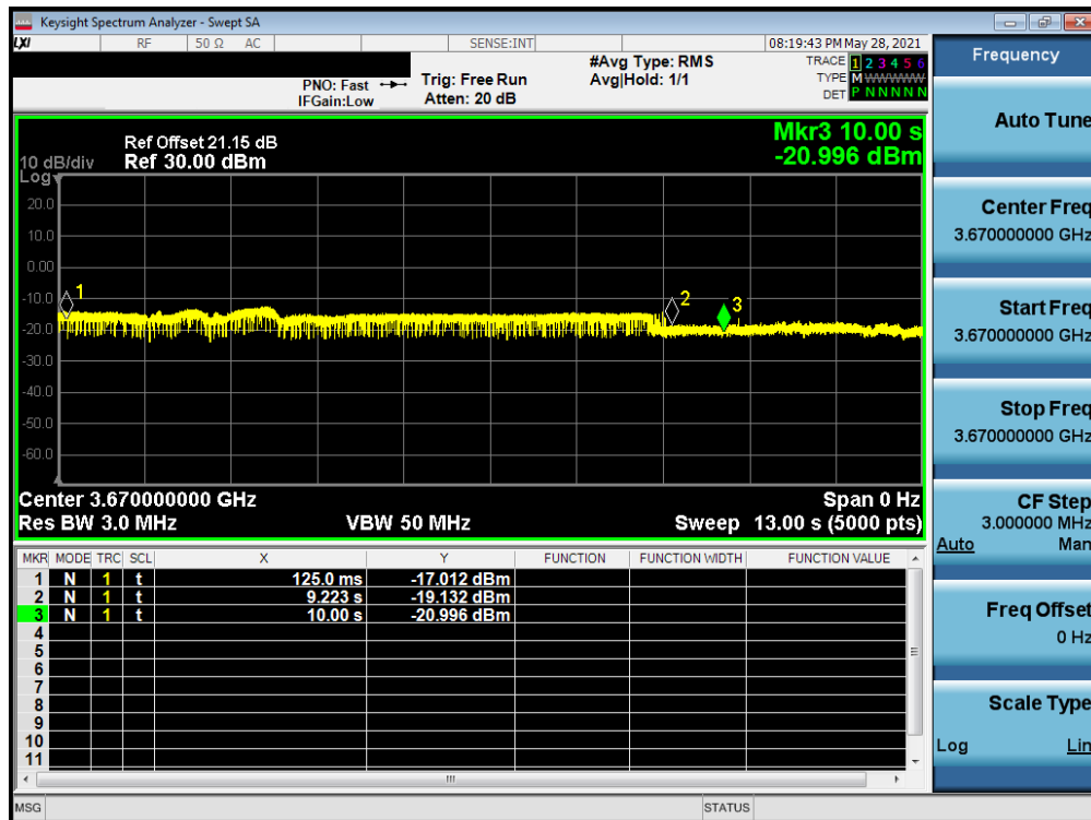
Plot 7-71. Run#2 End User Device Discontinues Operations within 10s
