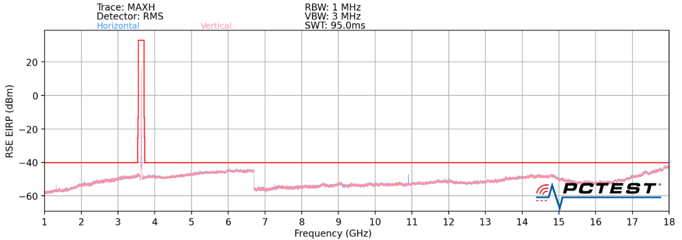
Plot 7-65. Radiated Spurious Plot (ULCA LB48) Mid Channel – CLOSED
