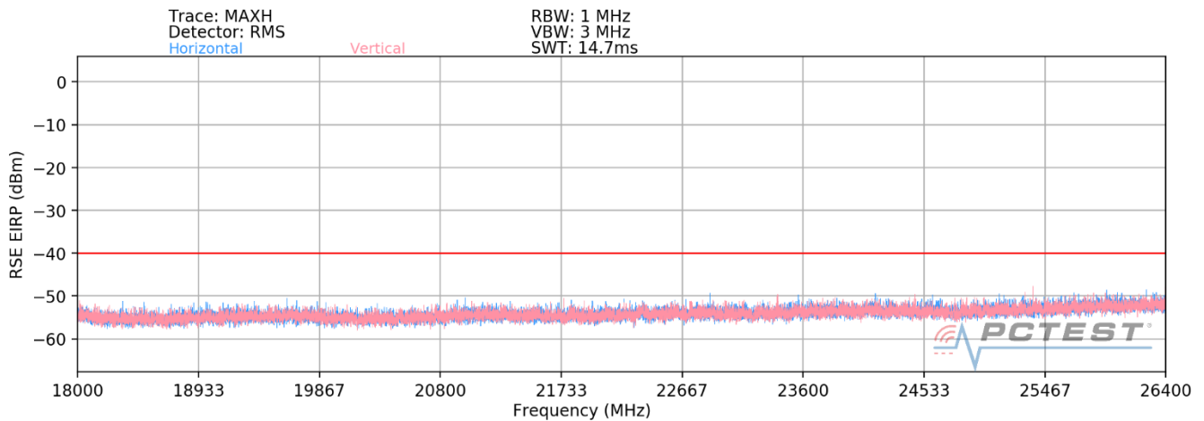
Plot 7-59. Radiated Spurious Plot (LTE Band 48) – CLOSED
