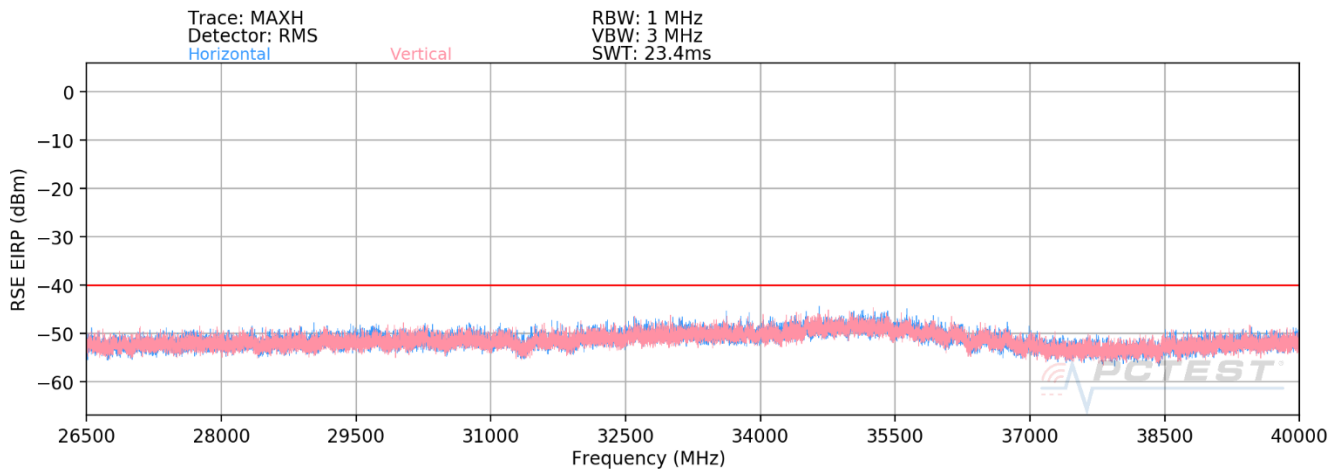
Plot 7-57. Radiated Spurious Plot (LTE Band 48) – OPEN
