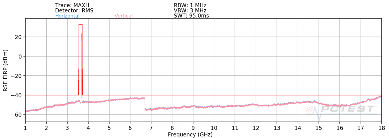
Plot 7-63. Radiated Spurious Plot (ULCA LB48) High Channel – OPEN
