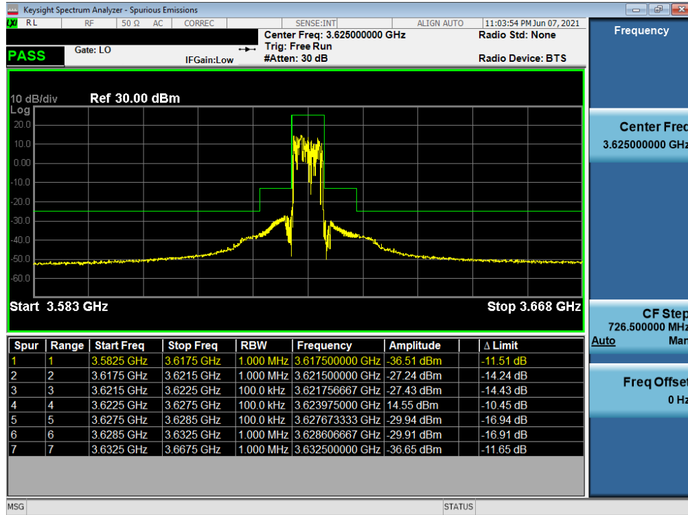
Plot 7-39. Channel Edge Plot (LTE Band 48 - 5MHz QPSK - Mid Channel)
