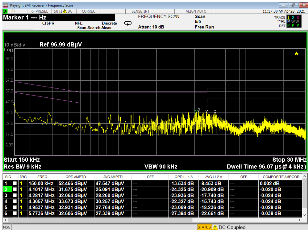
Plot 7-4. Line Conducted Plot
