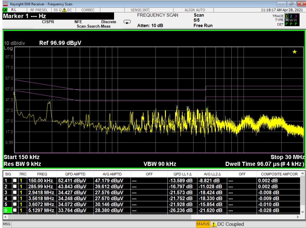
Plot 7-3. Line Conducted Plot
