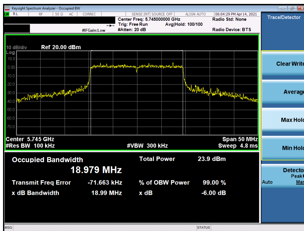
Plot 7-119. 6dB Bandwidth Plot MIMO ANT2 (20MHz BW 802.11ax – 242 Tones (UNII Band 3) – Ch. 149)
