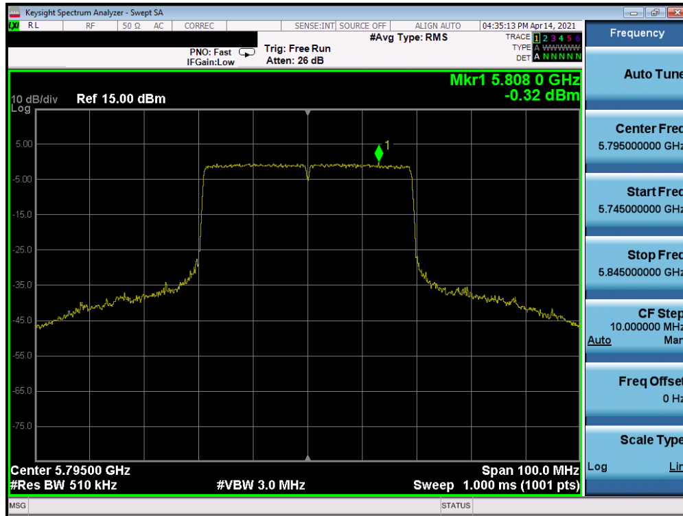
Plot 7-185. Power Spectral Density Plot MIMO ANT1 (40MHz BW 802.11ax – Full Tones (UNII Band 3) – Ch. 159)
