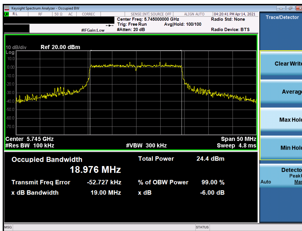
Plot 7-113. 6dB Bandwidth Plot MIMO ANT1 (20MHz BW 802.11ax – 242 Tones (UNII Band 3) – Ch. 149)
