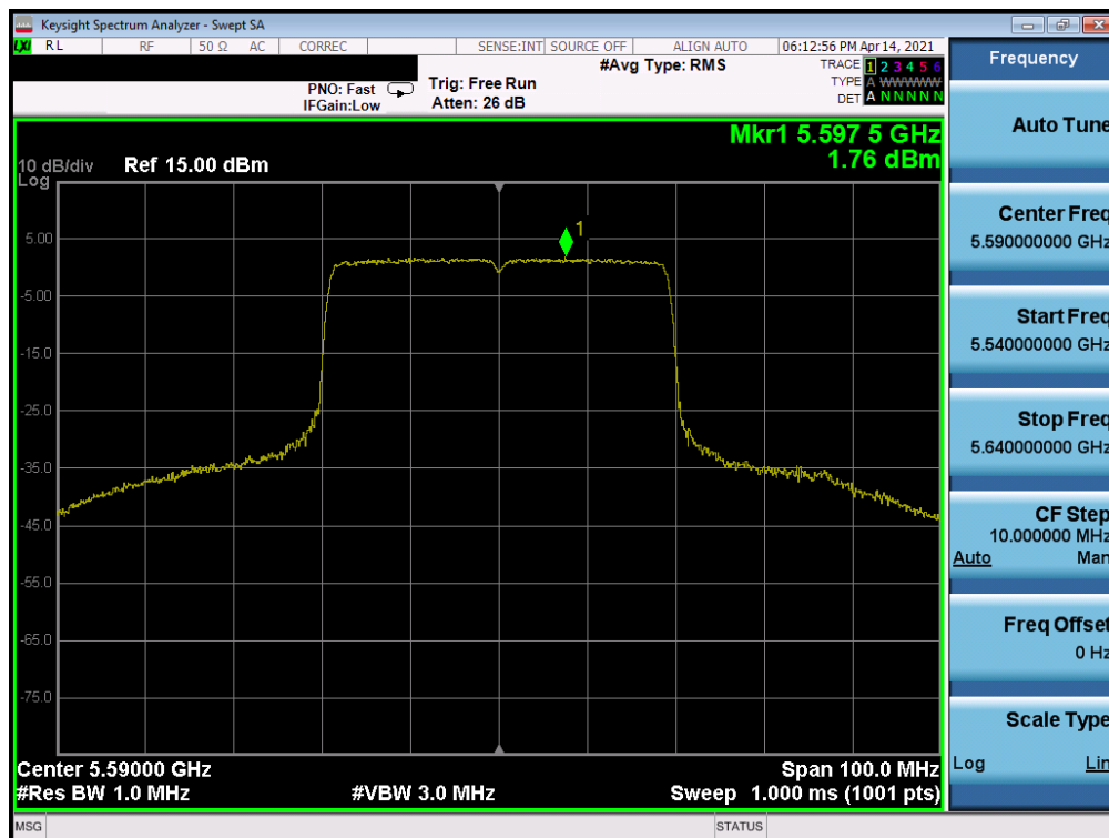
Plot 7-236. Power Spectral Density Plot MIMO ANT2 (40MHz BW 802.11ax – Full Tones (UNII Band 2C) – Ch. 118)
