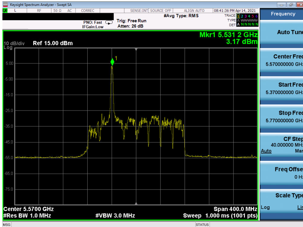
Plot 7-210. Power Spectral Density Plot MIMO ANT2 (160MHz BW(L) 802.11ax – 26 Tones (UNII Band 2C) – Ch. 114)
