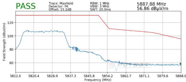
Plot 7-279. Radiated Upper Band Edge Plot MIMO (Peak - UNII Band 3 - 242 Tones)
