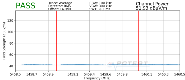
Plot 7-295. Radiated Lower Band Edge Plot MIMO (Average - UNII Band 2C - 996 Tones)
