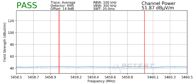
Plot 7-298. Radiated Lower Band Edge Plot MIMO with WCP (Average – UNII Band 2C – 996 Tones)
