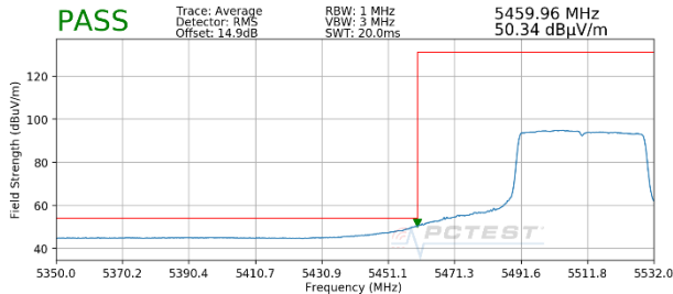
Plot 7-286. Radiated Lower Band Edge Plot MIMO (Average - UNII Band 2C - 484 Tones)
