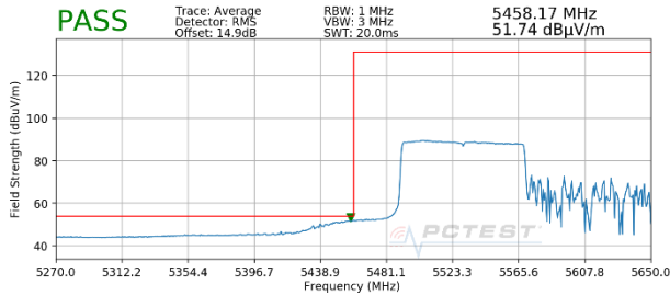
Plot 7-304. Radiated Lower Band Edge Plot MIMO (Average - UNII Band 2C - 996 Tones)
