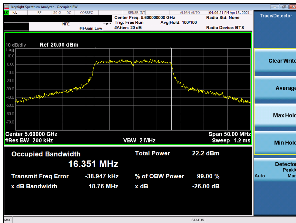
Plot 7-89. 26dB Bandwidth Plot MIMO ANT1 (802.11a (UNII Band 2C) – Ch. 120)
