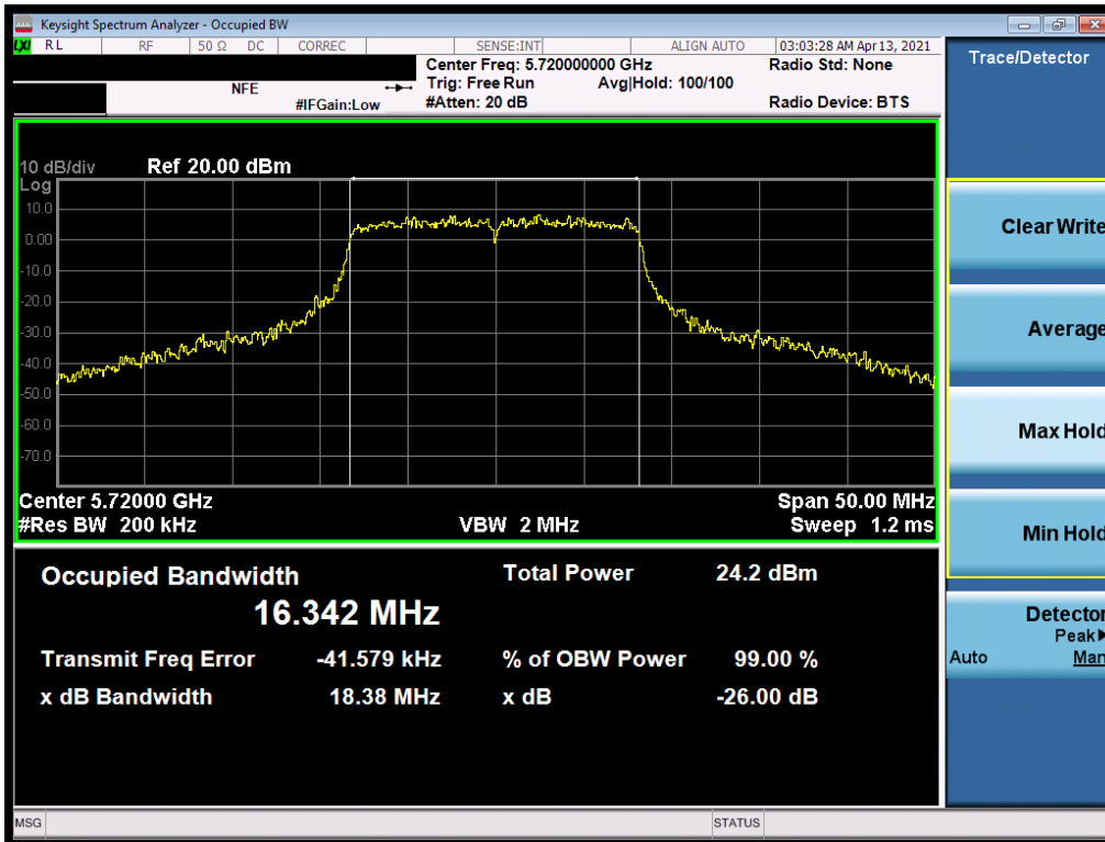
Plot 7-35. 26dB Bandwidth Plot SISO ANT1 (802.11a (UNII Band 2C) – Ch. 144)
