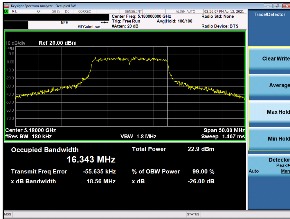
Plot 7-56. 26dB Bandwidth Plot MIMO ANT1 (802.11a (UNII Band 1) – Ch. 36)
