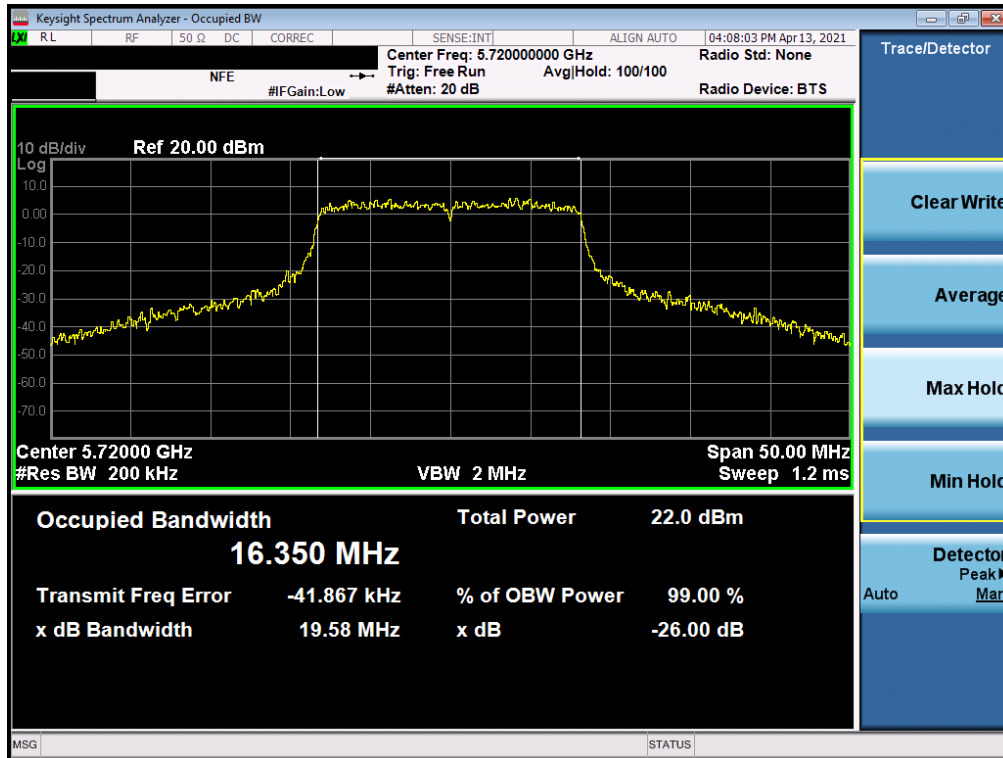
Plot 7-90. 26dB Bandwidth Plot MIMO ANT1 (802.11a (UNII Band 2C) – Ch. 144)
