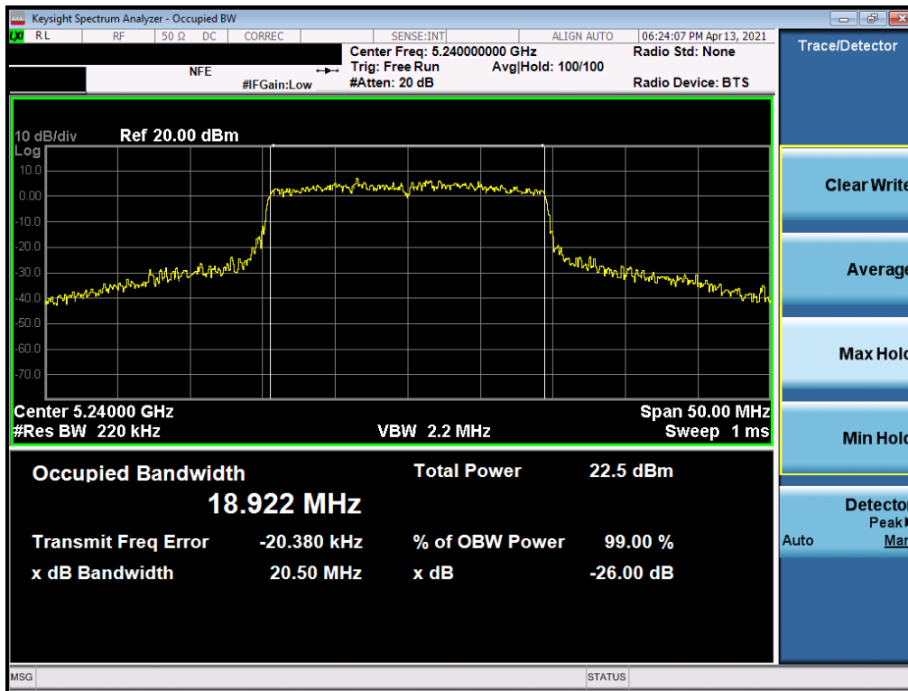
Plot 7-119. 26dB Bandwidth Plot MIMO ANT2 (20MHz BW 802.11ax (UNII Band 1) – Ch. 48)
