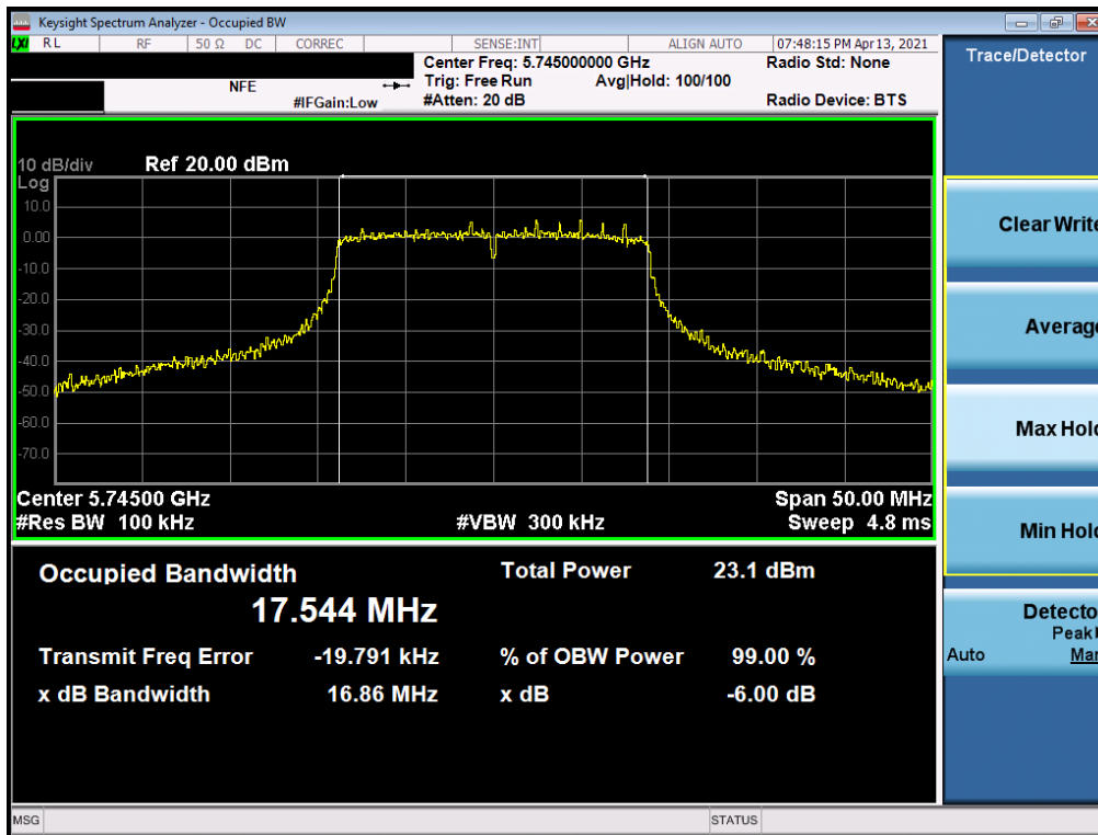
Plot 7-199. 6dB Bandwidth Plot MIMO ANT 2 (20MHz 802.11n (UNII Band 3) – Ch. 149)
