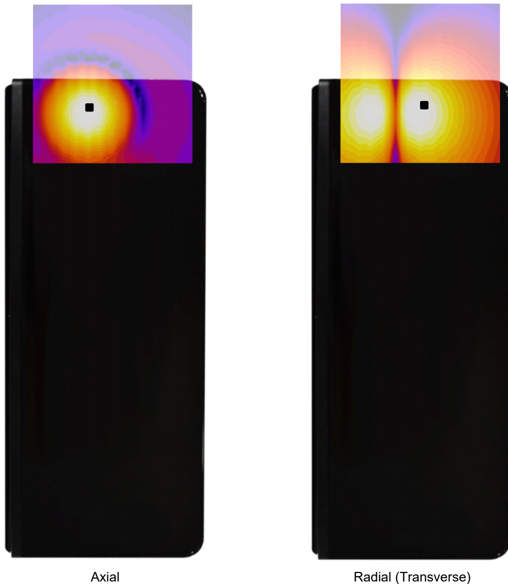
Figure 16-3 T-Coil Scan Overlay Magnetic Field Distributions
