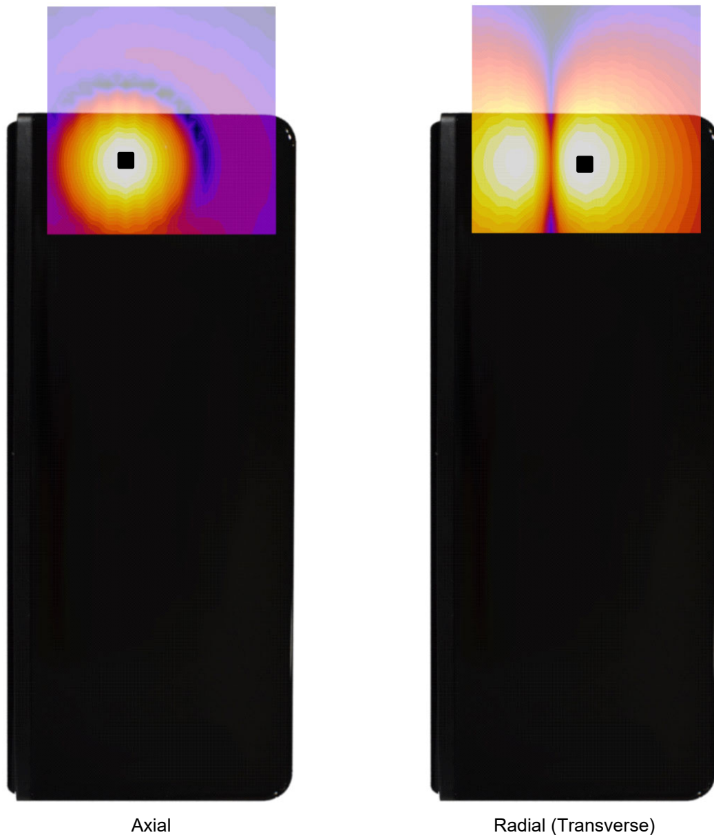
Figure 15-3 T-Coil Scan Overlay Magnetic Field Distributions
