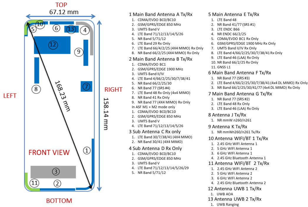
Figure C-1 DUT Antenna Locations – Closed
