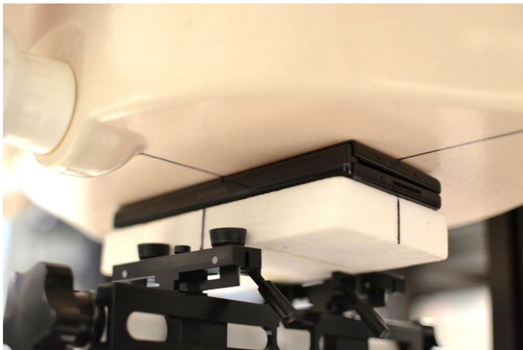
Figure C-9 SAR Test Setup Photo – Phablet Back Side at 0mm
