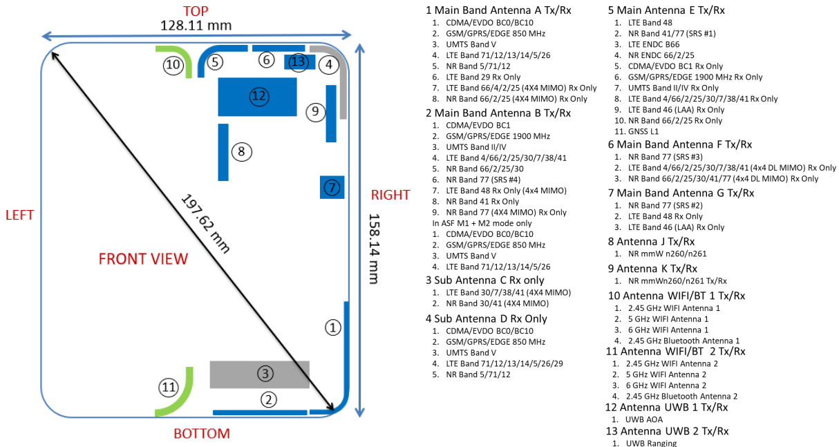
Figure C-2 DUT Antenna Locations - Open
