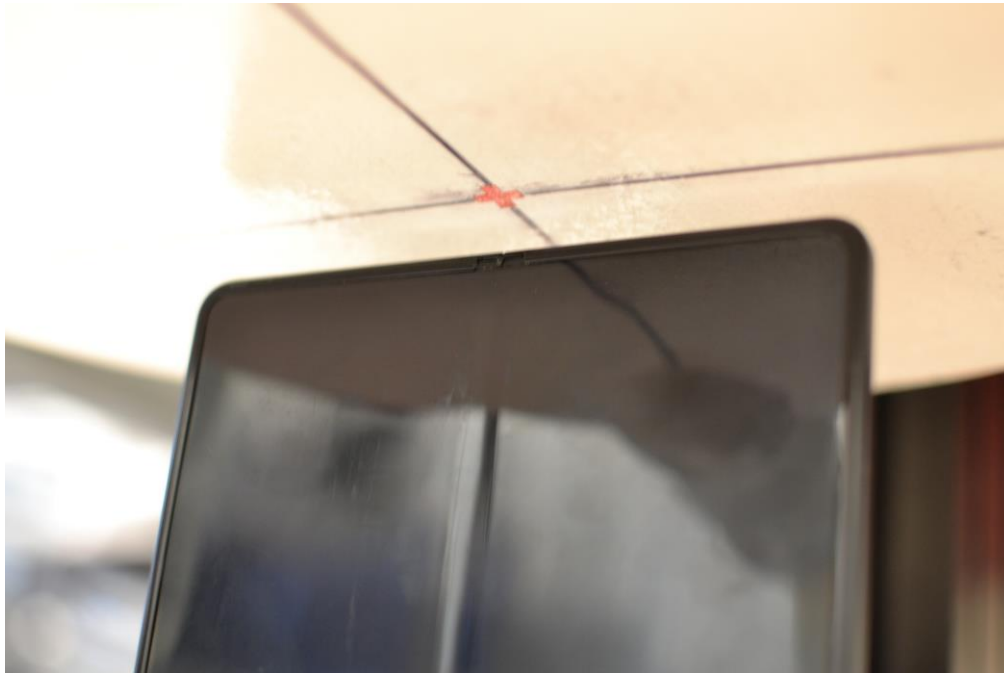
SAR Test Setup Photo 28– Open Configuration (UMPC), UMPC Body, Bottom Edge, 10 mm
