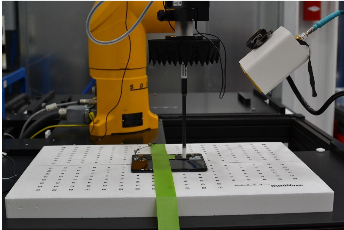
Test Setup Photo 11 – Power Density Setup Back Side (Figure 7-2)
