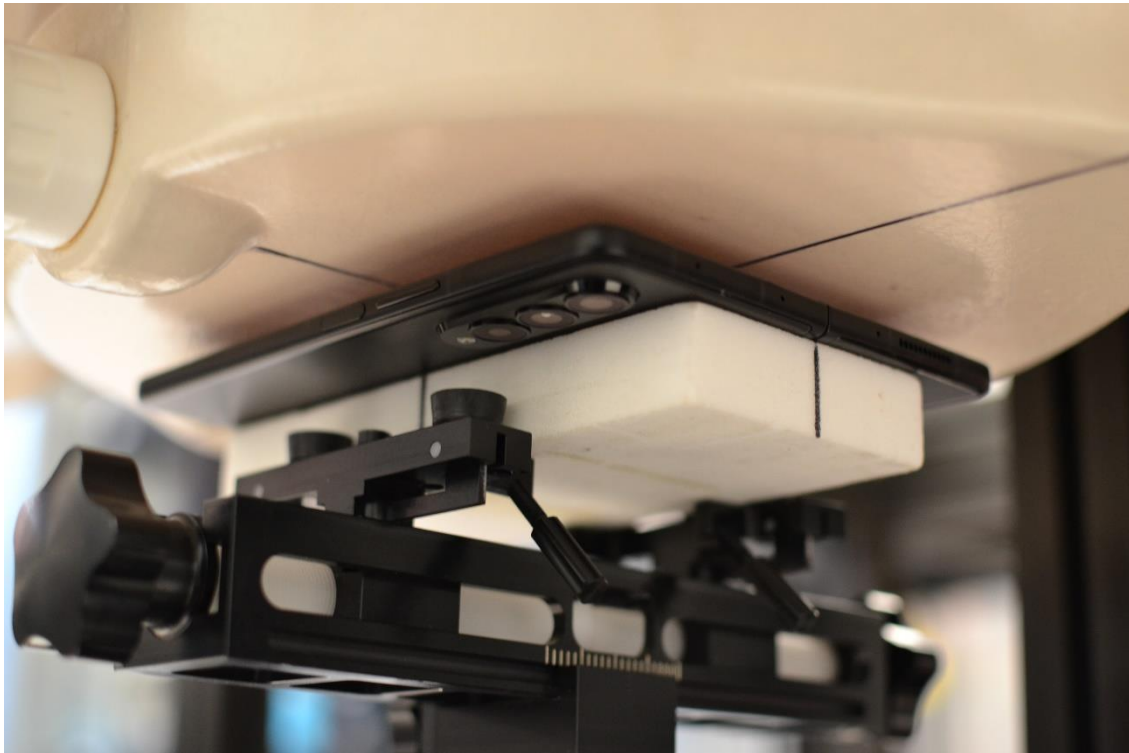
Test Setup Photo 6 – Folder Open, Front Side at 10 mm
