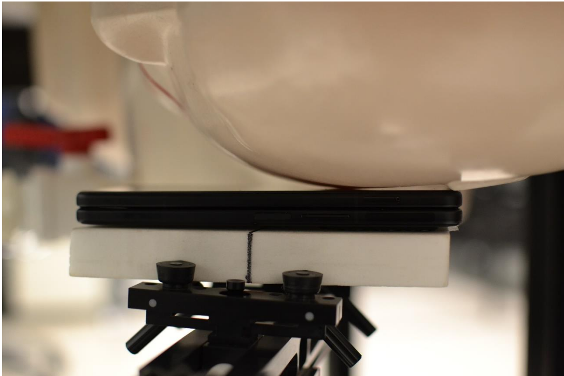
Test Setup Photo 10 – Folder Close, Left Head, Cheek
