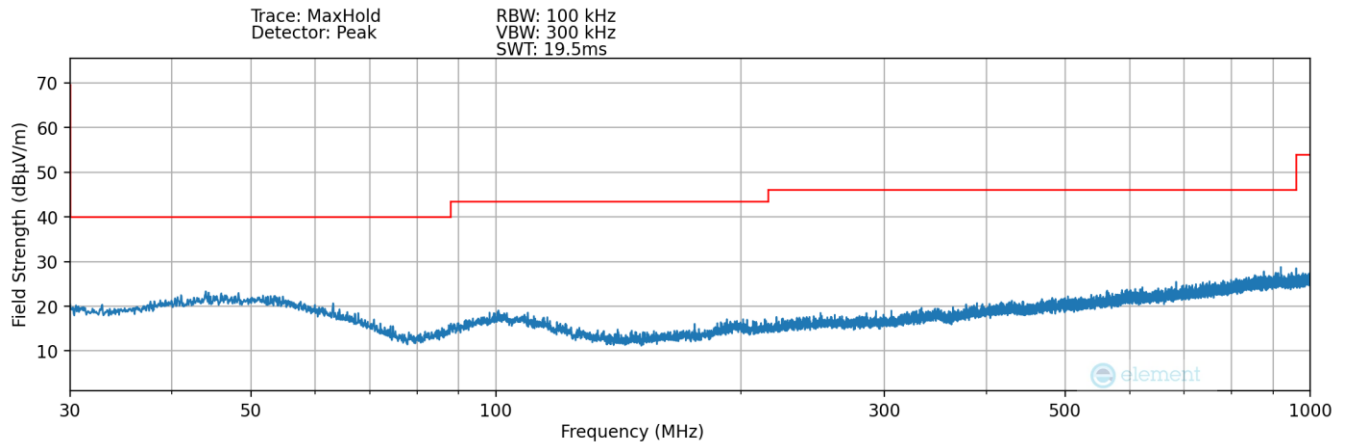
Plot 7-9. Radiated Spurious Plot 30MHz – 1GHz (Pol. H) – Closed
