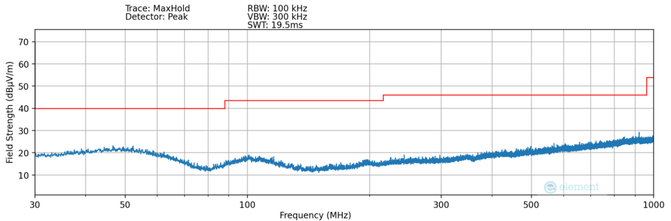
Plot 7-7. Radiated Spurious Plot 30MHz – 1GHz (Pol. H) – Open
