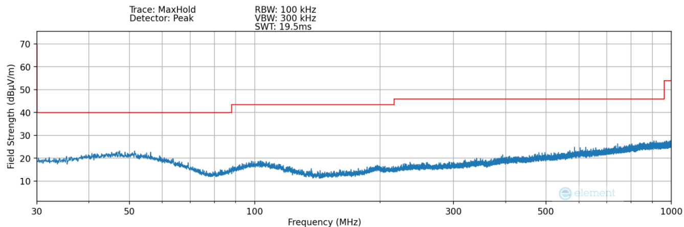
Plot 7-10. Radiated Spurious Plot 30MHz – 1GHz (Pol. V) – Closed
