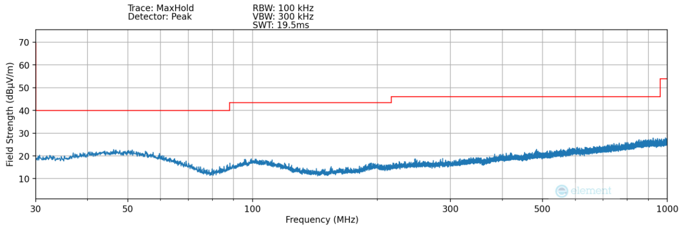
Plot 7-8. Radiated Spurious Plot 30MHz – 1GHz (Pol. V) – Open
