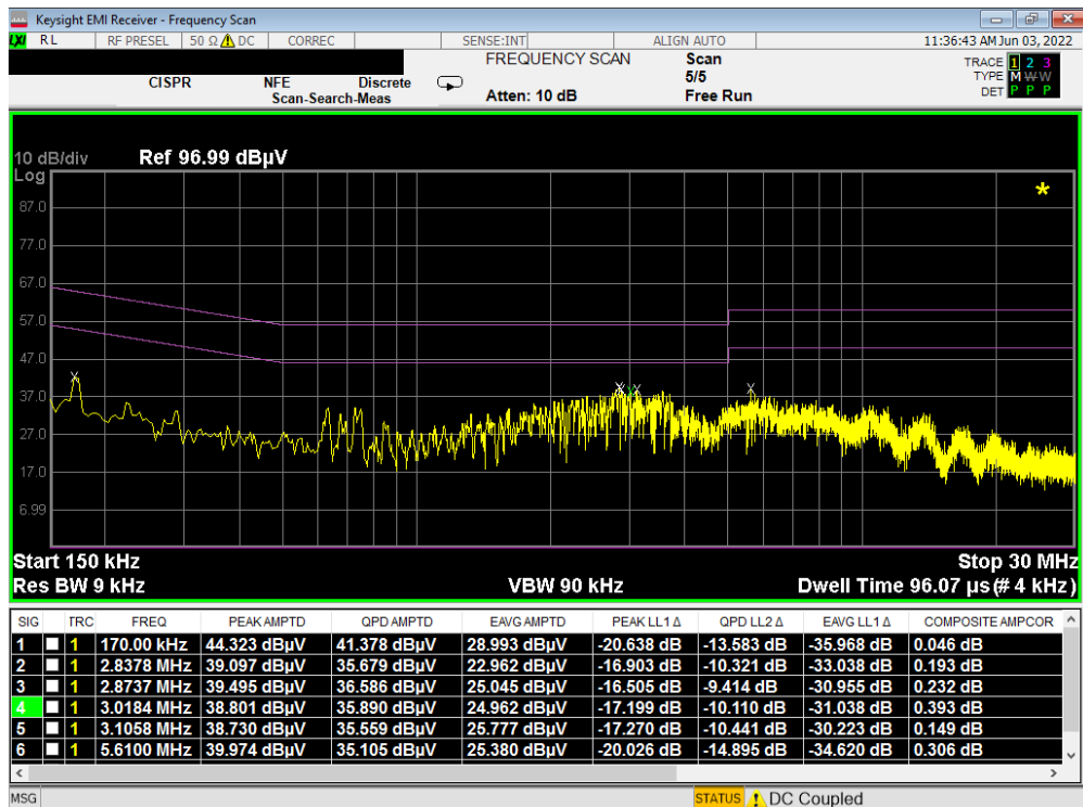
Plot 7-11. Line-Conducted Test Plot (N) - Device to Device
