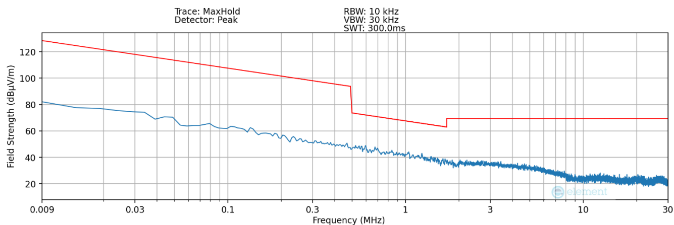
Plot 7-9. Radiated Spurious Plot 9kHz – 30MHz (Pol. Z – Digitizer – Click)
