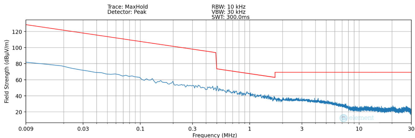
Plot 7-8 Radiated Spurious Plot 9kHz – 30MHz (Pol. Y – Digitizer – Click)
