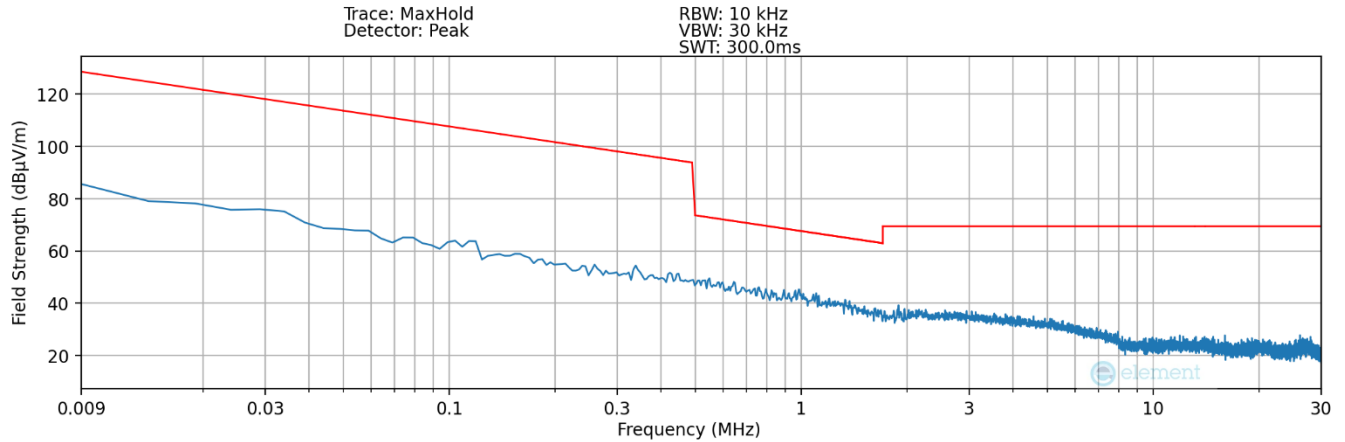
Plot 7-4. Radiated Spurious Plot 9kHz – 30MHz (Pol. X – Digitizer – Hover)
