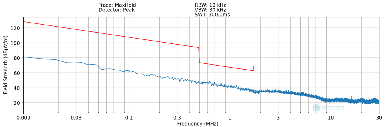
Plot 7-6. Radiated Spurious Plot 9kHz – 30MHz (Pol. Z– Digitizer – Hover)
