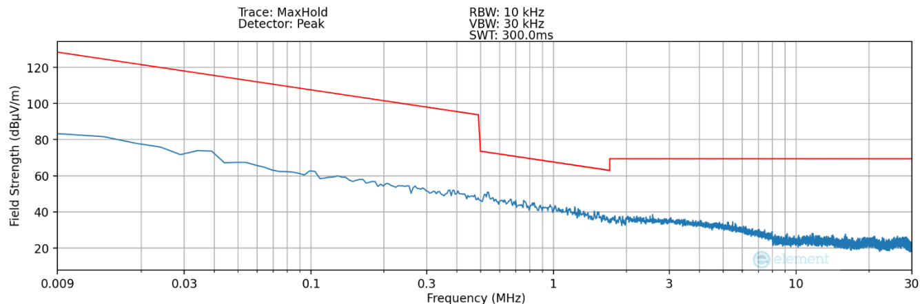
Plot 7-7. Radiated Spurious Plot 9kHz – 30MHz (Pol. X – Digitizer – Click)
