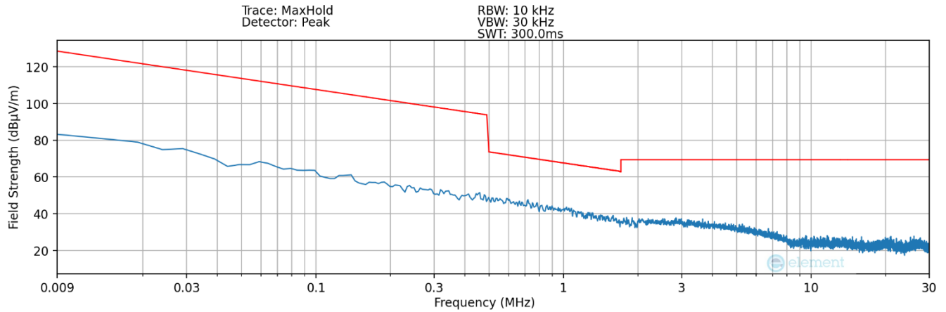
Plot 7-5Radiated Spurious Plot 9kHz – 30MHz (Pol. Y – Digitizer – Hover)
