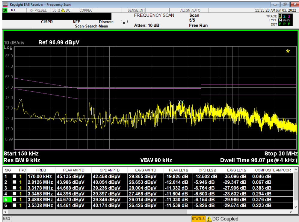
Plot 7-10. Line-Conducted Test Plot (L1) - Device to Device
