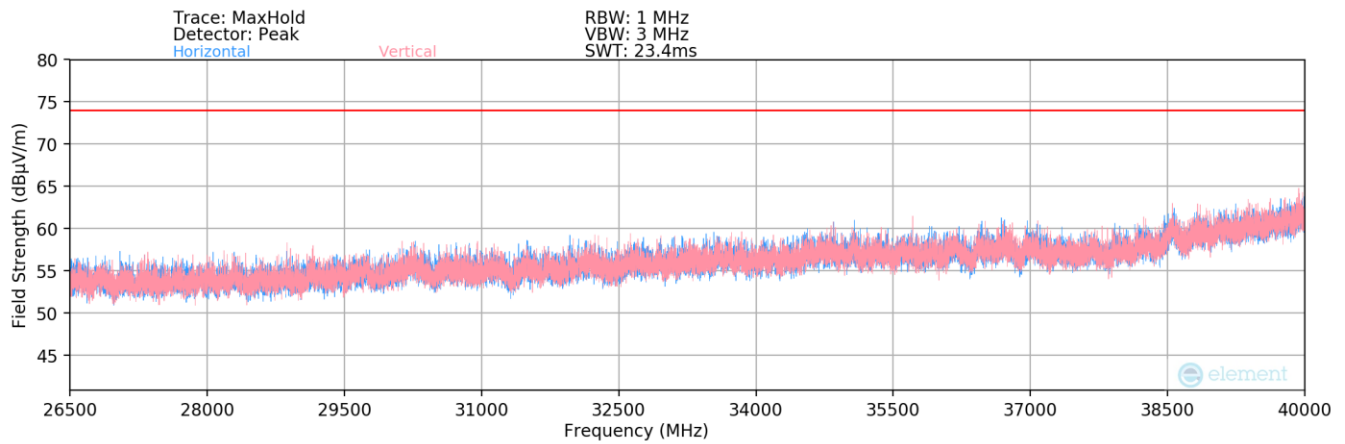
Plot 7-5. Radiated Spurious Plot above 26.5GHz
