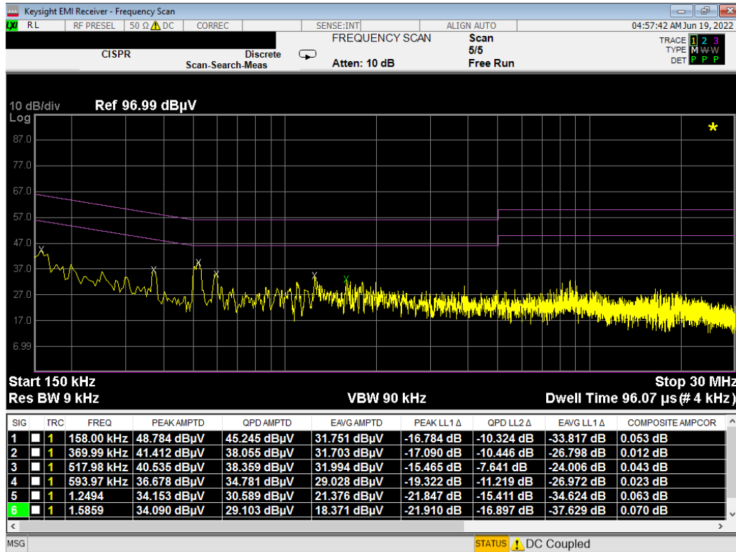
Plot 7-8. Line Conducted Plot (L1) - WCP
