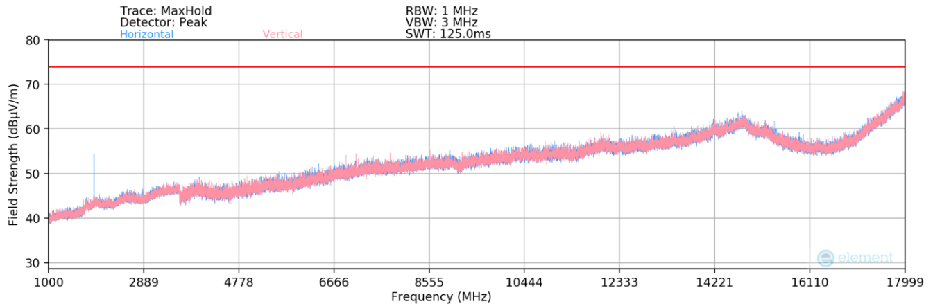
Plot 7-2. Radiated Spurious Plot above 1GHz – Open condition
