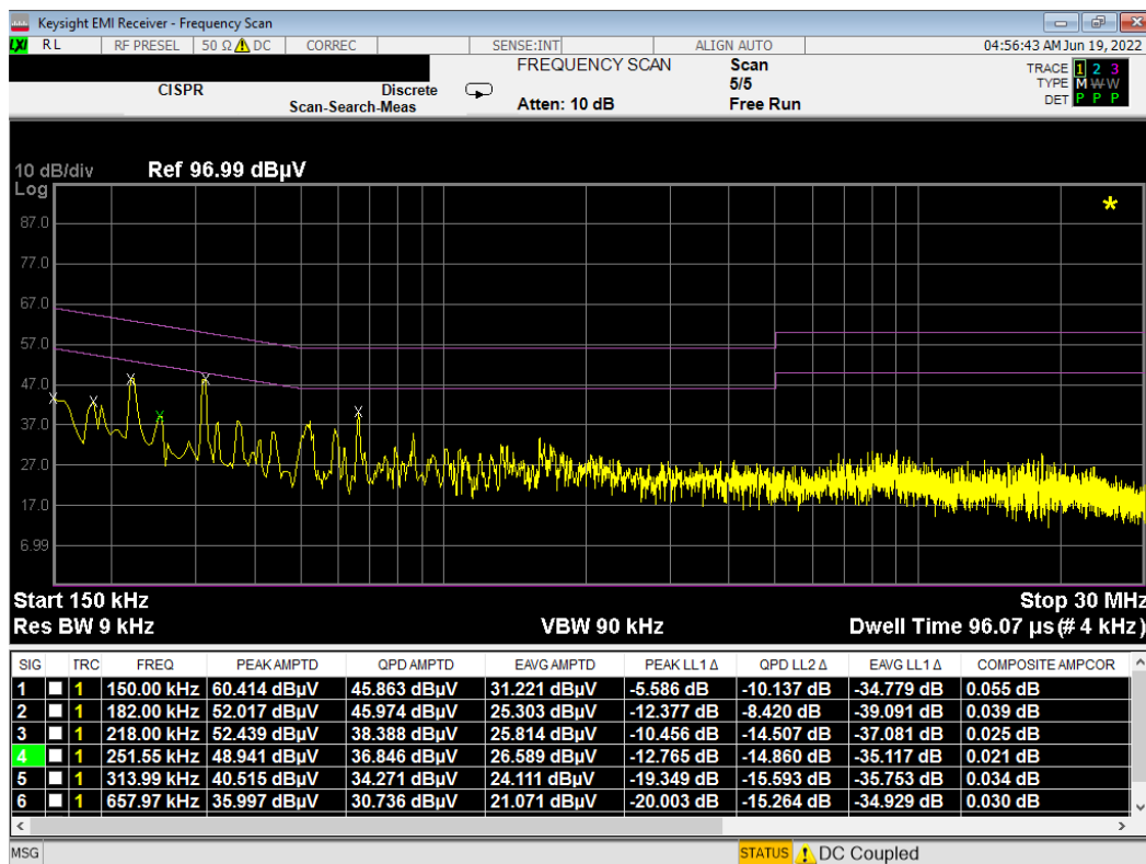
Plot 7-9. Line Conducted Plot (N) - WCP
