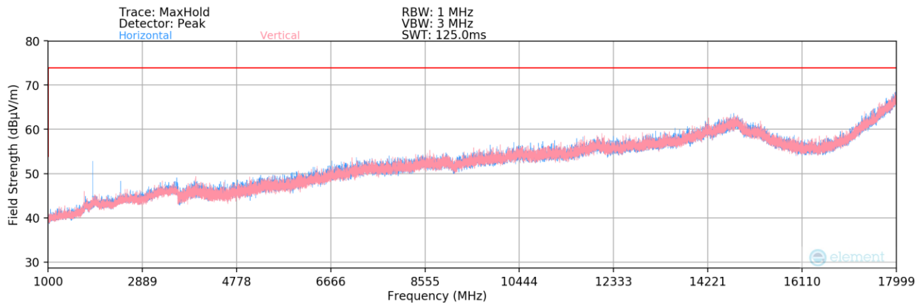
Plot 7-3. Radiated Spurious Plot above 1GHz – Half condition
