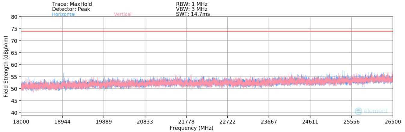
Plot 7-4. Radiated Spurious Plot above 18GHz
