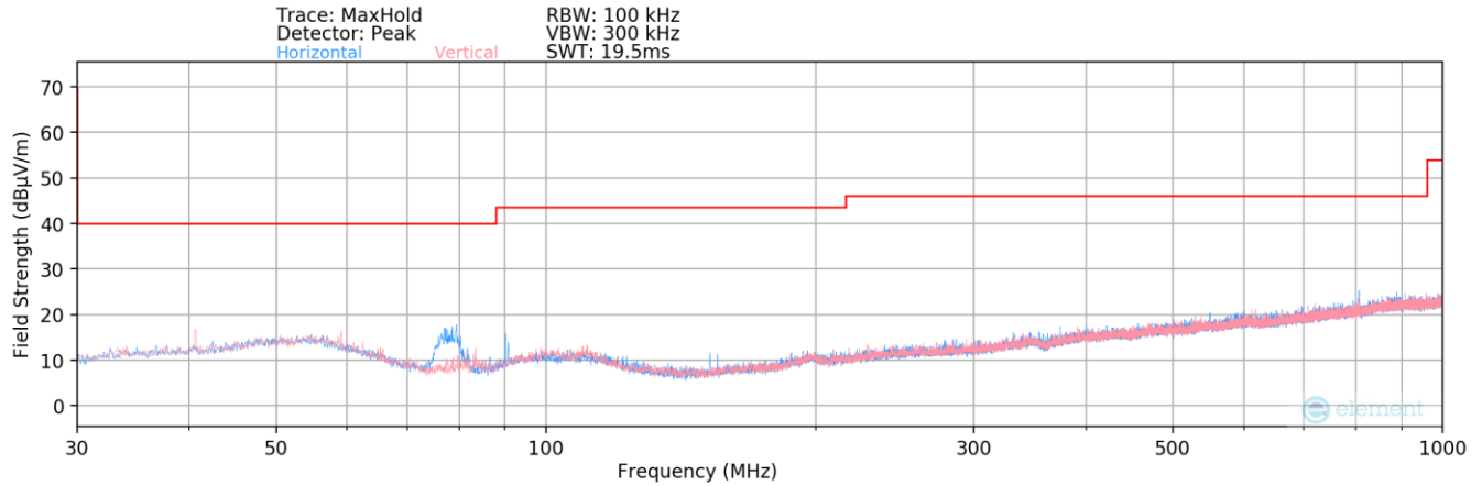
Plot 7-7. Radiated Spurious Plot 30MHz – 1GHz _OPEN
