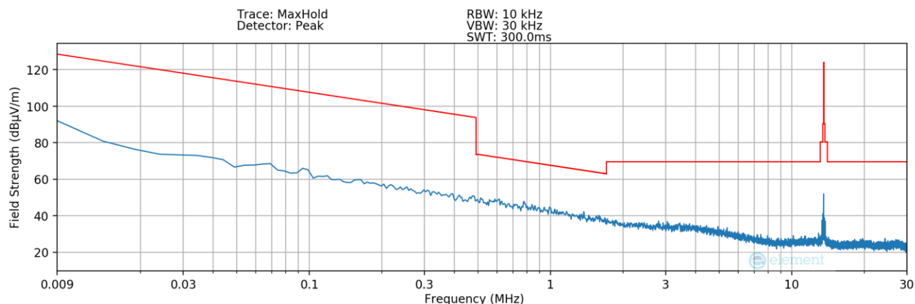
Plot 7-2. Radiated Spurious Plot 9kHz – 30MHz (Pol. Y) _OPEN
