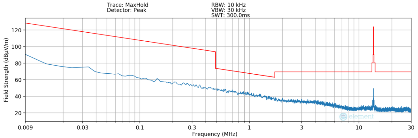
Plot 7-5. Radiated Spurious Plot 9kHz – 30MHz (Pol. Y) _CLOSED
