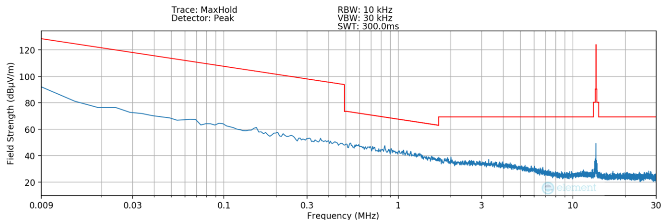
Plot 7-3. Radiated Spurious Plot 9kHz – 30MHz (Pol. Z) _OPEN
