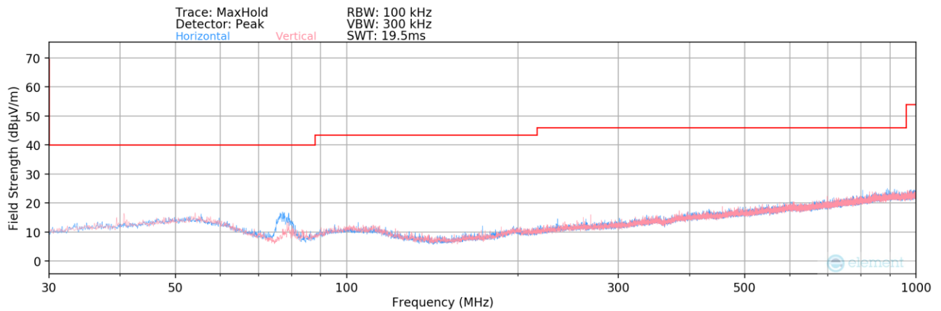
Plot 7-8. Radiated Spurious Plot 30MHz – 1GHz _CLOSED
