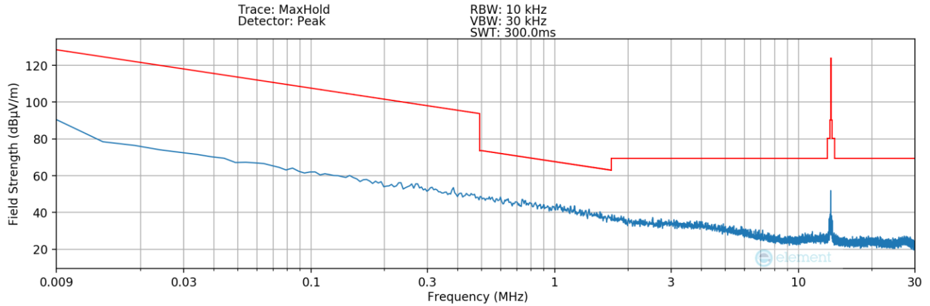
Plot 7-4. Radiated Spurious Plot 9kHz – 30MHz (Pol. X) _CLOSED
