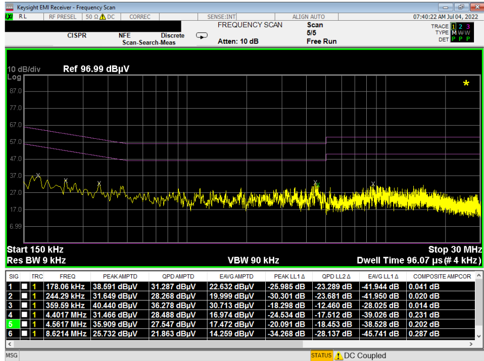
Plot 7-18. Line-Conducted Test Plot (N) – Digitizer (Click)
