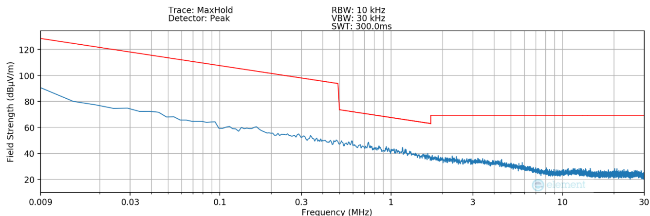
Plot 7-9. Radiated Spurious Plot 9kHz – 30MHz (Pol. Z– Digitizer – Hover)
