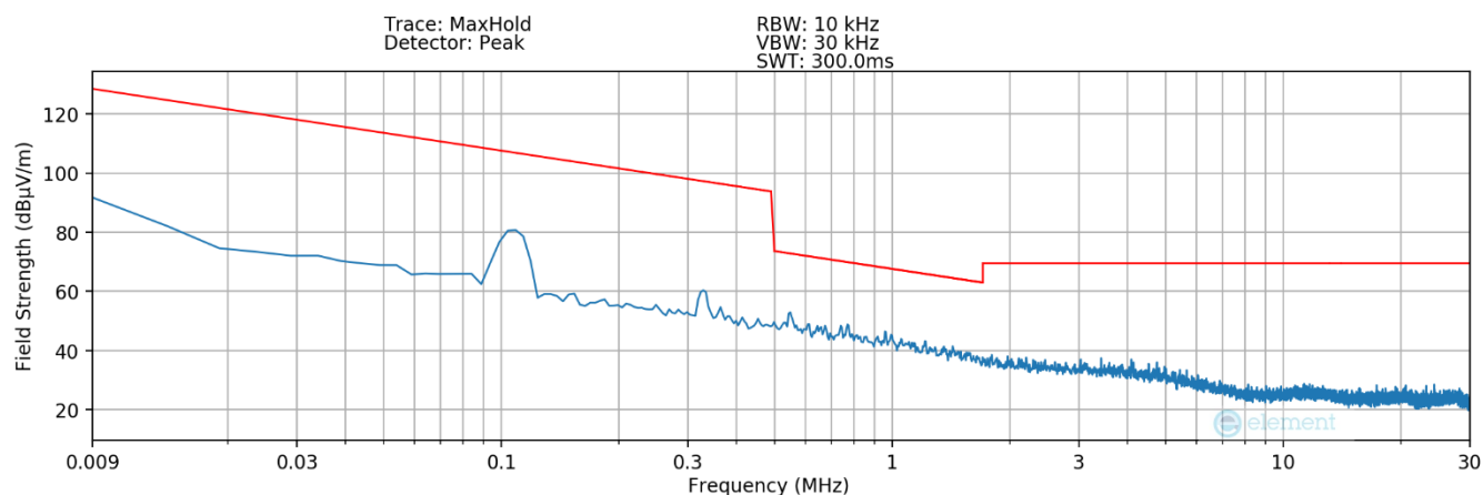
Plot 7-5Radiated Spurious Plot 9kHz – 30MHz (Pol. Y – Device to Device WPT)
