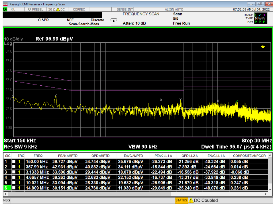
Plot 7-15. Line-Conducted Test Plot (L1) – Digitizer (Hover)
