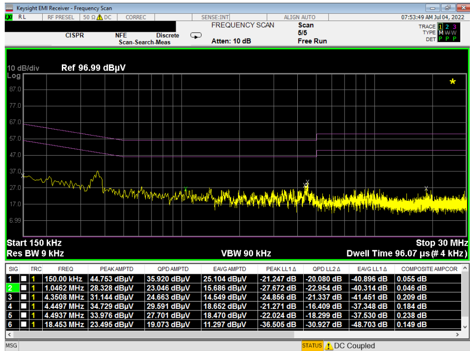
Plot 7-16. Line-Conducted Test Plot (N) – Digitizer (Hover)
