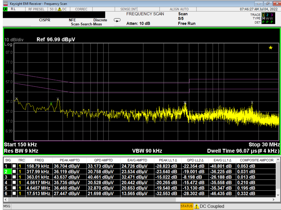
Plot 7-17. Line-Conducted Test Plot (L1) – Digitizer (Click)
