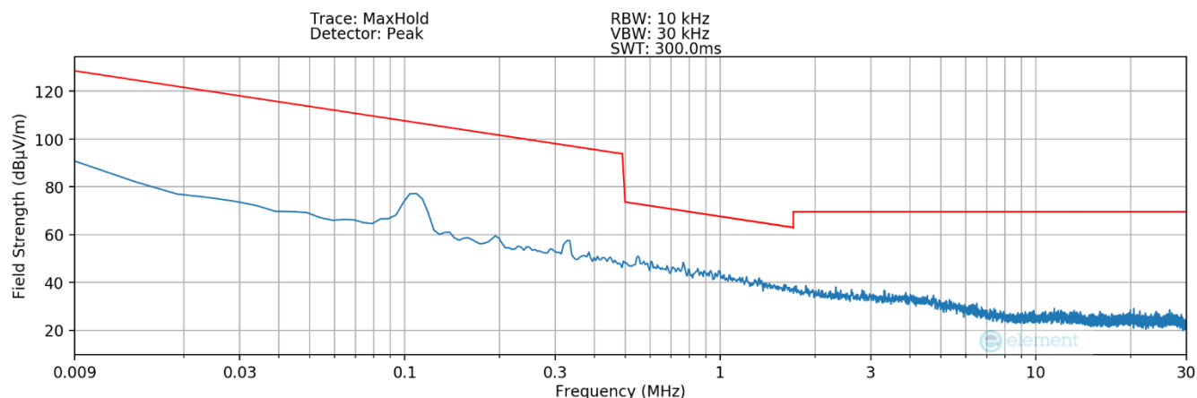
Plot 7-6. Radiated Spurious Plot 9kHz – 30MHz (Pol. Z – Device to Device WPT)
