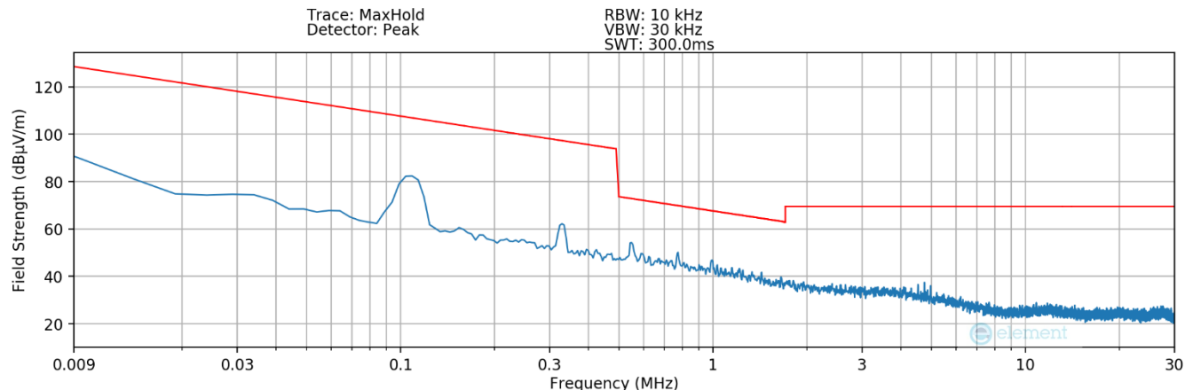
Plot 7-4. Radiated Spurious Plot 9kHz – 30MHz (Pol. X – Device to Device WPT)
