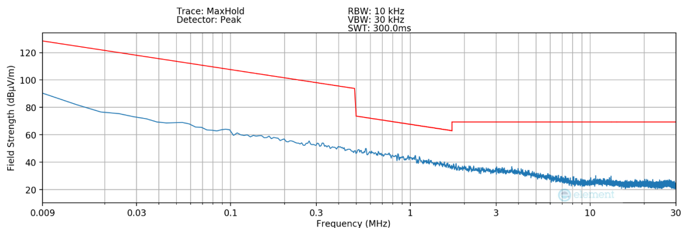
Plot 7-8 Radiated Spurious Plot 9kHz – 30MHz (Pol. Y – Digitizer – Hover)
