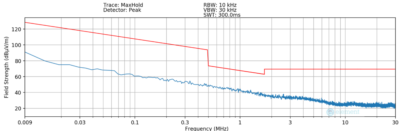
Plot 7-7. Radiated Spurious Plot 9kHz – 30MHz (Pol. X – Digitizer – Hover)
