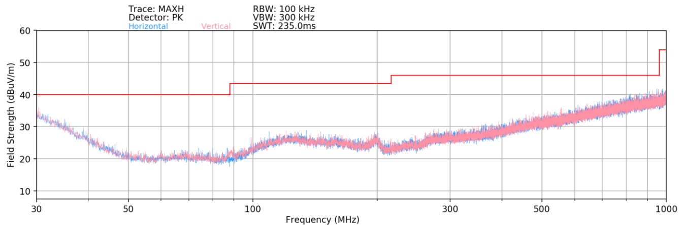
Plot 7-2. Radiated Spurious Plot below 1GHz – Closed
