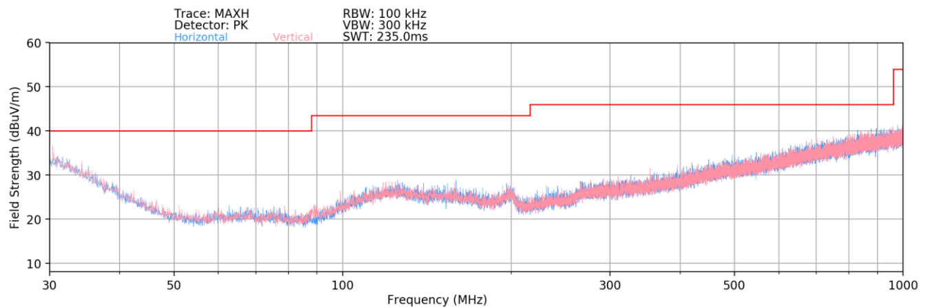
Plot 7-3. Radiated Spurious Plot below 1GHz - Half
