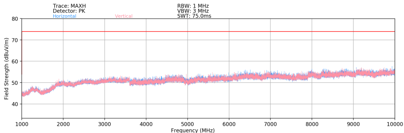
Plot 7-5. Radiated Spurious Plot above 1GHz – Closed
