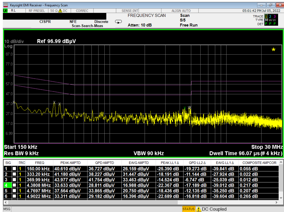
Plot 7-8. Line Conducted Plot (N)
