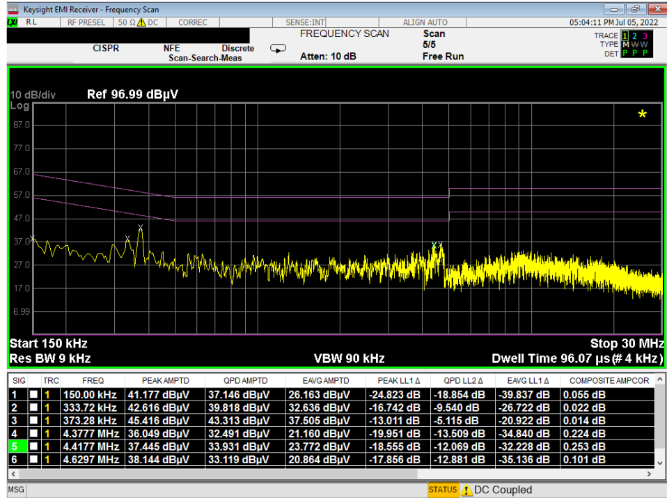
Plot 7-7. Line Conducted Plot (L1)
