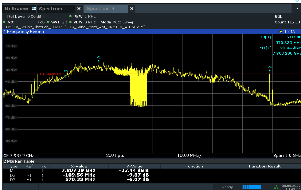
Plot 7-28. 10dBc Bandwidth – CH.9 - SP0 – Preamble 27
