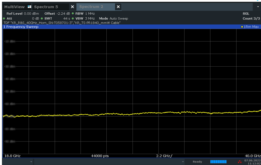
Plot 7-63. Radiated Spurious Pre-Scan 18 – 40 GHz - CH.5 - ANT 1
