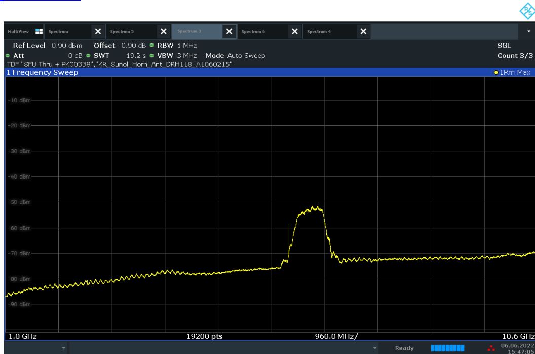
Plot 7-59. Radiated Spurious Pre-Scan 1000 - 10600 MHz - CH.5 - ANT 1
