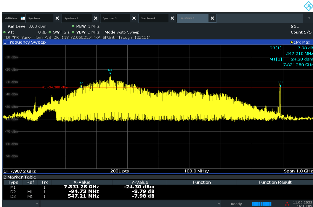
Plot 7-32. 10dBc Bandwidth – CH.9 – SP1 – Preamble 9
