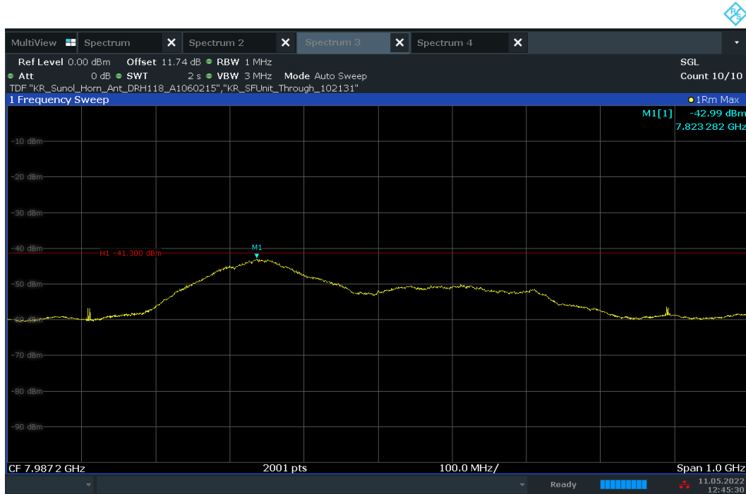
Plot 7-52. UWB Average Power Measurement - ANT 2 - CH.9 – BPRF
