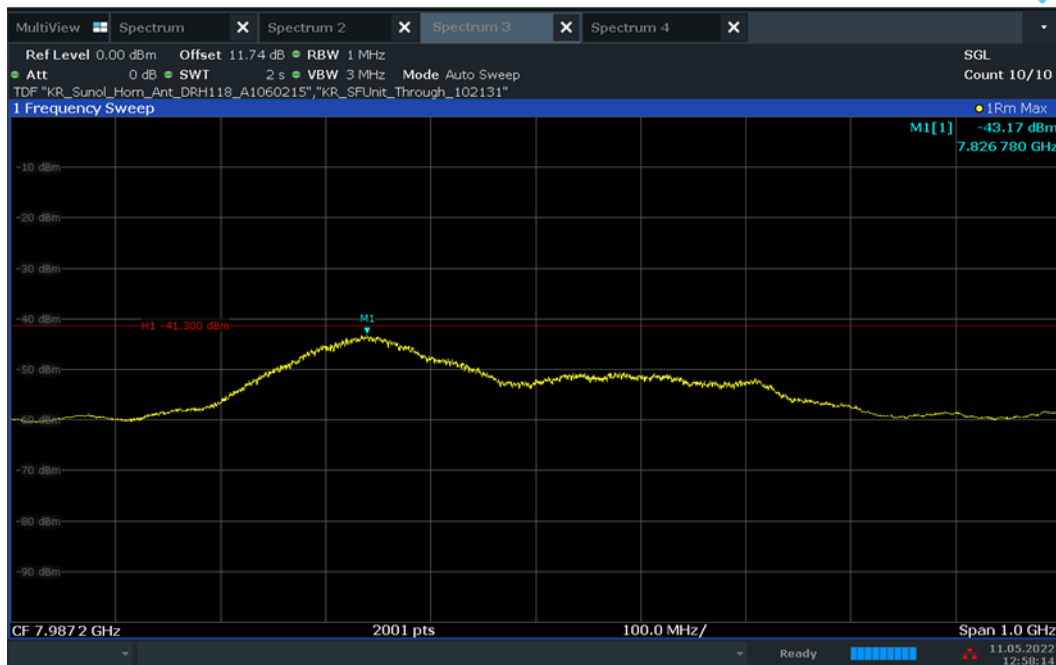
Plot 7-58. UWB Average Power Measurement - ANT 2 - CH.9 – HPRF
