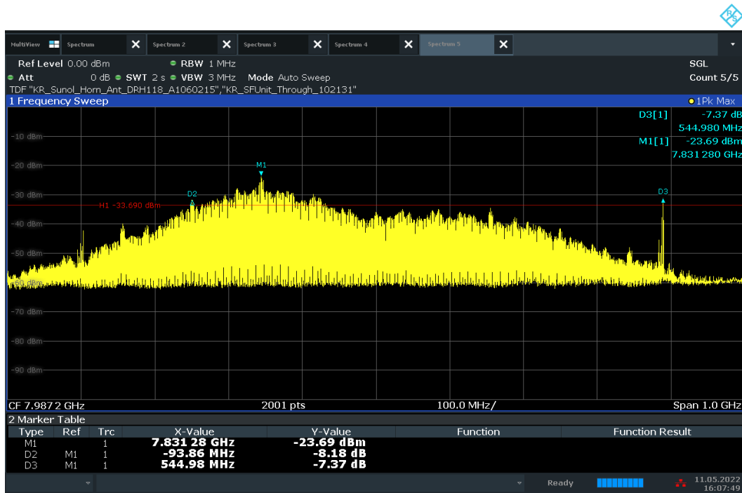
Plot 7-31. 10dBc Bandwidth – CH.9 - SP0 – Preamble 9
