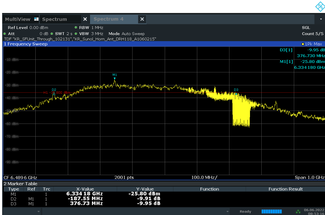
Plot 7-2. 10dBc Bandwidth – CH.5 – SP1 – Preamble 9
