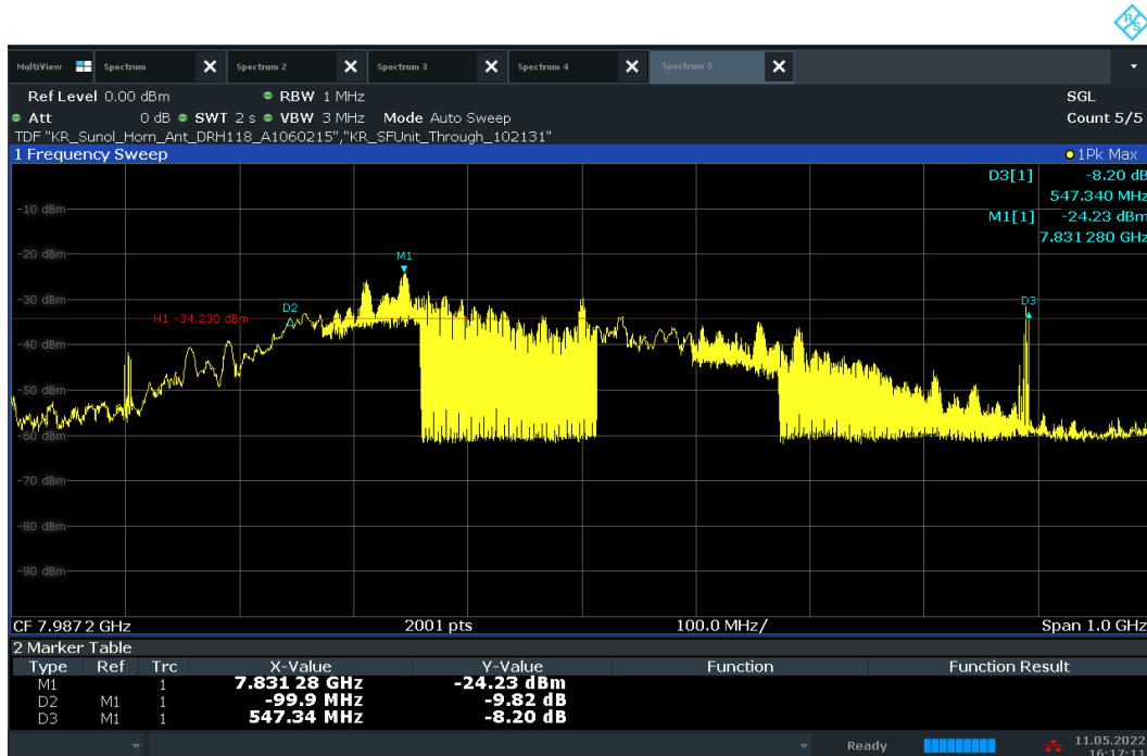
Plot 7-34. 10dBc Bandwidth – CH.9 - SP0 – Preamble 10
