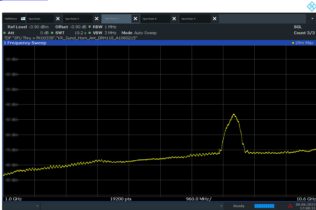
Plot 7-69. Radiated Spurious Pre-Scan 1000 - 10600 MHz - CH.9 - ANT 2
