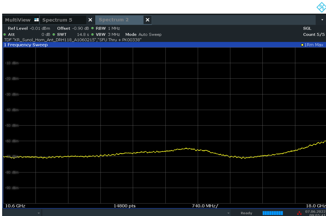
Plot 7-65. Radiated Spurious Pre-Scan 10600 - 18000 MHz - CH.9 - ANT 1
