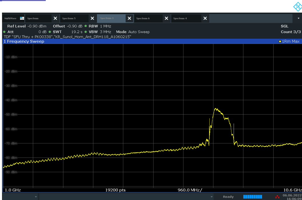
Plot 7-64. Radiated Spurious Pre-Scan 1000 - 10600 MHz - CH.9 - ANT 1
