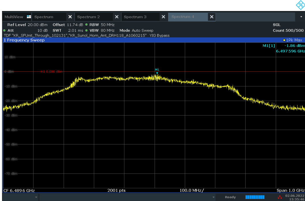
Plot 7-47. UWB Peak Power Measurement - ANT 1 - CH.5 – BPRF
