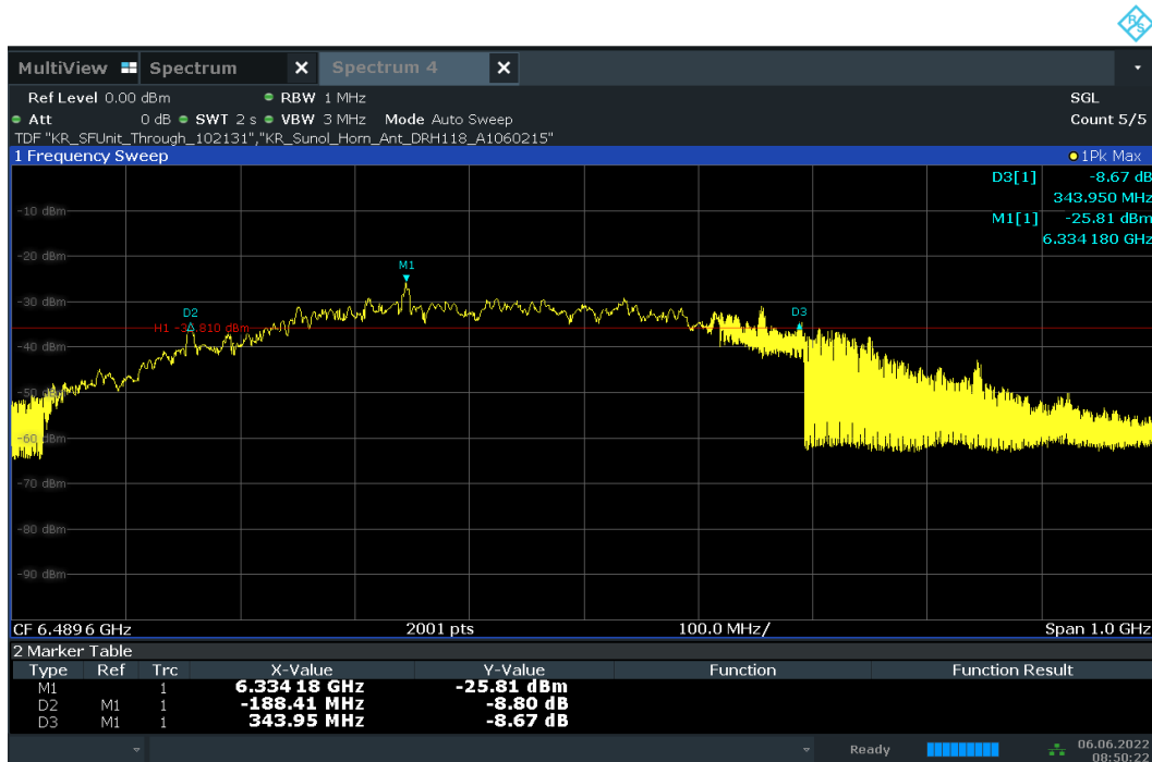
Plot 7-1. 10dBc Bandwidth – CH.5 - SP0 – Preamble 9
