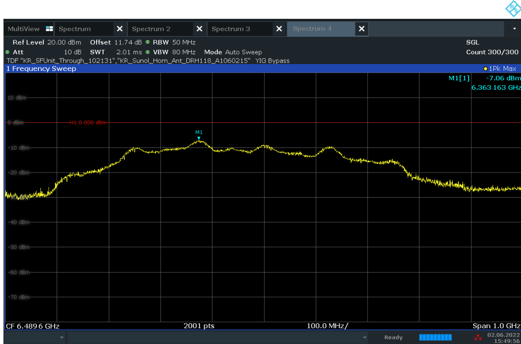
Plot 7-53. UWB Peak Power Measurement - ANT 1 - CH.5 – HPRF
