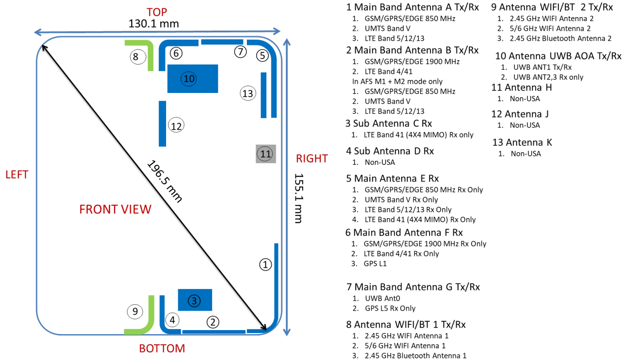
Figure F-2 DUT Antenna Locations – Open
