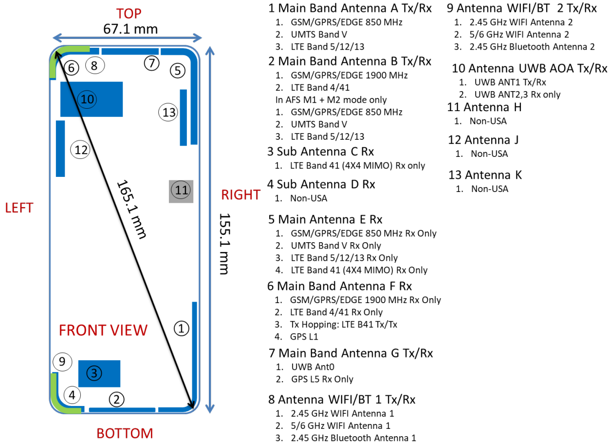
Figure F-1 DUT Antenna Locations – Closed
