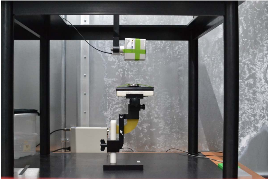
Test Setup Photo 27 E-field, Back side, 15cm
