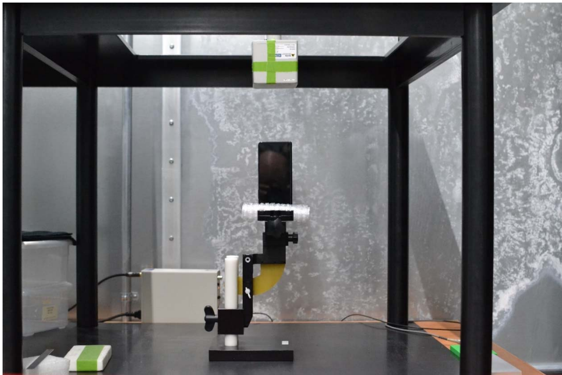
Test Setup Photo 22 H-field, Bottom edge, 15cm
