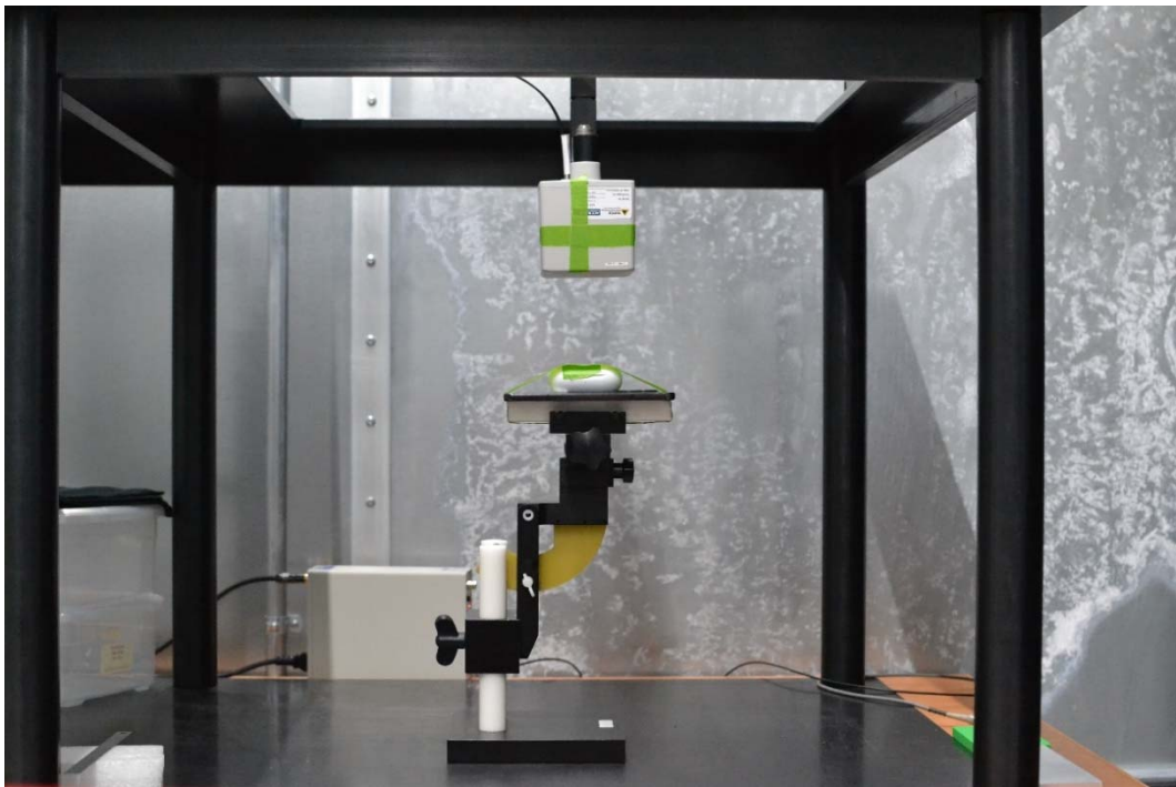
Test Setup Photo 30 H-field, Back side, 15cm
