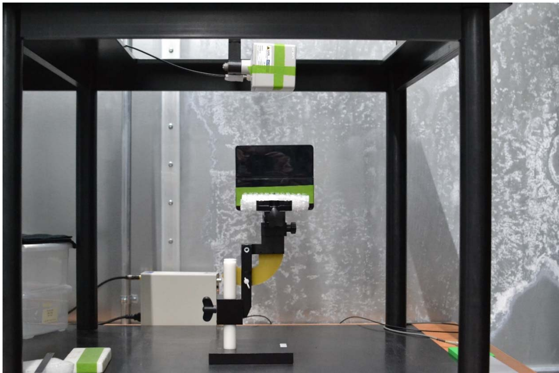
Test Setup Photo 6 E-field, Left edge, 15cm
