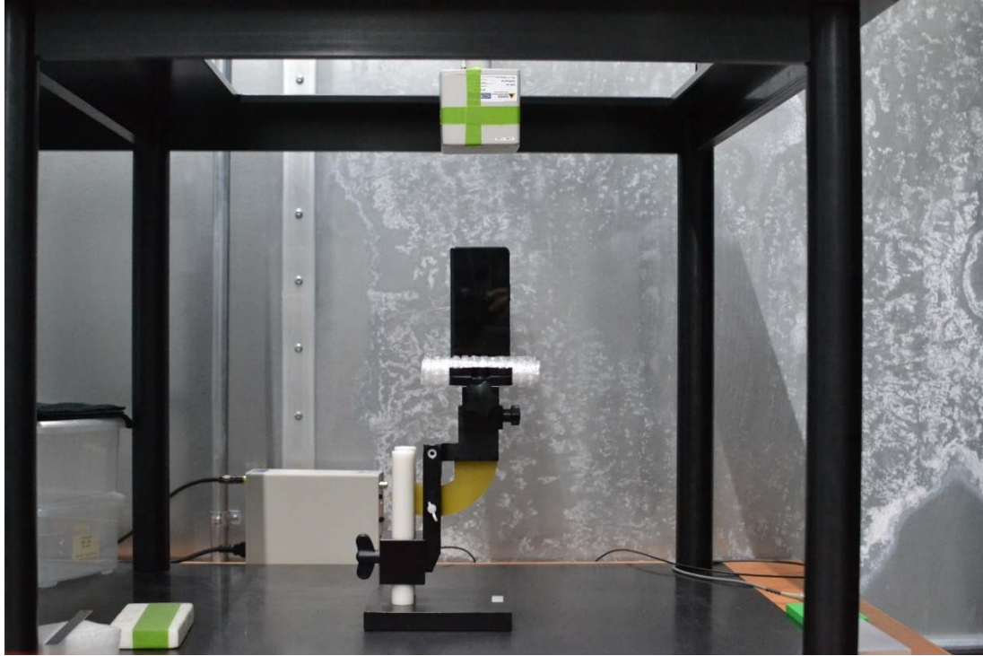
Test Setup Photo 21 H-field, Top edge, 15cm
