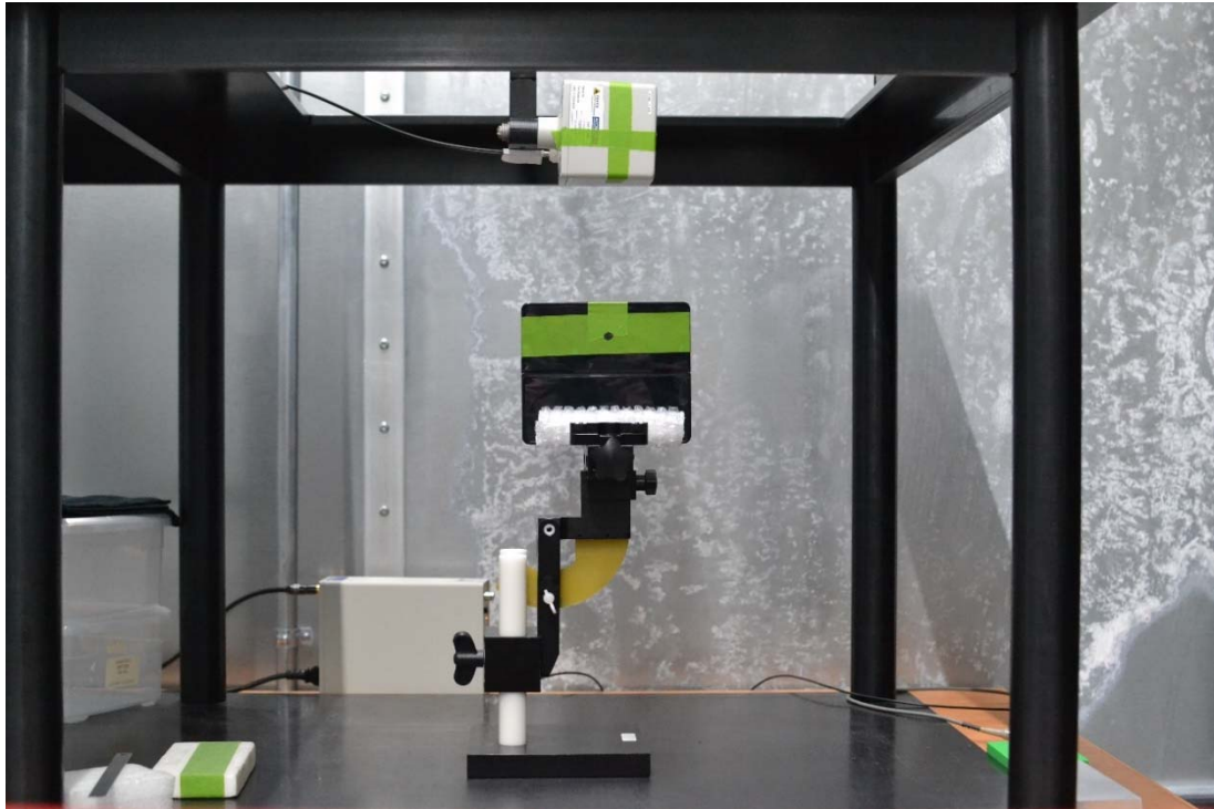
Test Setup Photo 5 E-field, Right edge, 15cm
