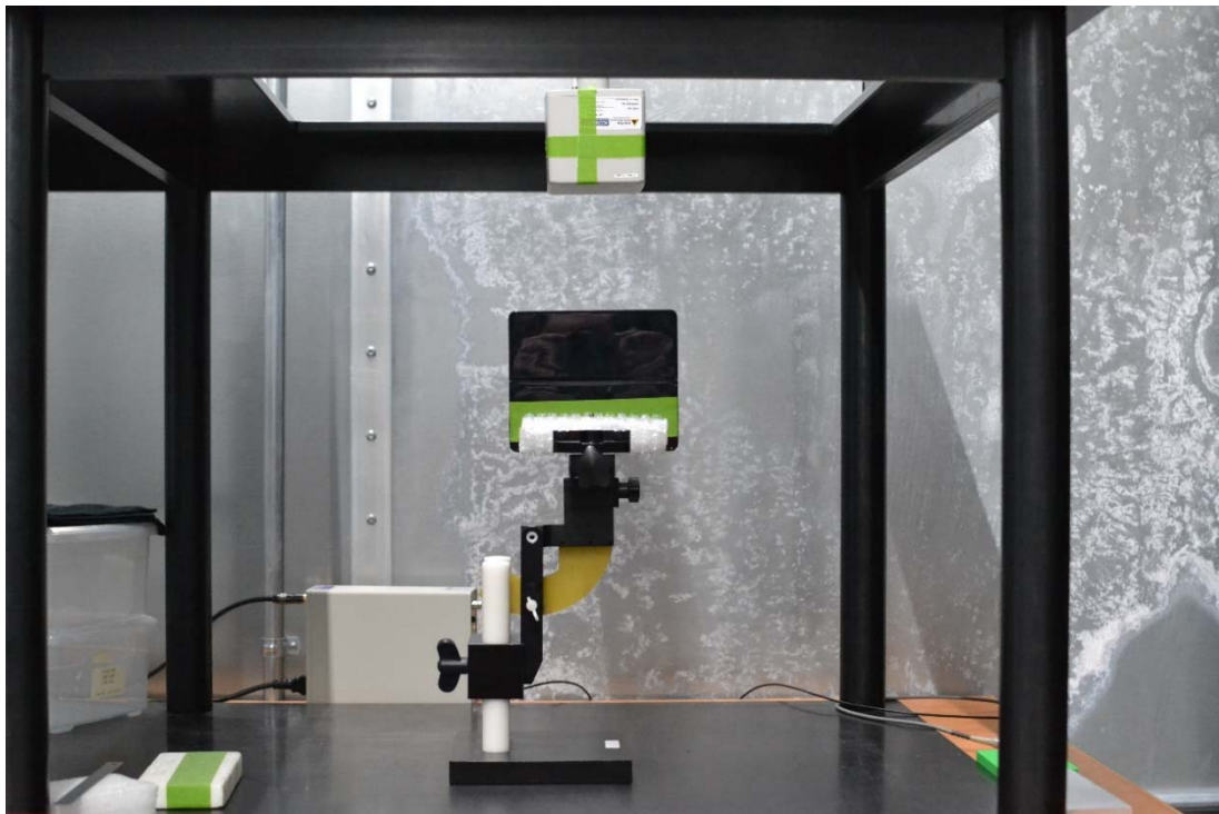
Test Setup Photo 12 H-field, Left edge, 15cm
