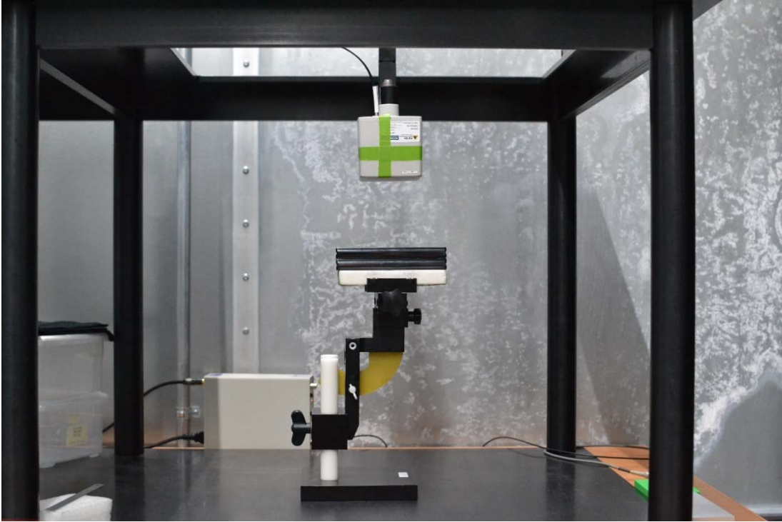
Test Setup Photo 19 H-field, Back side, 15cm
