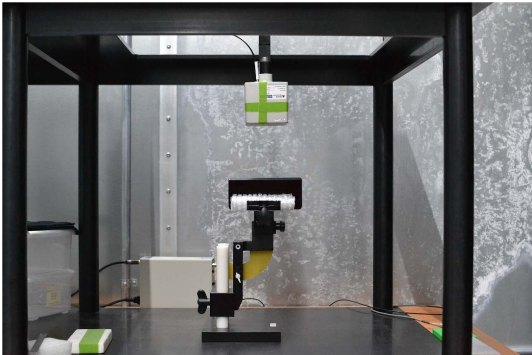
Test Setup Photo 24 H-field, Left edge, 15cm
