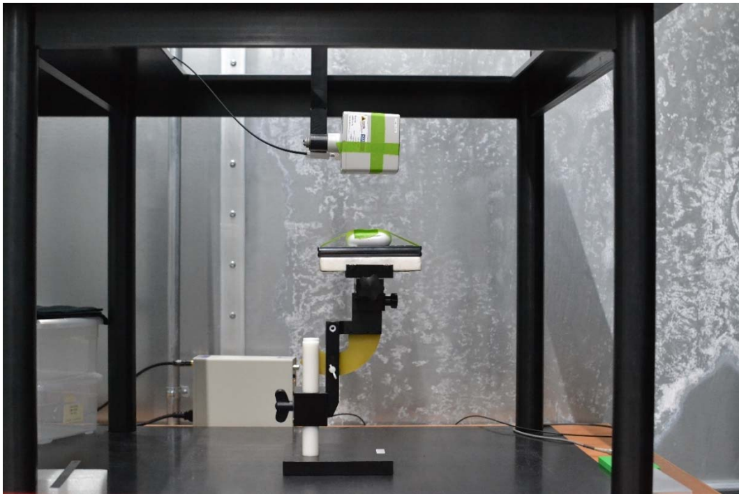
Test Setup Photo 31 E-field, Back side, 15cm
