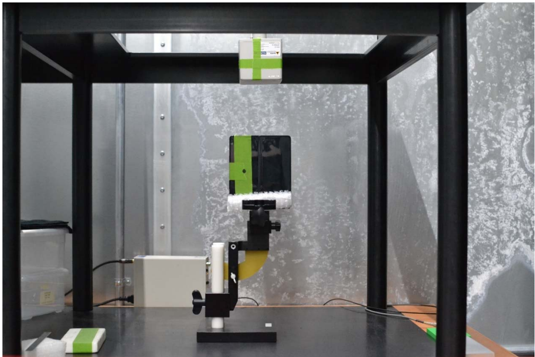
Test Setup Photo 10 H-field, Bottom edge, 15cm
