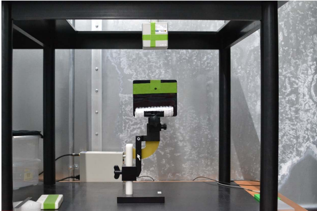
Test Setup Photo 11 H-field, Right edge, 15cm
