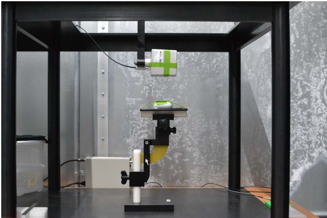
Test Setup Photo 29 E-field, Back side, 15cm
