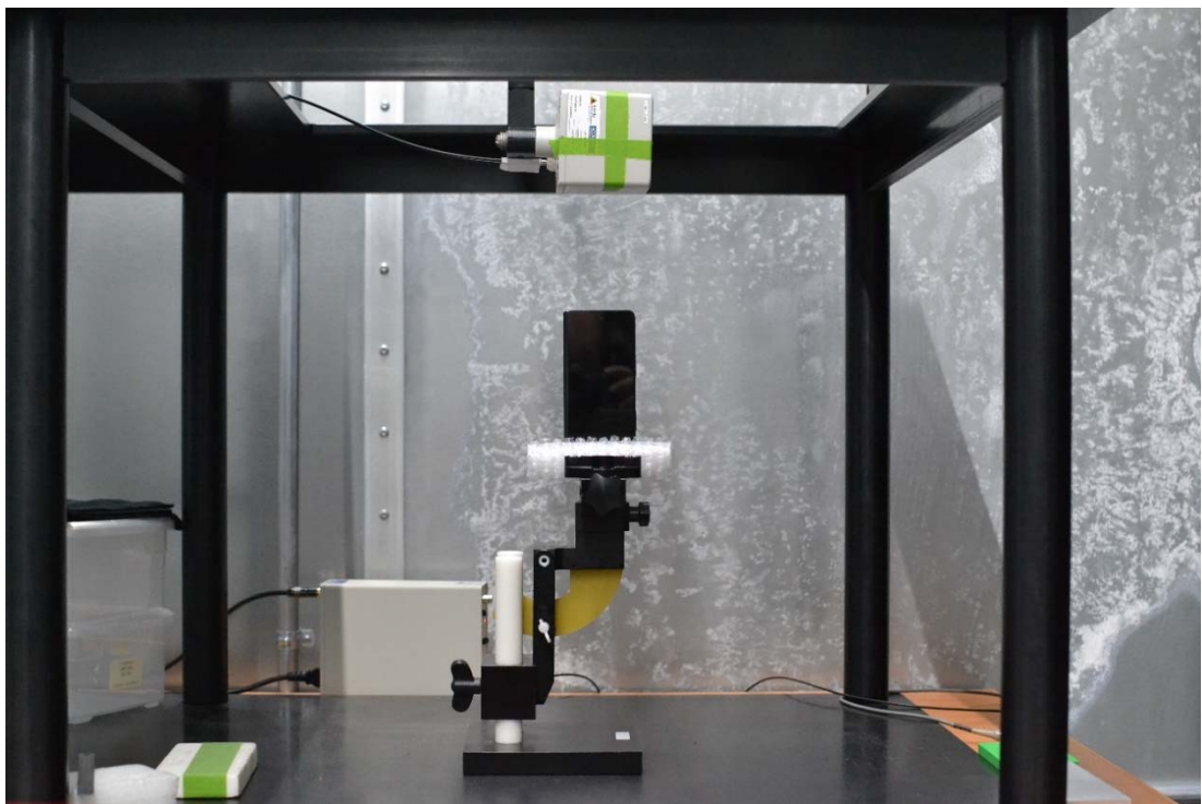
Test Setup Photo 15 E-field, Top edge, 15cm
