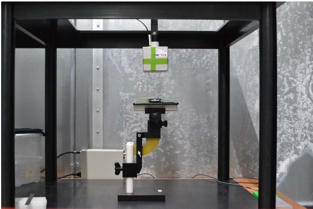
Test Setup Photo 26 H-field, Back side, 15cm
