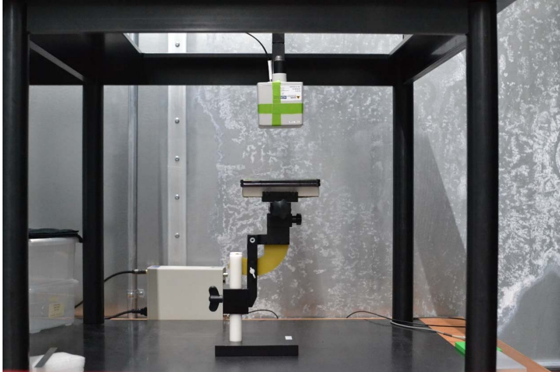
Test Setup Photo 7 H-field, Back side, 15cm
