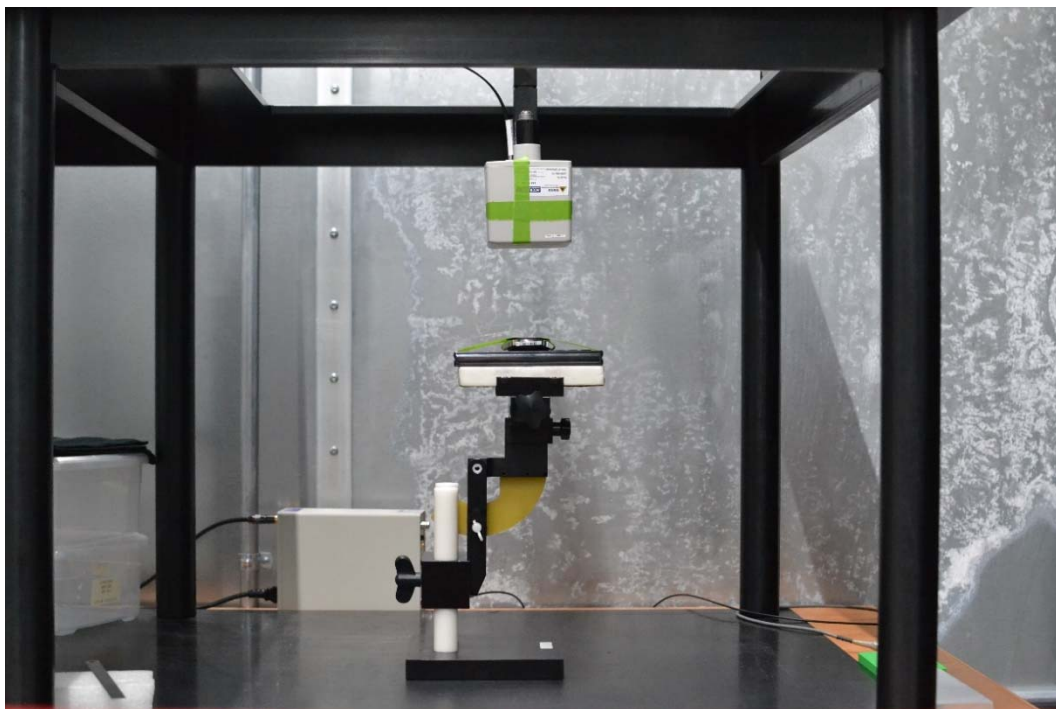
Test Setup Photo 28 H-field, Back side, 15cm
