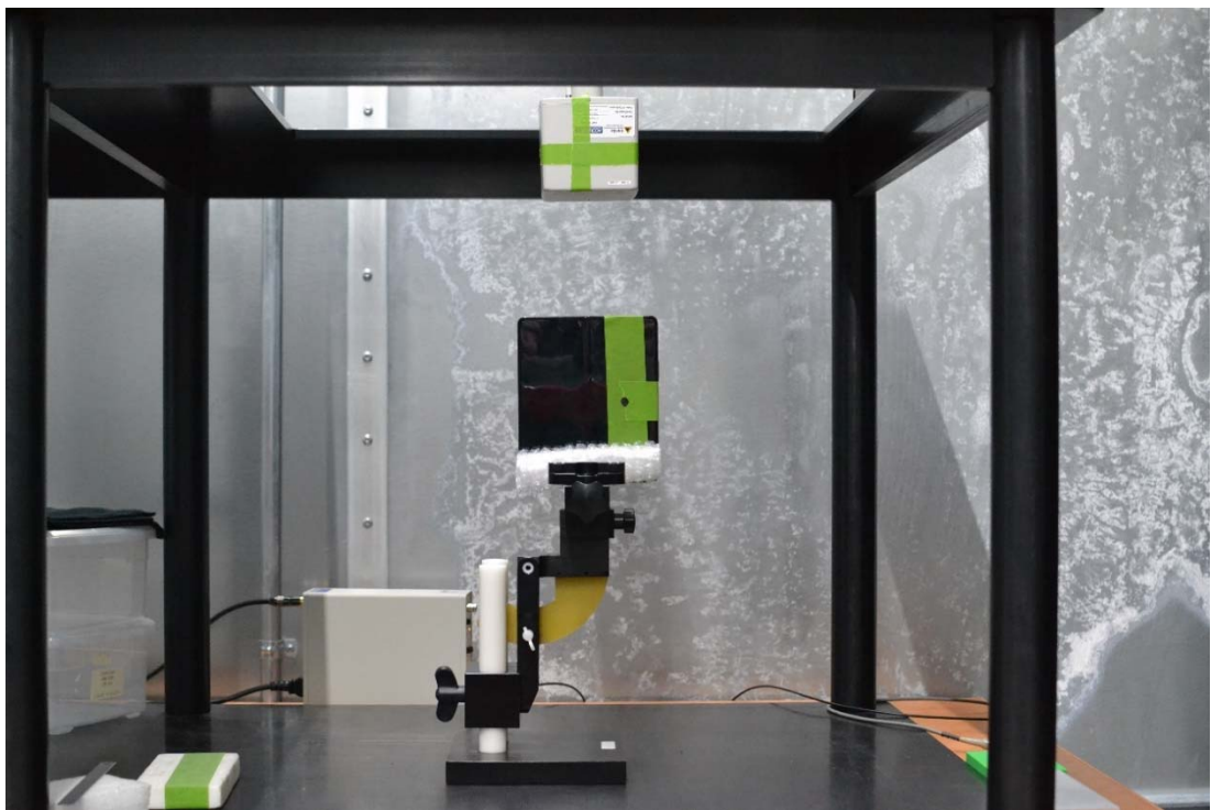
Test Setup Photo 9 H-field, Top edge, 15cm
