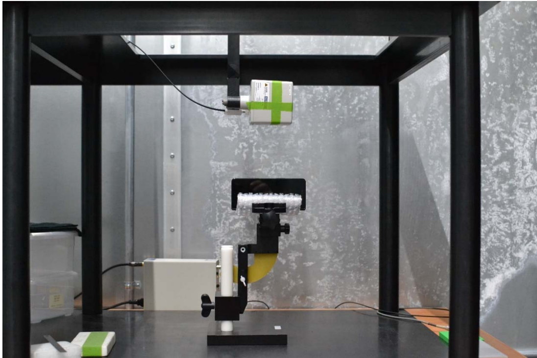
Test Setup Photo 17 E-field, Right edge, 15cm
