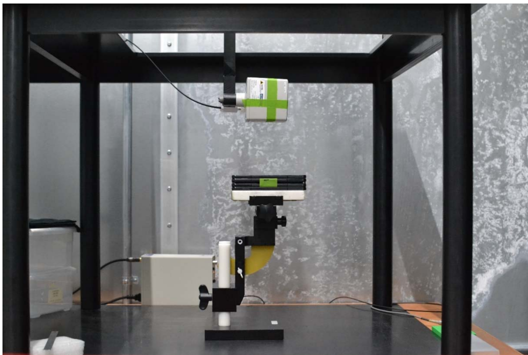
Test Setup Photo 14 E-field, Front side, 15cm
