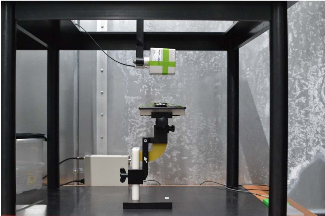
Test Setup Photo 25 E-field, Back side, 15cm
