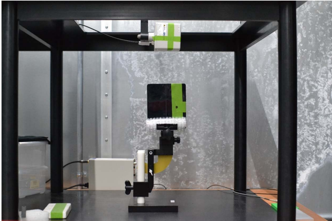
Test Setup Photo 3 E-field, Top edge, 15cm
