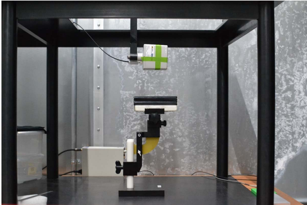
Test Setup Photo 13 E-field, Back side, 15cm
