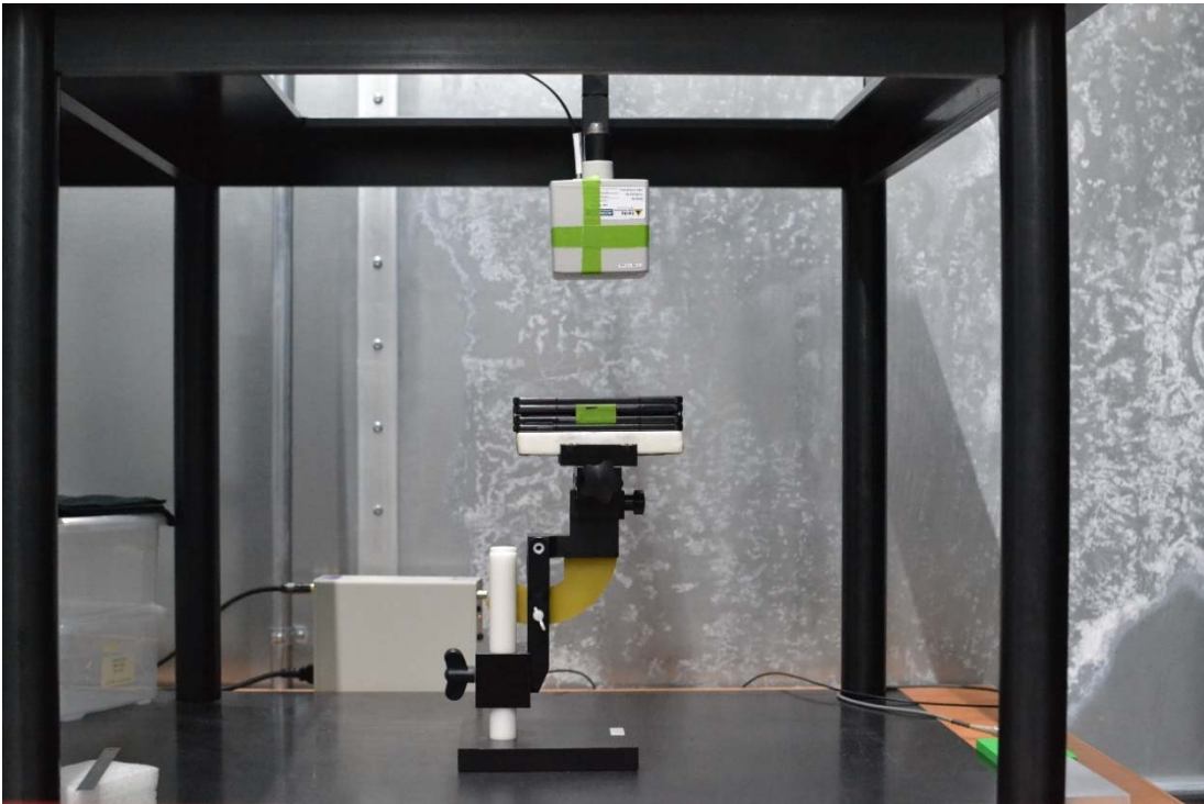
Test Setup Photo 20 H-field, Front side, 15cm
