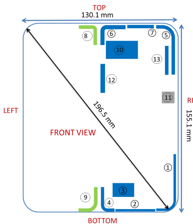
Figure E-3 DUT Antenna Locations – Open Configuration (UMPC)
