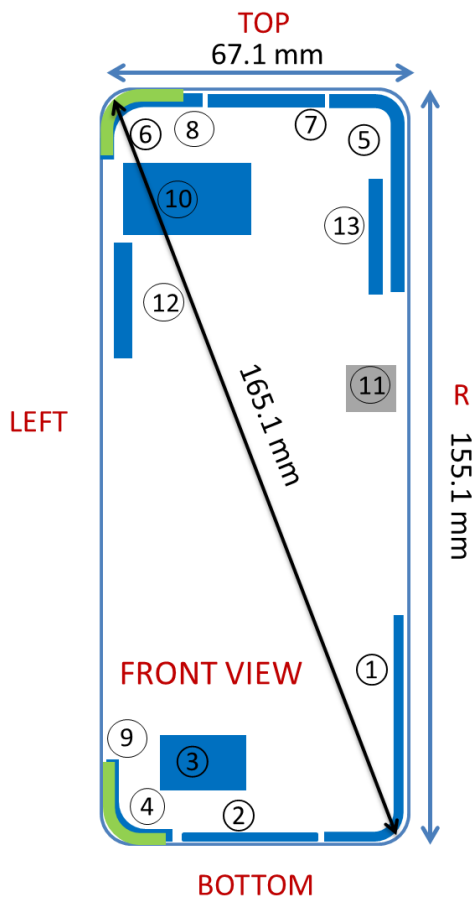
Figure E-1 DUT Antenna Locations – Closed Configuration (Handset)
