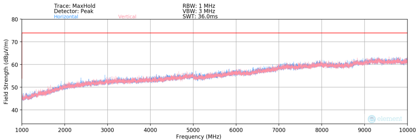
Plot 7-5. Radiated Spurious Plot above 1GHz – Closed
