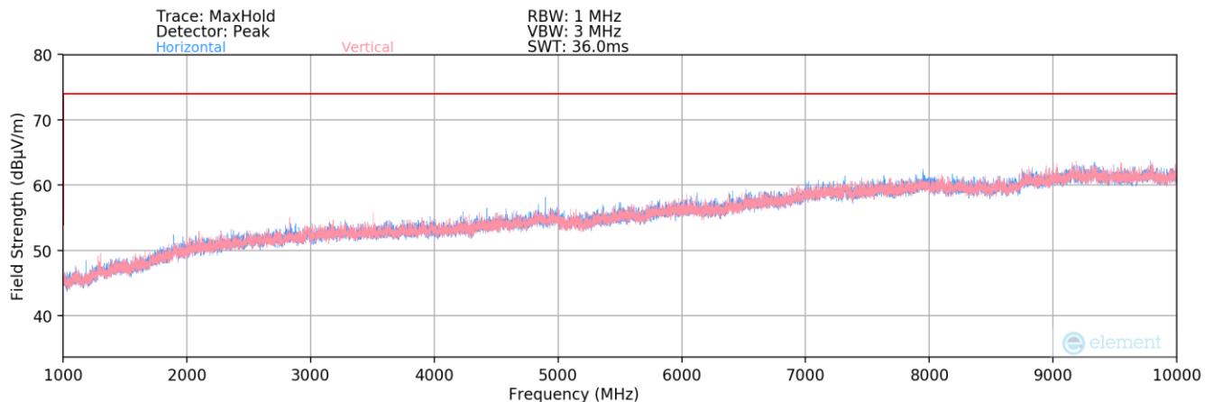
Plot 7-6. Radiated Spurious Plot above 1GHz – Half
