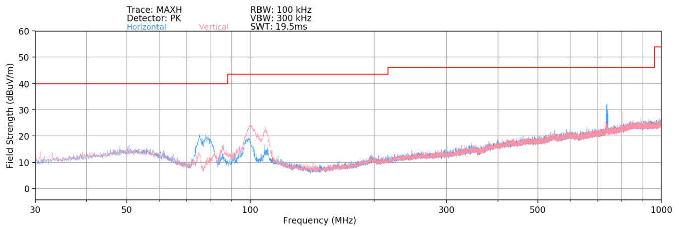
Plot 7-2. Radiated Spurious Plot below 1GHz – Closed
