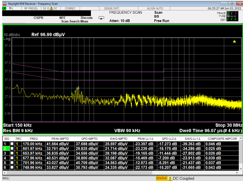
Plot 7-9. Line Conducted Plot (L1) - Closed
