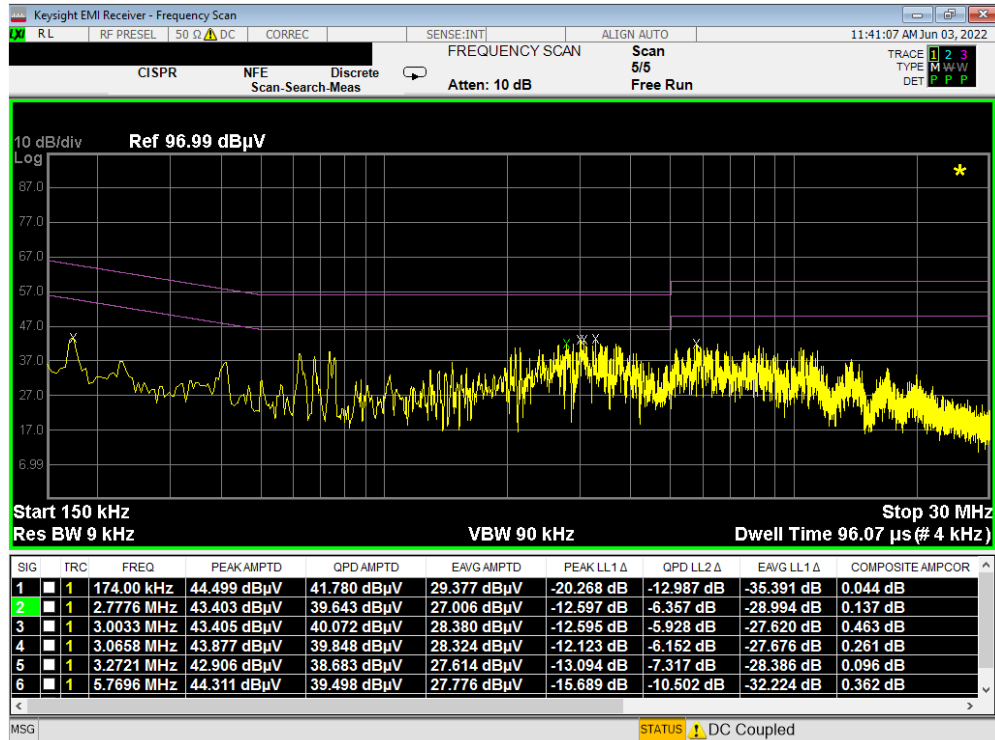
Plot 7-7. Line Conducted Plot (L1) - Open
