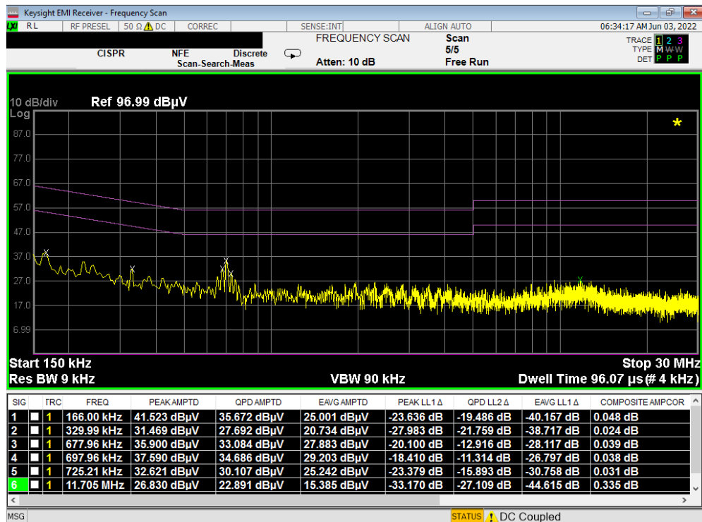
Plot 7-10. Line Conducted Plot (N) - Closed
