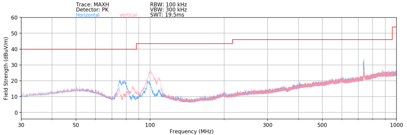
Plot 7-1. Radiated Spurious Plot below 1GHz – Open
