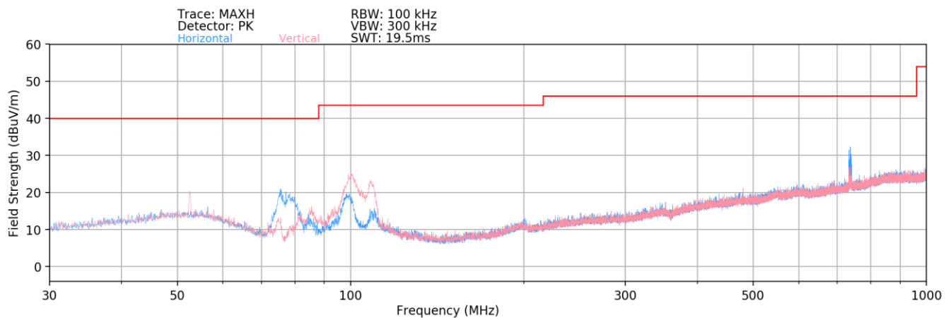
Plot 7-3. Radiated Spurious Plot below 1GHz - Half
