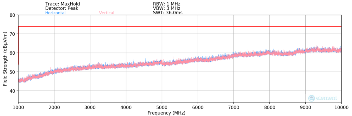
Plot 7-4. Radiated Spurious Plot above 1GHz – Open
