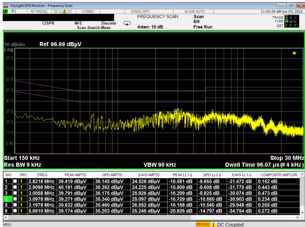
Plot 7-8. Line Conducted Plot (N) - Open
