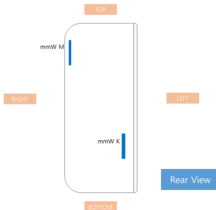
Figure 1: Location of mmW antenna modules looking from back of the DUT - Closed
