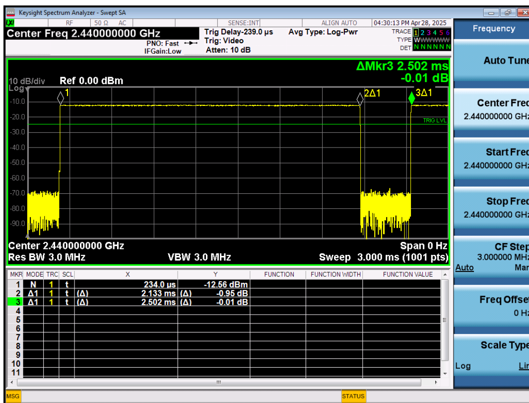
Figure 10-5 Bluetooth LE Antenna F Transmission Plot
