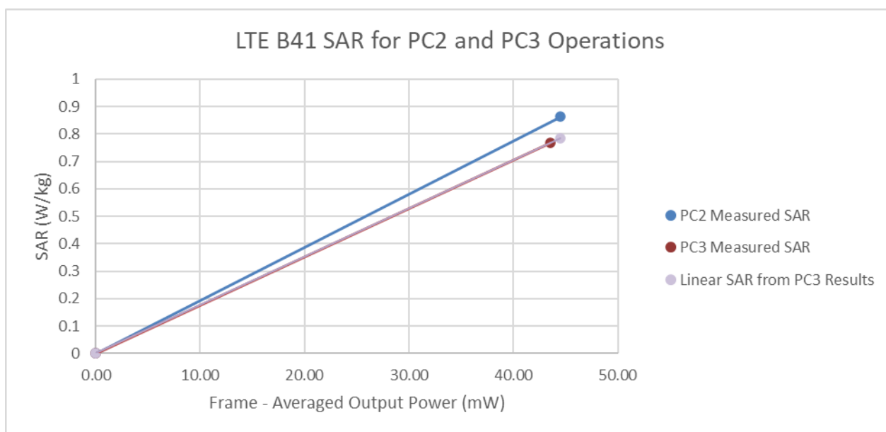
Figure 15-2 LTE Band 41 Antenna G Body-worn/Hotspot Linearity
