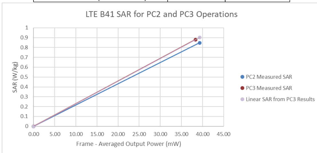
Figure 15-1 LTE Band 41 Antenna G Head Linearity
