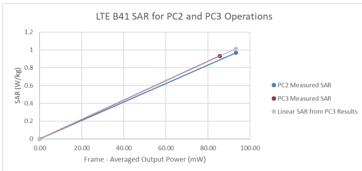
Figure 15-3 LTE Band 41 Antenna G DSI = 0 (F/O Body) Body Linearity
