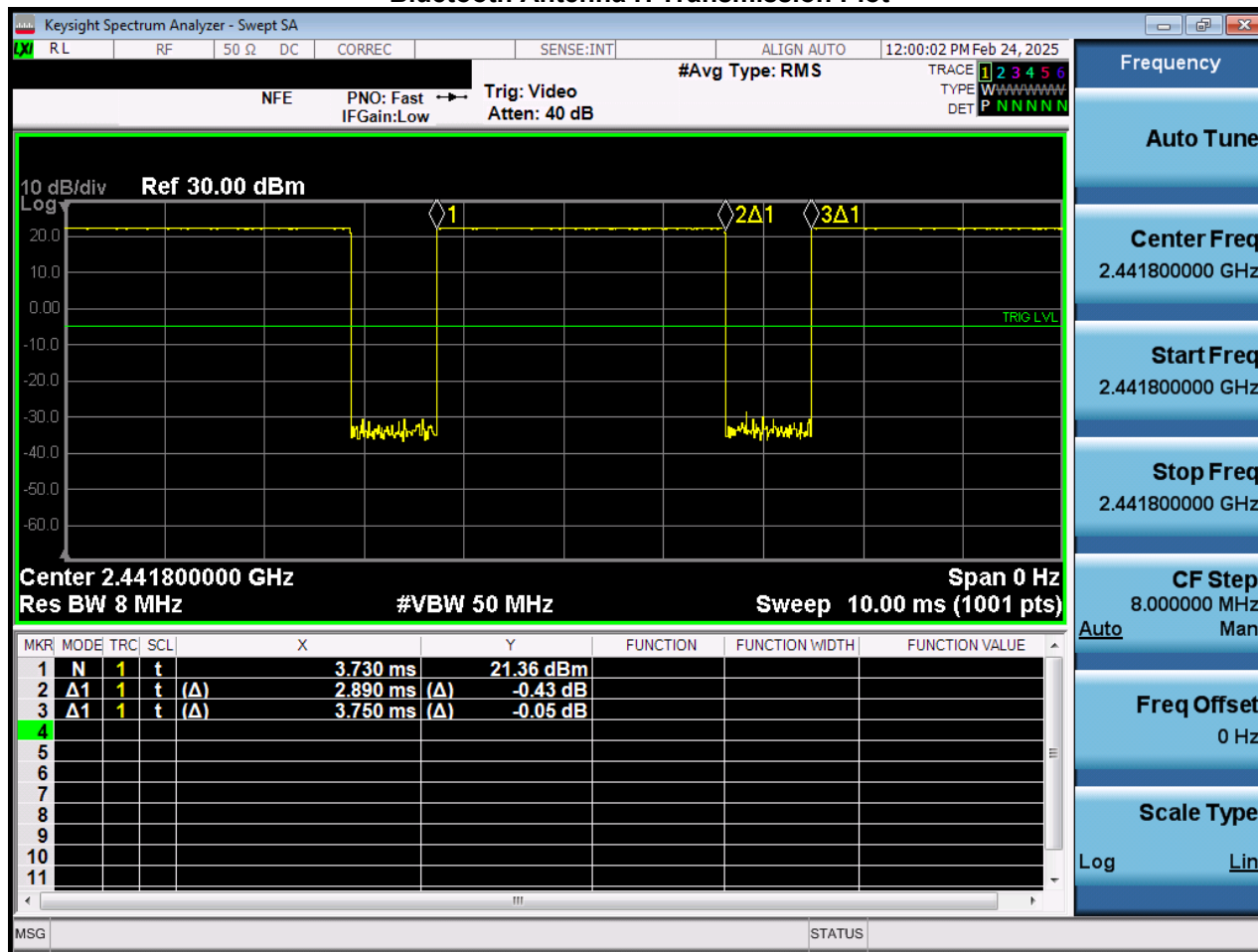
Figure 10-2 Bluetooth Antenna H Transmission Plot
