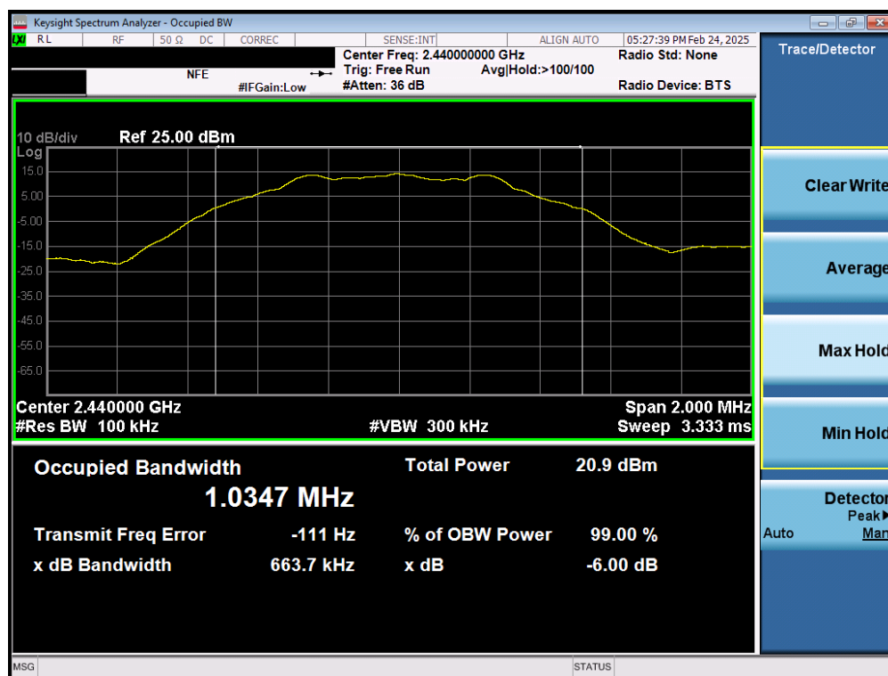
Plot 7-26. 6dB Bandwidth Plot (Bluetooth (LE), 1Mbps – Ch. 17) – Dual Ant 1
