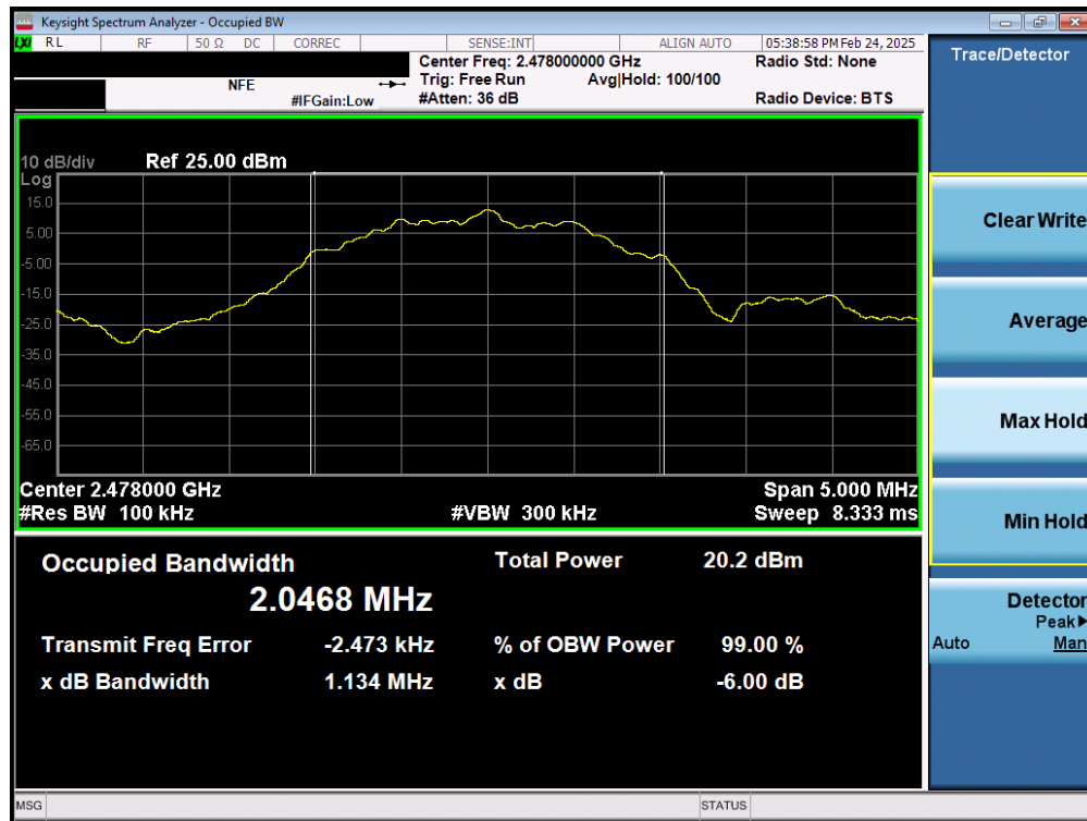
Plot 7-30. 6dB Bandwidth Plot (Bluetooth (LE), 2Mbps – Ch. 36) – Dual Ant 1
