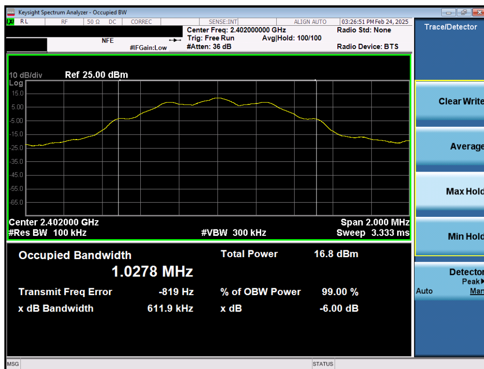
Plot 7-13. 6dB Bandwidth Plot (Bluetooth (LE), 125kbps – Ch. 37) – Ant 2
