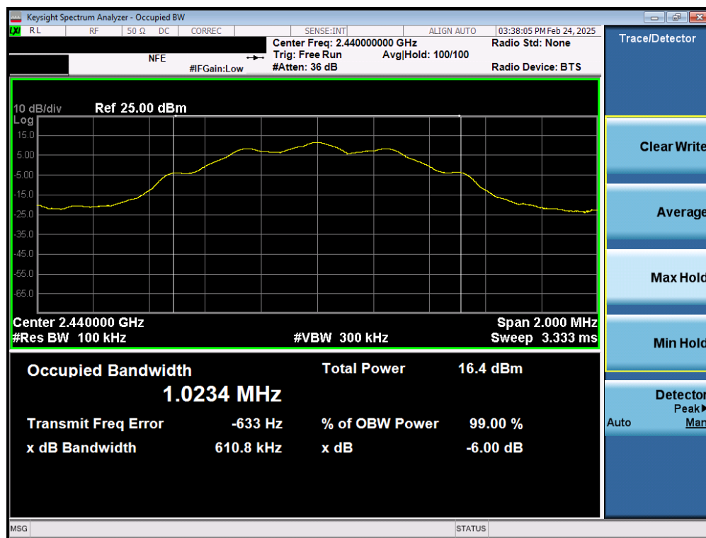
Plot 7-14. 6dB Bandwidth Plot (Bluetooth (LE), 125kbps – Ch. 17) – Ant 2
