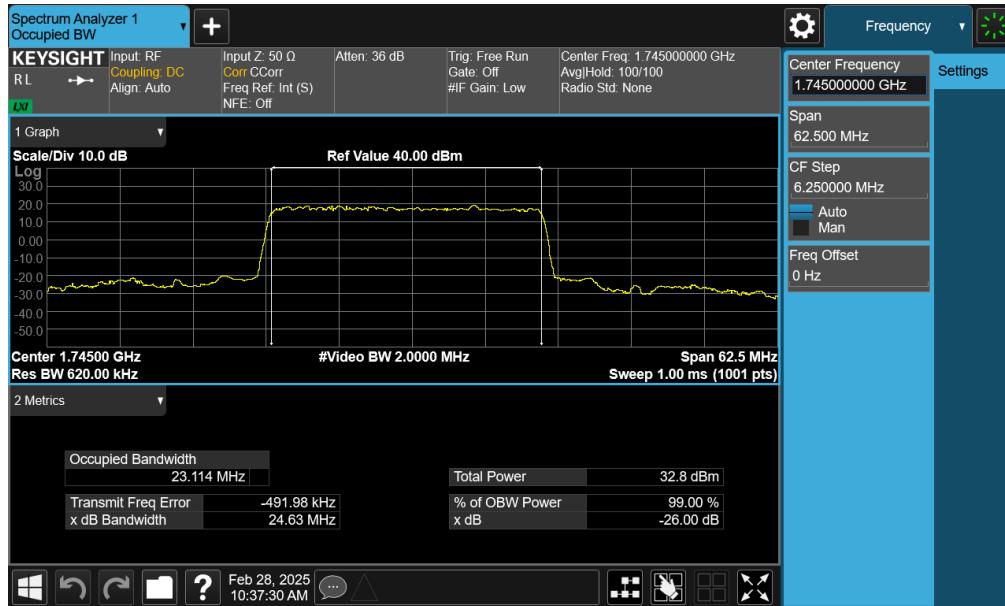
Plot 7-131. Occupied Bandwidth Plot (NR Band n66 - 25.0MHz DFT-s-OFDM BPSK - Full RB – ANT2)
