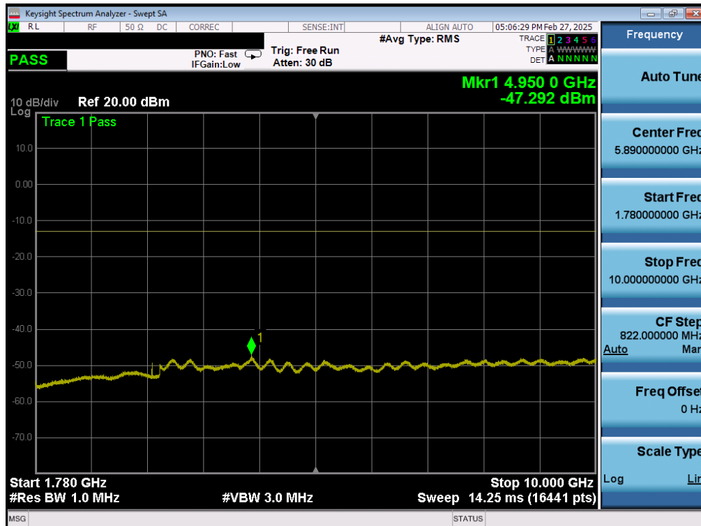
Plot 7-174. Conducted Spurious Plot (LTE Band 66/4 - 20MHz QPSK - 1 RB – Mid Channel)
