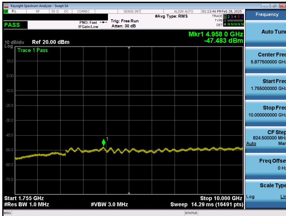
Plot 7-147. Conducted Spurious Plot (WCDMA-AWS - 5MHz QPSK - 1 RB – Low Channel)
