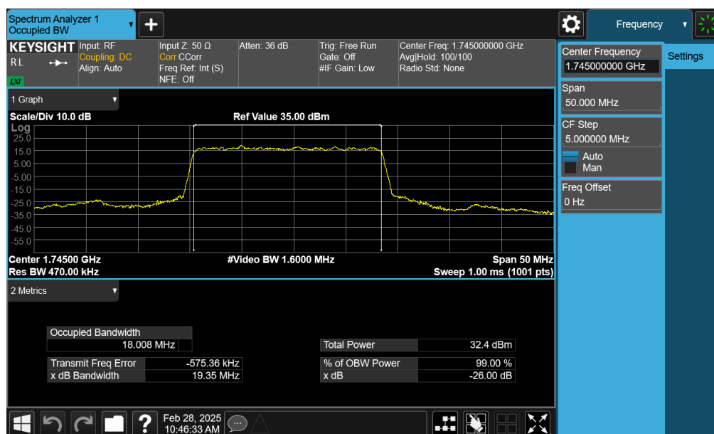
Plot 7-134. Occupied Bandwidth Plot (NR Band n66 - 20.0MHz DFT-s-OFDM BPSK - Full RB – ANT2)
