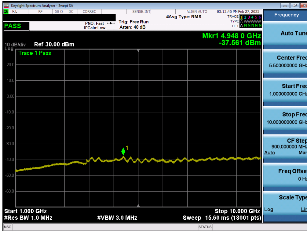
Plot 7-169. Conducted Spurious Plot (LTE Band 13 - 10MHz QPSK - 1 RB)
