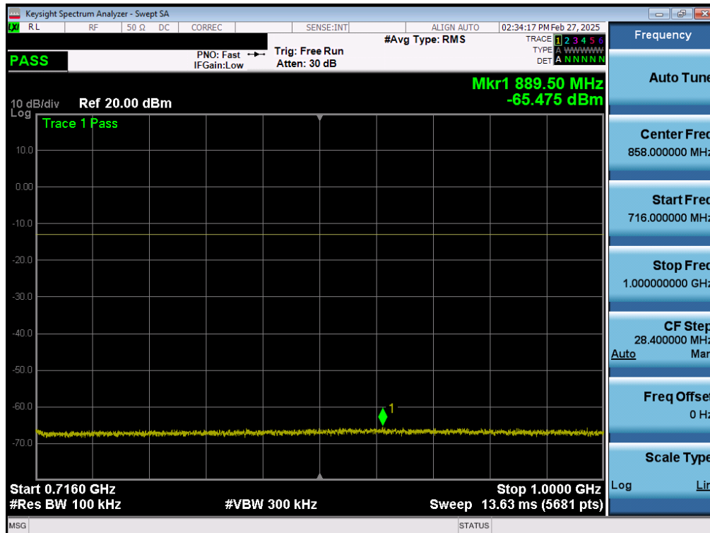
Plot 7-165. Conducted Spurious Plot (LTE Band 12/17 - 10MHz QPSK - 1 RB - Low Channel - ANT2)
