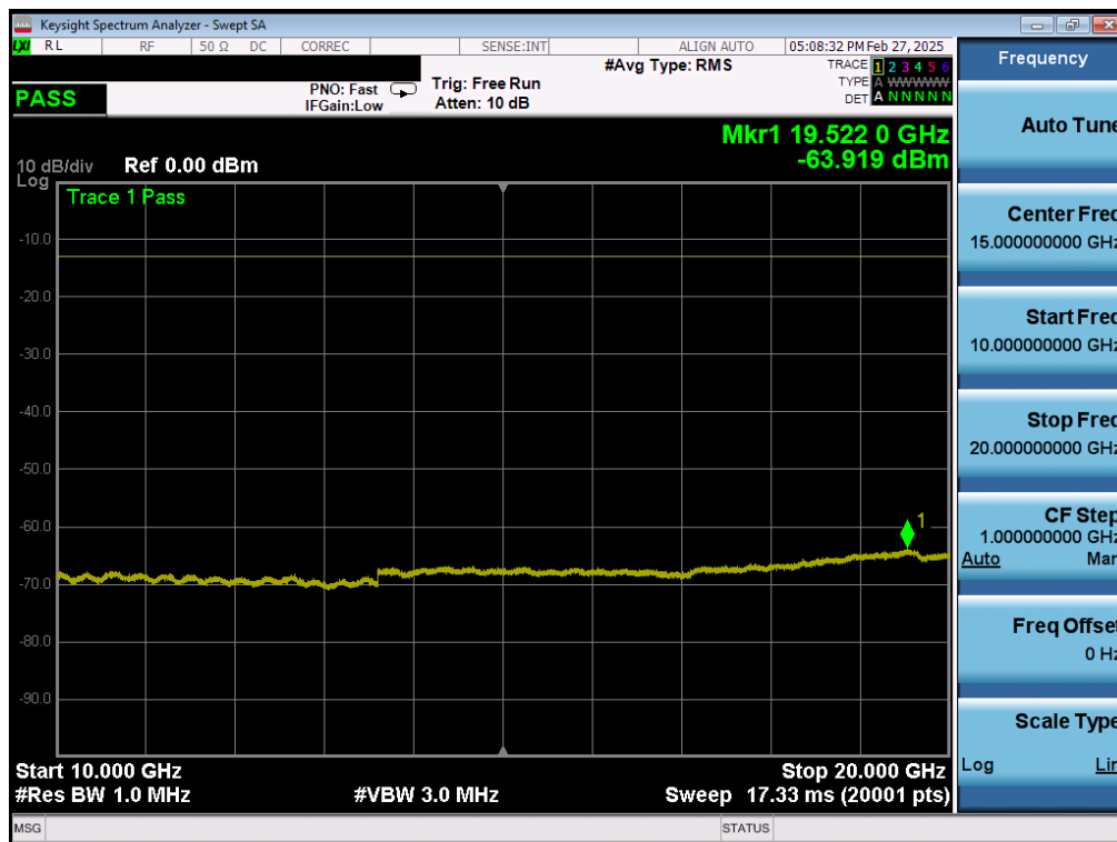
Plot 7-175. Conducted Spurious Plot (LTE Band 66/4 - 20MHz QPSK - 1 RB – High Channel)
