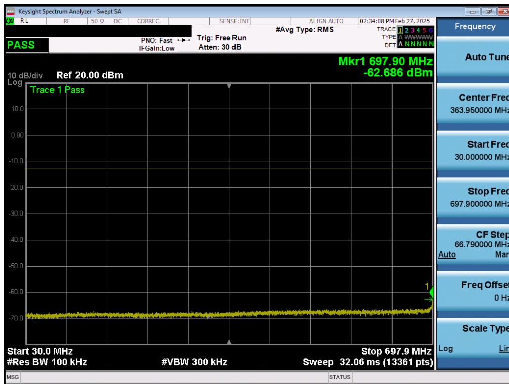
Plot 7-164. Conducted Spurious Plot (LTE Band 12/17 - 10MHz QPSK - 1 RB - Low Channel - ANT2)
