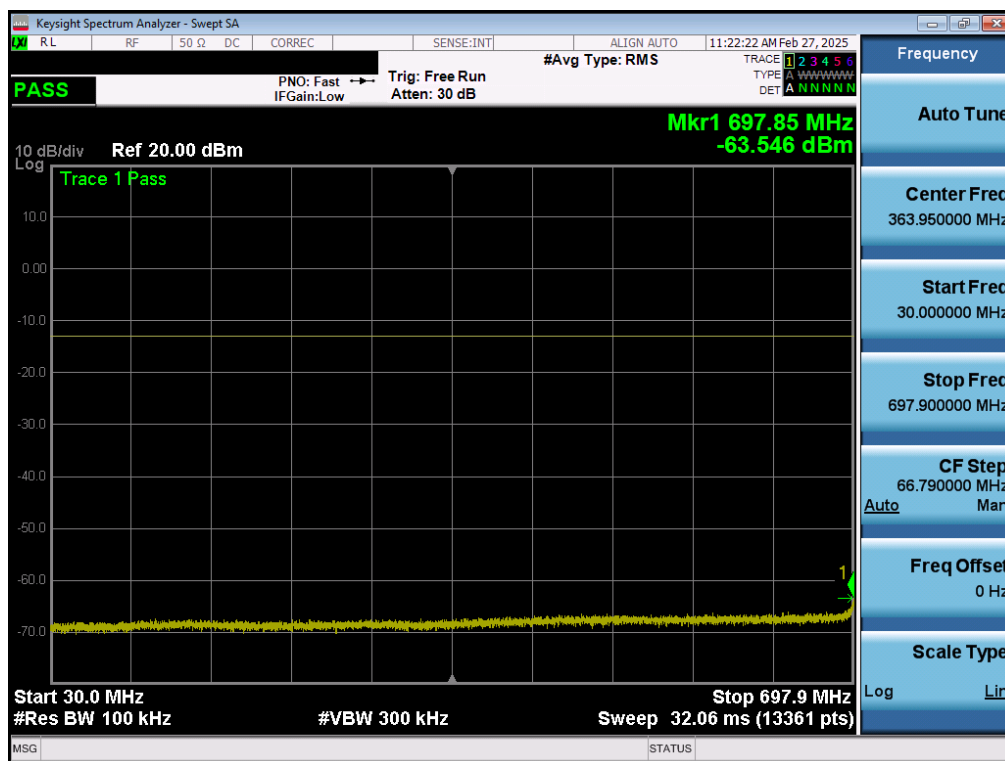
Plot 7-149. Conducted Spurious Plot (LTE Band 12/17 - 10MHz QPSK - 1 RB - Low Channel - ANT1)
