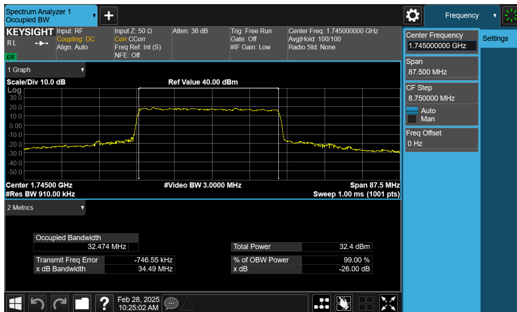
Plot 7-126. Occupied Bandwidth Plot (NR Band n66 - 35.0MHz CP-OFDM QPSK - Full RB – ANT2)
