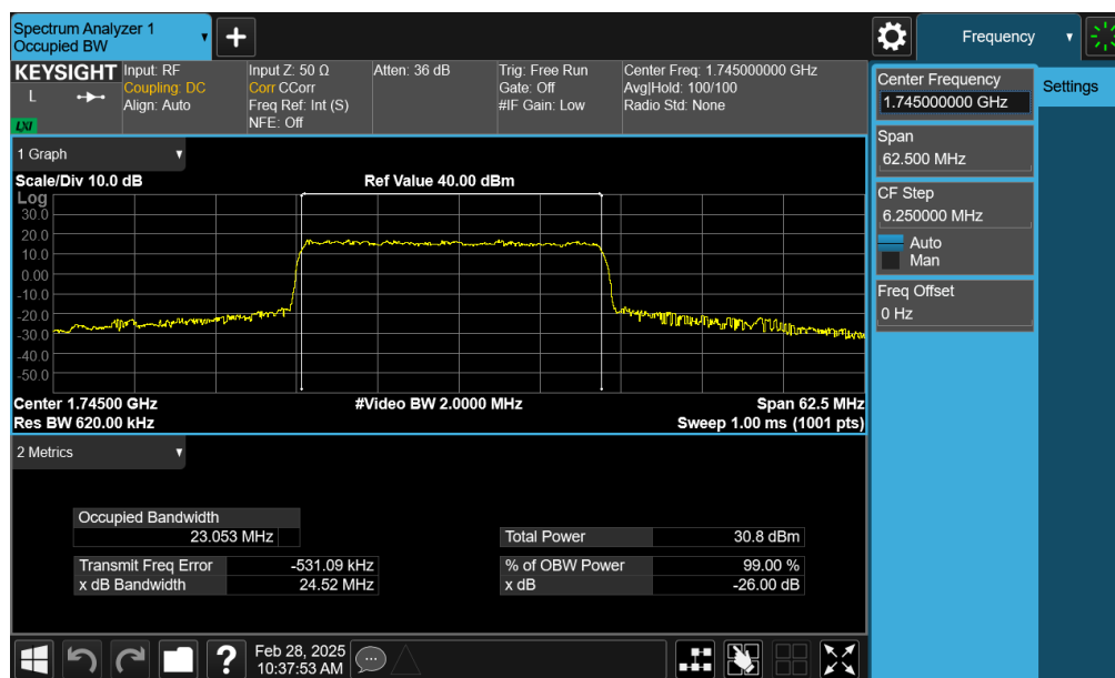
Plot 7-133. Occupied Bandwidth Plot (NR Band n66 - 25.0MHz CP-OFDM 16QAM - Full RB – ANT2)
