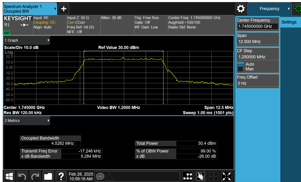
Plot 7-145. Occupied Bandwidth Plot (NR Band n66 - 5.0MHz CP-OFDM 16QAM - Full RB – ANT2)
