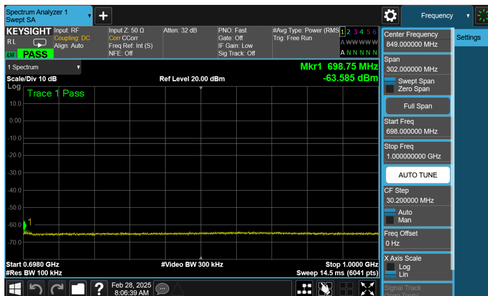
Plot 7-171. Conducted Spurious Plot (NR Band n71 - 35MHz - 1 RB - ANT2)
