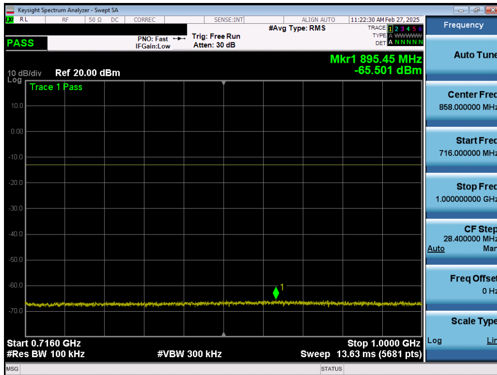
Plot 7-150. Conducted Spurious Plot (LTE Band 12/17 - 10MHz QPSK - 1 RB - Low Channel - ANT1)
