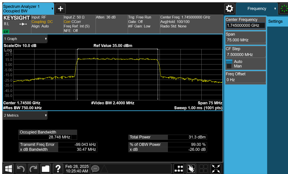
Plot 7-130. Occupied Bandwidth Plot (NR Band n66 - 30.0MHz CP-OFDM 16QAM - Full RB – ANT2)
