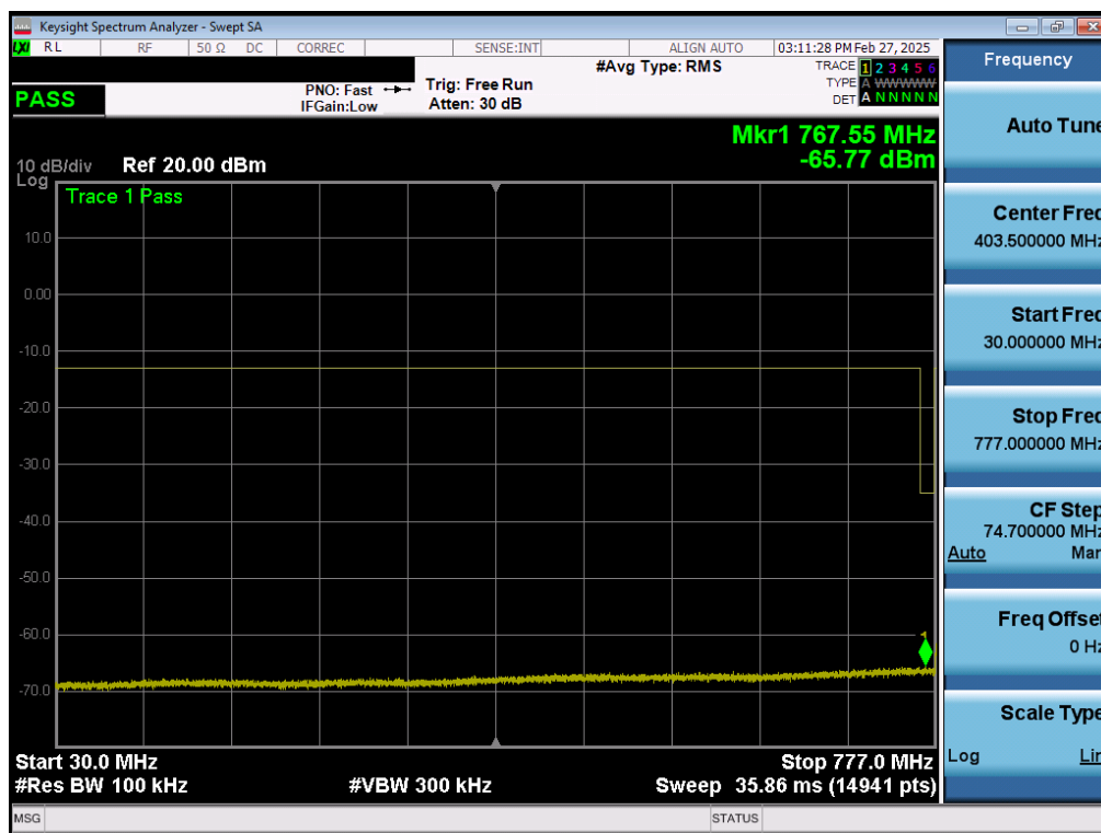
Plot 7-167. Conducted Spurious Plot (LTE Band 13 - 10MHz QPSK - 1 RB)
