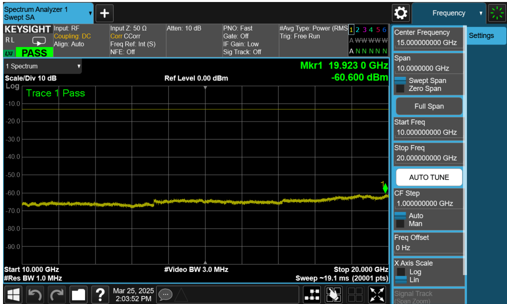
Plot 7-163. Conducted Spurious Plot (NR Band n66 - 45.0MHz - 1 RB - Low Channel - ANT1)
