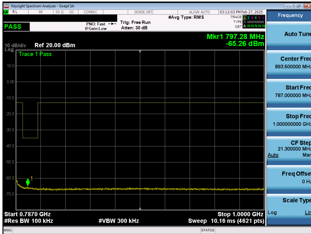
Plot 7-168. Conducted Spurious Plot (LTE Band 13 - 10MHz QPSK - 1 RB)
