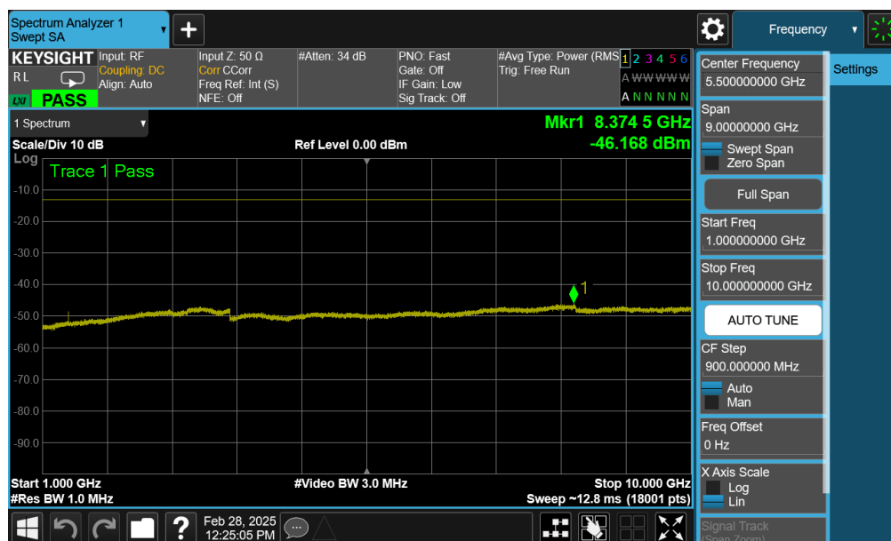
Plot 7-157. Conducted Spurious Plot (NR Band n71 - 35MHz - 1 RB - ANT1)
