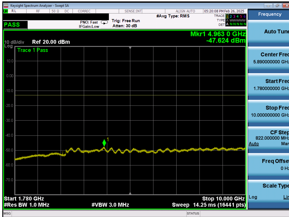
Plot 7-159. Conducted Spurious Plot (LTE Band 66/4 - 20MHz QPSK - 1 RB – Mid Channel)
