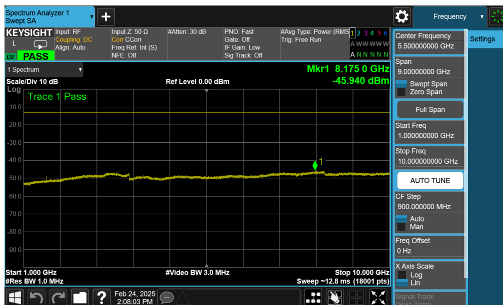
Plot 7-154. Conducted Spurious Plot (LTE Band 13 - 10MHz QPSK - 1 RB)
