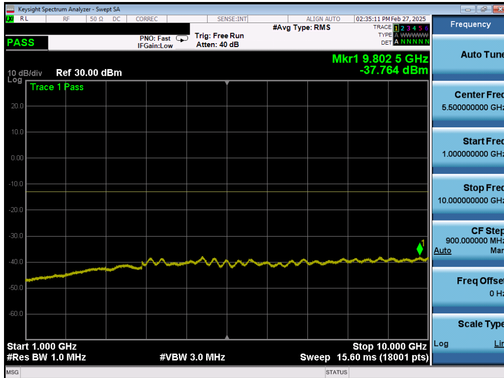
Plot 7-166. Conducted Spurious Plot (LTE Band 12/17 - 10MHz QPSK - 1 RB - Low Channel - ANT2)
