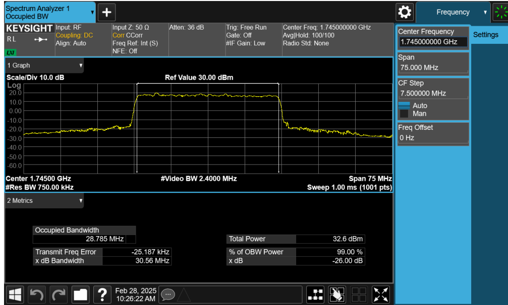
Plot 7-129. Occupied Bandwidth Plot (NR Band n66 - 30.0MHz CP-OFDM QPSK - Full RB – ANT2)
