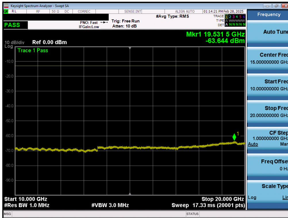
Plot 7-148. Conducted Spurious Plot (WCDMA-AWS - 5MHz QPSK - 1 RB – Low Channel)
