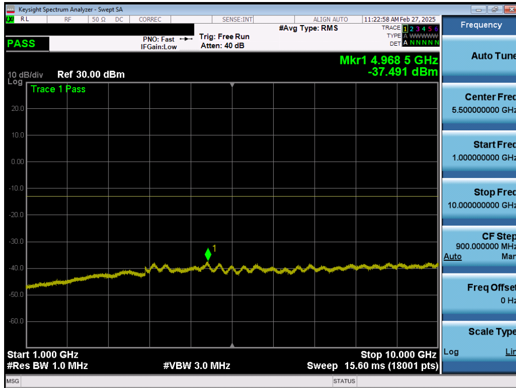
Plot 7-151. Conducted Spurious Plot (LTE Band 12/17 - 10MHz QPSK - 1 RB - Low Channel - ANT1)
