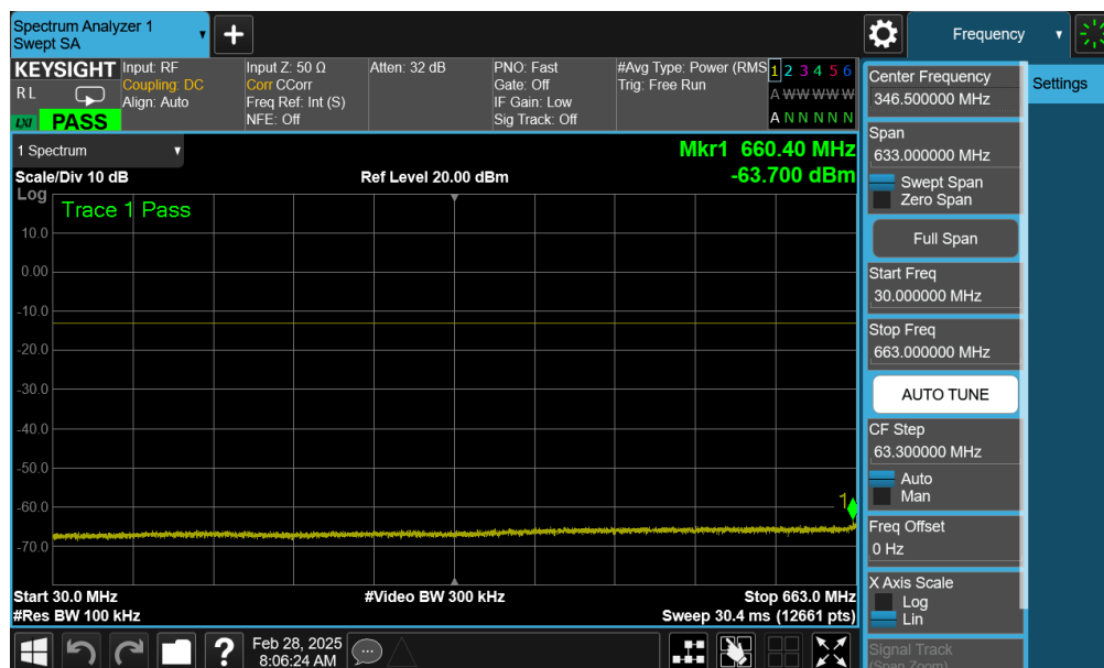
Plot 7-170. Conducted Spurious Plot (NR Band n71 - 35MHz - 1 RB - ANT2)
