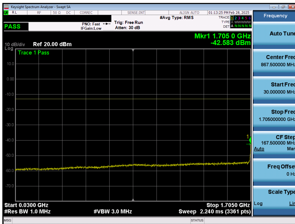
Plot 7-146. Conducted Spurious Plot (WCDMA-AWS - 5MHz QPSK - 1 RB – Low Channel)
