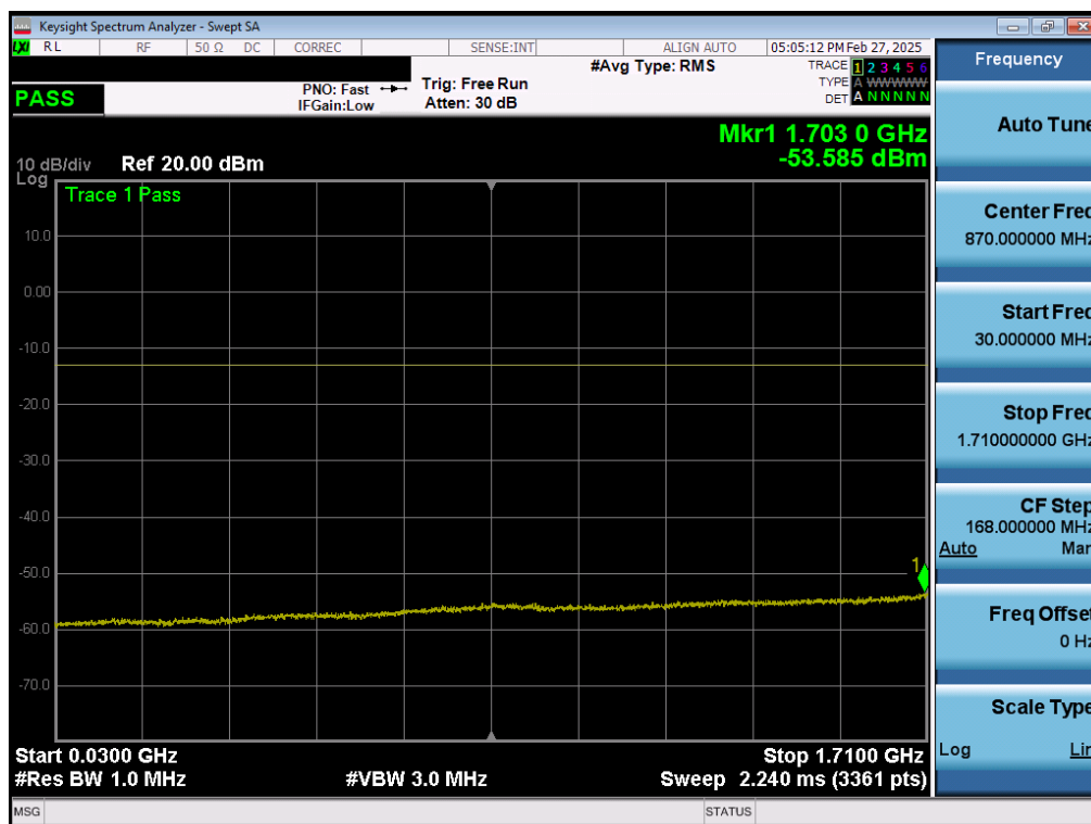
Plot 7-173. Conducted Spurious Plot (LTE Band 66/4 - 20MHz QPSK - 1 RB – Mid Channel)
