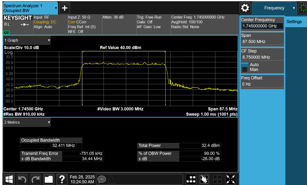
Plot 7-125. Occupied Bandwidth Plot (NR Band n66 - 35.0MHz DFT-s-OFDM BPSK - Full RB – ANT2)
