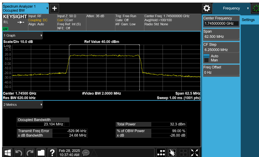
Plot 7-132. Occupied Bandwidth Plot (NR Band n66 - 25.0MHz CP-OFDM QPSK - Full RB – ANT2)
