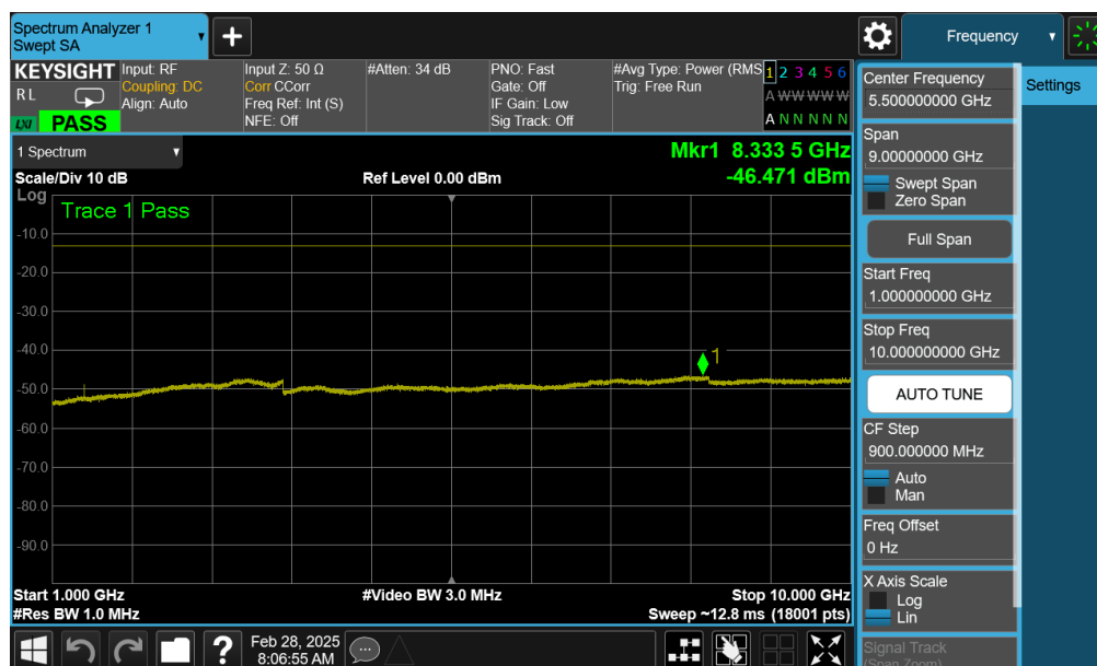
Plot 7-172. Conducted Spurious Plot (NR Band n71 - 35MHz - 1 RB - ANT2)
