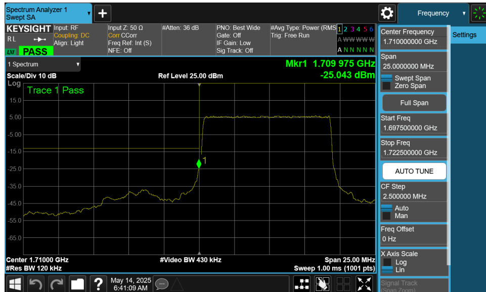
Plot 6-17. Lower Band Edge Plot (NR Band n66 – 10.0MHz - Full RB - ANT2)
