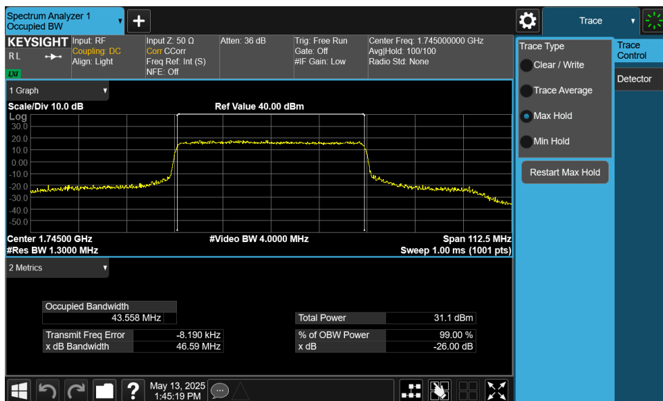
Plot 6-5. Occupied Bandwidth Plot (NR Band n66 - 45.0MHz CP-OFDM QPSK - Full RB – ANT2)
