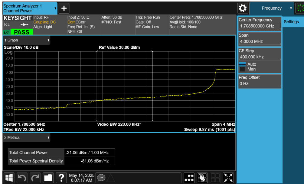
Plot 6-12. Lower Extended Band Edge Plot (LTE Band 66/4 - 3MHz QPSK – Full RB - ANT2)
