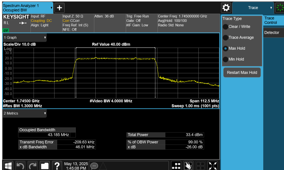
Plot 6-4. Occupied Bandwidth Plot (NR Band n66 - 45.0MHz DFT-s-OFDM BPSK - Full RB – ANT2)
