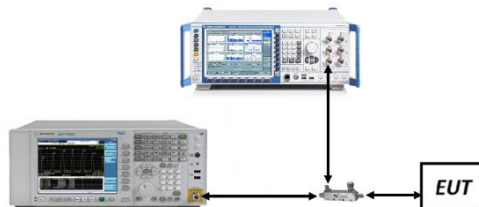
Figure 6-3. Test Instrument & Measurement Setup
