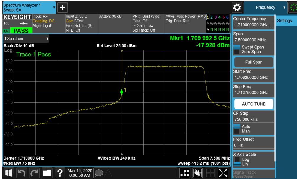
Plot 6-11. Lower Band Edge Plot (LTE Band 66/4 - 3MHz QPSK – Full RB - ANT2)
