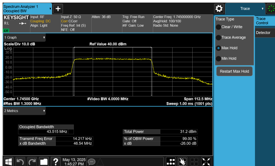
Plot 6-6. Occupied Bandwidth Plot (NR Band n66 - 45.0MHz CP-OFDM 16QAM - Full RB - ANT2)
