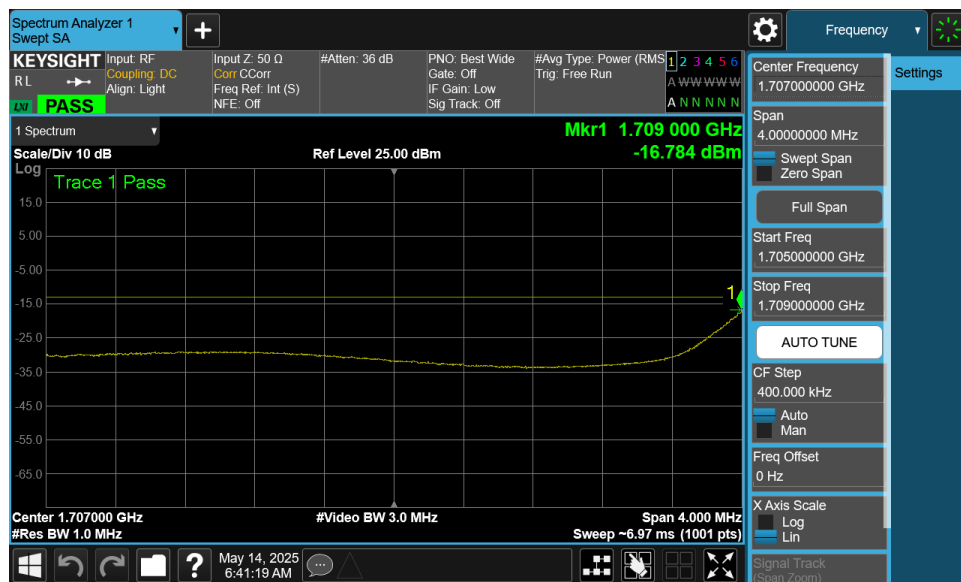
Plot 6-18. Lower Extended Band Edge Plot (NR Band n66 – 10.0MHz - Full RB - ANT2)
