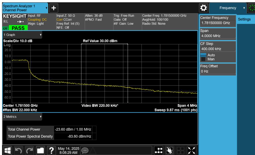
Plot 6-16. Upper Extended Band Edge Plot (LTE Band 66 - 3MHz QPSK – Full RB - ANT2)
