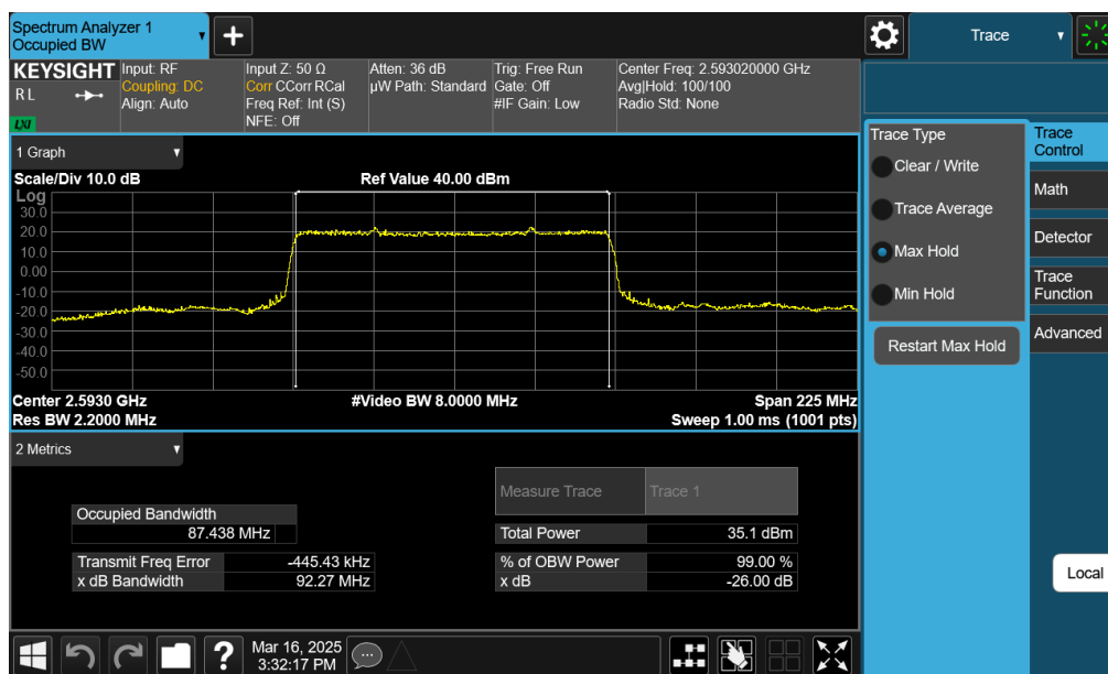
Plot 7-20. Occupied Bandwidth Plot (NR Band n41 PC2 – 90MHz \pi/2 BPSK – Full RB – Default – Ant1)
