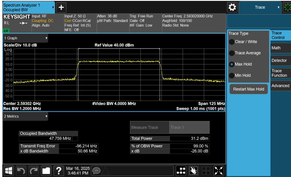
Plot 7-33. Occupied Bandwidth Plot (NR Band n41 PC2 – 50MHz QPSK – Full RB – Default – Ant1)
