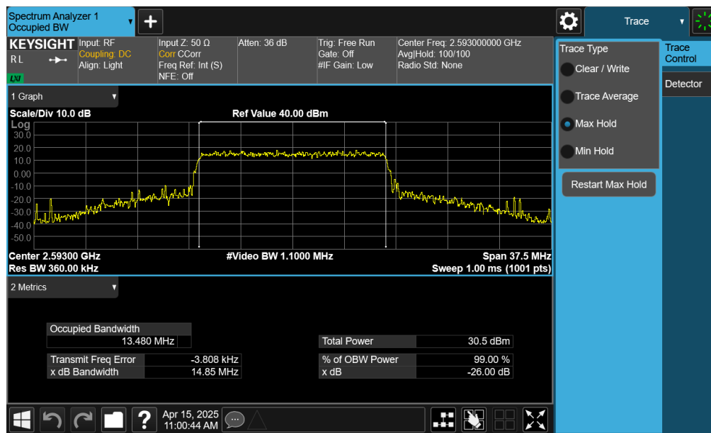
Plot 7-12. Occupied Bandwidth Plot (LTE Band 41(PC2) - 15MHz 16-QAM - Full RB - Ant1)
