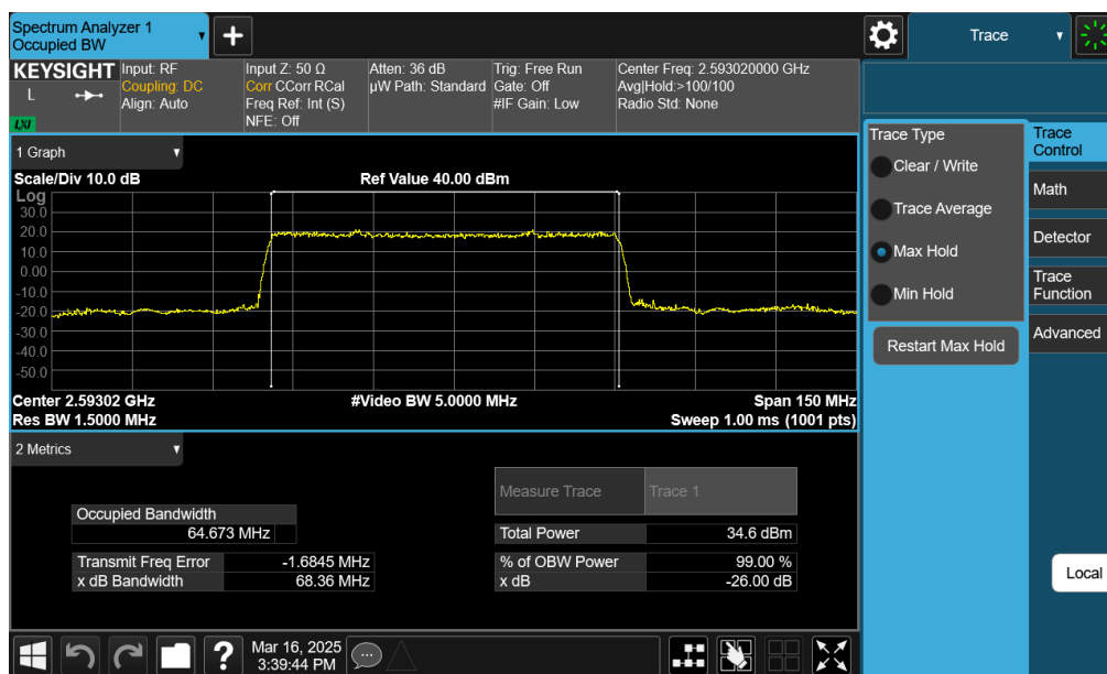
Plot 7-26. Occupied Bandwidth Plot (NR Band n41 PC2 – 70MHz \pi/2 BPSK – Full RB – Default – Ant1)
