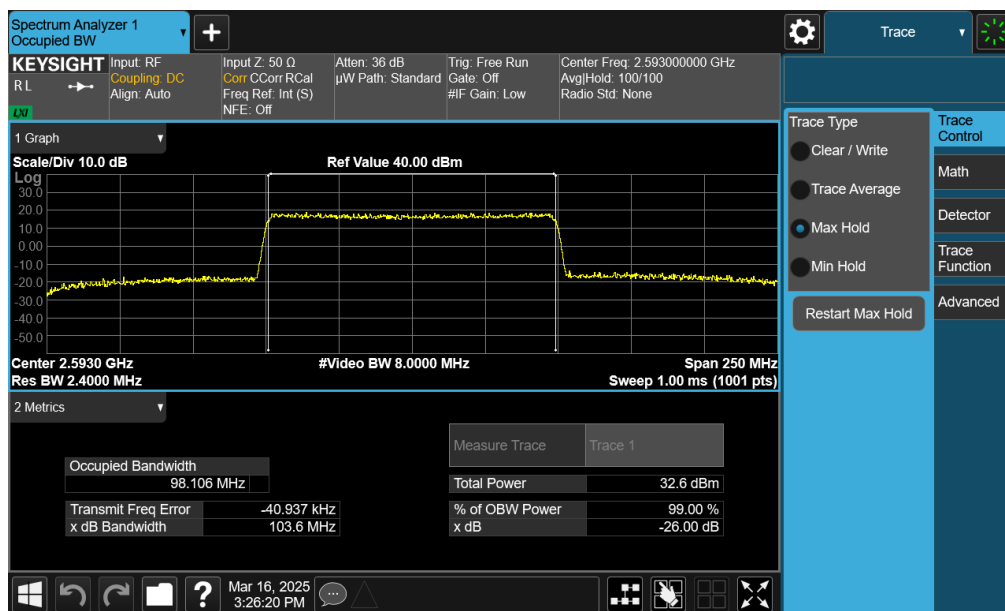
Plot 7-18. Occupied Bandwidth Plot (NR Band n41 PC2 – 100MHz QPSK – Full RB – Default – Ant1)
