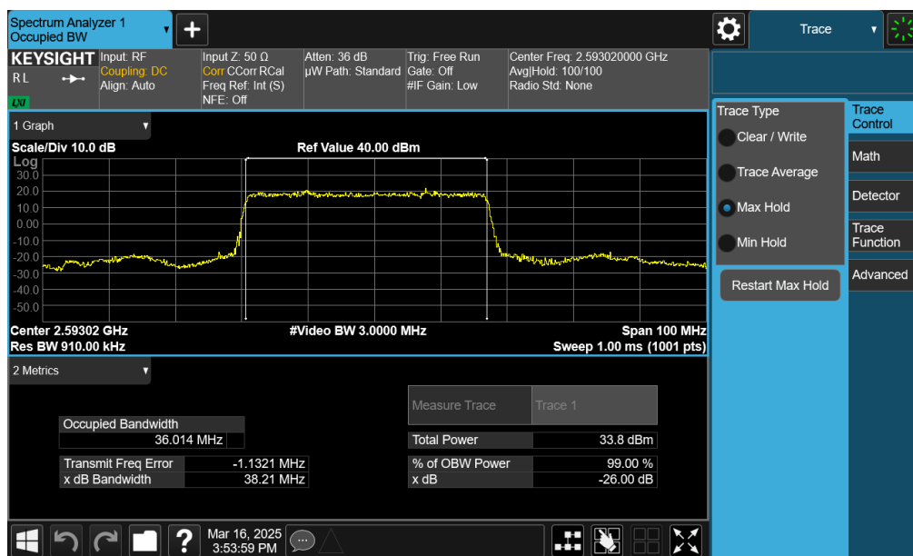
Plot 7-38. Occupied Bandwidth Plot (NR Band n41 PC2 – 40MHz \pi/2 BPSK – Full RB – Default – Ant1)
