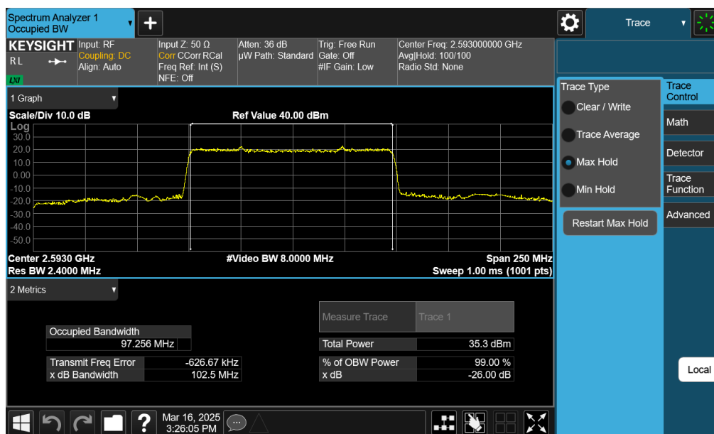
Plot 7-17. Occupied Bandwidth Plot (NR Band n41 PC2 – 100MHz \pi/2 BPSK – Full RB – Default – Ant1)
