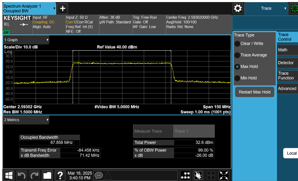
Plot 7-28. Occupied Bandwidth Plot (NR Band n41 PC2 – 70MHz 16-QAM – Full RB – Default – Ant1)
