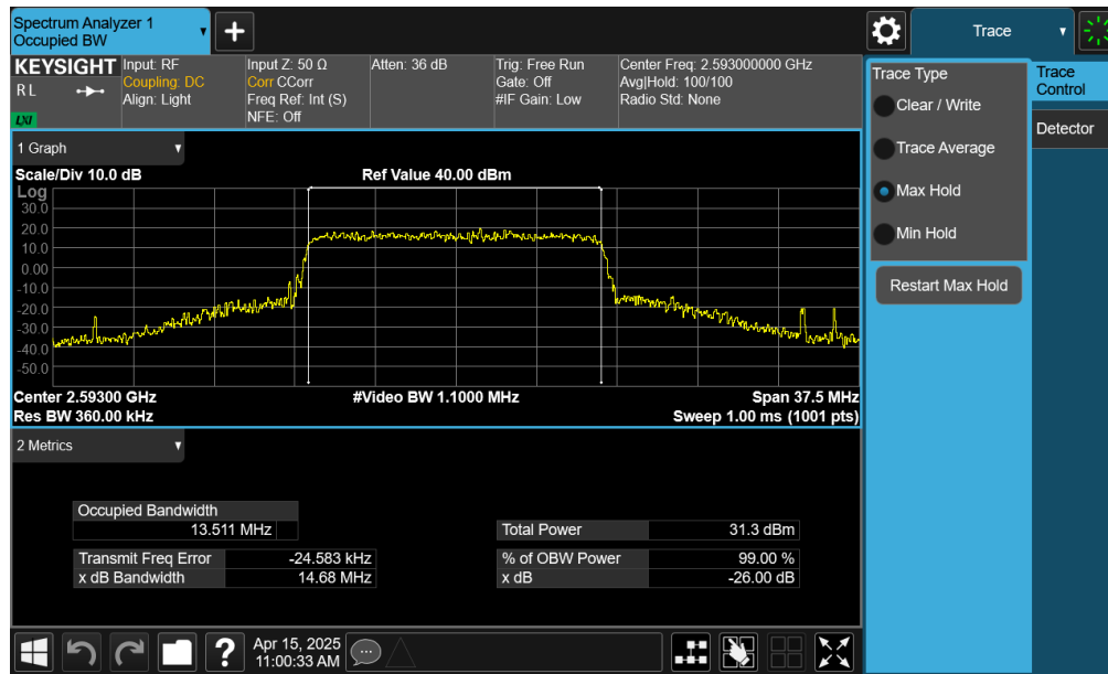
Plot 7-11. Occupied Bandwidth Plot (LTE Band 41(PC2) - 15MHz QPSK - Full RB - Ant1)
