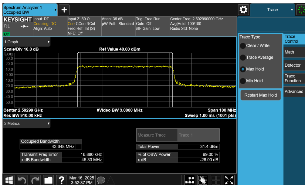
Plot 7-37. Occupied Bandwidth Plot (NR Band n41 PC2 – 45MHz 16-QAM – Full RB – Default – Ant1)
