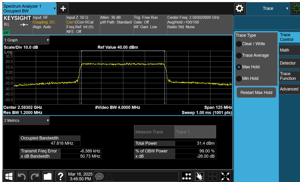
Plot 7-34. Occupied Bandwidth Plot (NR Band n41 PC2 – 50MHz 16-QAM – Full RB – Default – Ant1)
