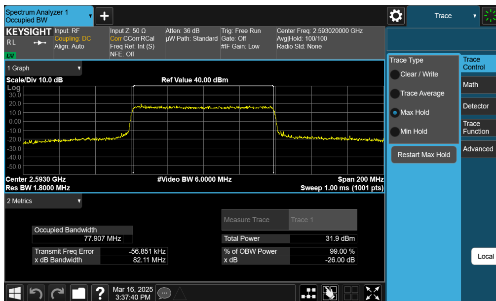
Plot 7-25. Occupied Bandwidth Plot (NR Band n41 PC2 – 80MHz 16-QAM – Full RB – Default – Ant1)
