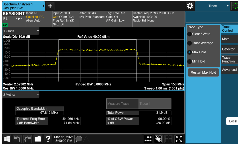
Plot 7-27. Occupied Bandwidth Plot (NR Band n41 PC2 – 70MHz QPSK – Full RB – Default – Ant1)
