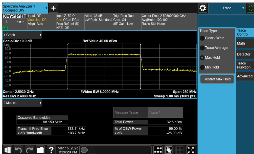
Plot 7-19. Occupied Bandwidth Plot (NR Band n41 PC2 – 100MHz 16-QAM – Full RB – Default – Ant1)
