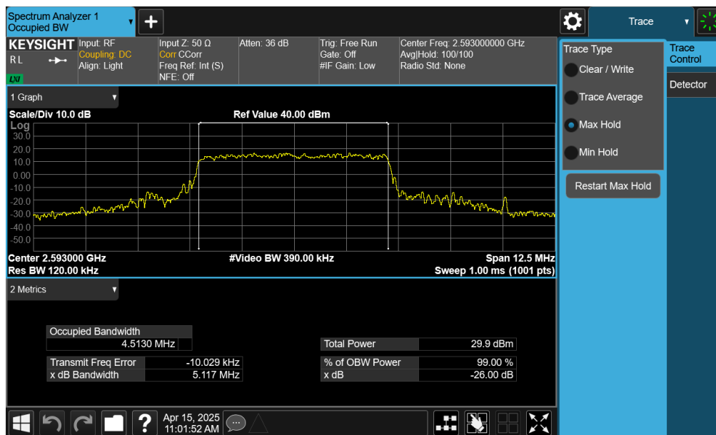
Plot 7-16. Occupied Bandwidth Plot (LTE Band 41(PC2) - 5MHz 16-QAM - Full RB - Ant1)
