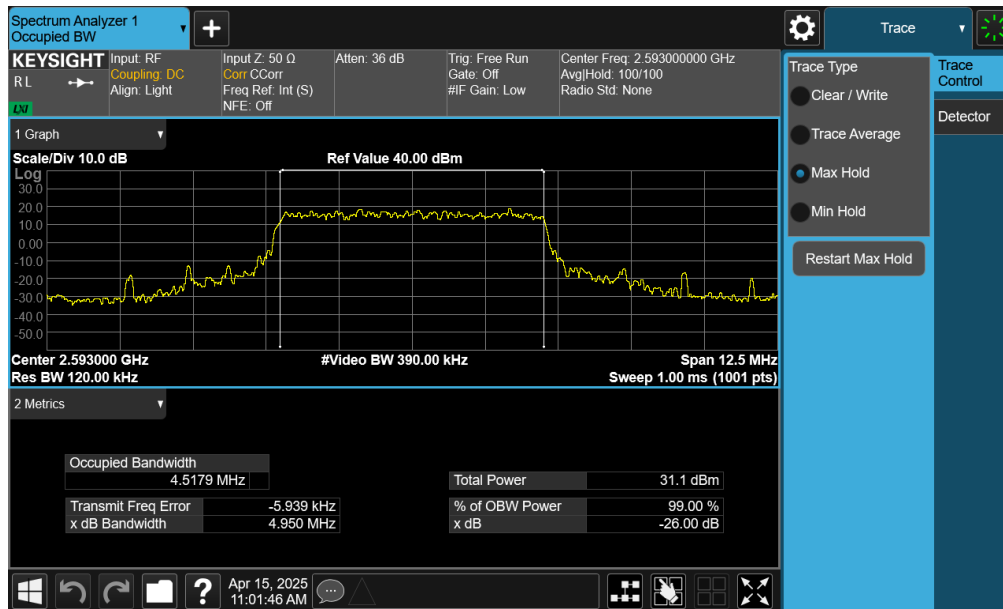
Plot 7-15. Occupied Bandwidth Plot (LTE Band 41(PC2) - 5MHz QPSK - Full RB - Ant1)
