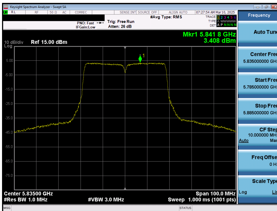
Plot 7-87. Power Spectral Density Plot MIMO ANT1 (40MHz 802.11n (UNII Band 3/4) – Ch. 167)
