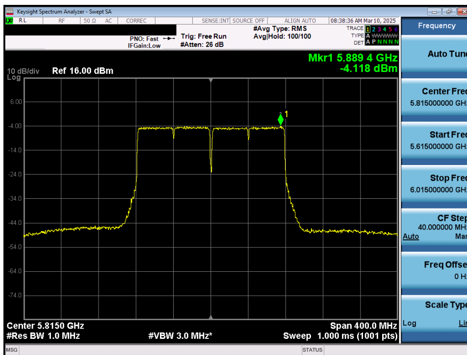
Plot 7-91. Power Spectral Density Plot MIMO ANT1 (160MHz 802.11ac (UNII Band 3/4) – Ch. 163)
