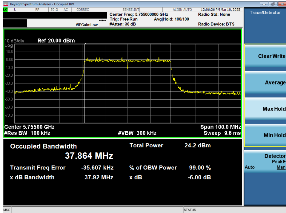
Plot 7-49. 6dB Bandwidth Plot MIMO ANT2 (40MHz 802.11ax/be (UNII Band 3) – Ch. 151)
