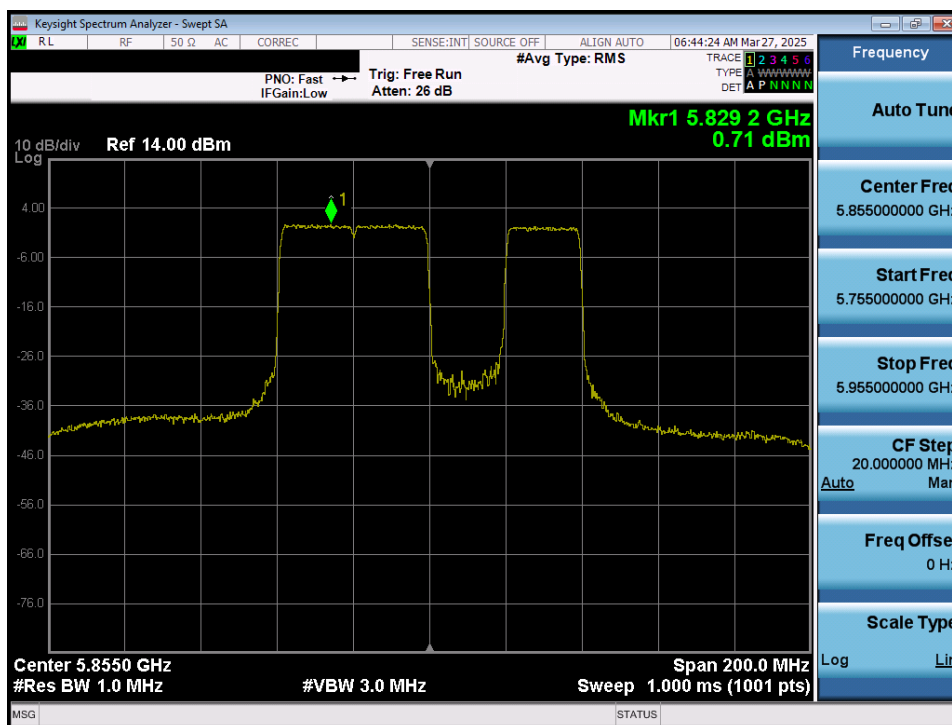
Plot 7-93. Power Spectral Density Plot MIMO ANT1 (80MHz 802.11be (20MHz Puncture) (UNII Band 3/4) – Ch. 171)
