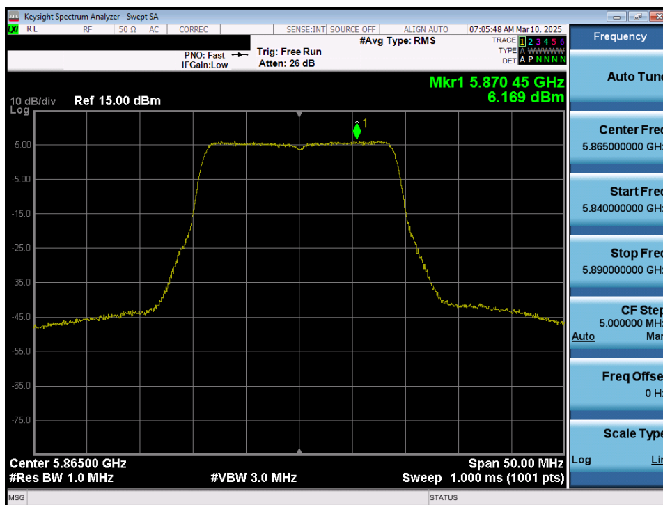
Plot 7-85. Power Spectral Density Plot MIMO ANT1 (20MHz 802.11n (UNII Band 4) – Ch.173)
