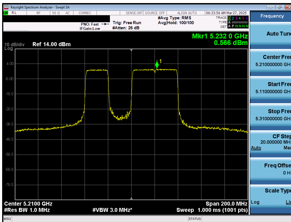
Plot 7-74. Power Spectral Density Plot MIMO ANT1 (80MHz 802.11be (20MHz Puncture) (UNII Band 1) – Ch. 42)
