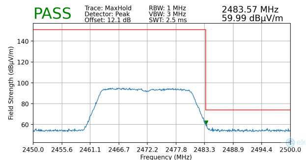
Plot 7-105. Radiated Restricted Upper Band Edge Measurement MIMO (Peak)
