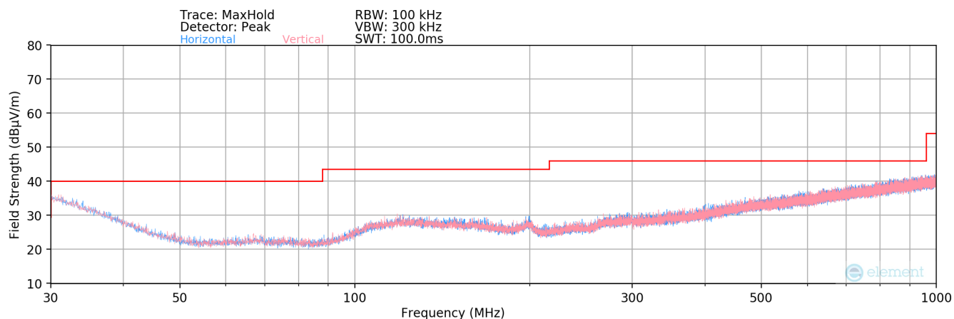
Plot 7-93. Radiated Spurious Plot below 1GHz MIMO
