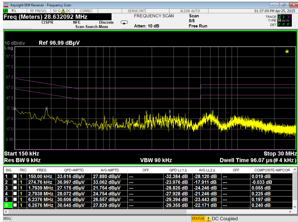
Plot 7-108. Line Conducted Plot with 802.11b (L1)
