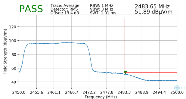
Plot 7-106. Radiated Restricted Band Edge Measurement MIMO with WCP (Average)
