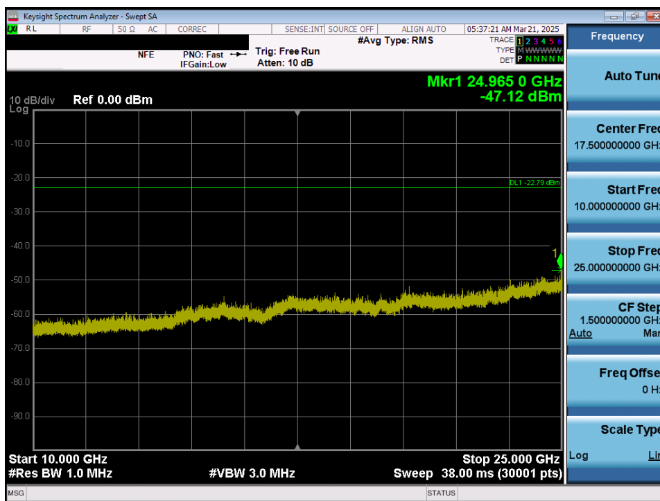
Plot 7-90. Conducted Spurious Plot MIMO ANT2 (802.11b – Ch. 6)
