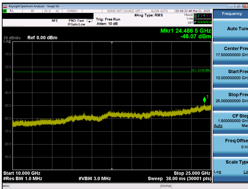
Plot 7-86. Conducted Spurious Plot MIMO ANT1 (802.11b – Ch. 11)
