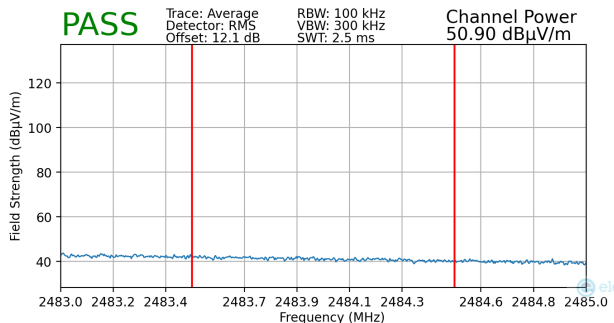
Plot 7-100. Radiated Restricted Upper Band Edge Measurement MIMO (Average)
