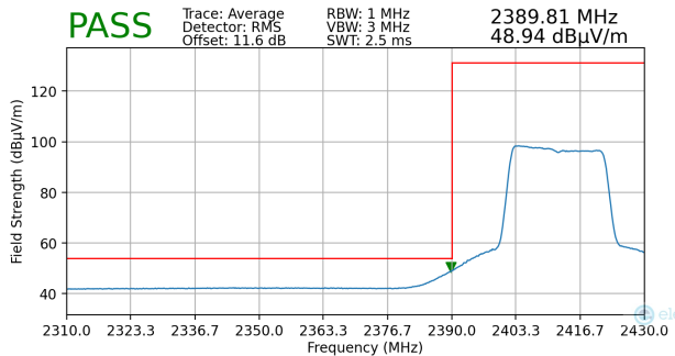
Plot 7-98. Radiated Restricted Lower Band Edge Measurement MIMO (Average)
