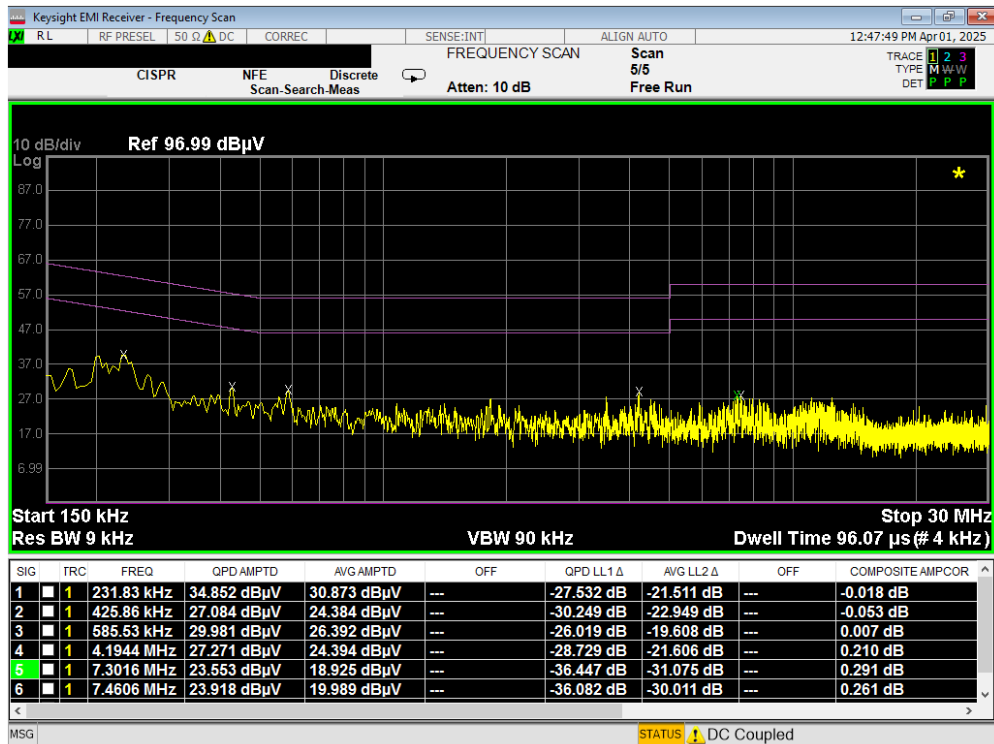
Plot 7-111. Line Conducted Plot with 802.11b (N) with WCP
