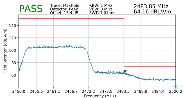
Plot 7-107. Radiated Restricted Band Edge Measurement MIMO with WCP (Peak)
