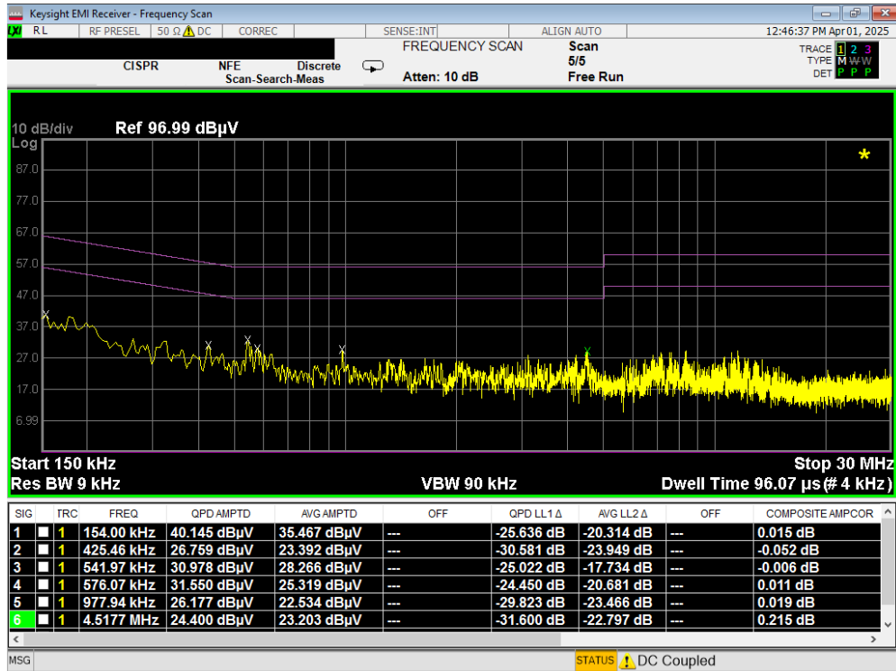
Plot 7-110. Line Conducted Plot with 802.11b (L1) with WCP
