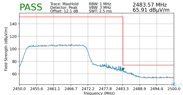
Plot 7-101. Radiated Restricted Upper Band Edge Measurement MIMO (Peak)
