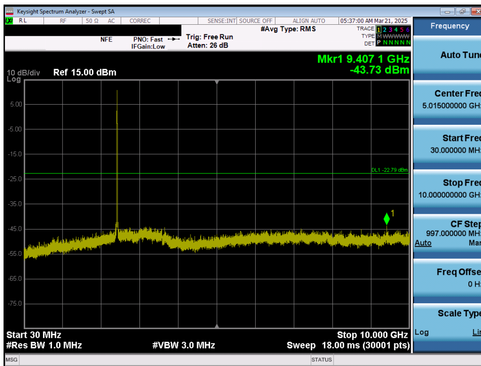
Plot 7-89. Conducted Spurious Plot MIMO ANT2 (802.11b – Ch. 6)
