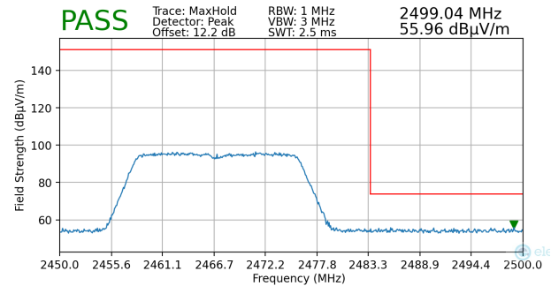
Plot 7-103. Radiated Restricted Upper Band Edge Measurement MIMO (Peak)
