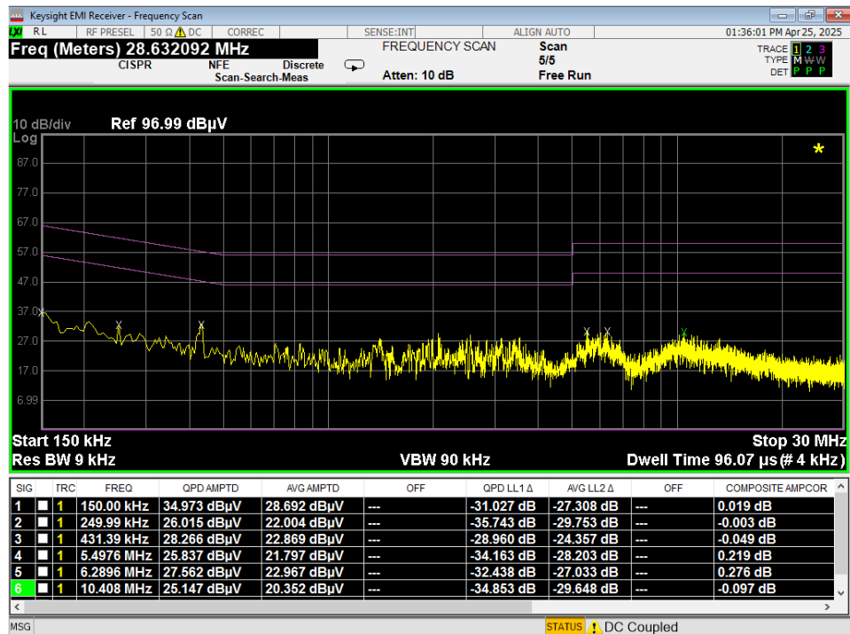
Plot 7-109. Line Conducted Plot with 802.11b (N)
