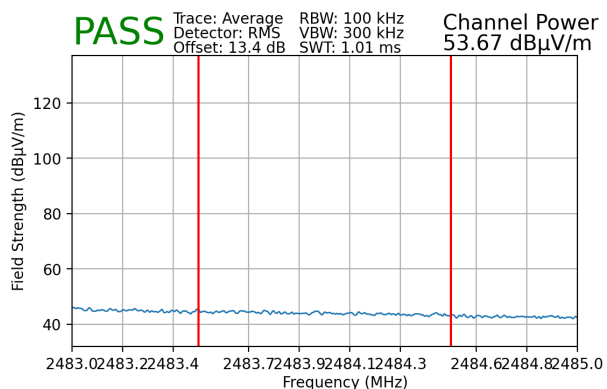
Plot 9-1. Radiated Restricted Upper Band Edge Measurement MIMO (Average)
