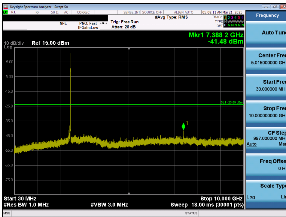
Plot 7-85. Conducted Spurious Plot MIMO ANT1 (802.11b – Ch. 11)
