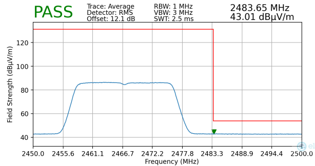
Plot 7-102. Radiated Restricted Upper Band Edge Measurement MIMO (Average)
