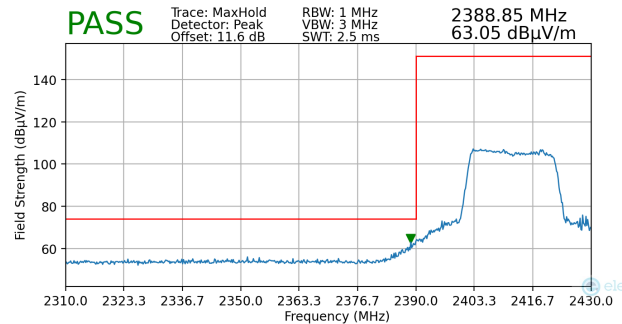
Plot 7-99. Radiated Restricted Lower Band Edge Measurement MIMO (Peak)
