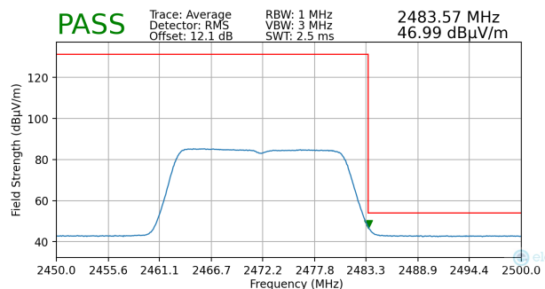
Plot 7-104. Radiated Restricted Upper Band Edge Measurement MIMO (Average)
