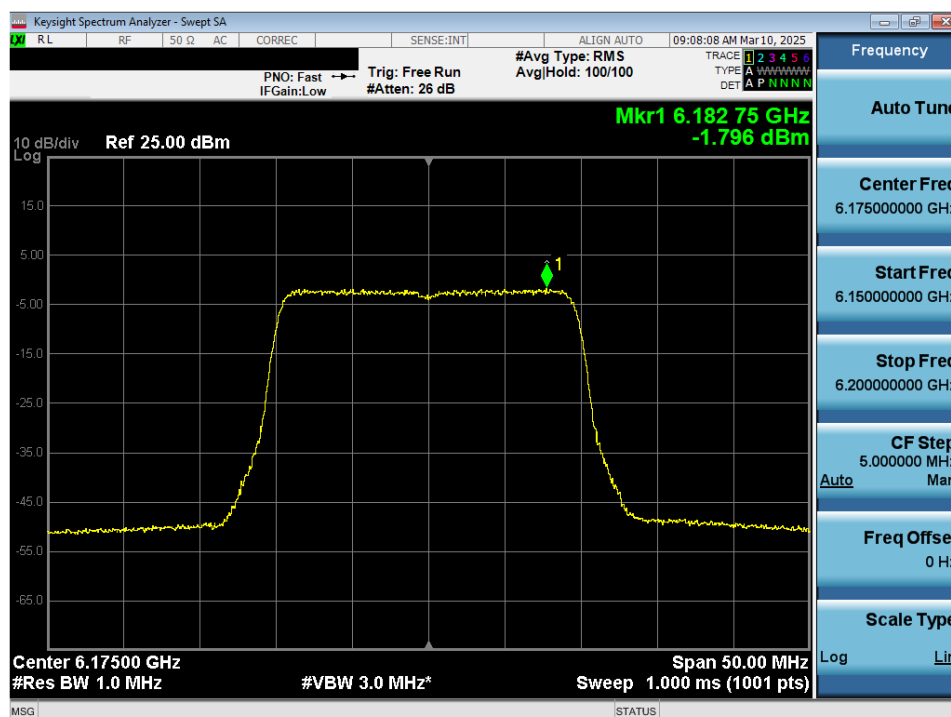
Plot 7-38. Power Spectral Density Plot MIMO ANT2 (20MHz 802.11ax/be (UNII Band 5) – Ch. 45) - LPI
