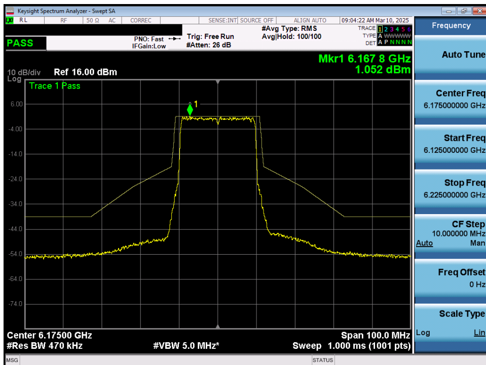
Plot 7-59. In Band Emissions Plot MIMO ANT1 (20MHz 802.11ax/be (UNII Band 5) – Ch. 45) - SP
