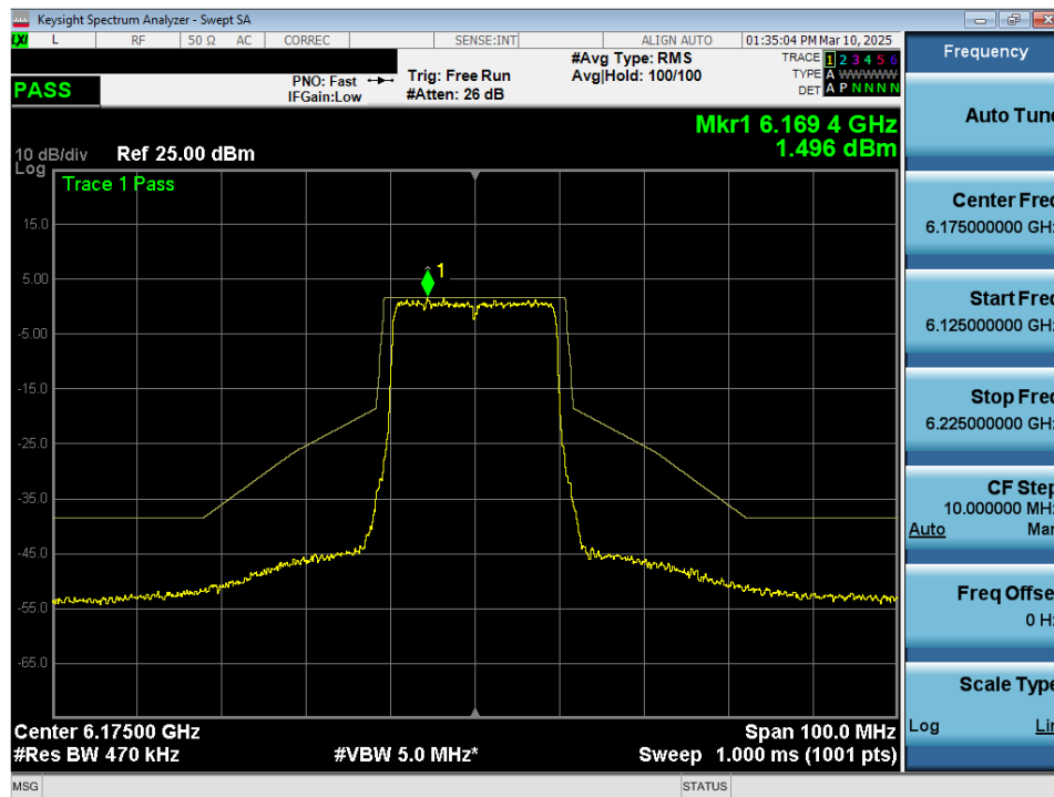
Plot 7-71. In Band Emissions Plot MIMO ANT2 (20MHz 802.11ax/be (UNII Band 5) – Ch. 45) - SP
