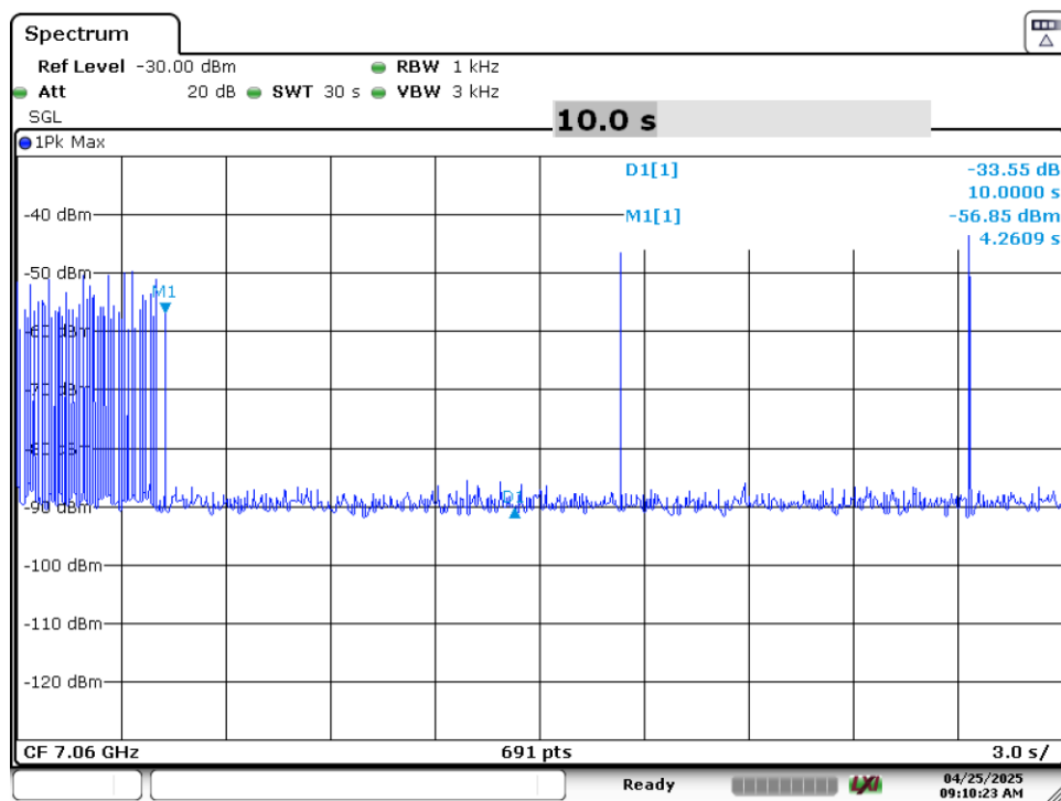
Plot 7-88. Contention Based Protocol Timing Plot (320MHz (UNII Band 8) – Ch. 191 Mid)
