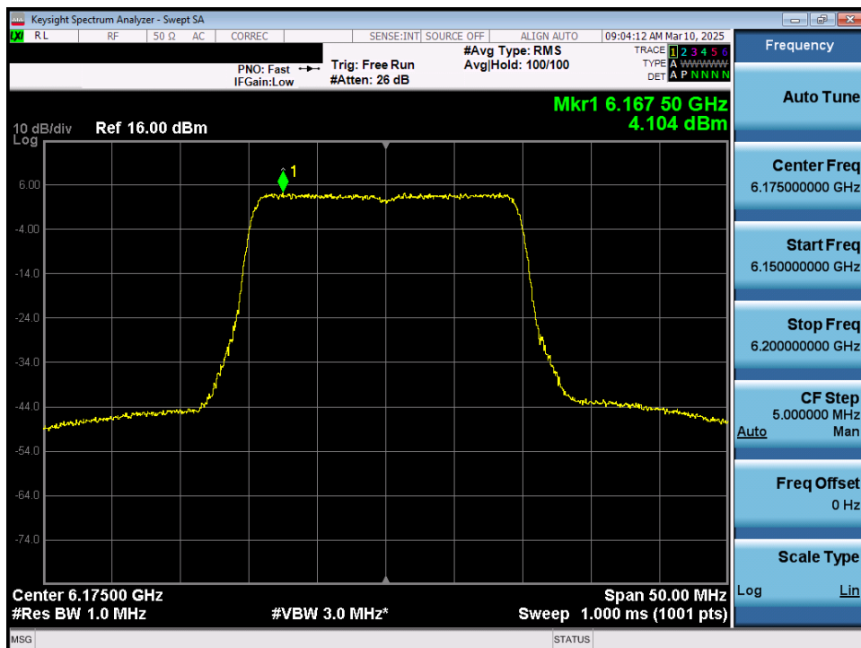
Plot 7-35. Power Spectral Density Plot MIMO ANT1 (20MHz 802.11ax/be (UNII Band 5) – Ch. 45) - SP
