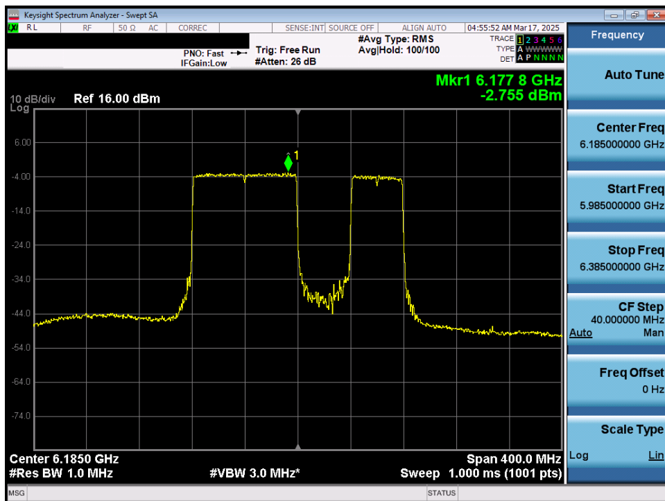
Plot 7-32. Power Spectral Density Plot MIMO ANT1 (160MHz 802.11be (UNII Band 5) – Ch. 47) – 40MHz Punctured - LPI/SP
