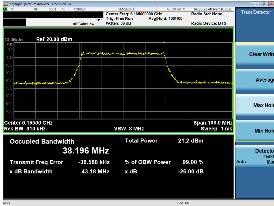
Plot 7-15. 26dB Bandwidth Plot MIMO ANT2 (40MHz 802.11ax/be (UNII Band 5) – Ch. 43) - LPI
