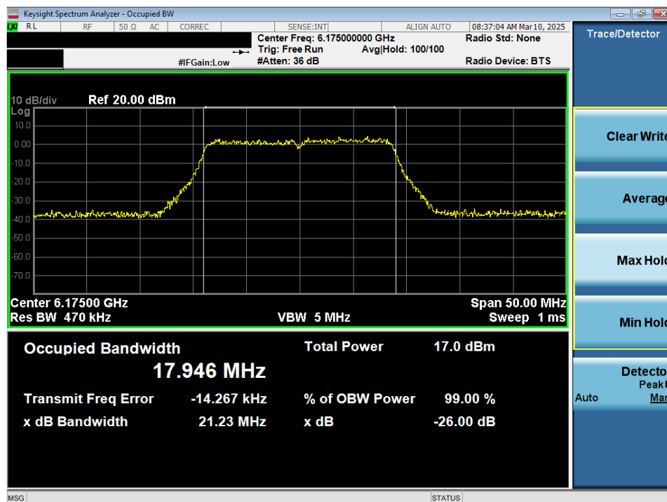
Plot 7-13. 26dB Bandwidth Plot MIMO ANT2 (20MHz 802.11a (UNII Band 5) – Ch. 45) - LPI
