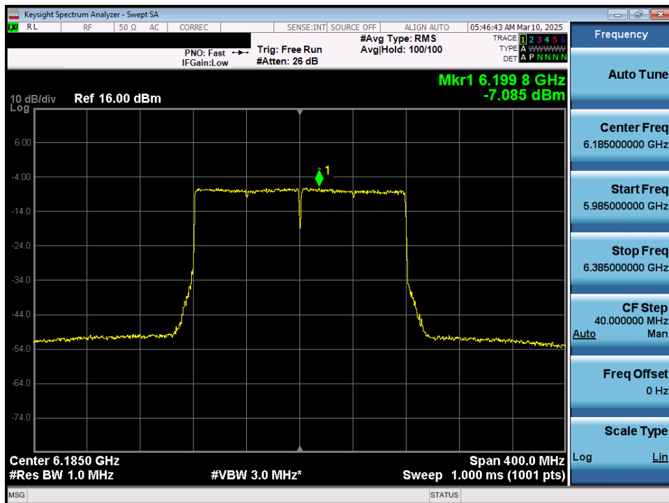
Plot 7-29. Power Spectral Density Plot MIMO ANT1 (160MHz 802.11ax/be (UNII Band 5) – Ch. 47) - LPI/SP
