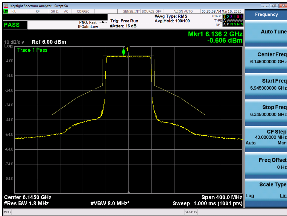
Plot 7-52. In Band Emissions Plot MIMO ANT1 (80MHz 802.11ax/be (UNII Band 5) – Ch. 39) – LPI/SP
