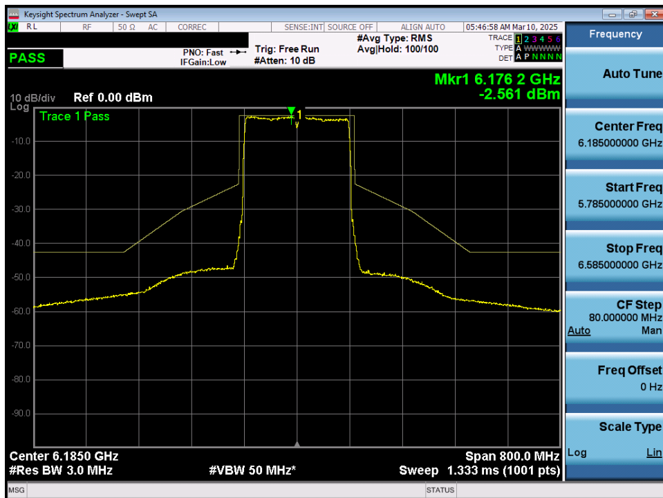
Plot 7-53. In Band Emissions Plot MIMO ANT1 (160MHz 802.11ax/be (UNII Band 5) – Ch. 47) - LPI/SP
