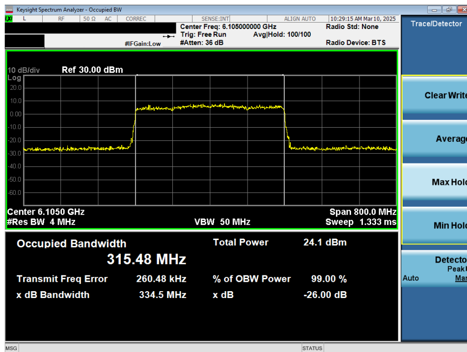
Plot 7-18. 26dB Bandwidth Plot MIMO ANT2 (320MHz 802.11ax/be (UNII Band 5) – Ch. 31) - LPI/SP
