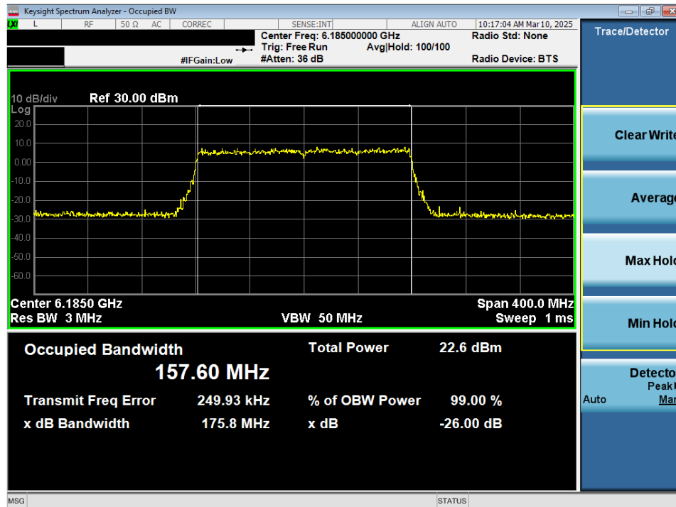
Plot 7-17. 26dB Bandwidth Plot MIMO ANT2 (160MHz 802.11ax/be (UNII Band 5) – Ch. 47) - LPI/SP
