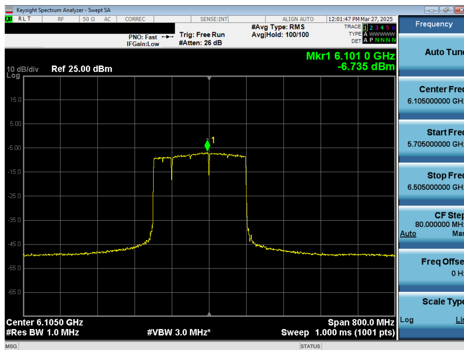
Plot 7-45. Power Spectral Density Plot MIMO ANT2 (320MHz 802.11be (UNII Band 5) – Ch. 31) – 120MHz Punctured – LPI/SP
