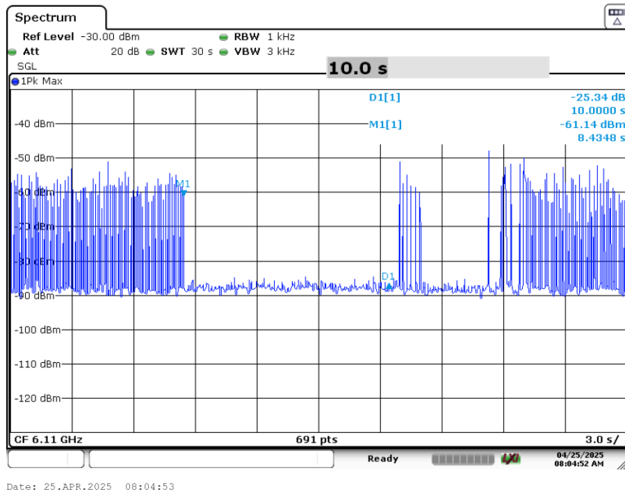
Plot 7-75. Contention Based Protocol Timing Plot (320MHz (UNII Band 5) – Ch. 31 Low)
