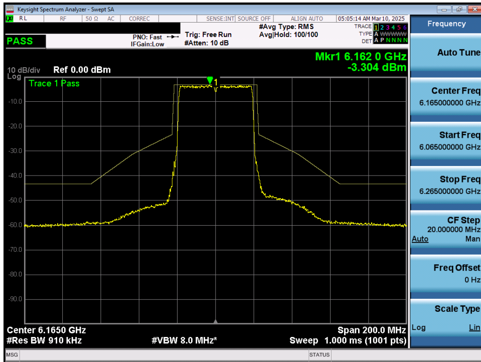
Plot 7-51. In Band Emissions Plot MIMO ANT1 (40MHz 802.11ax/be (UNII Band 5) – Ch. 43) - LPI
