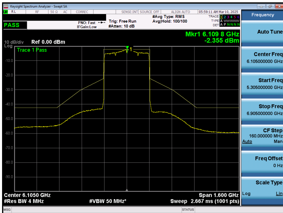
Plot 7-54. In Band Emissions Plot MIMO ANT1 (320MHz 802.11ax/be (UNII Band 5) – Ch. 31) - LPI/SP
