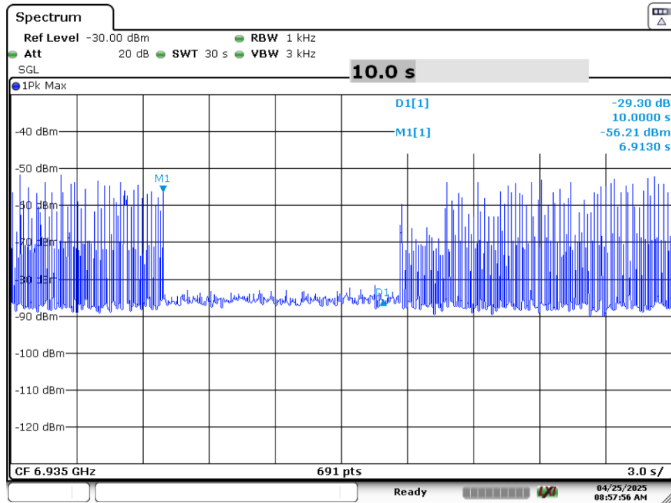
Plot 7-86. Contention Based Protocol Timing Plot (20MHz (UNII Band 8) – Ch. 197)
