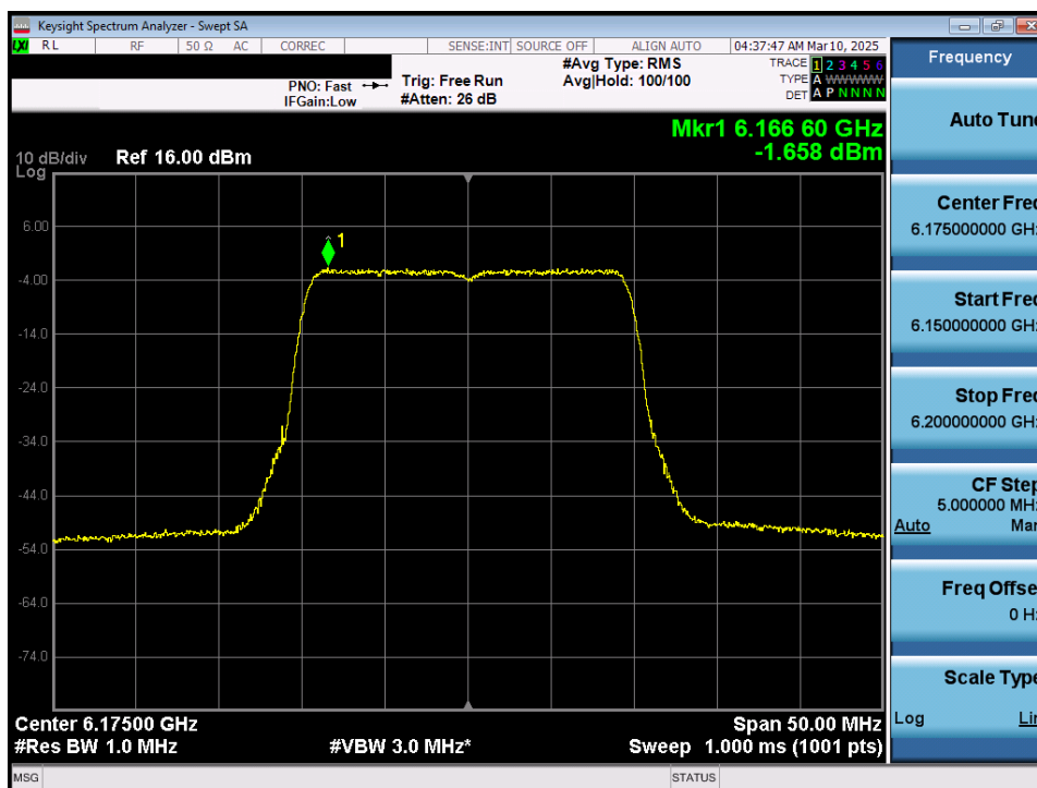
Plot 7-26. Power Spectral Density Plot MIMO ANT1 (20MHz 802.11ax/be (UNII Band 5) – Ch. 45) - LPI
