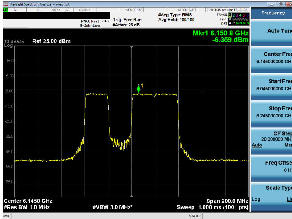
Plot 7-43. Power Spectral Density Plot MIMO ANT2 (80MHz 802.11be (UNII Band 5) – Ch. 39) – 20MHz Punctured - LPI/SP
