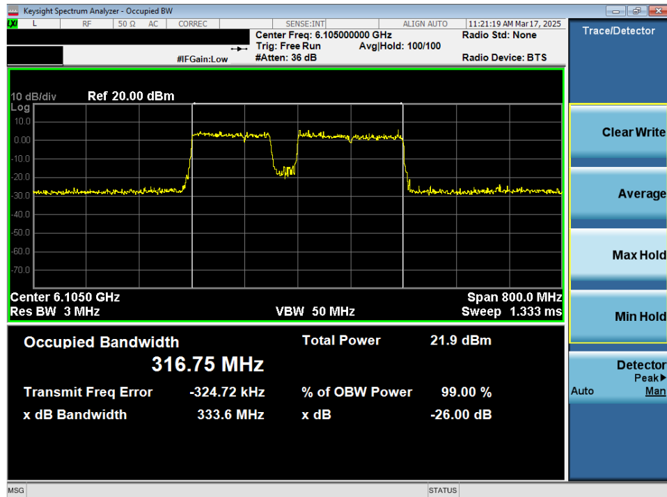
Plot 7-21. 26dB Bandwidth Plot MIMO ANT2 (320MHz 802.11be (UNII Band 5) – Ch. 31) – 40MHz Punctured – LPI/SP
