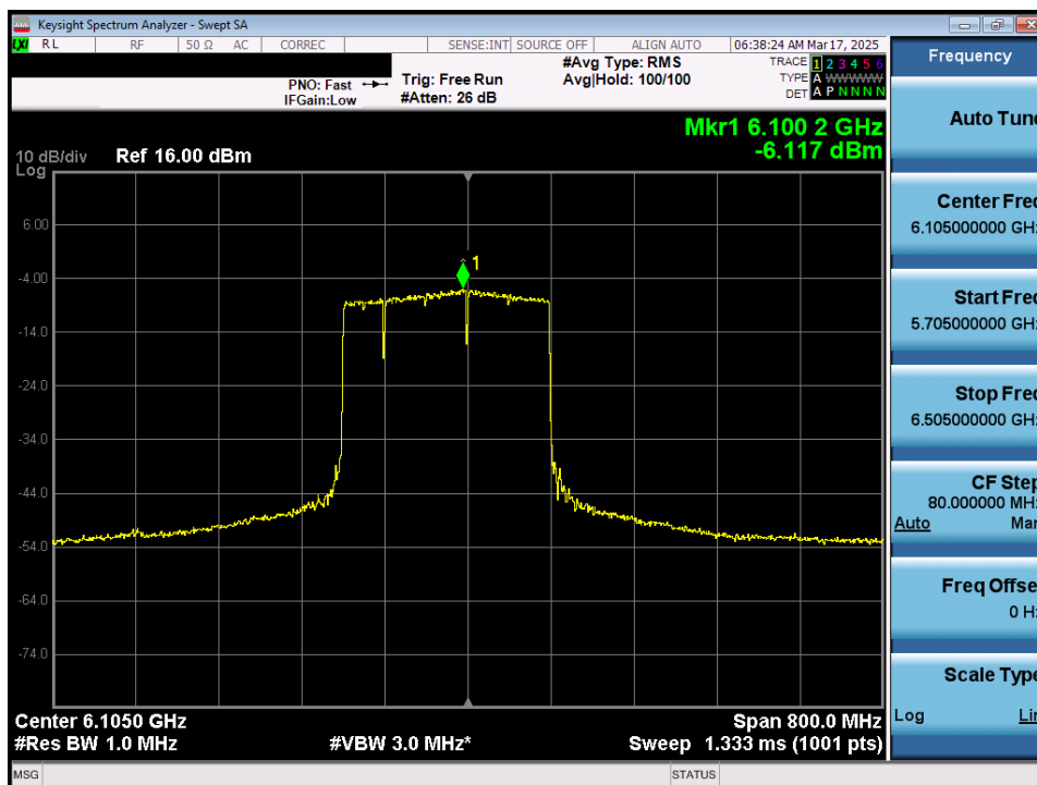
Plot 7-33. Power Spectral Density Plot MIMO ANT1 (320MHz 802.11be (UNII Band 5) – Ch. 31) – 120MHz Punctured – LPI/SP
