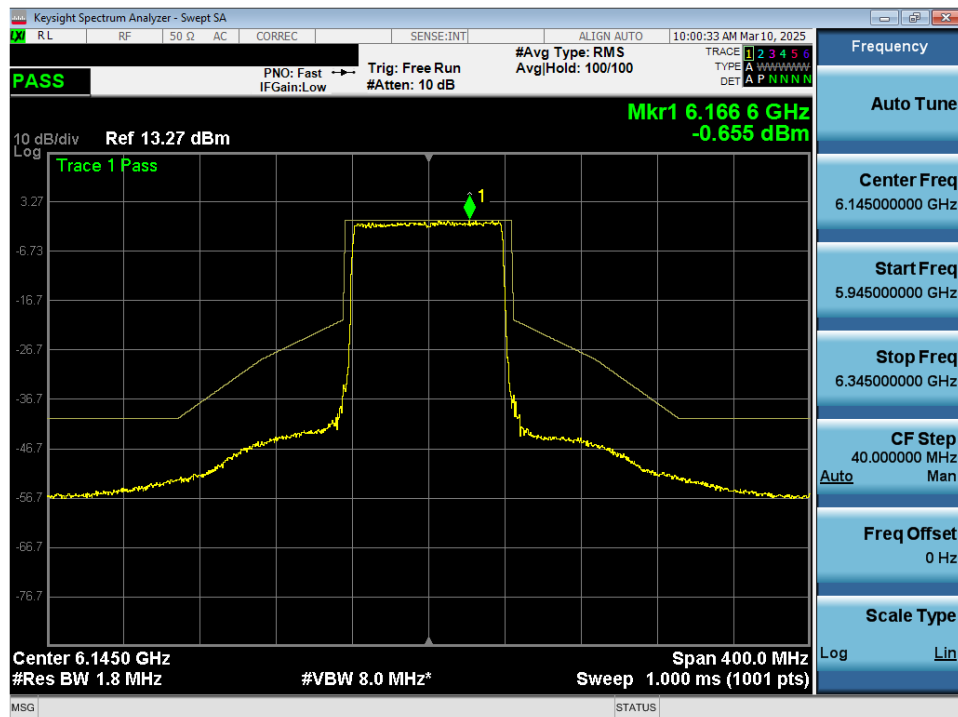
Plot 7-64. In Band Emissions Plot MIMO ANT2 (80MHz 802.11ax/be (UNII Band 5) – Ch. 39) - LPI/SP
