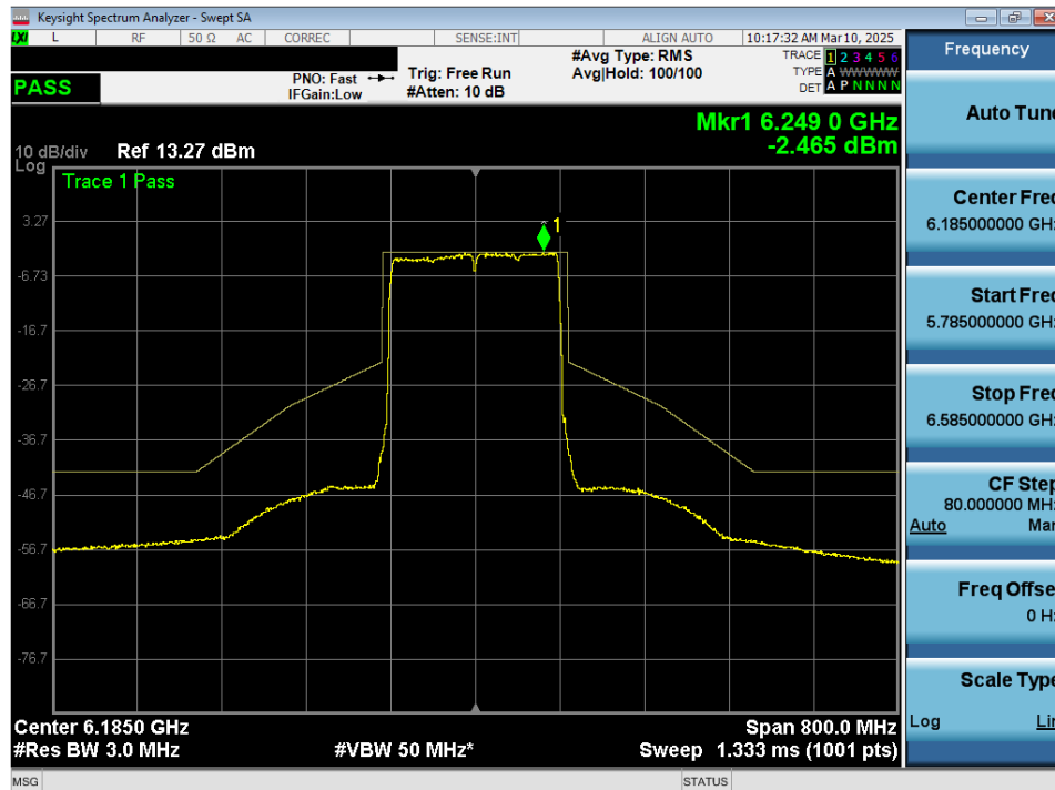
Plot 7-65. In Band Emissions Plot MIMO ANT2 (160MHz 802.11ax/be (UNII Band 5) – Ch. 47) - LPI/SP
