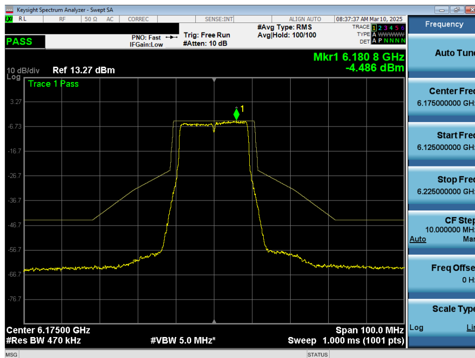
Plot 7-61. In Band Emissions Plot MIMO ANT2 (20MHz 802.11a (UNII Band 5) – Ch. 45) - LPI
