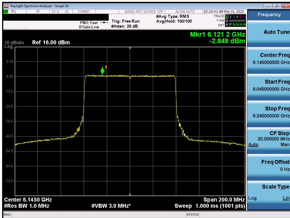
Plot 7-28. Power Spectral Density Plot MIMO ANT1 (80MHz 802.11ax/be (UNII Band 5) – Ch. 39) – LPI/SP
