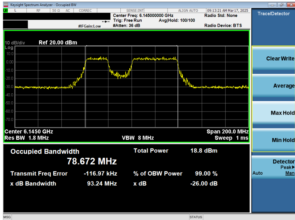
Plot 7-19. 26dB Bandwidth Plot MIMO ANT2 (80MHz 802.11be (UNII Band 5) – Ch. 39) – 20MHz Punctured - LPI/SP
