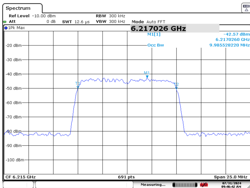
Plot 7-73. AWGN Signal (Demonstration)
