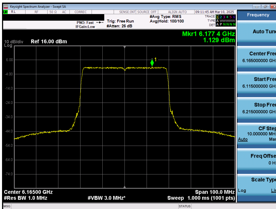
Plot 7-36. Power Spectral Density Plot MIMO ANT1 (40MHz 802.11ax/be (UNII Band 5) – Ch. 43) - SP
