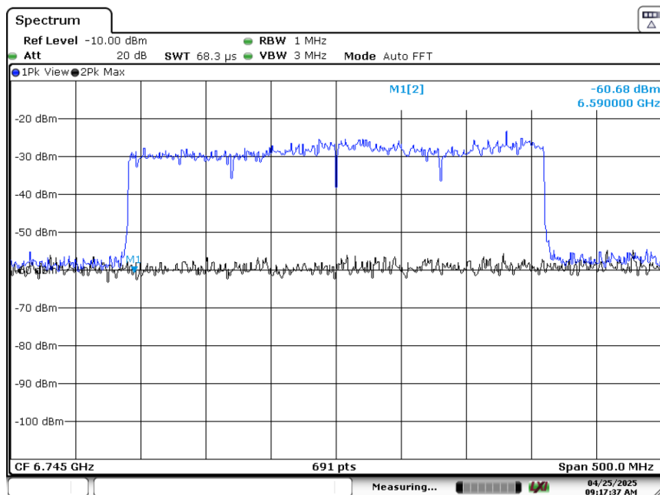
Plot 7-90. CBP 320MHz Channel - Injection Lower Edge – [6590 MHz]
