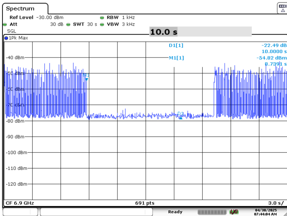
Plot 7-84. Contention Based Protocol Timing Plot (320MHz (UNII Band 7) – Ch. 159 Mid)
