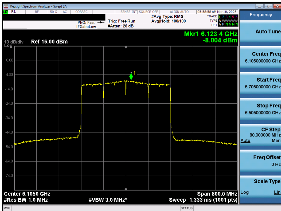
Plot 7-30. Power Spectral Density Plot MIMO ANT1 (320MHz 802.11ax/be (UNII Band 5) – Ch. 31) - LPI/SP
