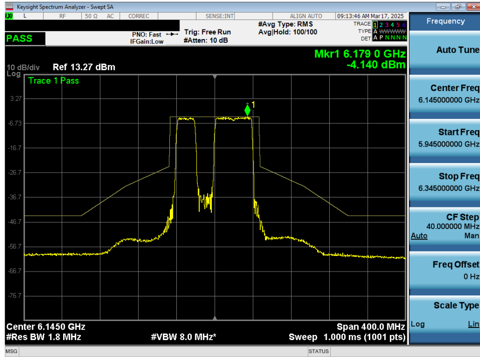
Plot 7-67. In Band Emissions Plot MIMO ANT2 (80MHz 802.11be (UNII Band 5) – Ch. 39) – 20MHz Punctured - LPI/SP
