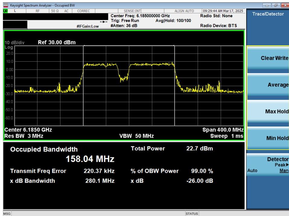
Plot 7-20. 26dB Bandwidth Plot MIMO ANT2 (160MHz 802.11be (UNII Band 5) – Ch. 47) – 20MHz Punctured - LPI/SP
