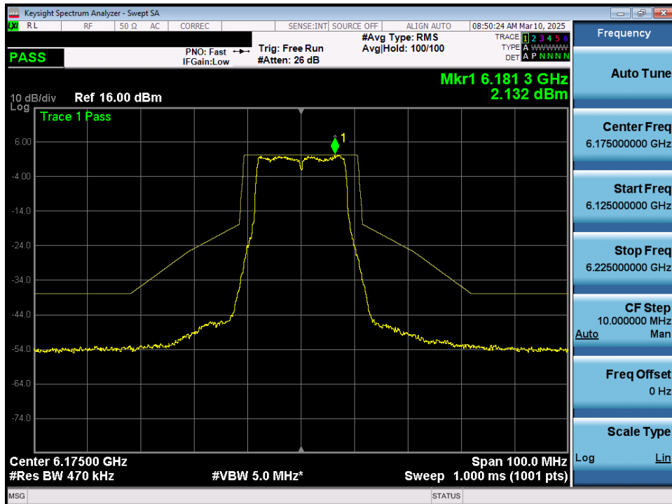
Plot 7-58. In Band Emissions Plot MIMO ANT1 (20MHz 802.11a (UNII Band 5) – Ch. 45) - SP
