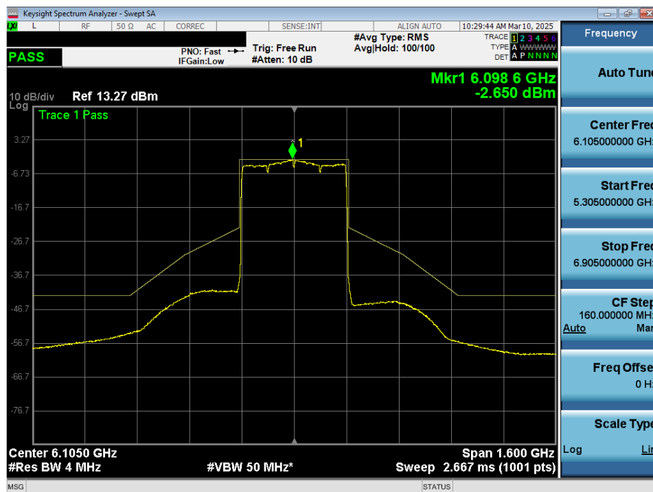
Plot 7-66. In Band Emissions Plot MIMO ANT2 (320MHz 802.11ax/be (UNII Band 5) – Ch. 31) - LPI/SP
