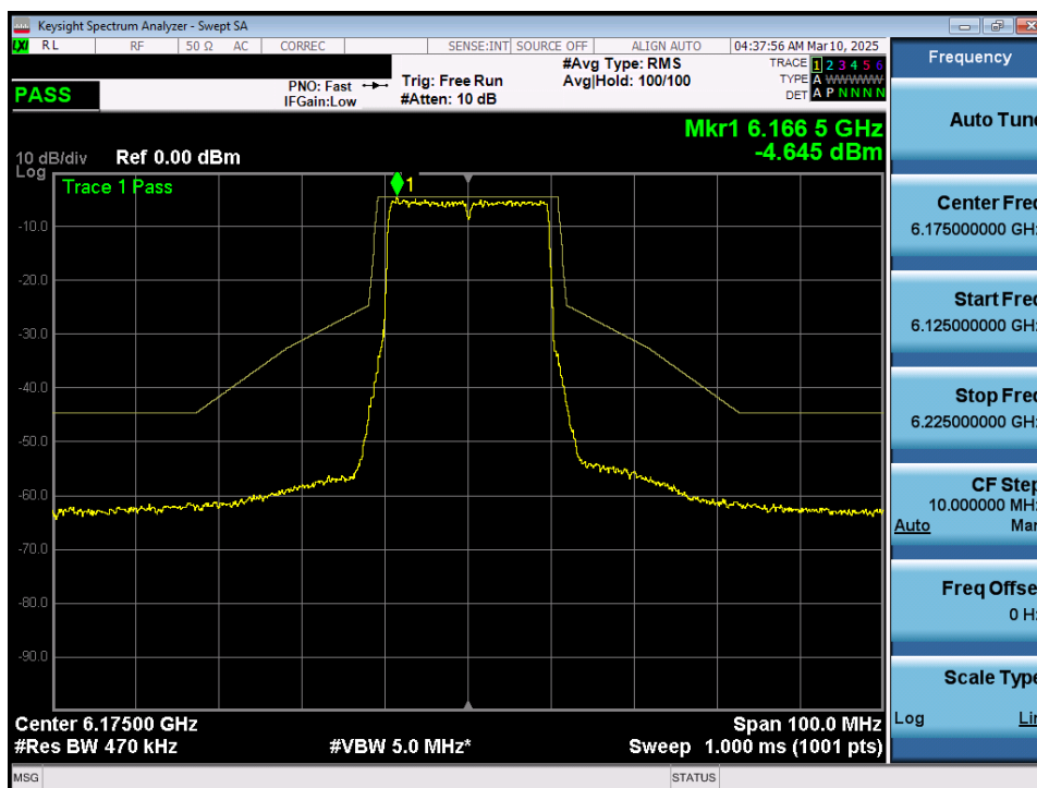
Plot 7-50. In Band Emissions Plot MIMO ANT1 (20MHz 802.11ax/be (UNII Band 5) – Ch. 45) - LPI
