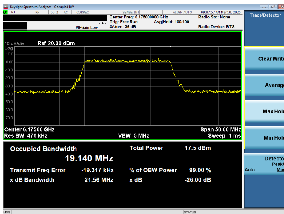
Plot 7-14. 26dB Bandwidth Plot MIMO ANT2 (20MHz 802.11ax/be (UNII Band 5) – Ch. 45) - LPI
