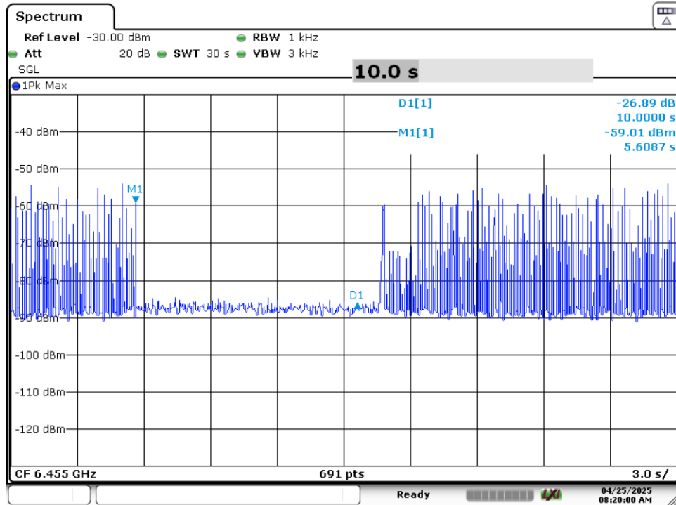
Plot 7-78. Contention Based Protocol Timing Plot (20MHz (UNII Band 6) – Ch. 101)
