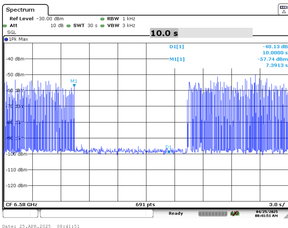
Plot 7-81. Contention Based Protocol Timing Plot (320MHz (UNII Band 6) – Ch. 95 High)
