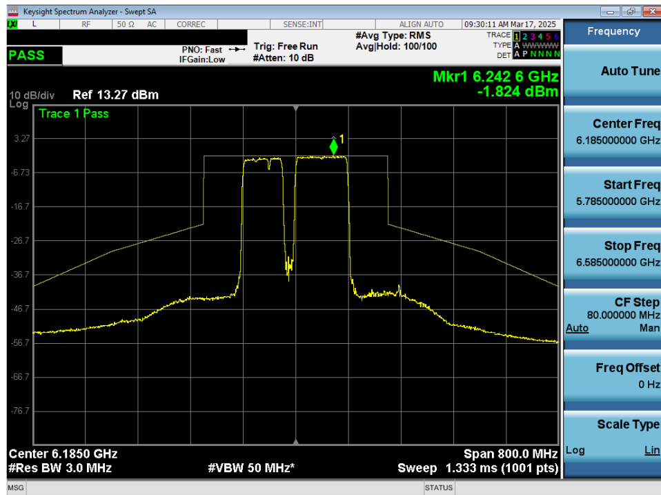
Plot 7-68. In Band Emissions Plot MIMO ANT2 (160MHz 802.11be (UNII Band 5) – Ch. 47) – 20MHz Punctured - LPI/SP
