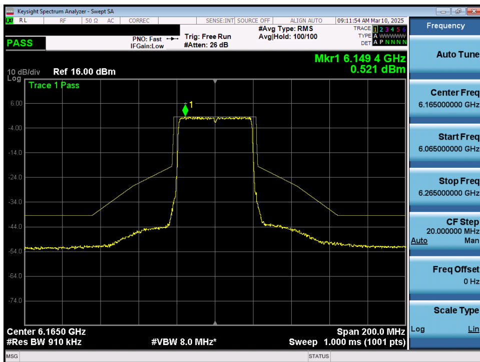
Plot 7-60. In Band Emissions Plot MIMO ANT1 (40MHz 802.11ax/be (UNII Band 5) – Ch. 43) - SP
