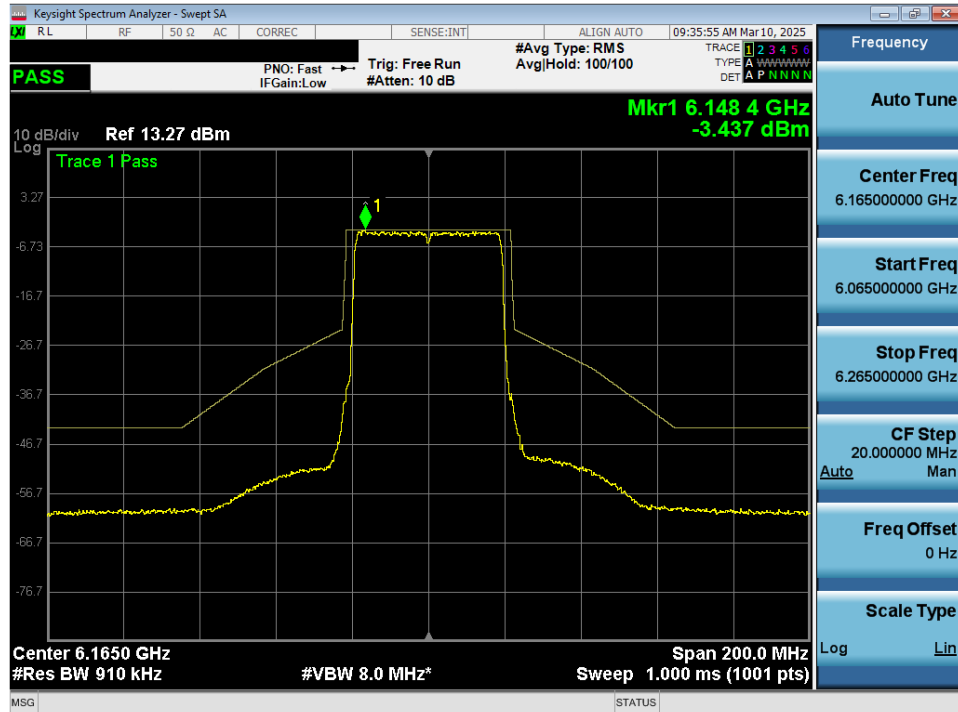
Plot 7-63. In Band Emissions Plot MIMO ANT2 (40MHz 802.11ax/be (UNII Band 5) – Ch. 43) - LPI
