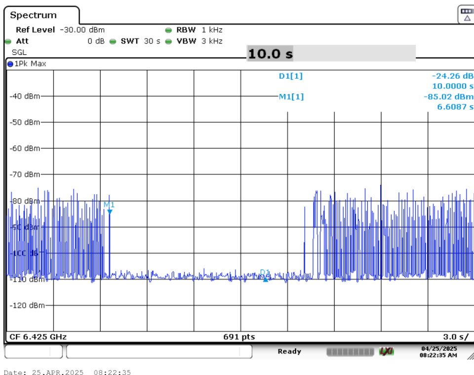
Plot 7-80. Contention Based Protocol Timing Plot (320MHz (UNII Band 6) – Ch. 95 Mid)
