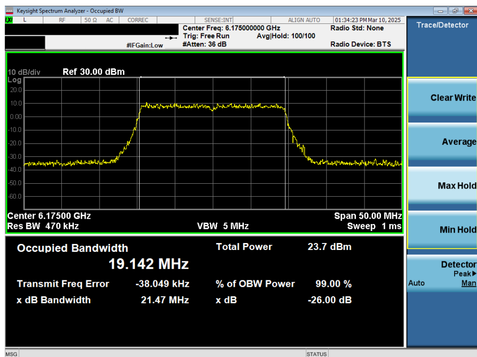
Plot 7-23. 26dB Bandwidth Plot MIMO ANT2 (20MHz 802.11ax/be (UNII Band 5) – Ch. 45) - SP
