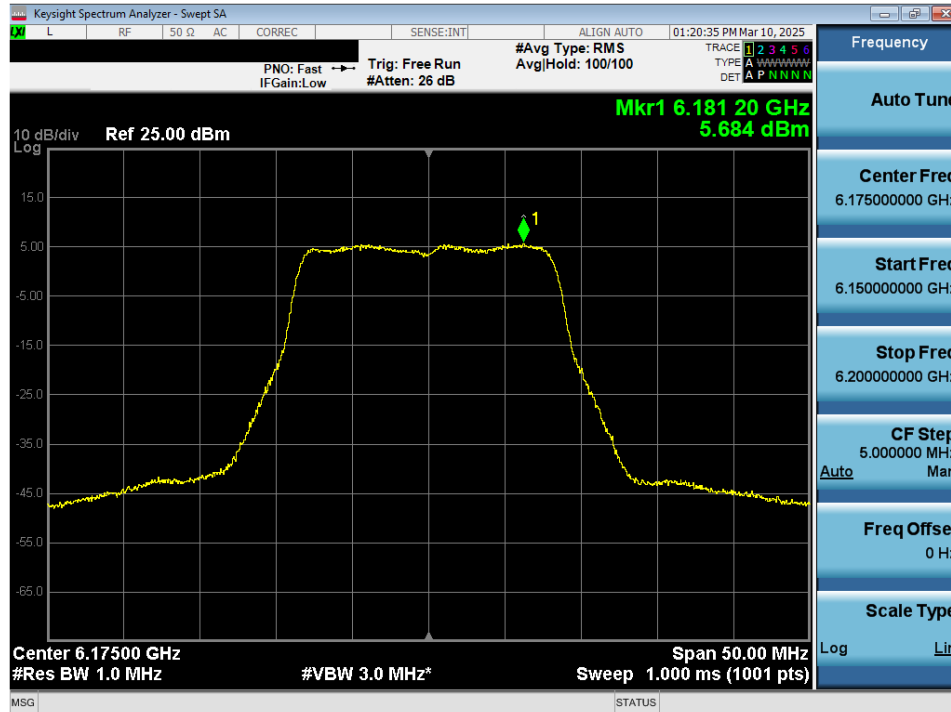
Plot 7-46. Power Spectral Density Plot MIMO ANT2 (20MHz 802.11a (UNII Band 5) – Ch. 45) - SP
