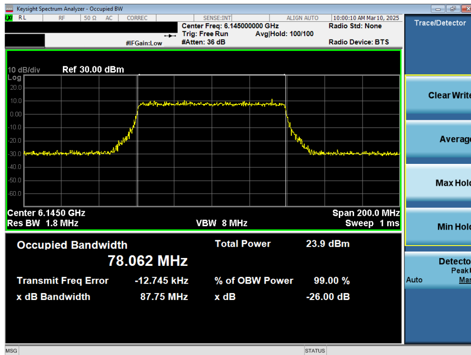
Plot 7-16. 26dB Bandwidth Plot MIMO ANT2 (80MHz 802.11ax/be (UNII Band 5) – Ch. 39) - LPI/SP
