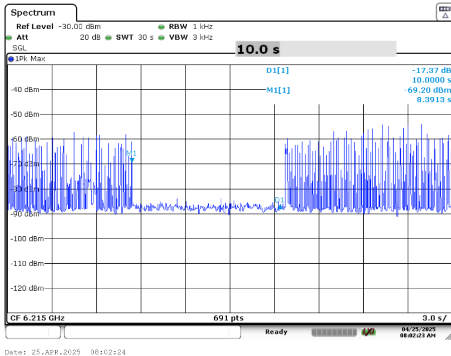
Plot 7-74. Contention Based Protocol Timing Plot (20MHz (UNII Band 5) – Ch. 53)
