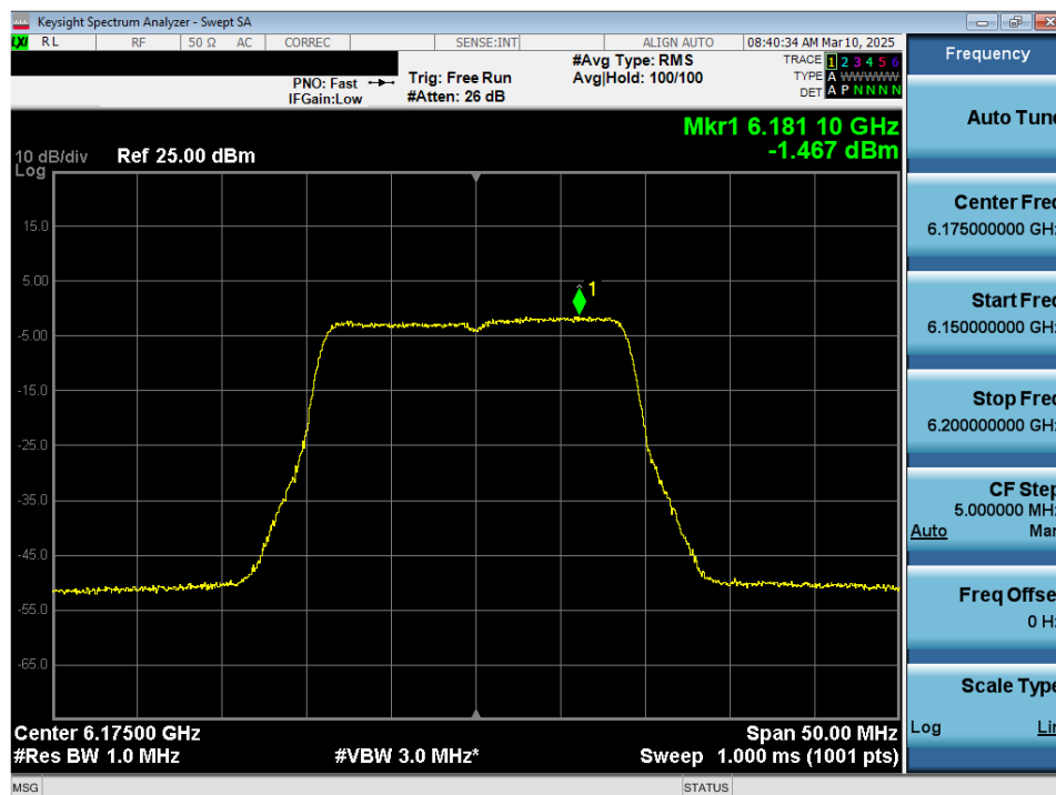
Plot 7-37. Power Spectral Density Plot MIMO ANT2 (20MHz 802.11a (UNII Band 5) – Ch. 45) - LPI
