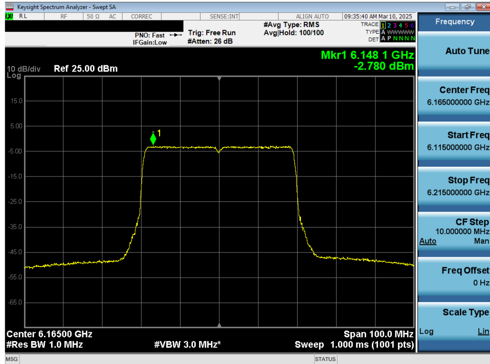
Plot 7-39. Power Spectral Density Plot MIMO ANT2 (40MHz 802.11ax/be (UNII Band 5) – Ch. 43) - LPI
