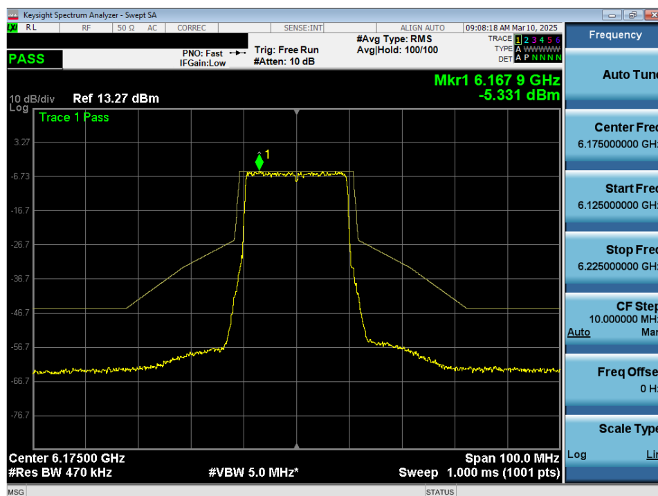
Plot 7-62. In Band Emissions Plot MIMO ANT2 (20MHz 802.11ax/be (UNII Band 5) – Ch. 45) - LPI
