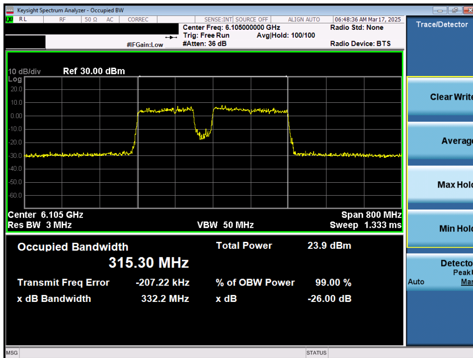
Plot 7-9. 26dB Bandwidth Plot MIMO ANT1 (320MHz 802.11be (UNII Band 5) – Ch. 31) – 40MHz Punctured – LPI/SP
