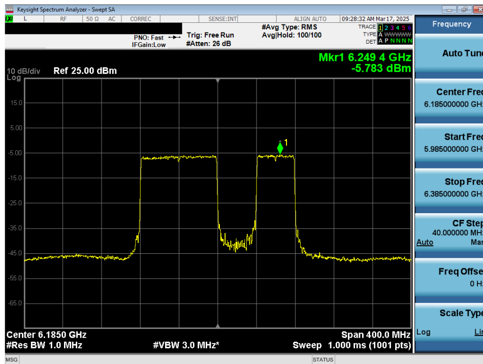
Plot 7-44. Power Spectral Density Plot MIMO ANT2 (160MHz 802.11be (UNII Band 5) – Ch. 47) – 40MHz Punctured - LPI/SP
