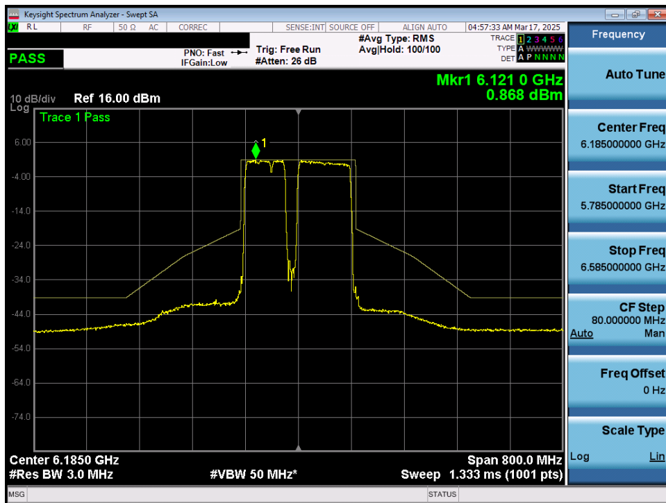
Plot 7-56. In Band Emissions Plot MIMO ANT1 (160MHz 802.11be (UNII Band 5) – Ch. 47) – 20MHz Punctured - LPI/SP
