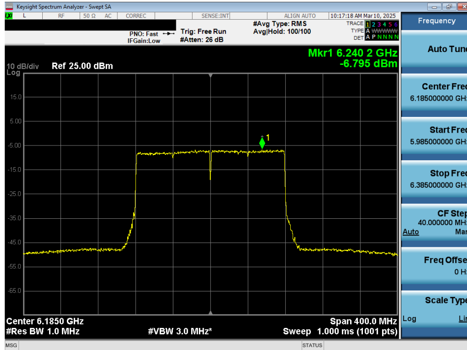
Plot 7-41. Power Spectral Density Plot MIMO ANT2 (160MHz 802.11ax/be (UNII Band 5) – Ch. 47) - LPI/SP
