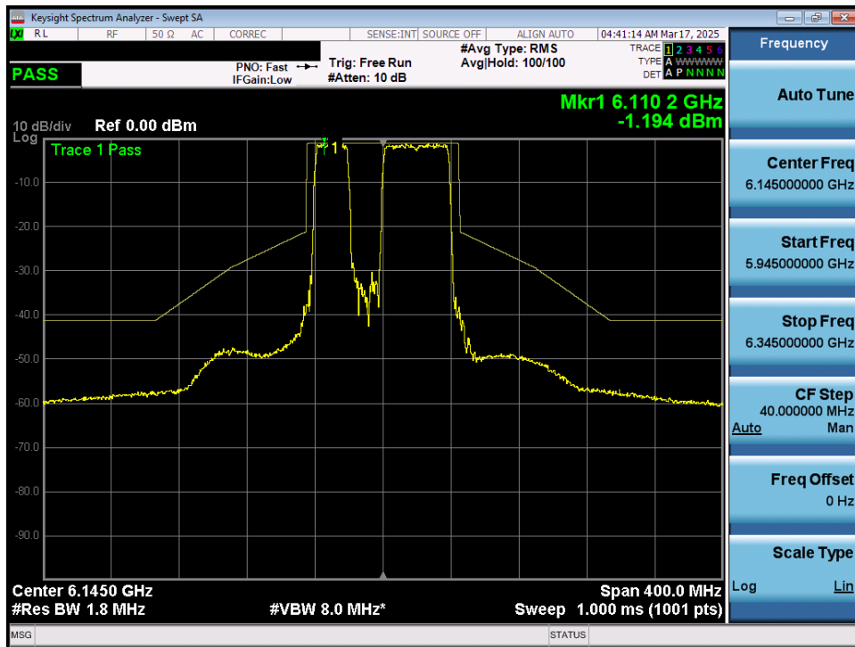
Plot 7-55. In Band Emissions Plot MIMO ANT1 (80MHz 802.11be (UNII Band 5) – Ch. 39) – 20MHz Punctured - LPI/SP
