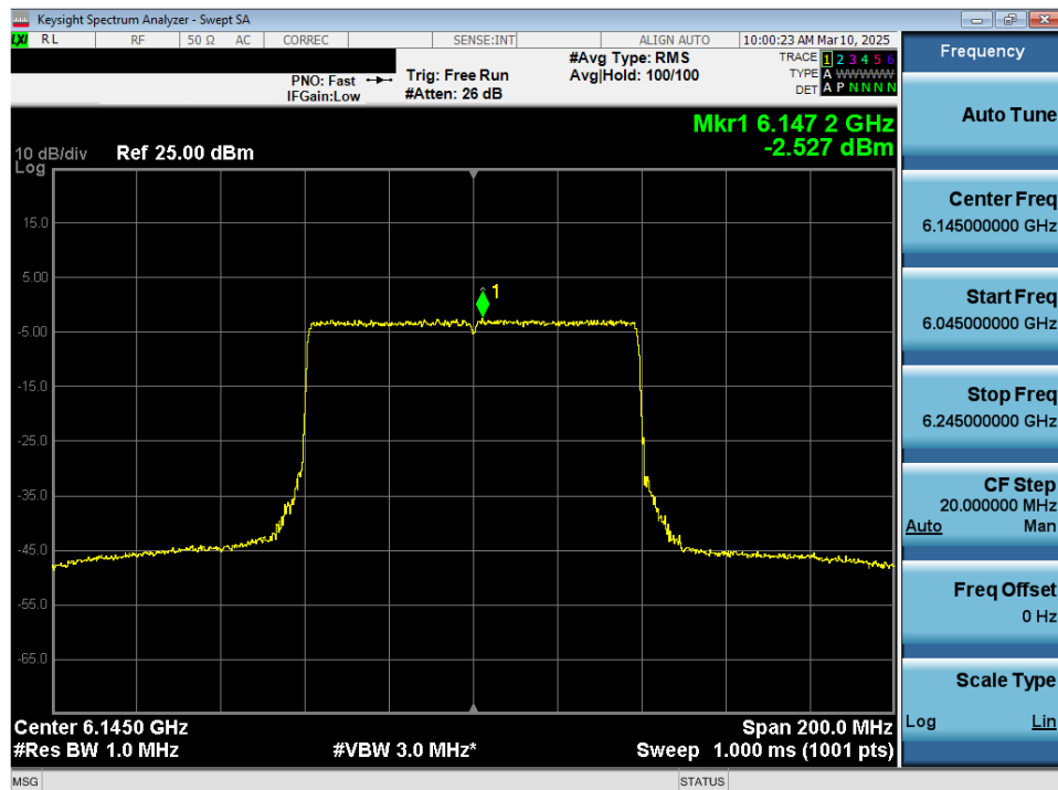
Plot 7-40. Power Spectral Density Plot MIMO ANT2 (80MHz 802.11ax/be (UNII Band 5) – Ch. 39) - LPI/SP
