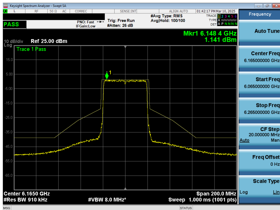
Plot 7-72. In Band Emissions Plot MIMO ANT2 (40MHz 802.11ax/be (UNII Band 5) – Ch. 43) - SP
