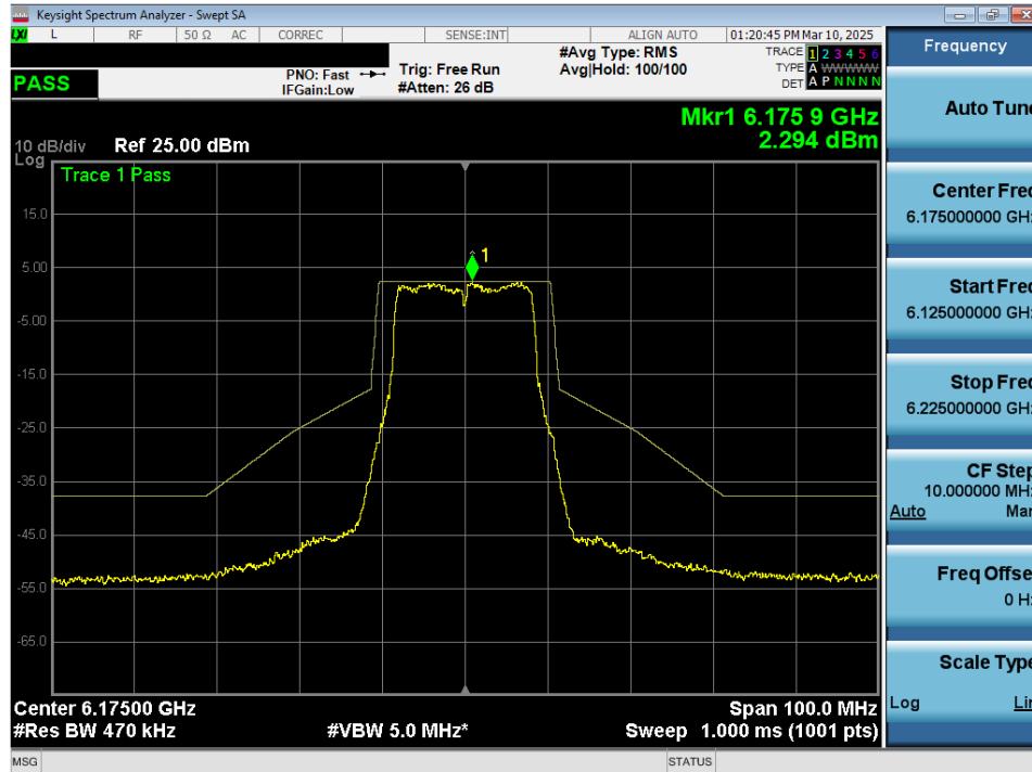
Plot 7-70. In Band Emissions Plot MIMO ANT2 (20MHz 802.11a (UNII Band 5) – Ch. 45) - SP
