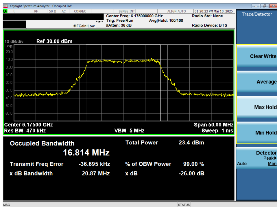
Plot 7-22. 26dB Bandwidth Plot MIMO ANT2 (20MHz 802.11a (UNII Band 5) – Ch. 45) - SP
