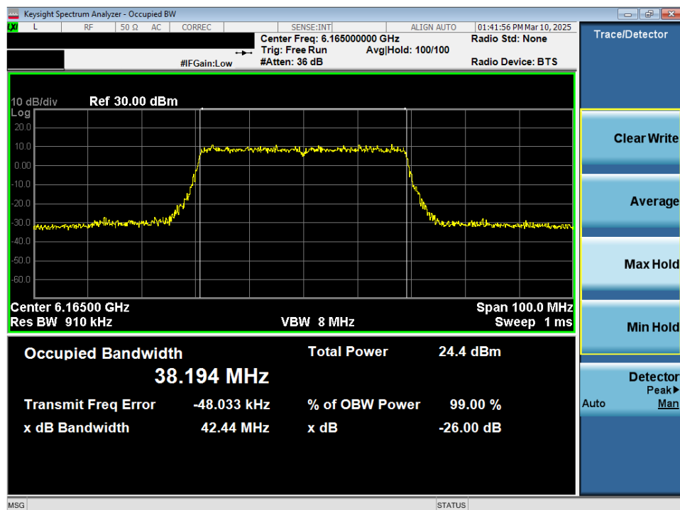
Plot 7-24. 26dB Bandwidth Plot MIMO ANT2 (40MHz 802.11ax/be (UNII Band 5) – Ch. 43) - SP
