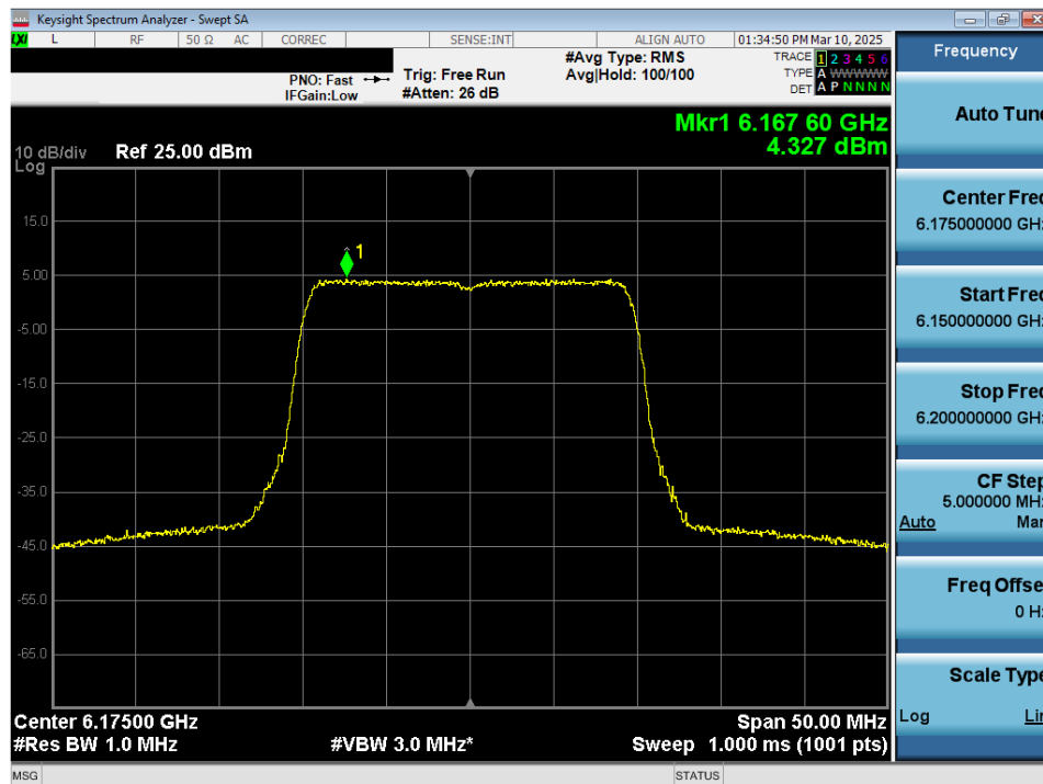
Plot 7-47. Power Spectral Density Plot MIMO ANT2 (20MHz 802.11ax/be (UNII Band 5) – Ch. 45) - SP
