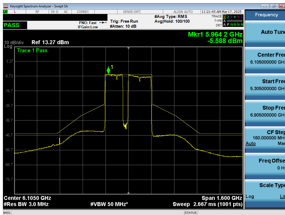
Plot 7-69. In Band Emissions Plot MIMO ANT2 (320MHz 802.11be (UNII Band 5) – Ch. 31) – 40MHz Punctured – LPI/SP
