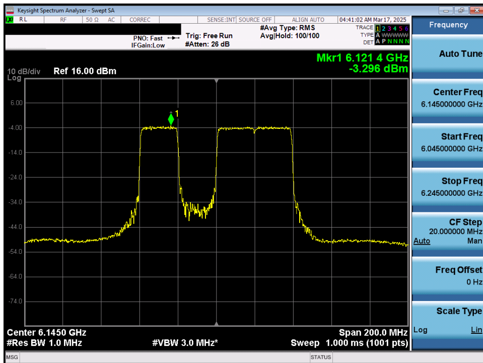
Plot 7-31. Power Spectral Density Plot MIMO ANT1 (80MHz 802.11be (UNII Band 5) – Ch. 39) – 20MHz Punctured - LPI/SP
