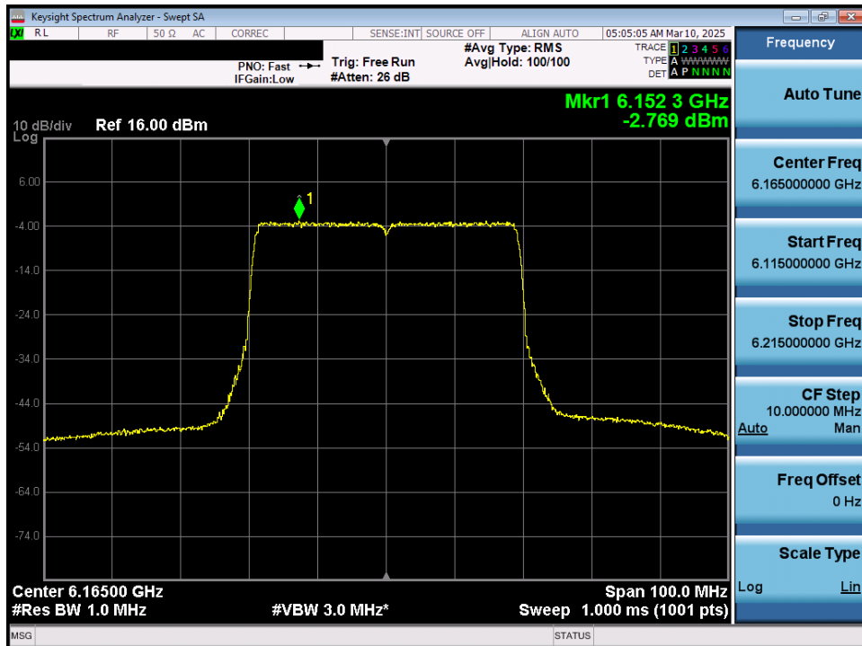
Plot 7-27. Power Spectral Density Plot MIMO ANT1 (40MHz 802.11ax/be (UNII Band 5) – Ch. 43) – LPI
