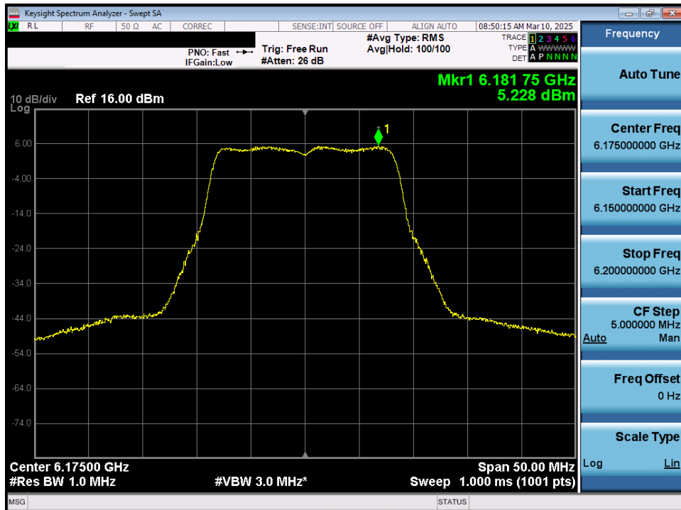
Plot 7-34. Power Spectral Density Plot MIMO ANT1 (20MHz 802.11a (UNII Band 5) – Ch. 45) - SP
