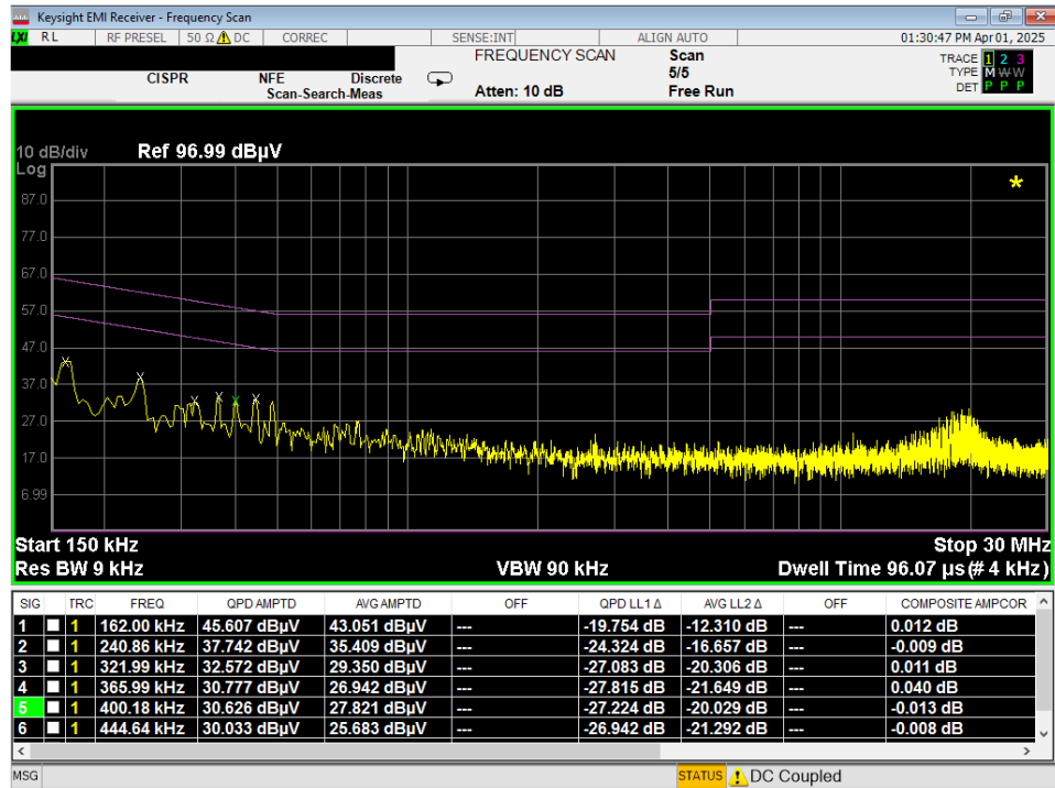
Plot 7-96. Line Conducted Plot with 802.11a UNII Band 7 (L1)
