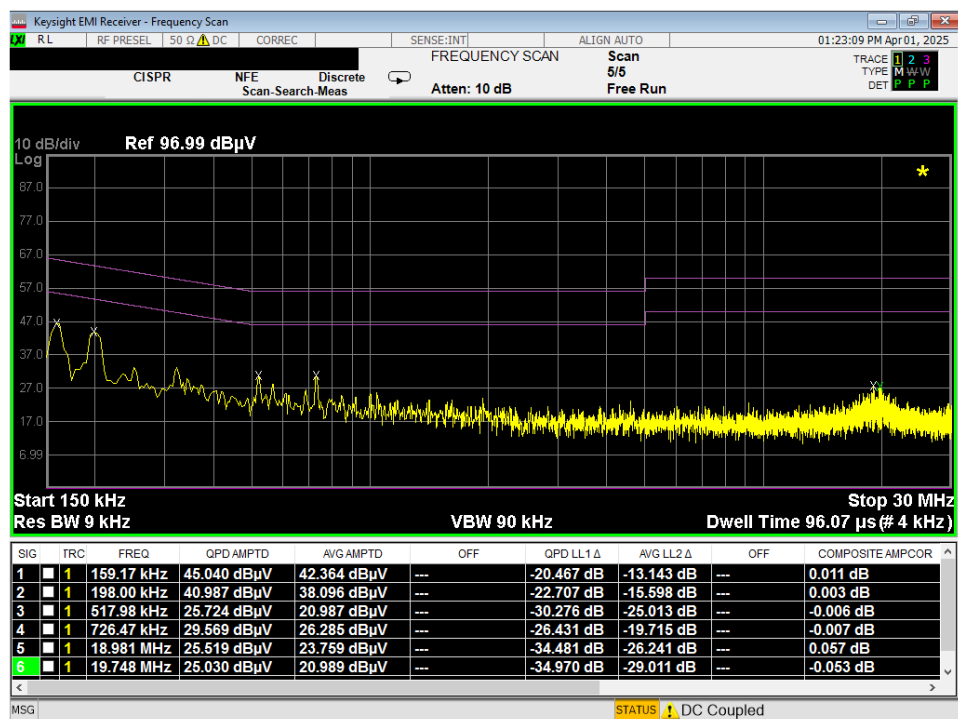
Plot 7-95. Line Conducted Plot with 802.11a UNII Band 5 (N)
