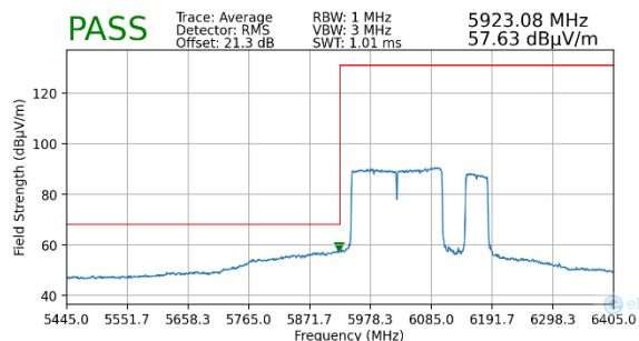
Plot 7-92. Radiated Lower Band Edge Plot MIMO (Average – UNII Band 5)
