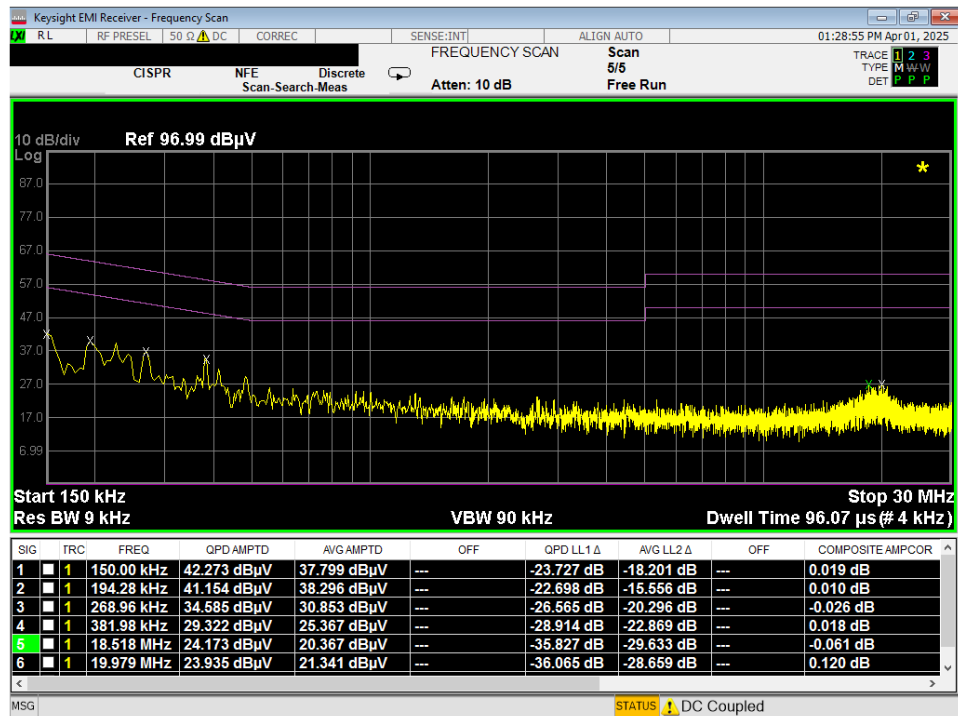
Plot 7-97. Line Conducted Plot with 802.11a UNII Band 7 (N)
