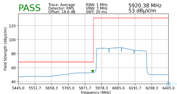
Plot 7-90. Radiated Lower Band Edge Plot MIMO (Average – UNII Band 5)
