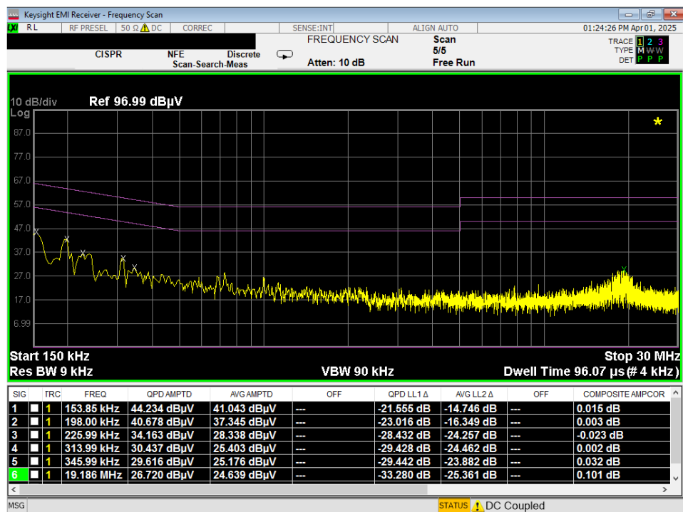
Plot 7-94. Line Conducted Plot with 802.11a UNII Band 5 (L1)
