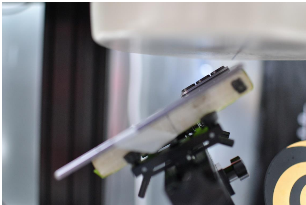
SAR Test Setup Photo 11 – Tablet, Folder Open, Back Side at 10mm (for AG1)
