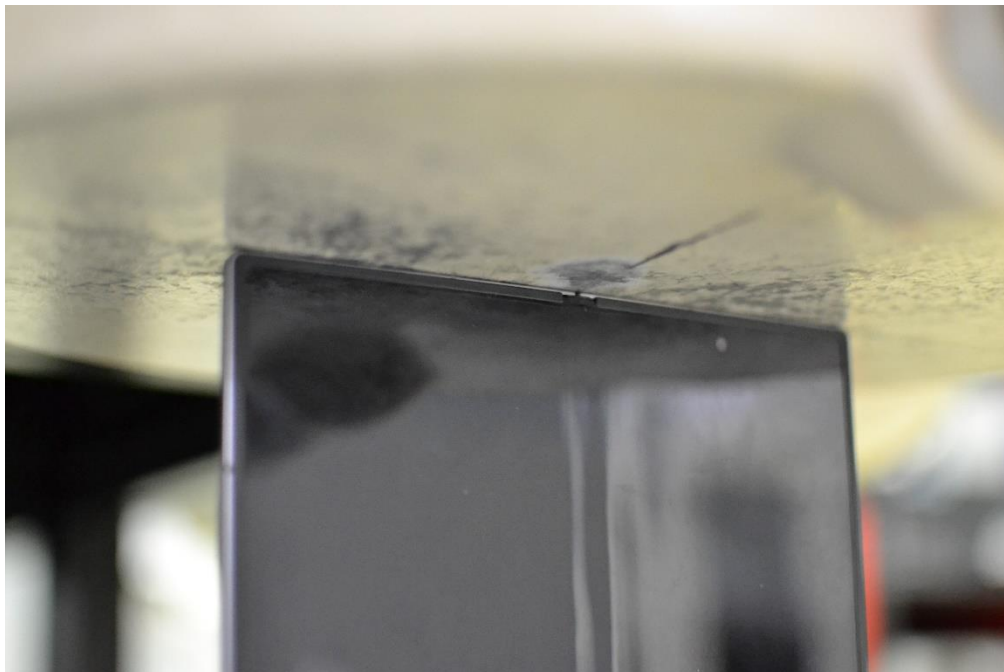
SAR Test Setup Photo 15 – Tablet, Folder Open, Top Edge at 0mm
