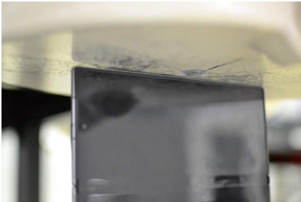
SAR Test Setup Photo 17 – Tablet, Folder Open, Right Edge at 0mm
