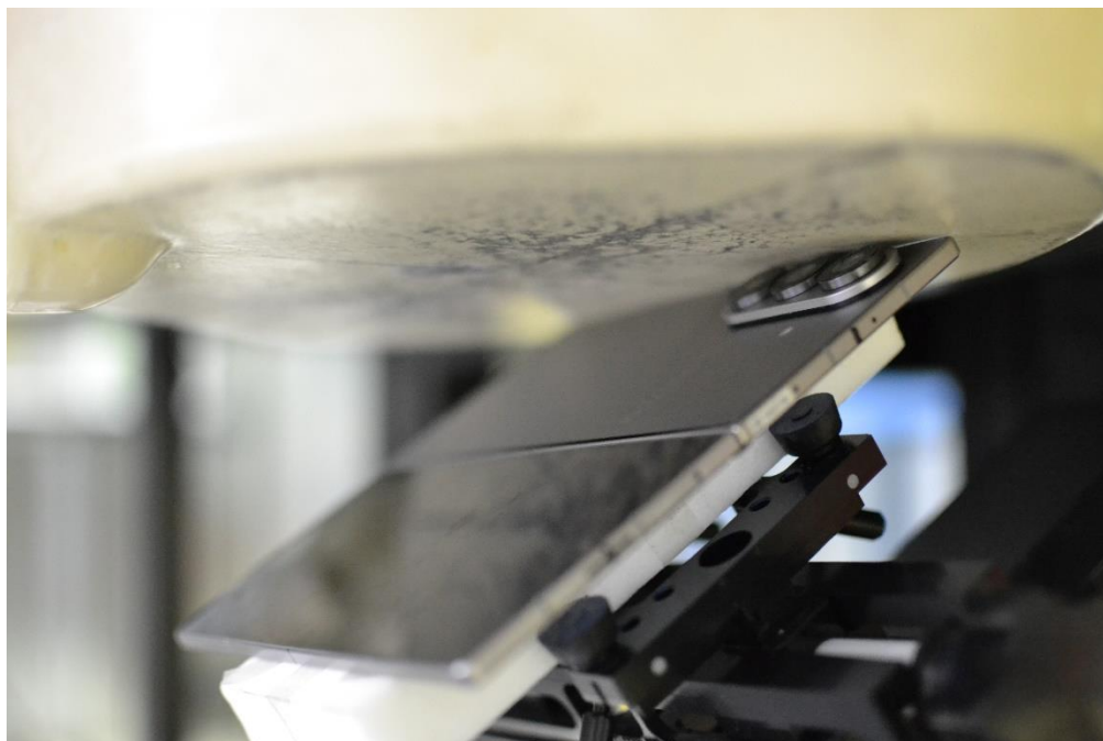
SAR Test Setup Photo 13 – Tablet, Folder Open, Back Side at 0mm (for Antenna H)
