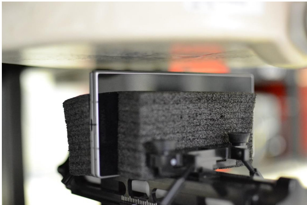
SAR Test Setup Photo 10 – Hotspot, Folder Closed, Left Edge at 10mm
