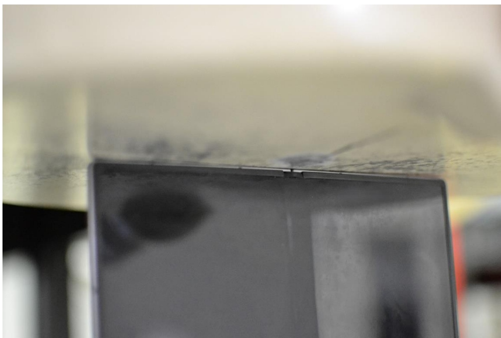
SAR Test Setup Photo 16 – Tablet, Folder Open, Bottom Edge at 0mm
