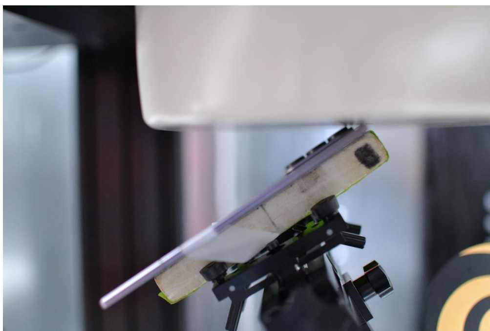
SAR Test Setup Photo 12 – Tablet, Folder Open, Back Side at 0mm (for AG1)
