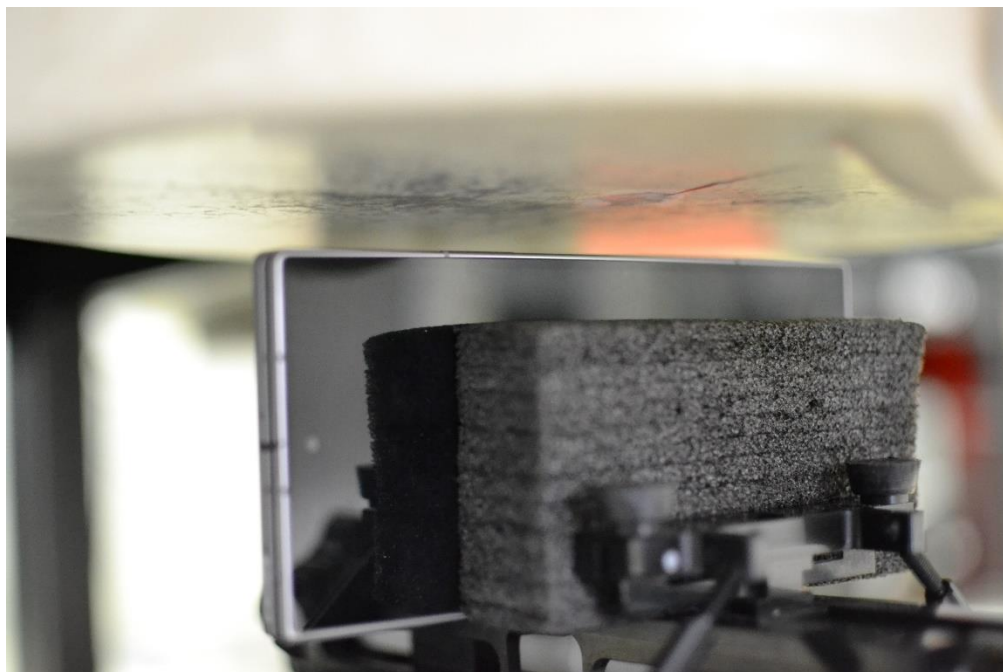
SAR Test Setup Photo 9 – Hotspot, Folder Closed, Right Edge at 10mm
