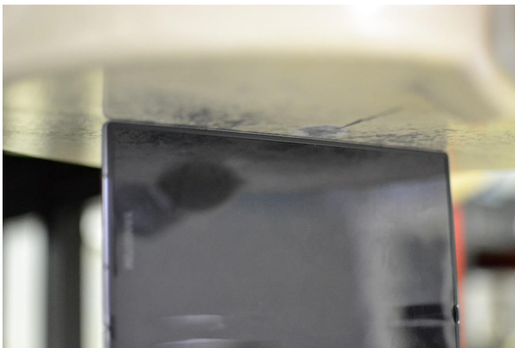
SAR Test Setup Photo 18 – Tablet, Folder Open, Left Edge at 0mm
