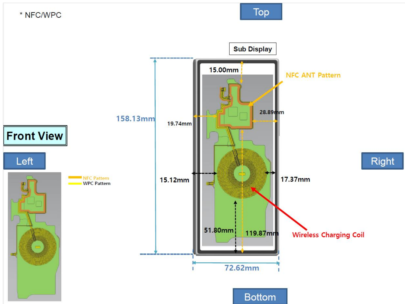
Figure G-3 NFC Antenna Locations – Folder Closed
