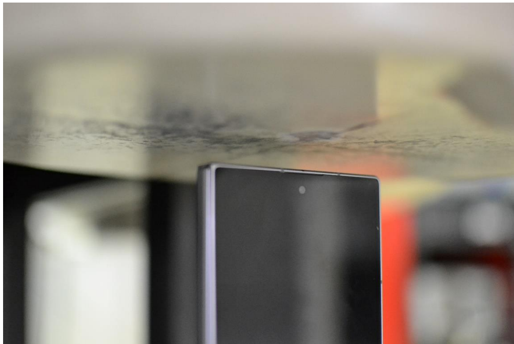
SAR Test Setup Photo 8 – Hotspot, Folder Closed, Top Edge at 10mm
