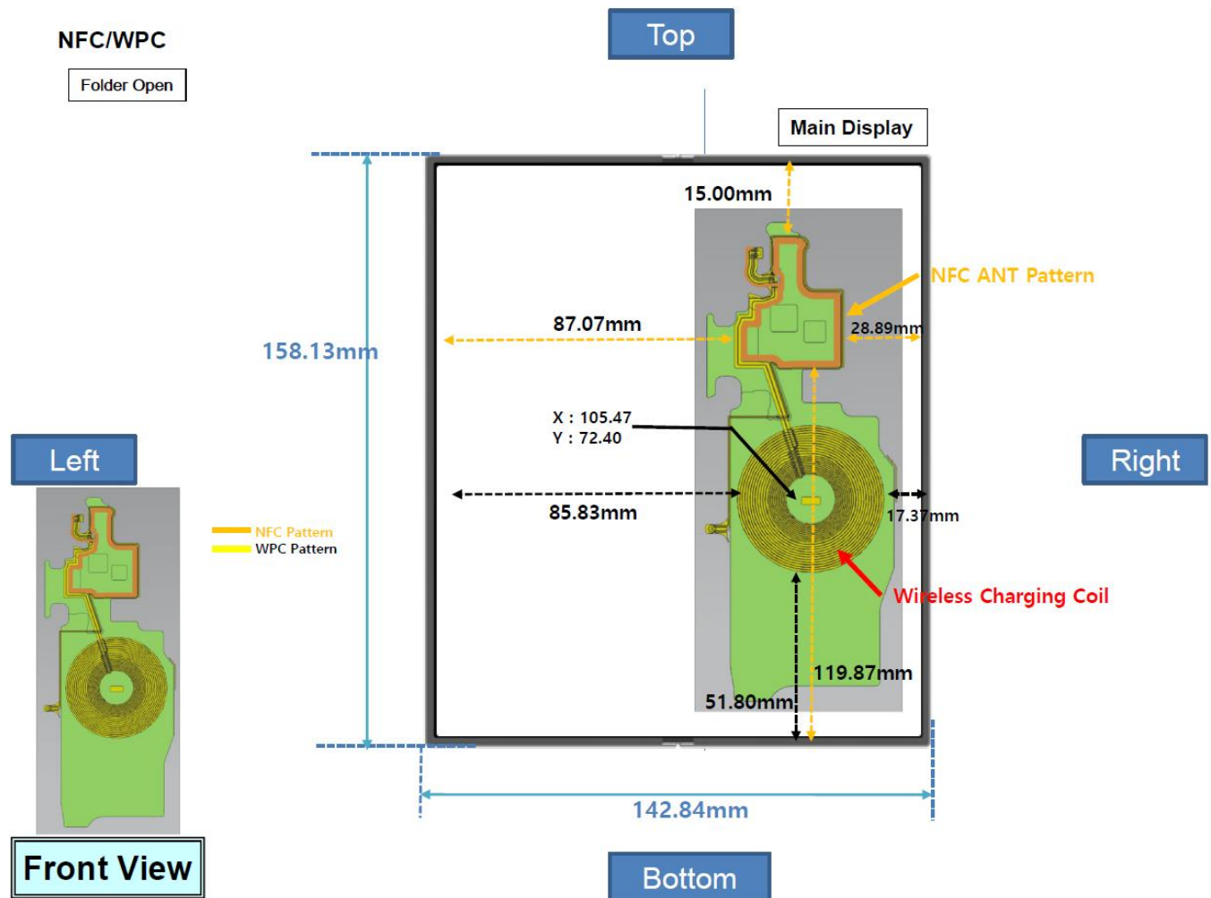
Figure G-4 NFC Antenna Locations – Folder Open
