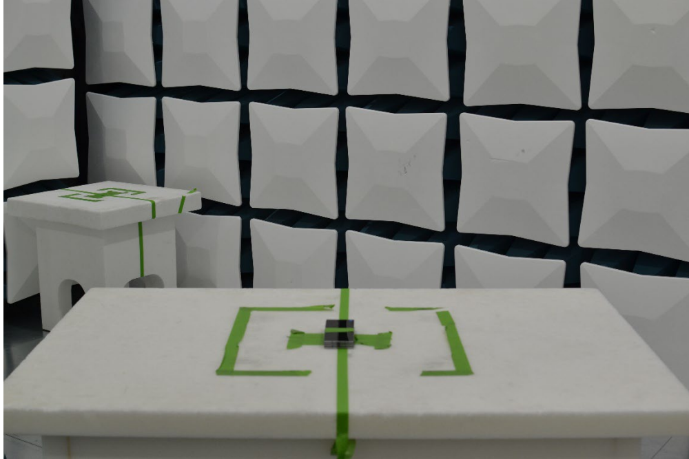
Figure 27. Test Setup – X – WPT – 30MHz-18GHz
