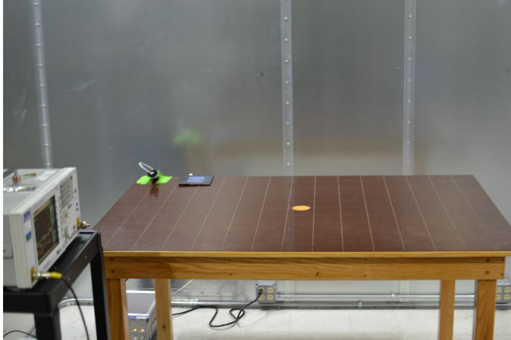
Figure 31. Test Setup – ACLC– <30MHz
