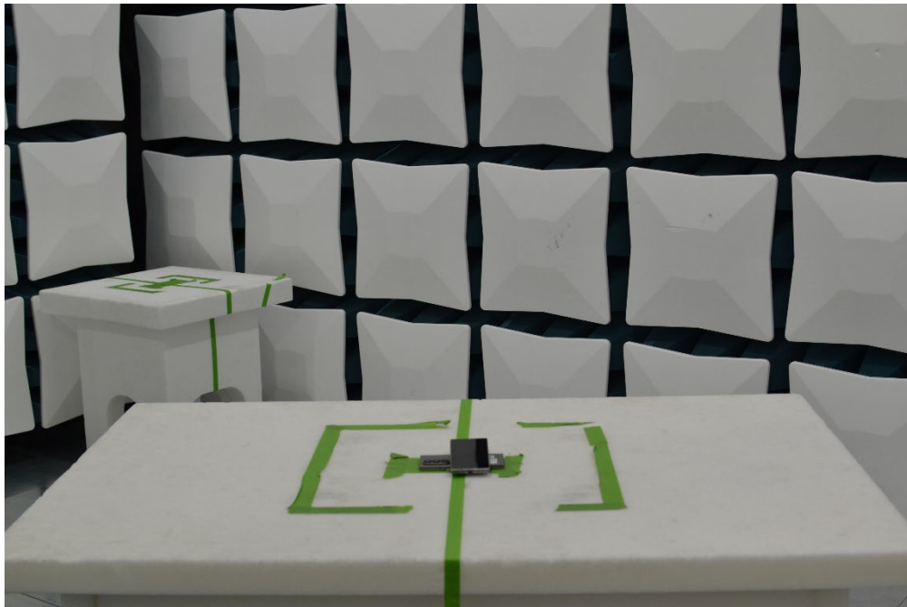
Figure 30. Test Setup – WPT – 30MHz-18GHz
