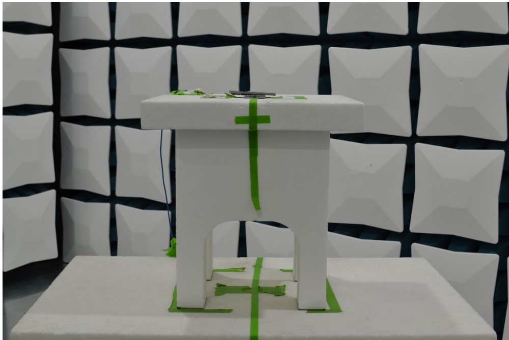
Figure 14. Test Setup – WPT
