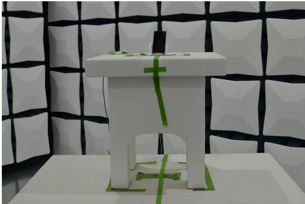
Figure 12. Test Setup – WCP – Closed
