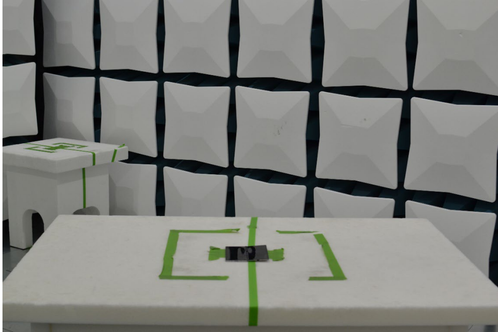
Figure 15. Test Setup – X Position – 30MHz-18GHz – Open
