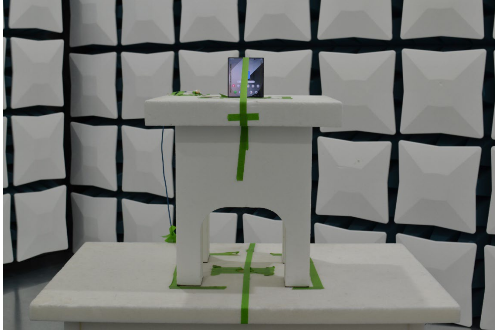
Figure 7. Test Setup – Z Position – 1GHz-40GHz – Open
