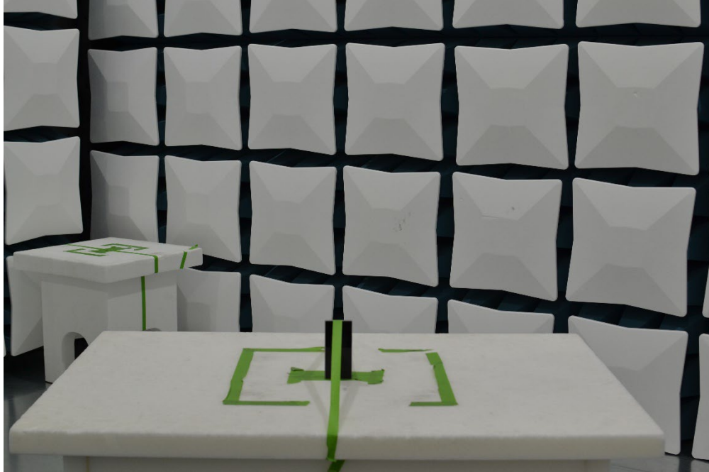
Figure 23. Test Setup – Z Position – 30MHz-18GHz – Closed
