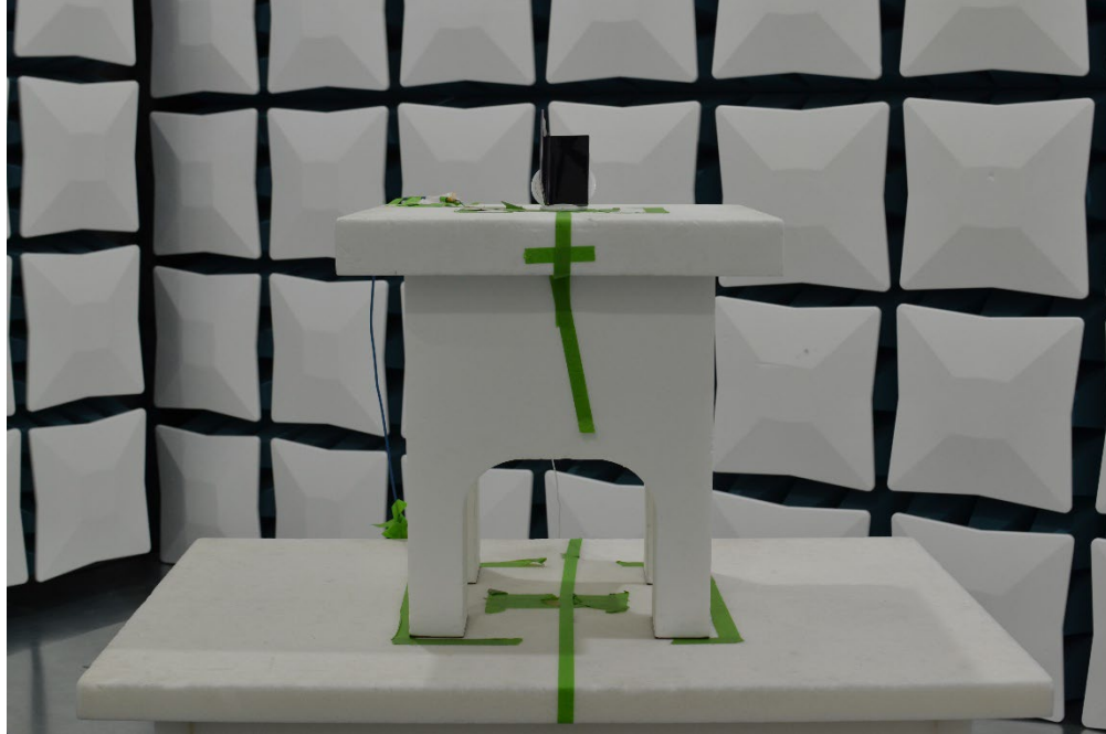
Figure 11. Test Setup – WCP – Half Open
