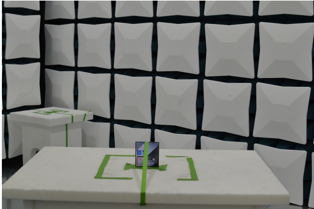
Figure 21. Test Setup – Z Position – 30MHz-18GHz – Open
