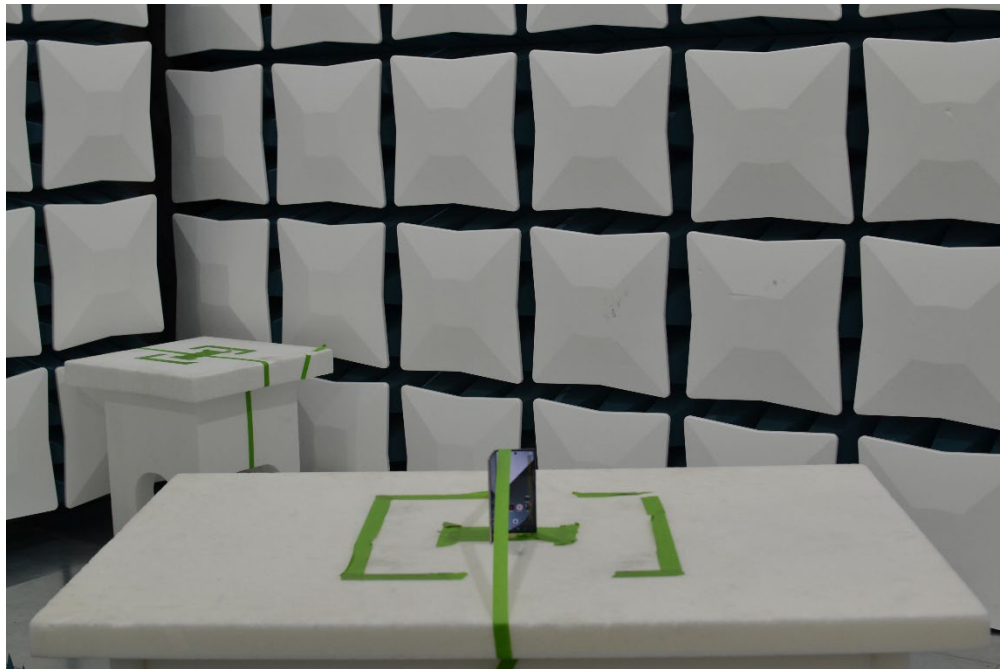
Figure 22. Test Setup – Z Position – 30MHz-18GHz – Half-Open
