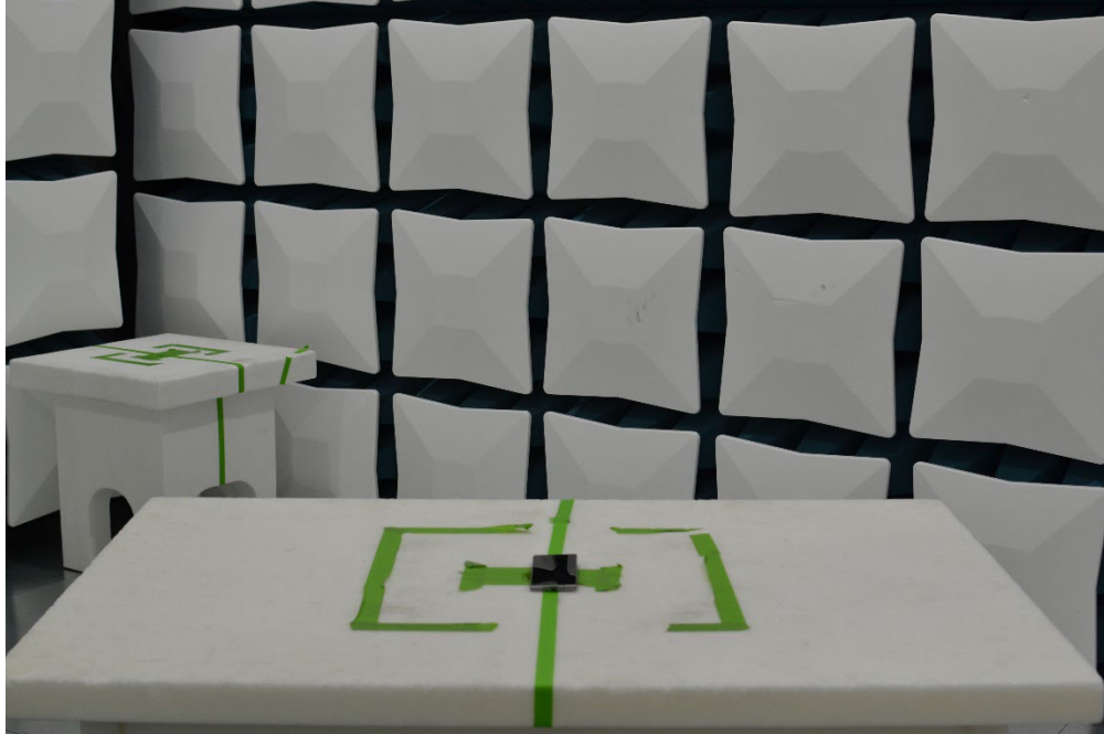
Figure 17. Test Setup – X Position – 30MHz-18GHz – Closed
