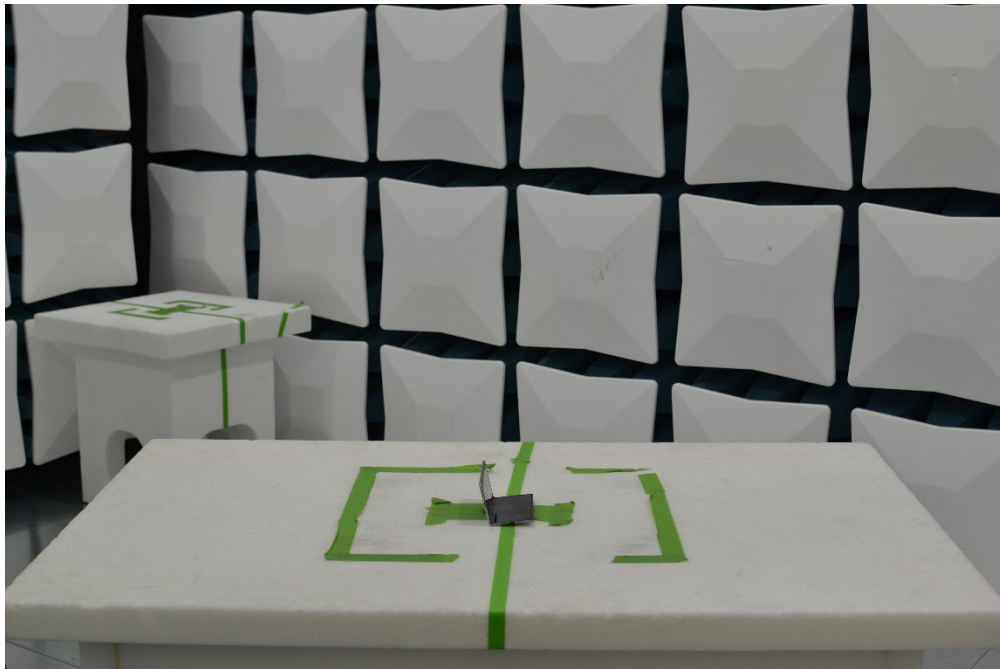
Figure 16. Test Setup – X Position – 30MHz-18GHz – Half Open
