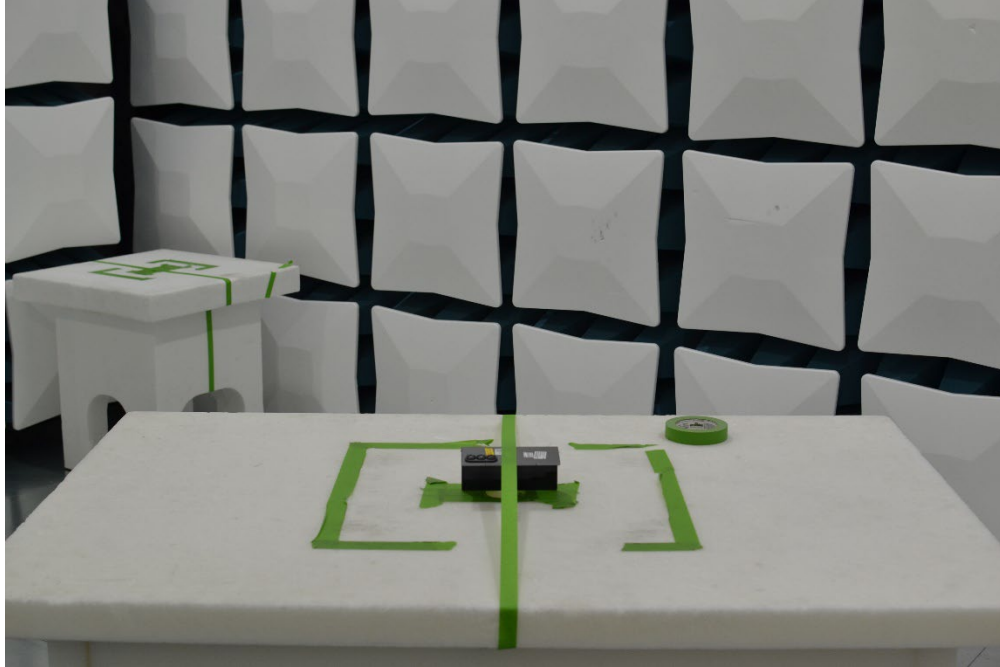
Figure 19. Test Setup – Y Position – 30MHz-18GHz – Half Open
