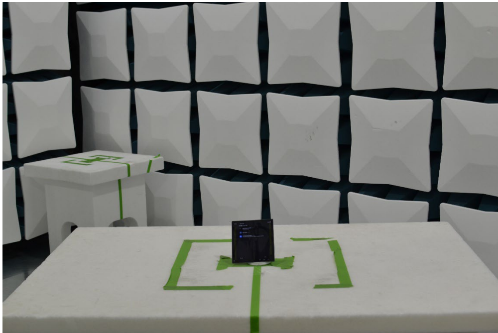
Figure 24. Test Setup – WCP – 30MHz-18GHz – Open
