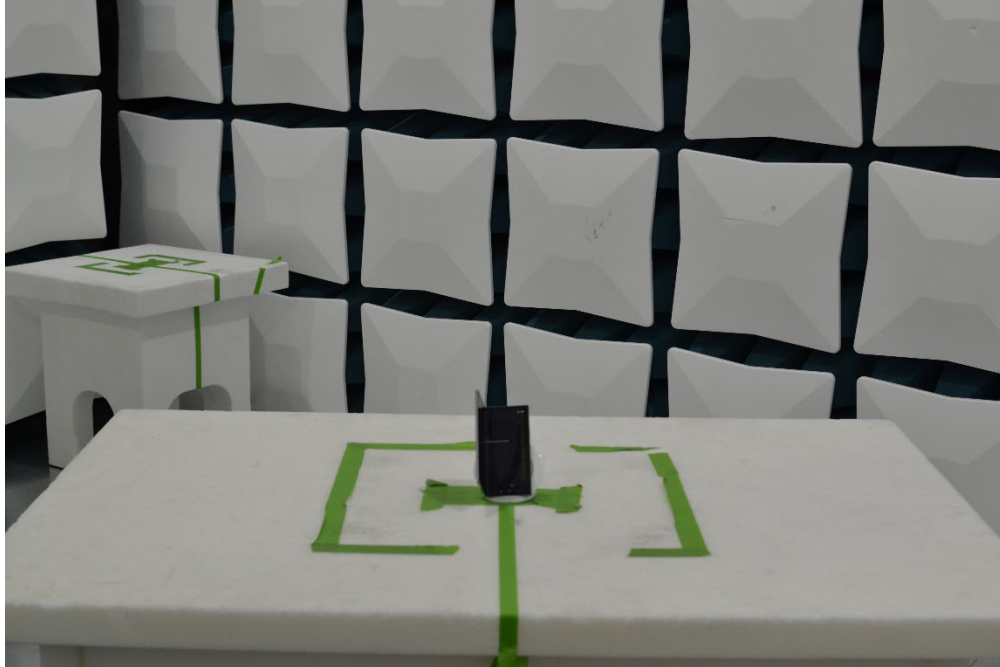
Figure 25. Test Setup – WCP – 30MHz-18GHz – Half Open
