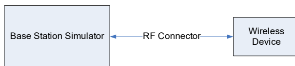
Figure 10-1 Power Measurement Setup – NR FDD
