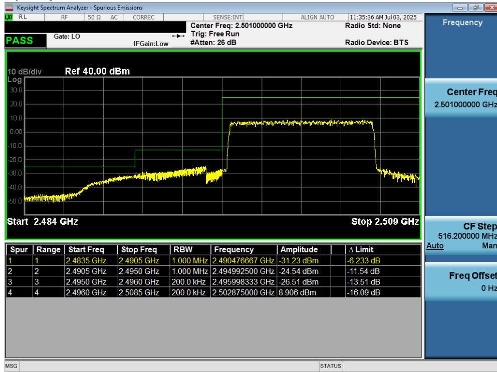
Plot 6-5. Lower ACP Plot (LTE Band 41(PC3) - 10MHz QPSK – Full RB – Ant2)
