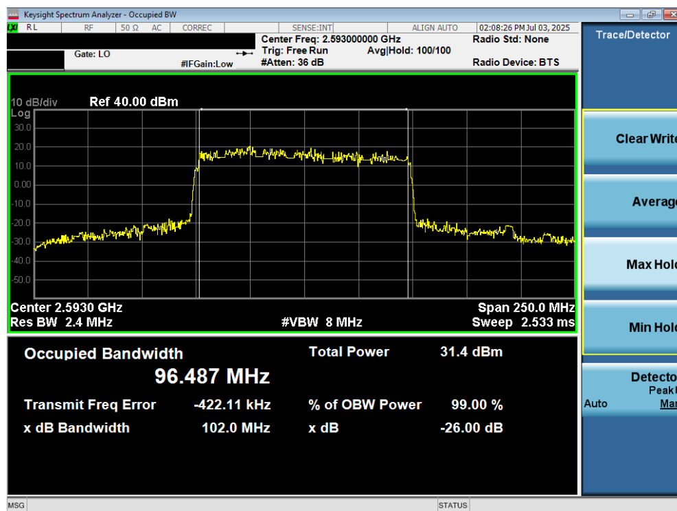
Plot 6-4. Occupied Bandwidth Plot (NR Band n41 PC3 – 100MHz \pi/2 BPSK – Full RB – Default – Ant1)
