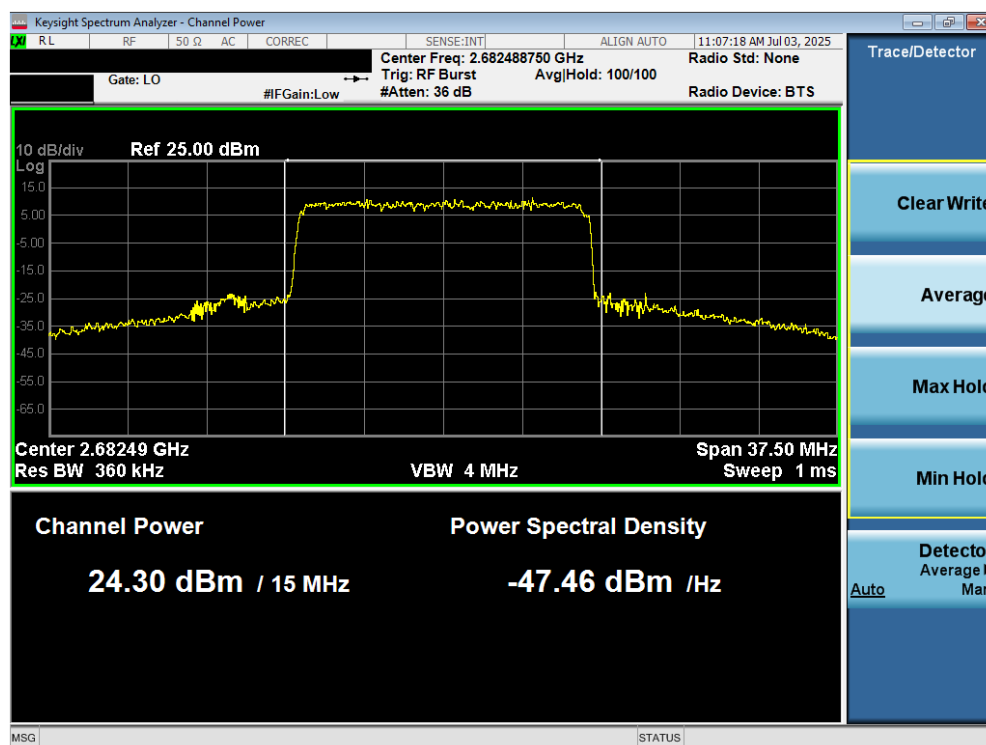
Plot 6-1. Max Conducted Power (LTE Band 41 PC3 - 15MHz QPSK – ANT2)
