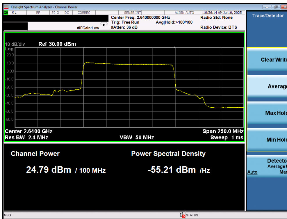
Plot 6-2. Max Conducted Power (NR Band n41 PC3 - 100MHz BPSK)
