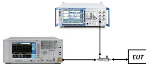
Figure 6-3. Test Instrument & Measurement Setup
