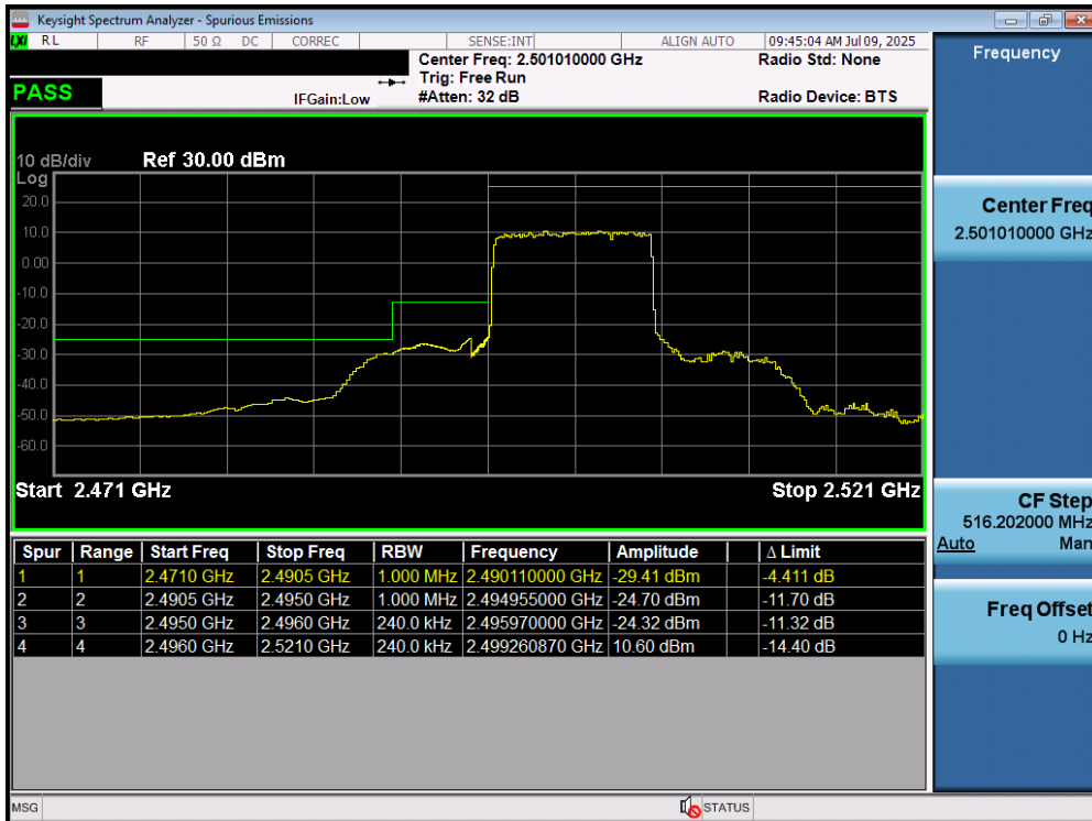
Plot 6-6. Lower ACP Plot (NR Band n41 PC3 - 10MHz CP-OFDM-QPSK – Full RB – Ant1)
