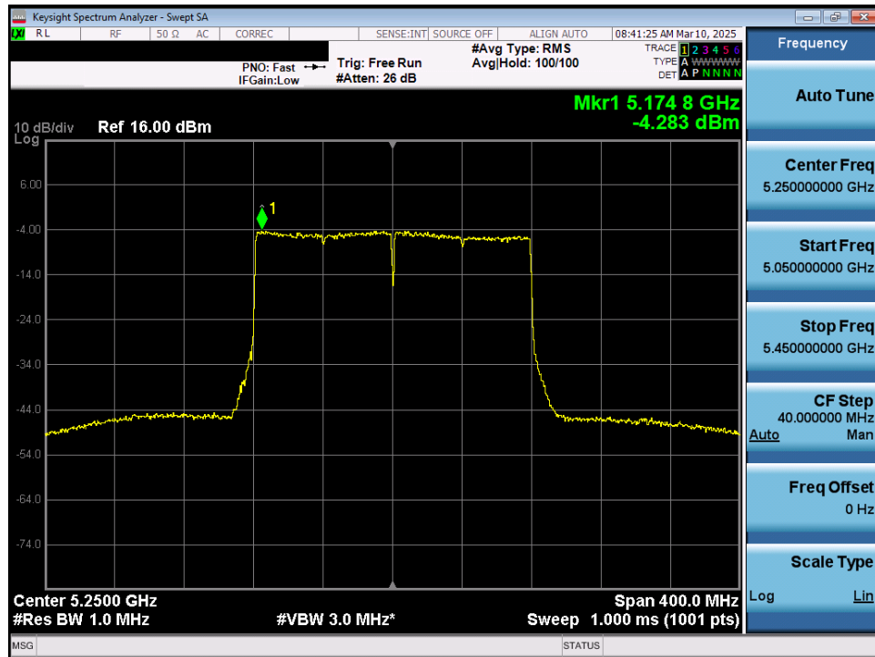
Plot 7-73. Power Spectral Density Plot MIMO ANT1 (160MHz 802.11ax/be (UNII Band 1/2A) – Ch. 50)
