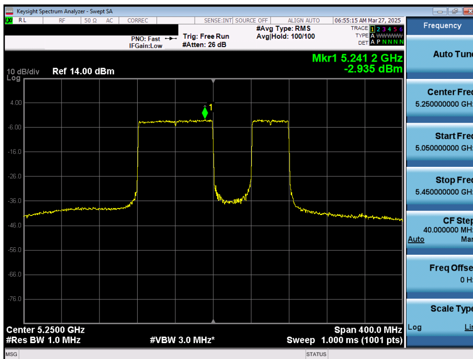
Plot 7-75. Power Spectral Density Plot MIMO ANT1 (160MHz 802.11be (40MHz Puncture) (UNII Band 1/2A) – Ch. 50)
