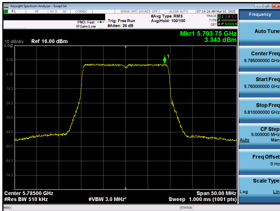
Plot 7-78. Power Spectral Density Plot MIMO ANT1 (20MHz 802.11ax/be (UNII Band 3) – Ch.157)
