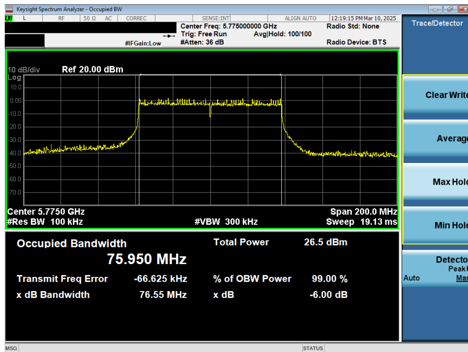
Plot 7-50. 6dB Bandwidth Plot MIMO ANT2 (80MHz 802.11ac (UNII Band 3) – Ch. 155)
