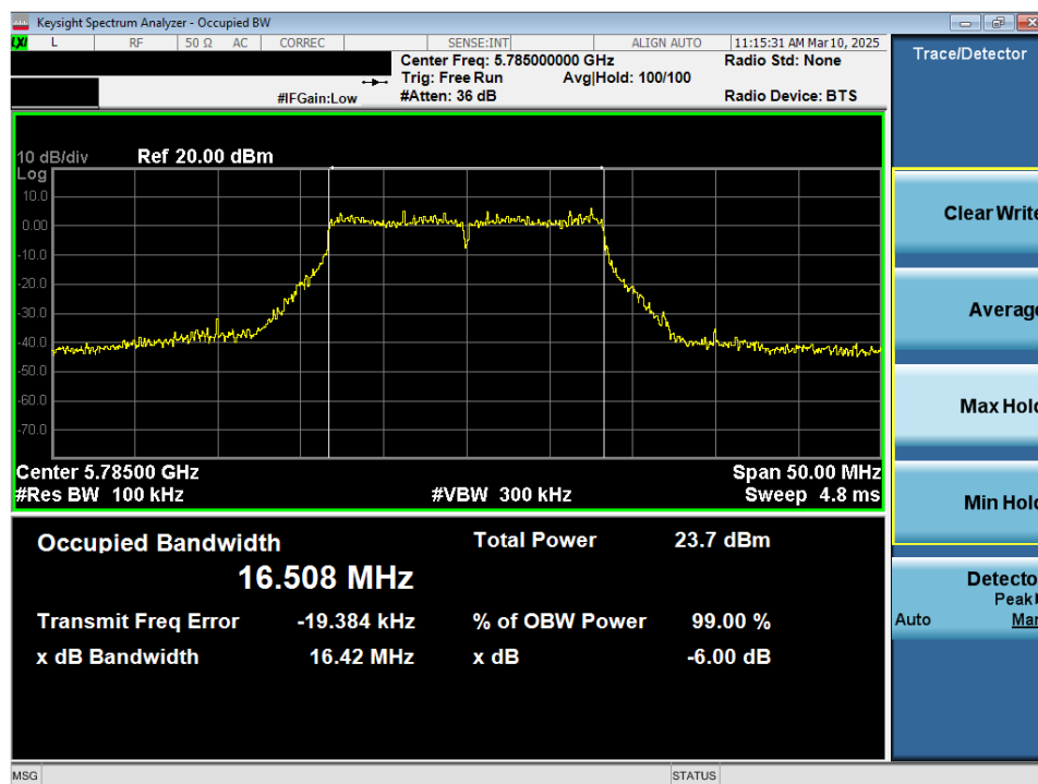
Plot 7-45. 6dB Bandwidth Plot MIMO ANT2 (20MHz 802.11a (UNII Band 3) – Ch.157)
