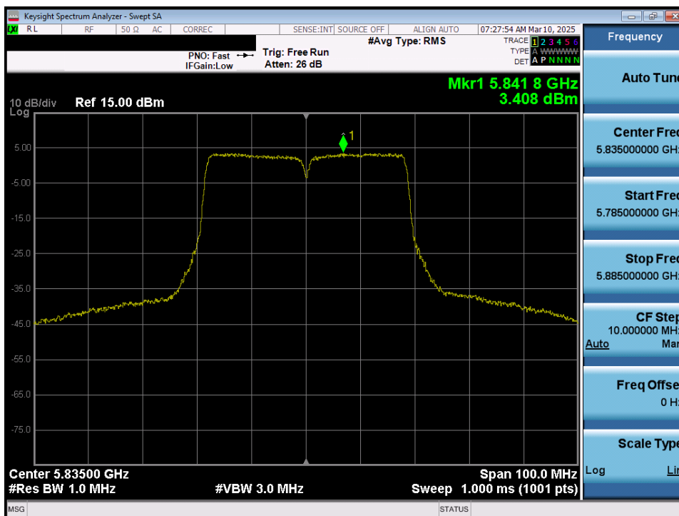
Plot 7-87. Power Spectral Density Plot MIMO ANT1 (40MHz 802.11n (UNII Band 3/4) – Ch. 167)
