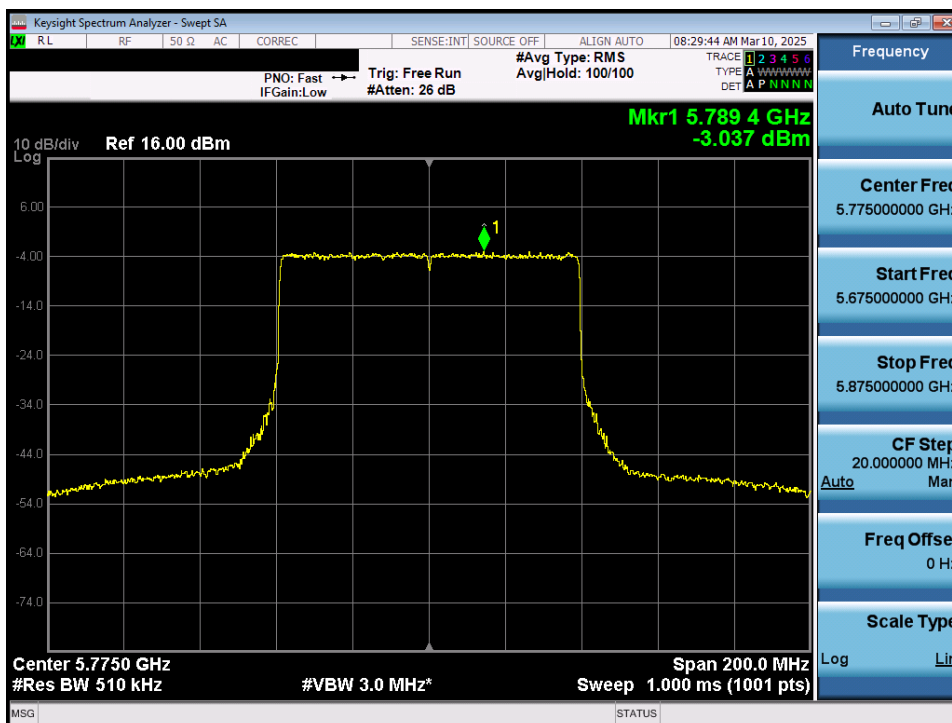
Plot 7-82. Power Spectral Density Plot MIMO ANT1 (80MHz 802.11ax/be (UNII Band 3) – Ch. 155)
