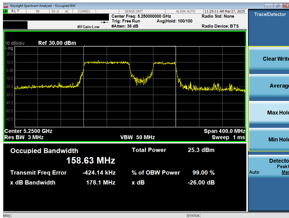
Plot 7-24. 26dB Bandwidth Plot MIMO ANT2 (160MHz 802.11be (40MHz Puncture) (UNII Band 1/2A) – Ch. 50)
