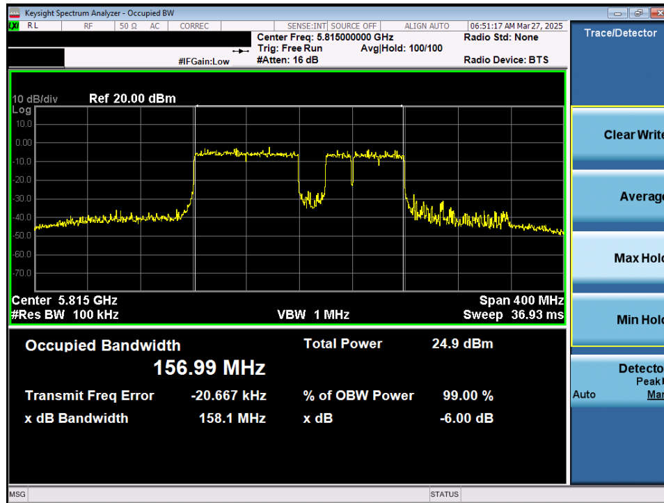
Plot 7-43. 6dB Bandwidth Plot MIMO ANT1 (160MHz 802.11be (20MHz Puncture) (UNII Band 3/4) – Ch. 163)
