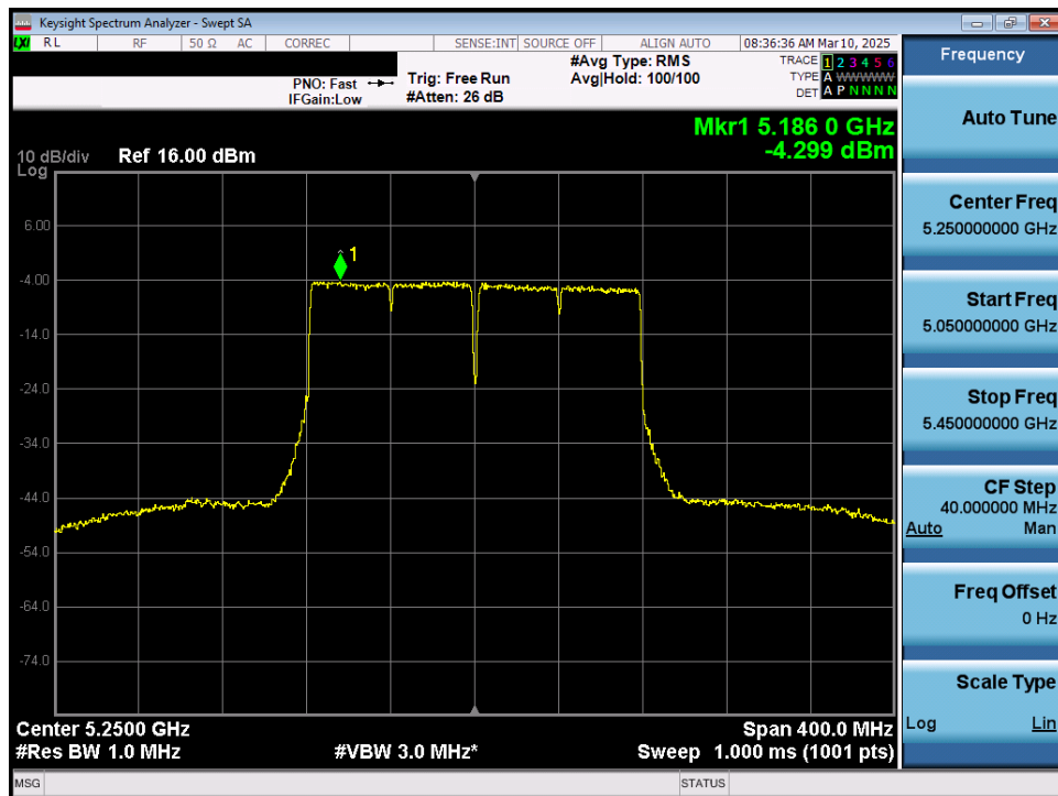
Plot 7-72. Power Spectral Density Plot MIMO ANT1 (160MHz 802.11ac (UNII Band 1/2A) – Ch. 50)
