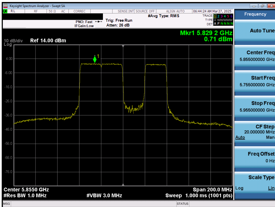
Plot 7-93. Power Spectral Density Plot MIMO ANT1 (80MHz 802.11be (20MHz Puncture) (UNII Band 3/4) – Ch. 171)
