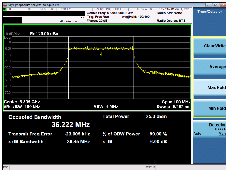
Plot 7-36. 6dB Bandwidth Plot MIMO ANT1 (40MHz 802.11n (UNII Band 3/4) – Ch. 167)
