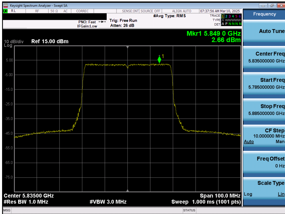
Plot 7-88. Power Spectral Density Plot MIMO ANT1 (40MHz 802.11ax/be (UNII Band 3/4) – Ch. 167)
