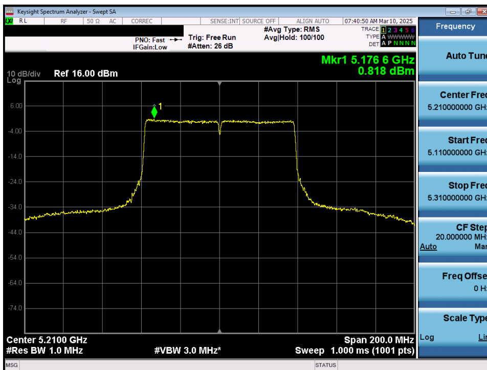
Plot 7-70. Power Spectral Density Plot MIMO ANT1 (80MHz 802.11ac (UNII Band 1) – Ch. 42)
