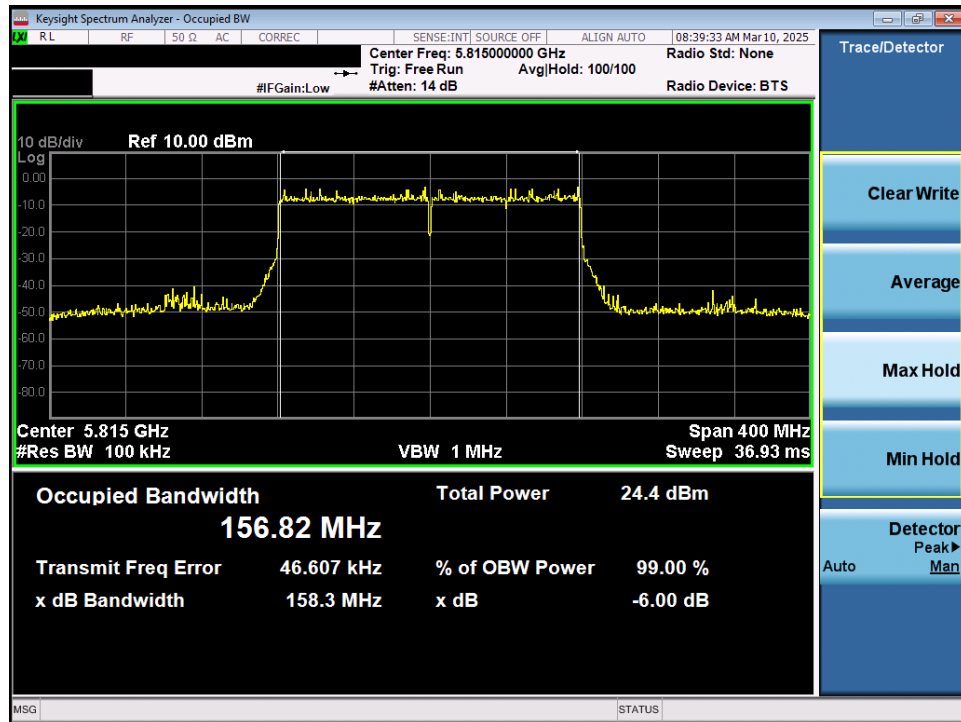
Plot 7-41. 6dB Bandwidth Plot MIMO ANT1 (160MHz 802.11ax/be (UNII Band 3/4) – Ch. 163)
