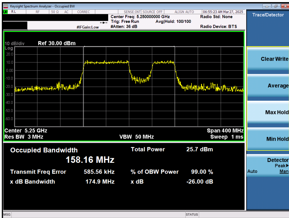
Plot 7-12. 26dB Bandwidth Plot MIMO ANT1 (160MHz 802.11be (40MHz Puncture) (UNII Band 1/2A) – Ch. 50)
