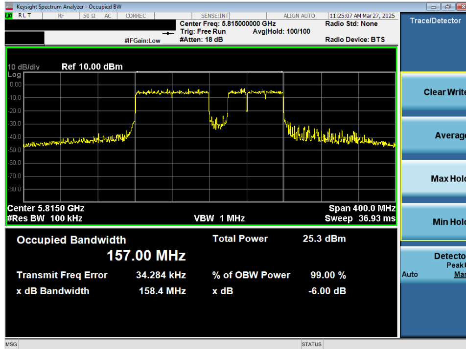
Plot 7-63. 6dB Bandwidth Plot MIMO ANT2 (160MHz 802.11be (20MHz Puncture) (UNII Band 3/4) – Ch. 163)
