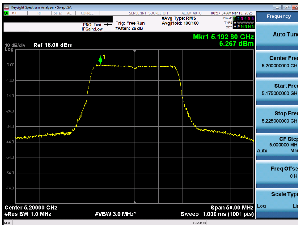
Plot 7-66. Power Spectral Density Plot MIMO ANT1 (20MHz 802.11n (UNII Band 1) – Ch. 40)
