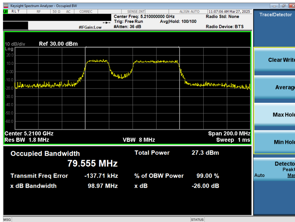
Plot 7-22. 26dB Bandwidth Plot MIMO ANT2 (80MHz 802.11be (20MHz Puncture Tones) (UNII Band 1) – Ch. 42)
