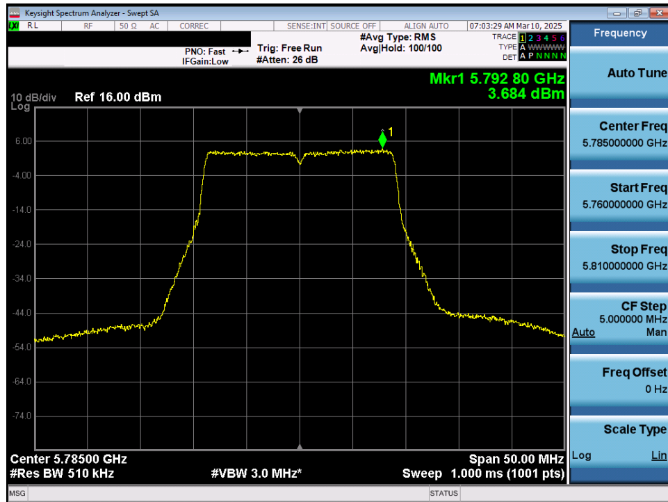
Plot 7-77. Power Spectral Density Plot MIMO ANT1 (20MHz 802.11n (UNII Band 3) – Ch.157)
