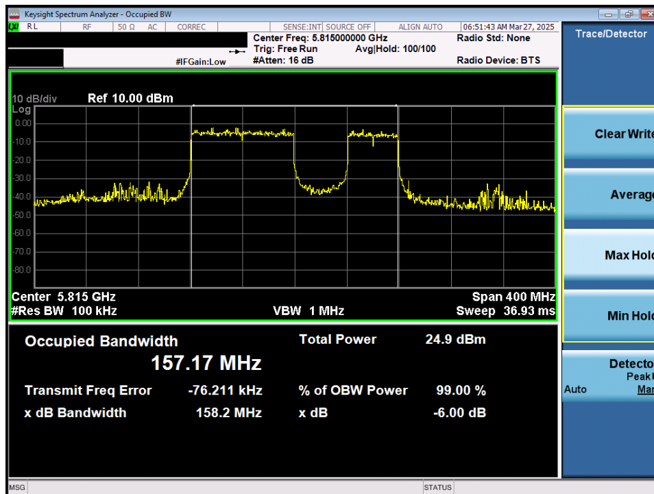
Plot 7-44. 6dB Bandwidth Plot MIMO ANT1 (160MHz 802.11be (40MHz Puncture) (UNII Band 3/4) – Ch. 163)
