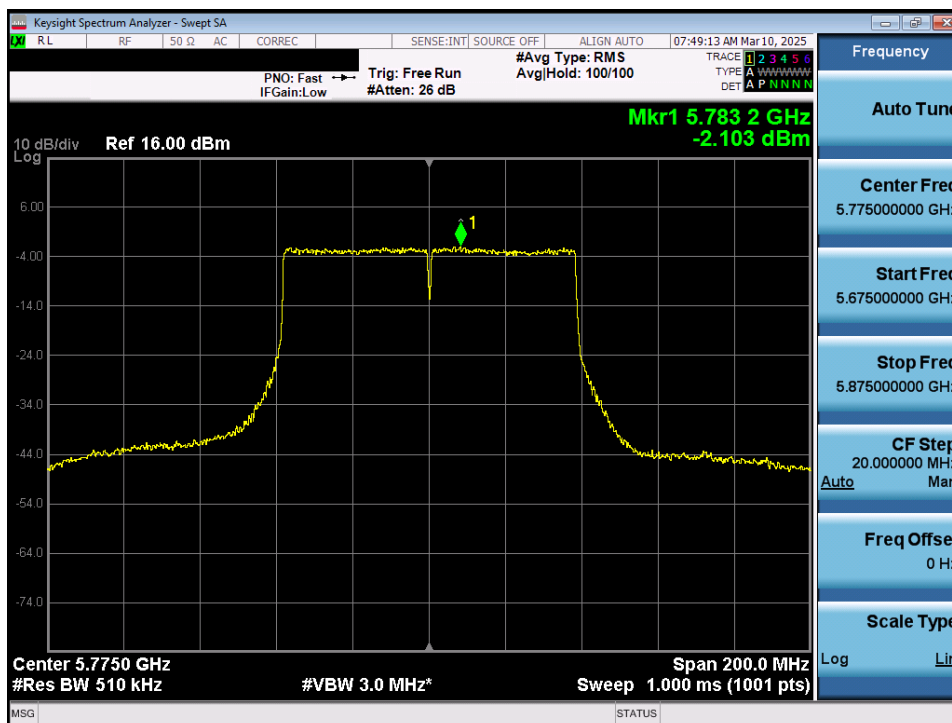
Plot 7-81. Power Spectral Density Plot MIMO ANT1 (80MHz 802.11ac (UNII Band 3) – Ch. 155)
