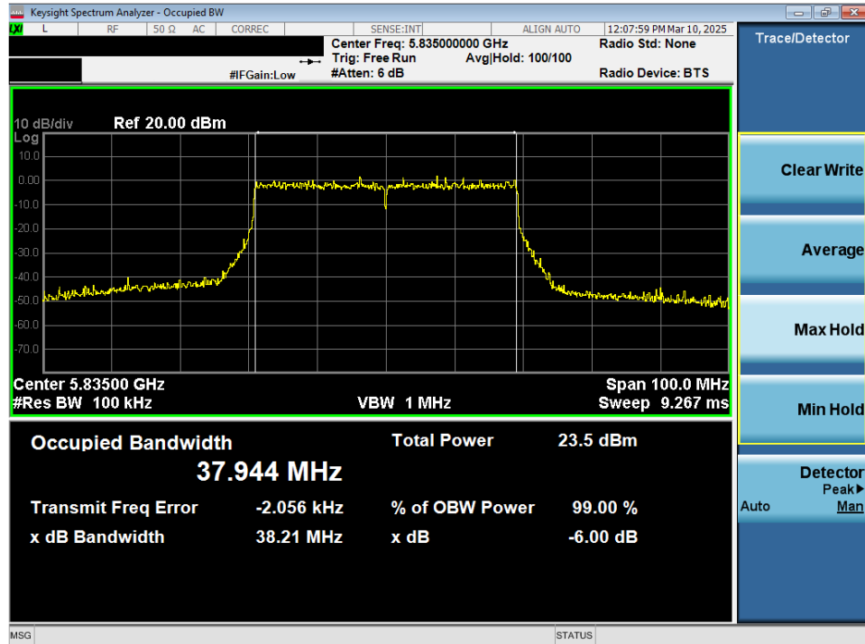
Plot 7-57. 6dB Bandwidth Plot MIMO ANT2 (40MHz 802.11ax/be (UNII Band 3/4) – Ch. 167)
