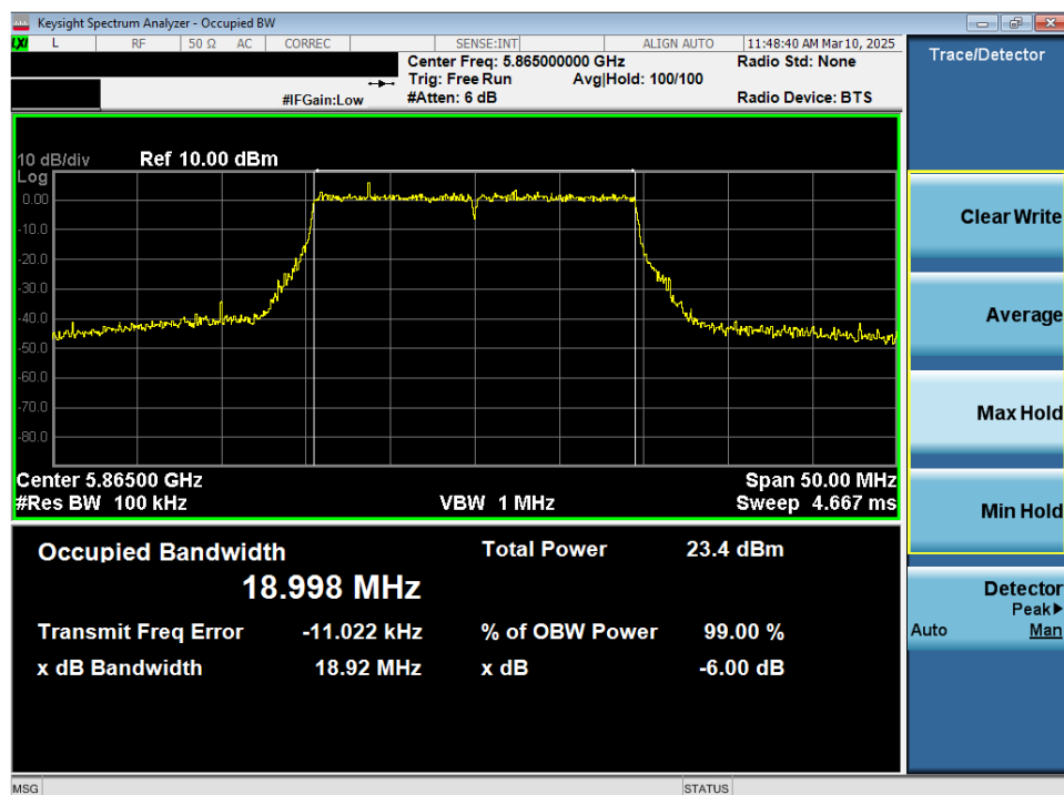
Plot 7-55. 6dB Bandwidth Plot MIMO ANT2 (20MHz 802.11ax/be (UNII Band 4) – Ch.173)
