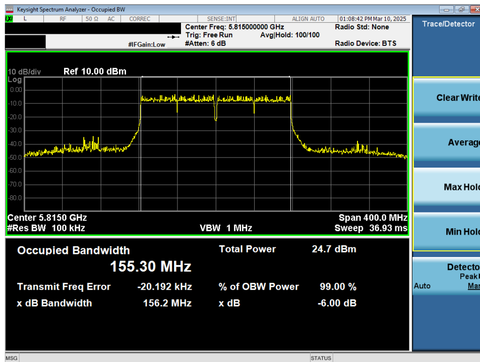
Plot 7-60. 6dB Bandwidth Plot MIMO ANT2 (160MHz 802.11ac (UNII Band 3/4) – Ch. 163)
