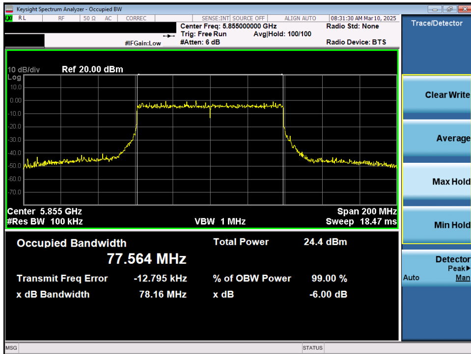
Plot 7-39. 6dB Bandwidth Plot MIMO ANT1 (80MHz 802.11ax/be (UNII Band 3/4) – Ch. 171)
