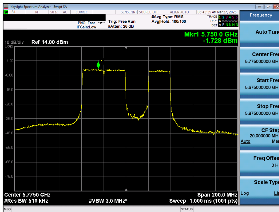
Plot 7-83. Power Spectral Density Plot MIMO ANT1 (80MHz 802.11be (20MHz Puncture) (UNII Band 3) – Ch. 155)
