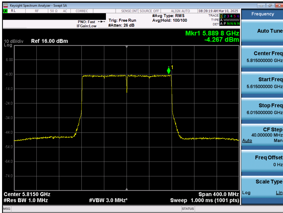
Plot 7-92. Power Spectral Density Plot MIMO ANT1 (160MHz 802.11ax/be (UNII Band 3/4) – Ch. 163)
