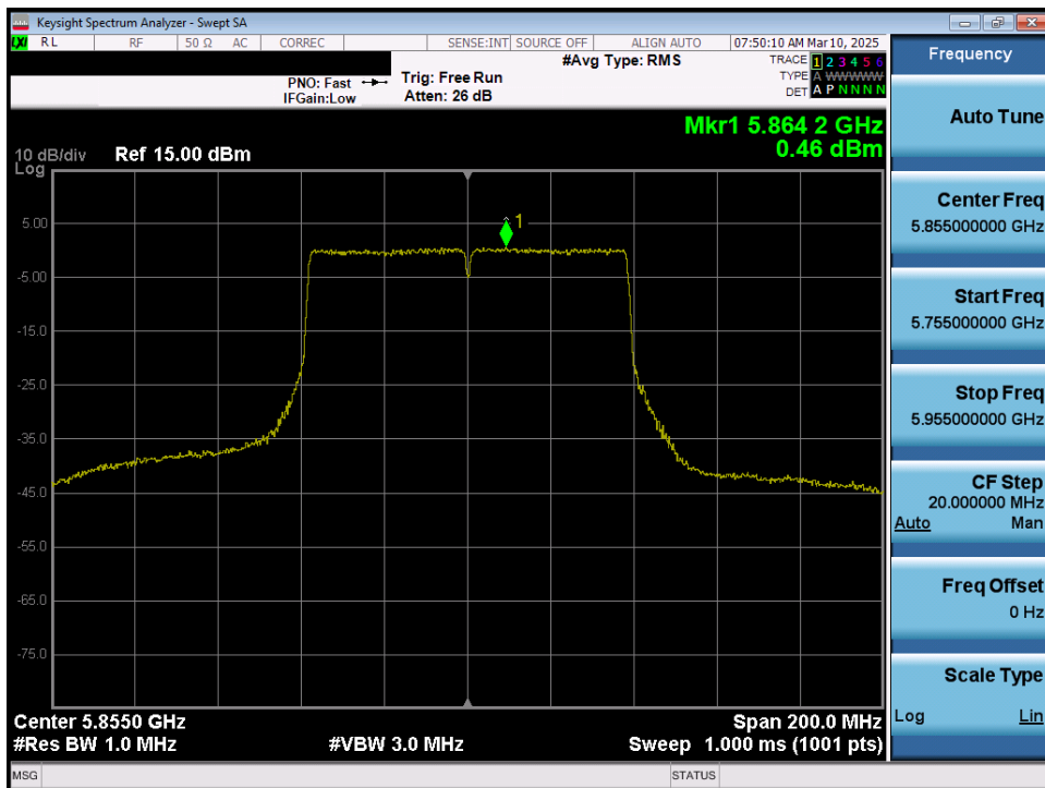
Plot 7-89. Power Spectral Density Plot MIMO ANT1 (80MHz 802.11ac (UNII Band 3/4) – Ch. 171)
