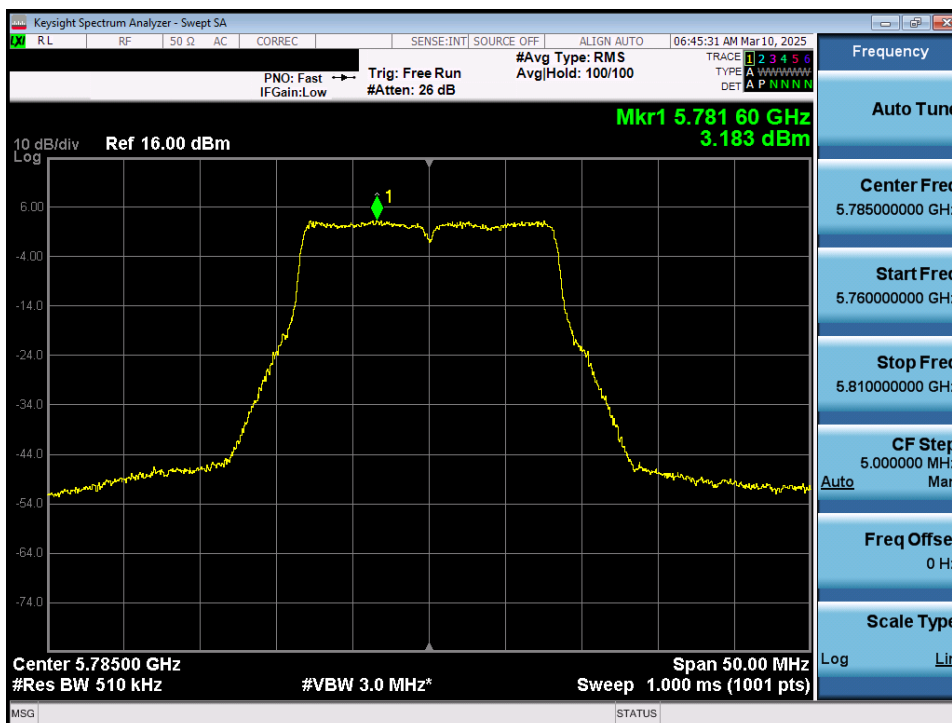
Plot 7-76. Power Spectral Density Plot MIMO ANT1 (20MHz 802.11a (UNII Band 3) – Ch.157)
