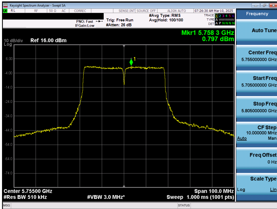
Plot 7-79. Power Spectral Density Plot MIMO ANT1 (40MHz 802.11n (UNII Band 3) – Ch. 151)
