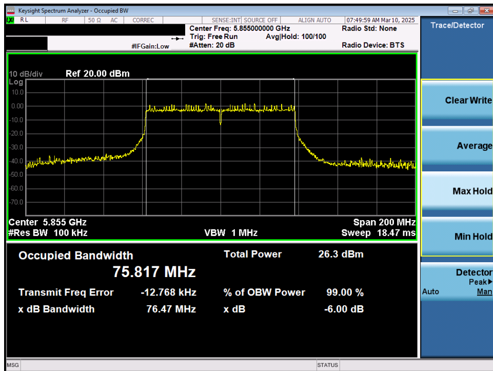
Plot 7-38. 6dB Bandwidth Plot MIMO ANT1 (80MHz 802.11ac (UNII Band 3/4) – Ch. 171)
