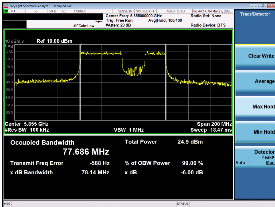
Plot 7-42. 6dB Bandwidth Plot MIMO ANT1 (80MHz 802.11be (20MHz Puncture) (UNII Band 3/4) – Ch. 171)
