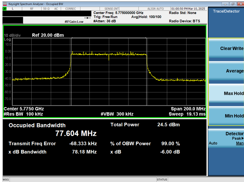
Plot 7-51. 6dB Bandwidth Plot MIMO ANT2 (80MHz 802.11ax/be (UNII Band 3) – Ch. 155)
