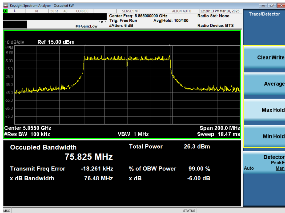
Plot 7-58. 6dB Bandwidth Plot MIMO ANT2 (80MHz 802.11ac (UNII Band 3/4) – Ch. 171)
