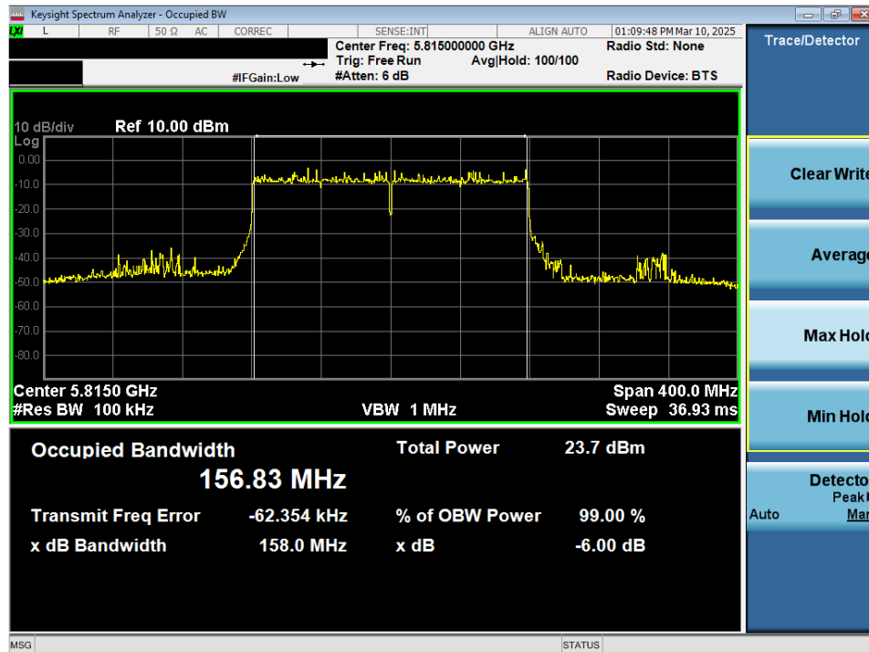
Plot 7-61. 6dB Bandwidth Plot MIMO ANT2 (160MHz 802.11ax/be (UNII Band 3/4) – Ch. 163)
