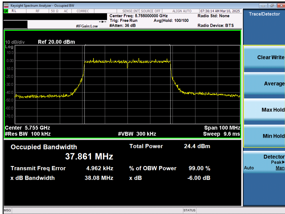
Plot 7-29. 6dB Bandwidth Plot MIMO ANT1 (40MHz 802.11ax/be (UNII Band 3) – Ch. 151)
