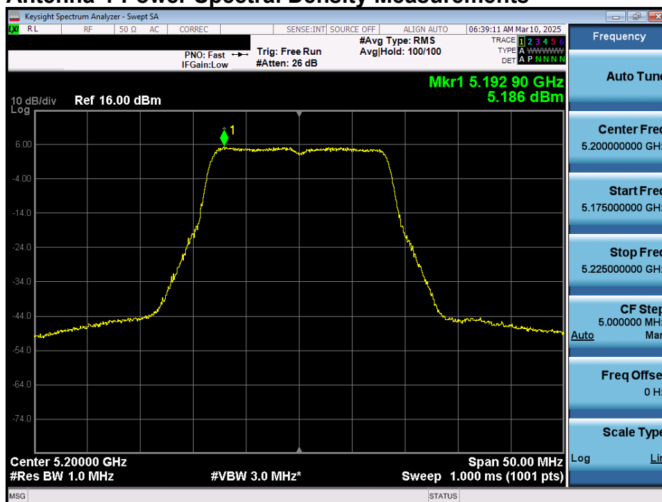
Plot 7-65. Power Spectral Density Plot MIMO ANT1 (20MHz 802.11a (UNII Band 1) – Ch. 40)
