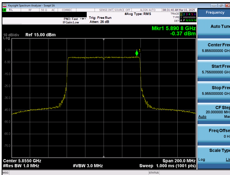
Plot 7-90. Power Spectral Density Plot MIMO ANT1 (80MHz 802.11ax/be (UNII Band 3/4) – Ch. 171)
