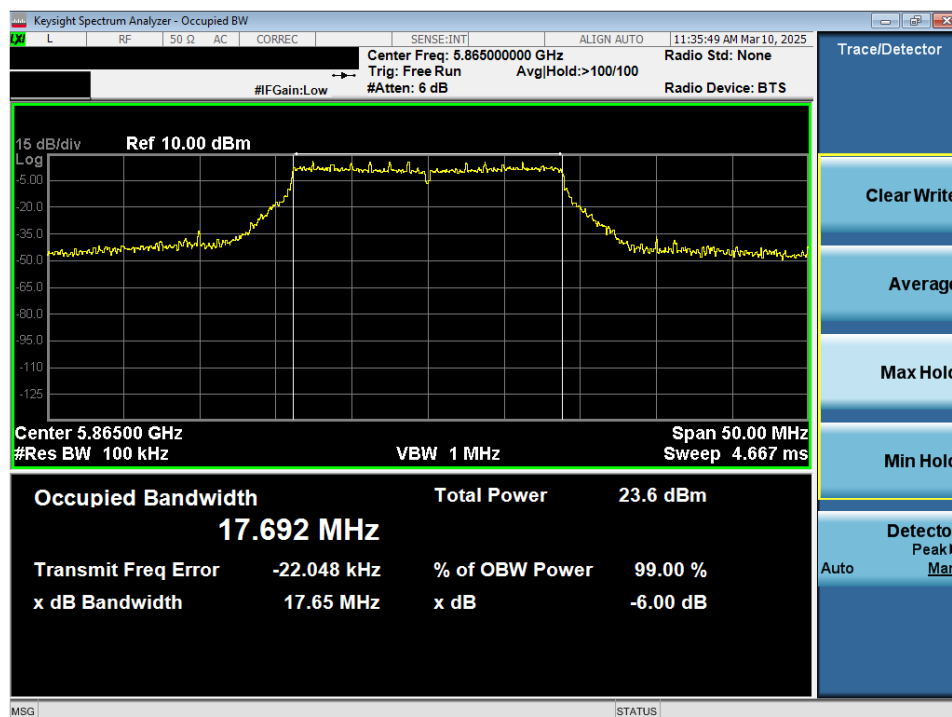
Plot 7-54. 6dB Bandwidth Plot MIMO ANT2 (20MHz 802.11n (UNII Band 4) – Ch.173)
