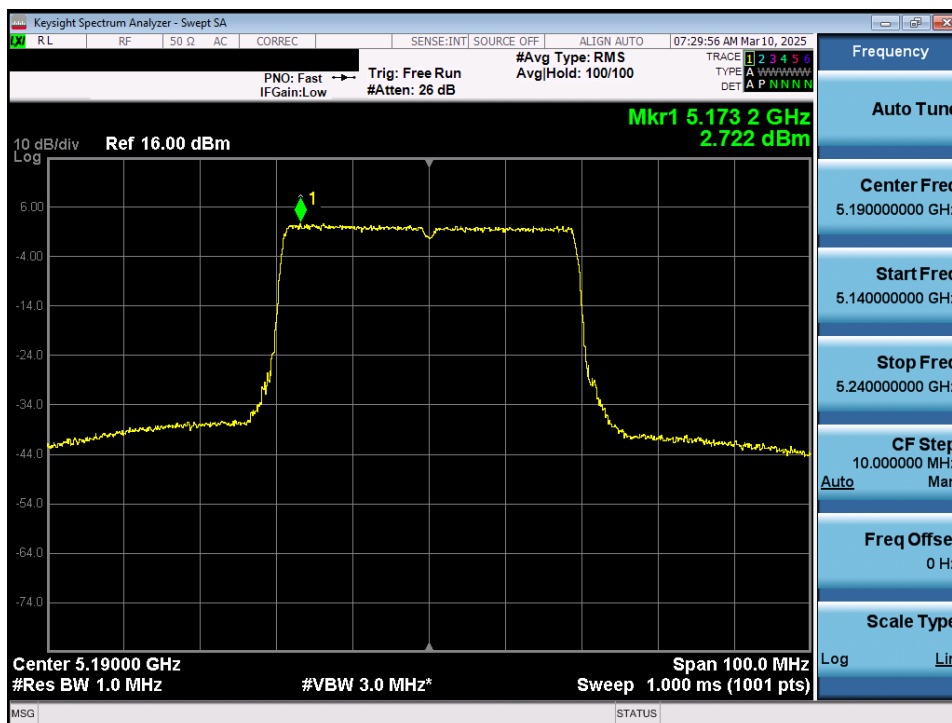
Plot 7-69. Power Spectral Density Plot MIMO ANT1 (40MHz 802.11ax/be (UNII Band 1) – Ch. 38)
