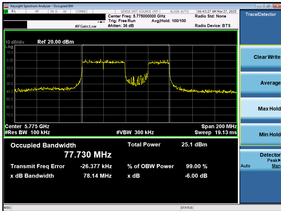
Plot 7-32. 6dB Bandwidth Plot MIMO ANT1 (80MHz 802.11be (20MHz Puncture) (UNII Band 3) – Ch. 155)
