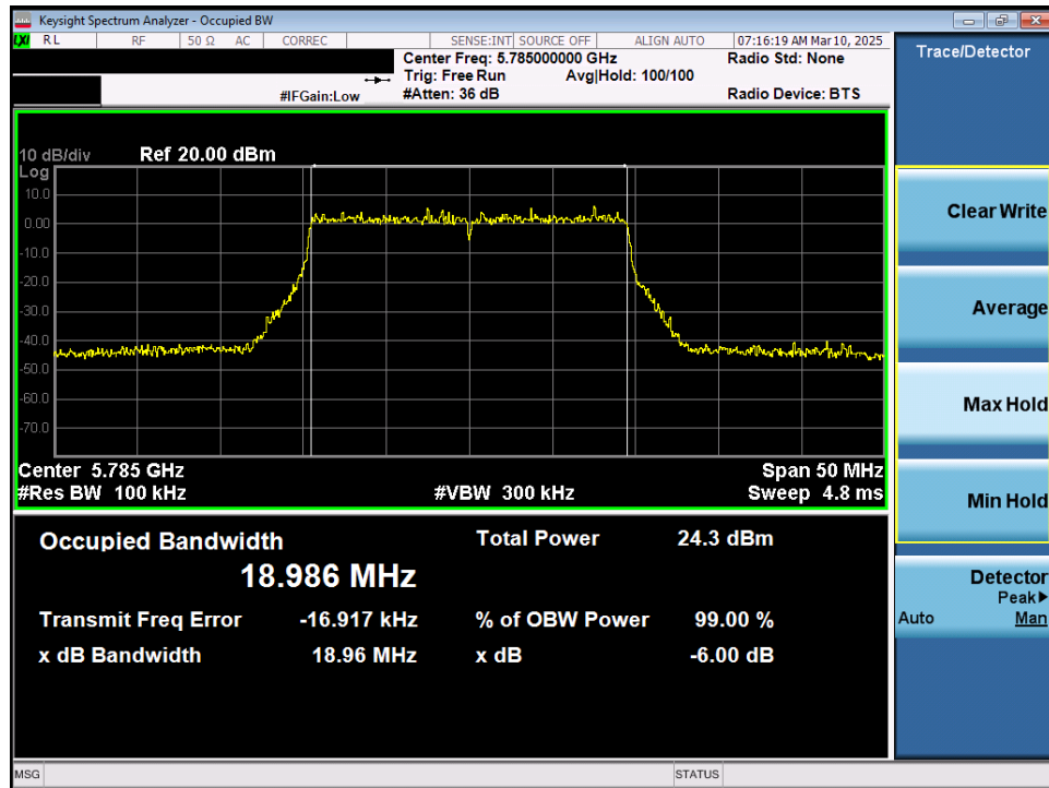
Plot 7-27. 6dB Bandwidth Plot MIMO ANT1 (20MHz 802.11ax/be (UNII Band 3) – Ch.157)
