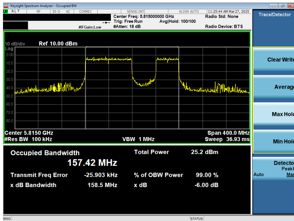
Plot 7-64. 6dB Bandwidth Plot MIMO ANT2 (160MHz 802.11be (40MHz Puncture) (UNII Band 3/4) – Ch. 163)
