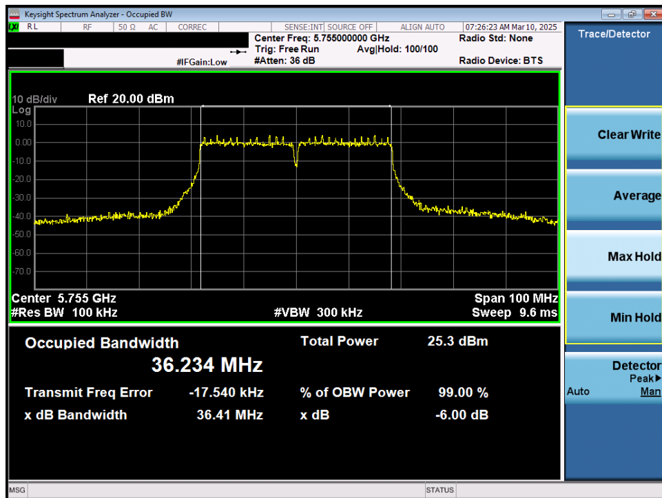
Plot 7-28. 6dB Bandwidth Plot MIMO ANT1 (40MHz 802.11n (UNII Band 3) – Ch. 151)
