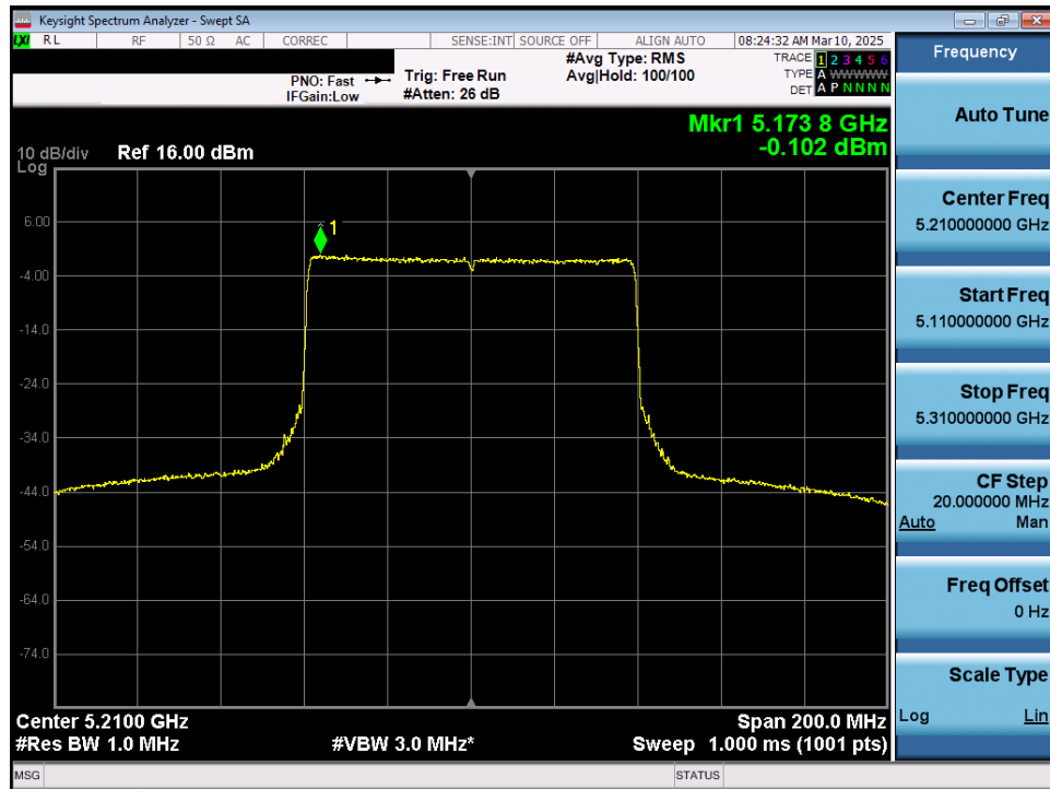
Plot 7-71. Power Spectral Density Plot MIMO ANT1 (80MHz 802.11ax/be (UNII Band 1) – Ch. 42)
