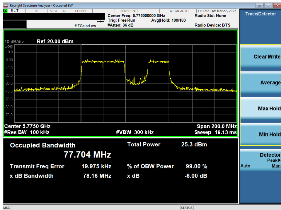
Plot 7-52. 6dB Bandwidth Plot MIMO ANT2 (80MHz 802.11be (20MHz Puncture) (UNII Band 3) – Ch. 155)
