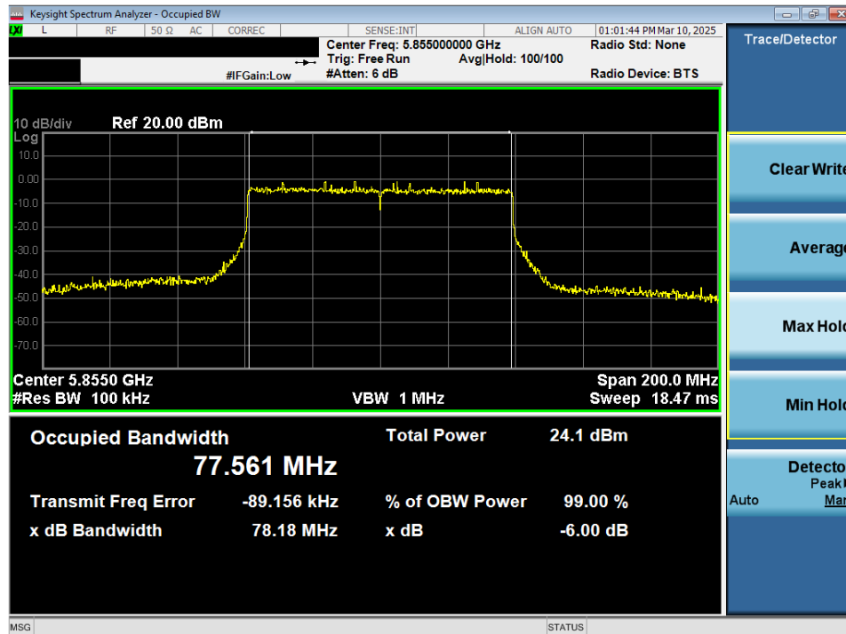
Plot 7-59. 6dB Bandwidth Plot MIMO ANT2 (80MHz 802.11ax/be (UNII Band 3/4) – Ch. 171)
