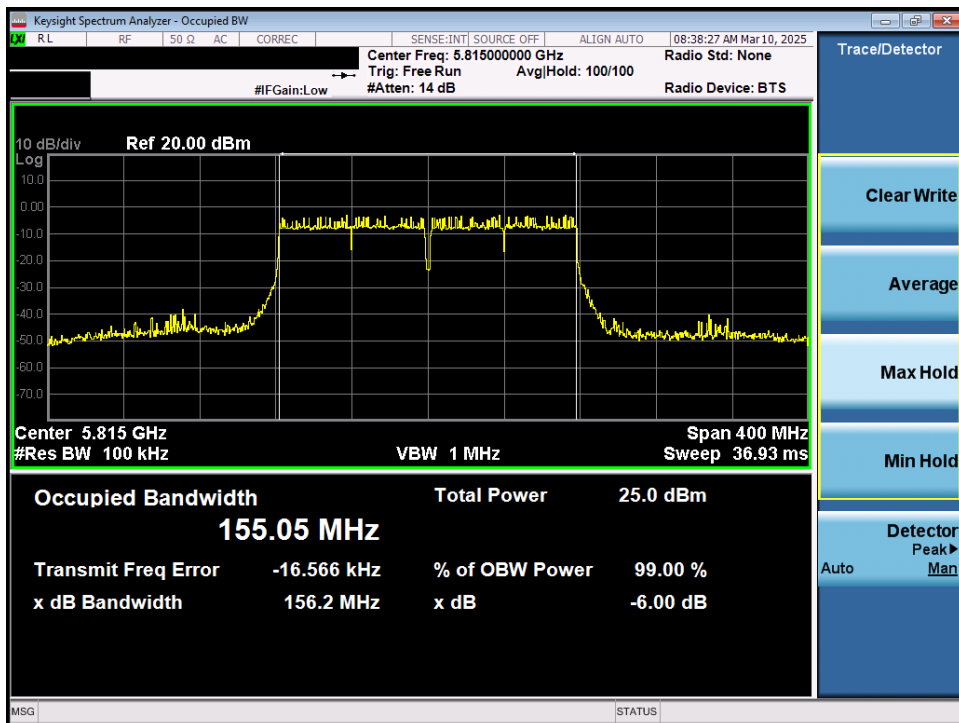
Plot 7-40. 6dB Bandwidth Plot MIMO ANT1 (160MHz 802.11ac (UNII Band 3/4) – Ch. 163)
