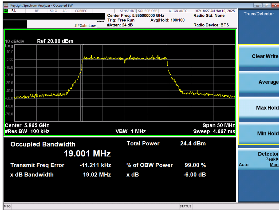
Plot 7-35. 6dB Bandwidth Plot MIMO ANT1 (20MHz 802.11ax/be (UNII Band 4) – Ch.173)
