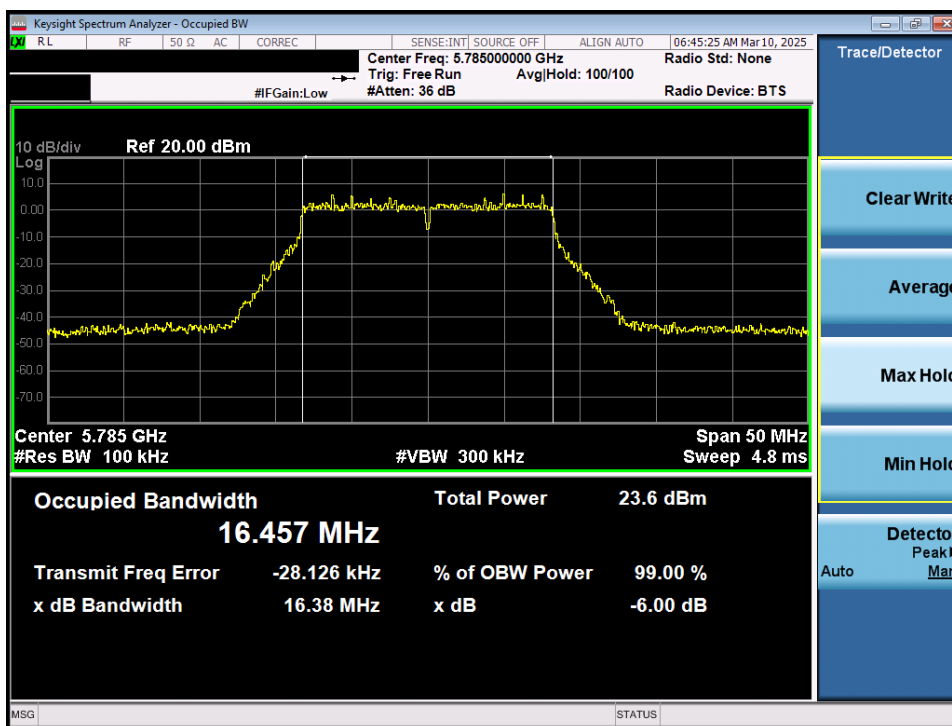
Plot 7-25. 6dB Bandwidth Plot MIMO ANT1 (20MHz 802.11a (UNII Band 3) – Ch.157)
