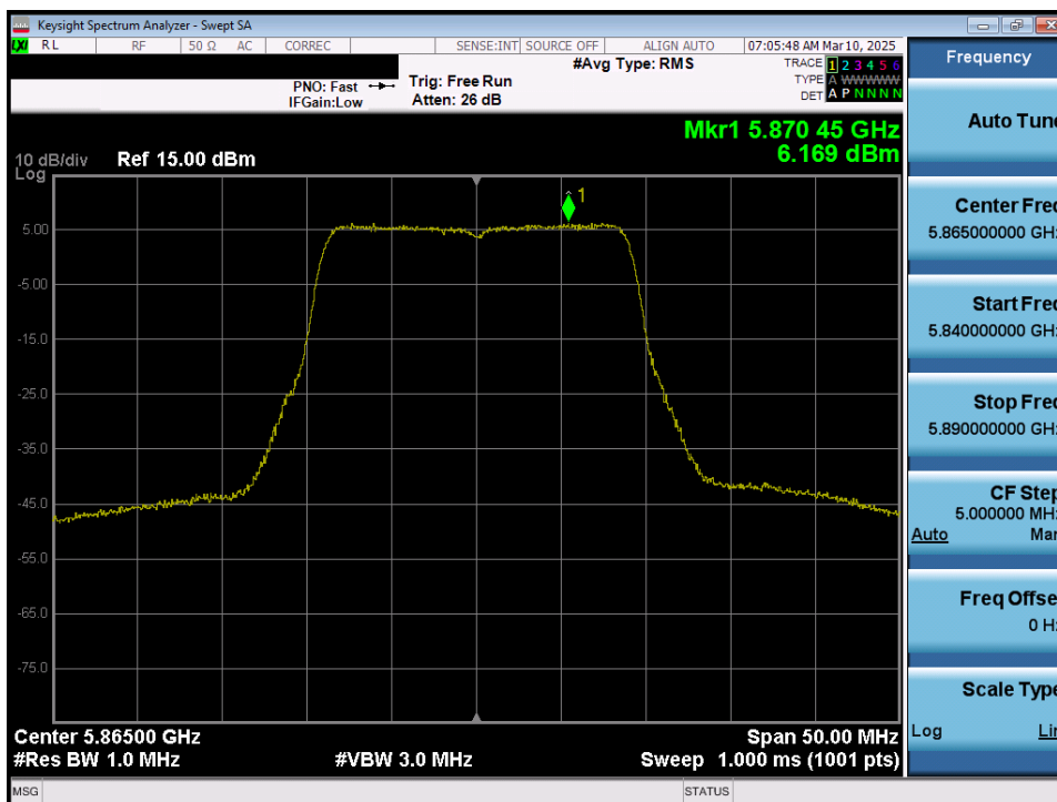
Plot 7-85. Power Spectral Density Plot MIMO ANT1 (20MHz 802.11n (UNII Band 4) – Ch.173)
