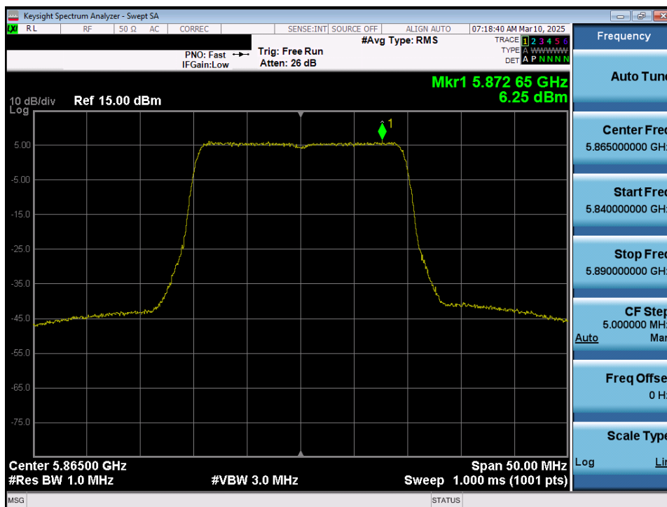
Plot 7-86. Power Spectral Density Plot MIMO ANT1 (20MHz 802.11ax/be (UNII Band 4) – Ch.173)
