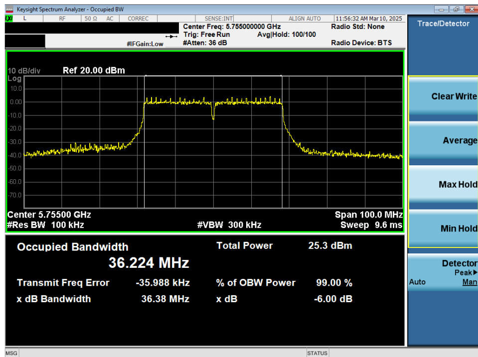
Plot 7-48. 6dB Bandwidth Plot MIMO ANT2 (40MHz 802.11n (UNII Band 3) – Ch. 151)
