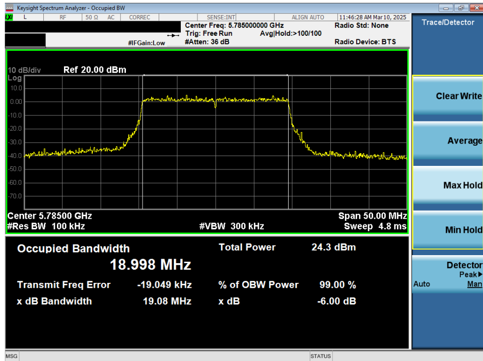
Plot 7-47. 6dB Bandwidth Plot MIMO ANT2 (20MHz 802.11ax/be (UNII Band 3) – Ch.157)
