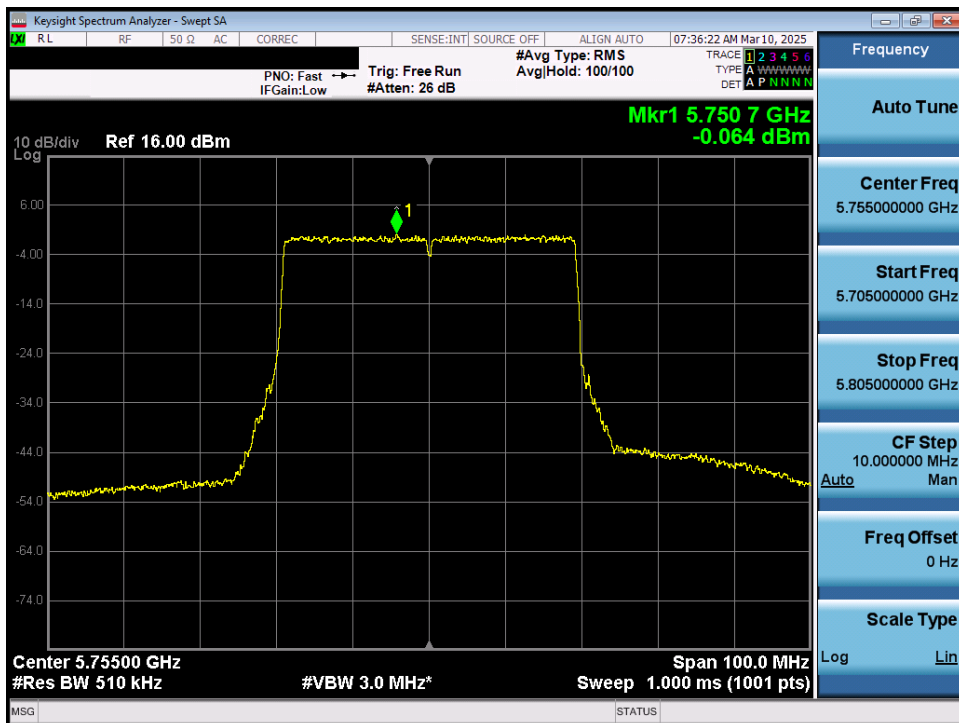
Plot 7-80. Power Spectral Density Plot MIMO ANT1 (40MHz 802.11ax/be (UNII Band 3) – Ch. 151)
