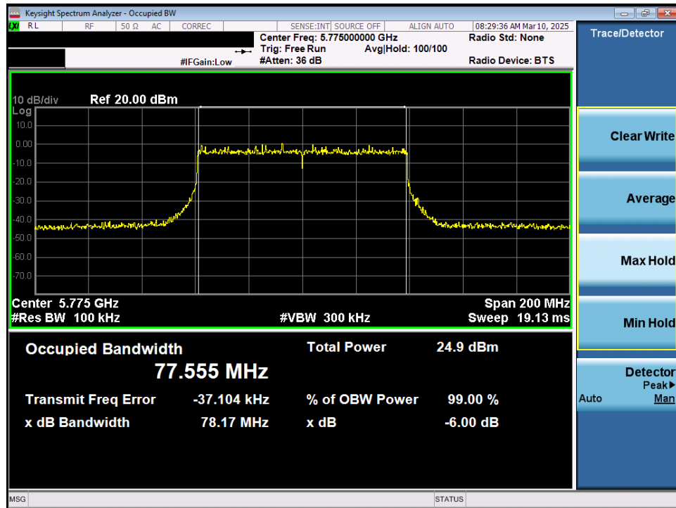
Plot 7-31. 6dB Bandwidth Plot MIMO ANT1 (80MHz 802.11ax/be (UNII Band 3) – Ch. 155)
