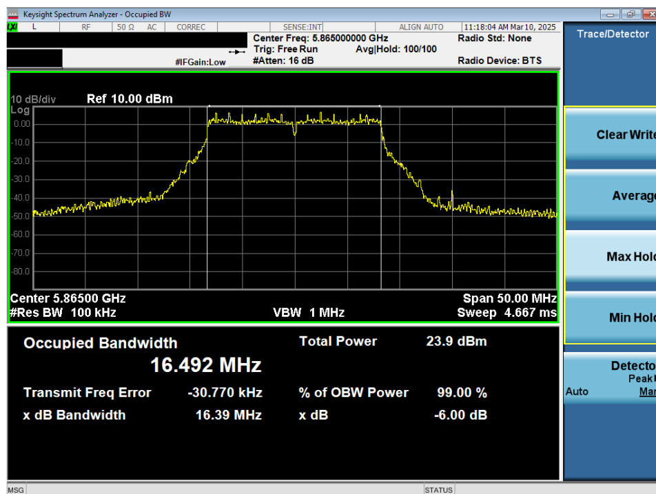
Plot 7-53. 6dB Bandwidth Plot MIMO ANT2 (20MHz 802.11a (UNII Band 4) – Ch.173)
