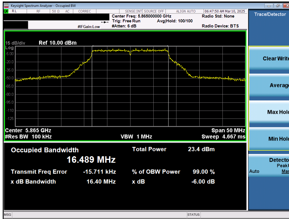
Plot 7-33. 6dB Bandwidth Plot MIMO ANT1 (20MHz 802.11a (UNII Band 4) – Ch.173)
