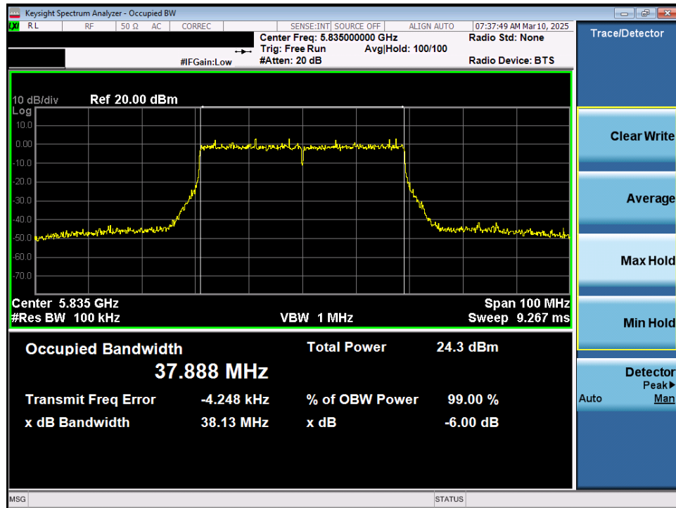
Plot 7-37. 6dB Bandwidth Plot MIMO ANT1 (40MHz 802.11ax/be (UNII Band 3/4) – Ch. 167)
