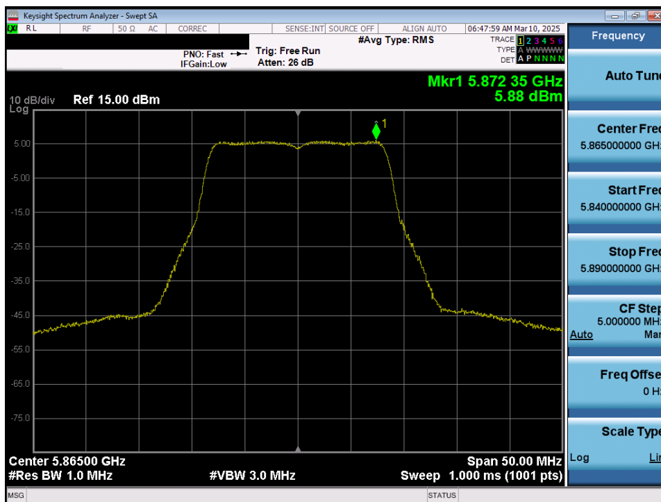
Plot 7-84. Power Spectral Density Plot MIMO ANT1 (20MHz 802.11a (UNII Band 4) – Ch.173)
