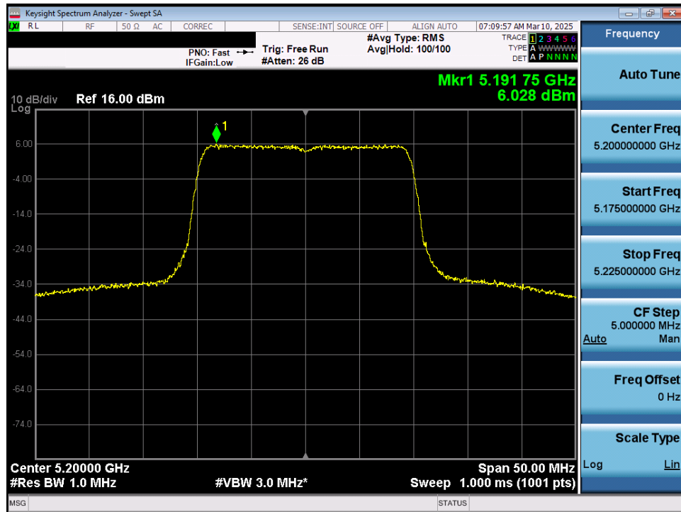
Plot 7-67. Power Spectral Density Plot MIMO ANT1 (20MHz 802.11ax/be (UNII Band 1) – Ch. 40)
