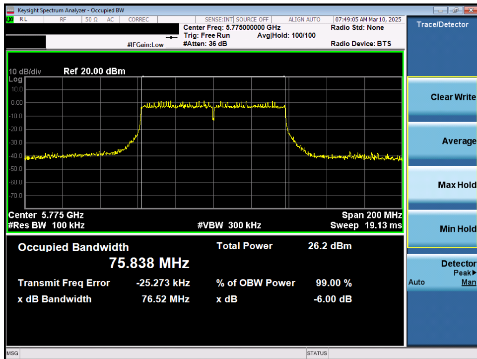
Plot 7-30. 6dB Bandwidth Plot MIMO ANT1 (80MHz 802.11ac (UNII Band 3) – Ch. 155)
