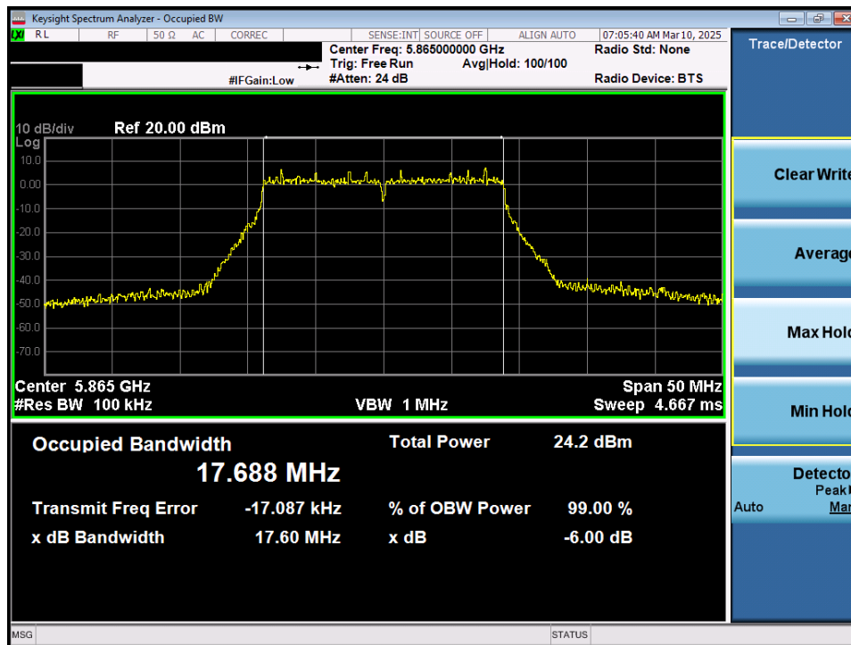
Plot 7-34. 6dB Bandwidth Plot MIMO ANT1 (20MHz 802.11n (UNII Band 4) – Ch.173)
