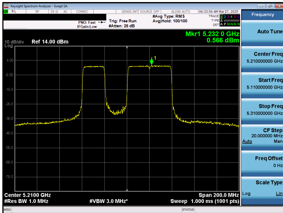
Plot 7-74. Power Spectral Density Plot MIMO ANT1 (80MHz 802.11be (20MHz Puncture) (UNII Band 1) – Ch. 42)
