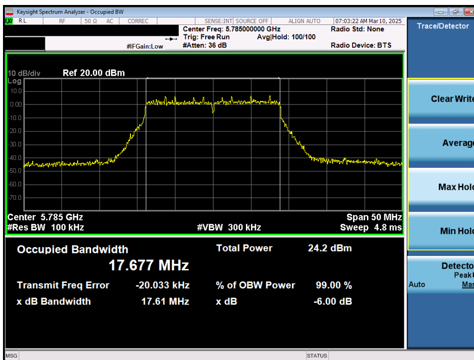
Plot 7-26. 6dB Bandwidth Plot MIMO ANT1 (20MHz 802.11n (UNII Band 3) – Ch.157)
