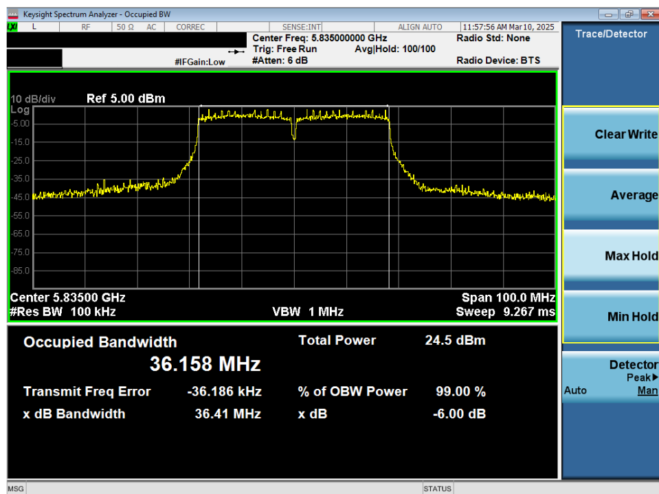
Plot 7-56. 6dB Bandwidth Plot MIMO ANT2 (40MHz 802.11n (UNII Band 3/4) – Ch. 167)
