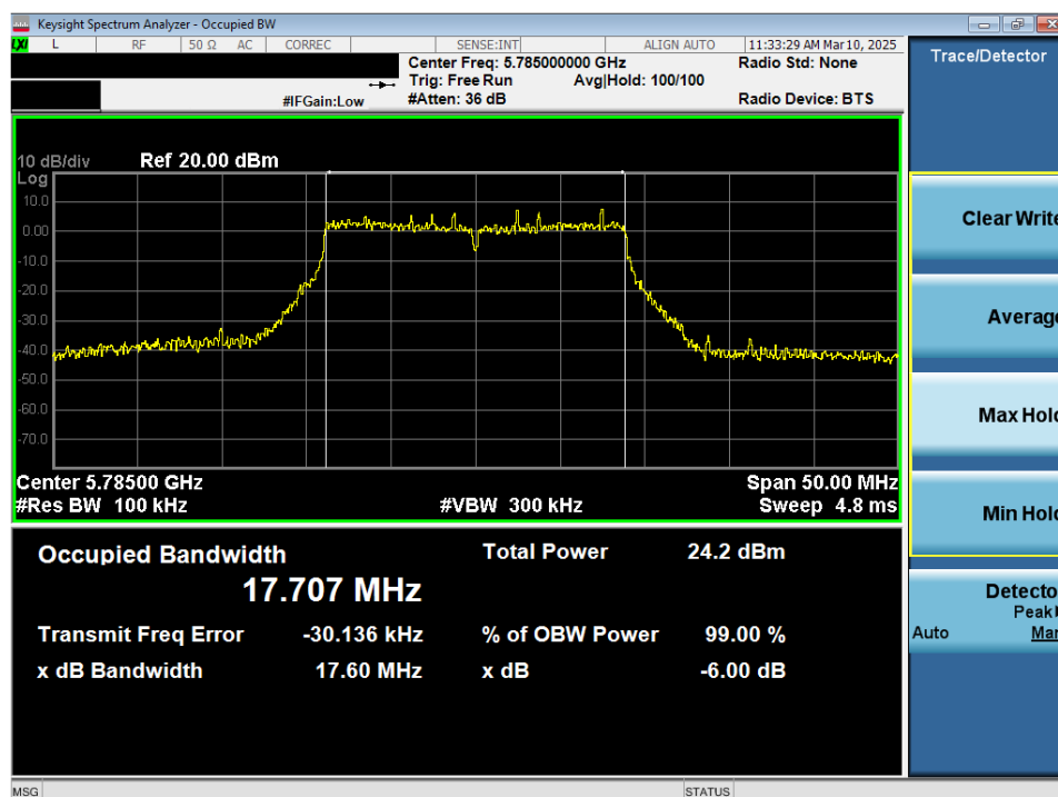
Plot 7-46. 6dB Bandwidth Plot MIMO ANT2 (20MHz 802.11n (UNII Band 3) – Ch.157)
