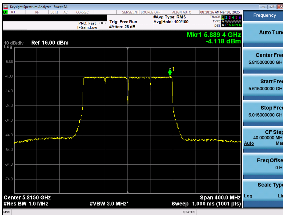
Plot 7-91. Power Spectral Density Plot MIMO ANT1 (160MHz 802.11ac (UNII Band 3/4) – Ch. 163)
