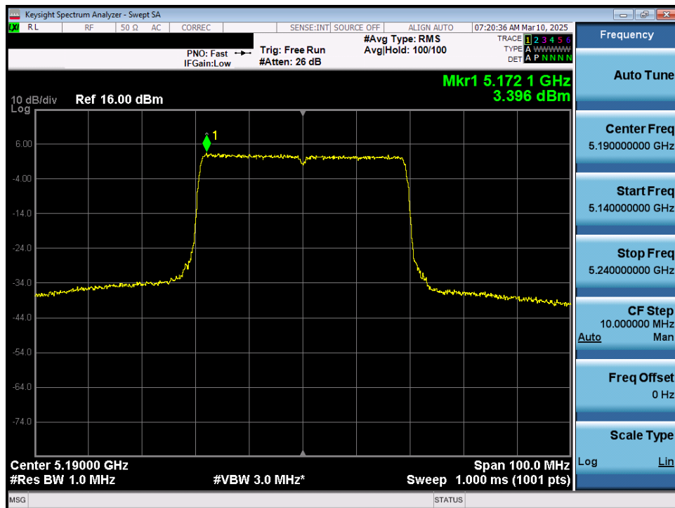
Plot 7-68. Power Spectral Density Plot MIMO ANT1 (40MHz 802.11n (UNII Band 1) – Ch. 38)
