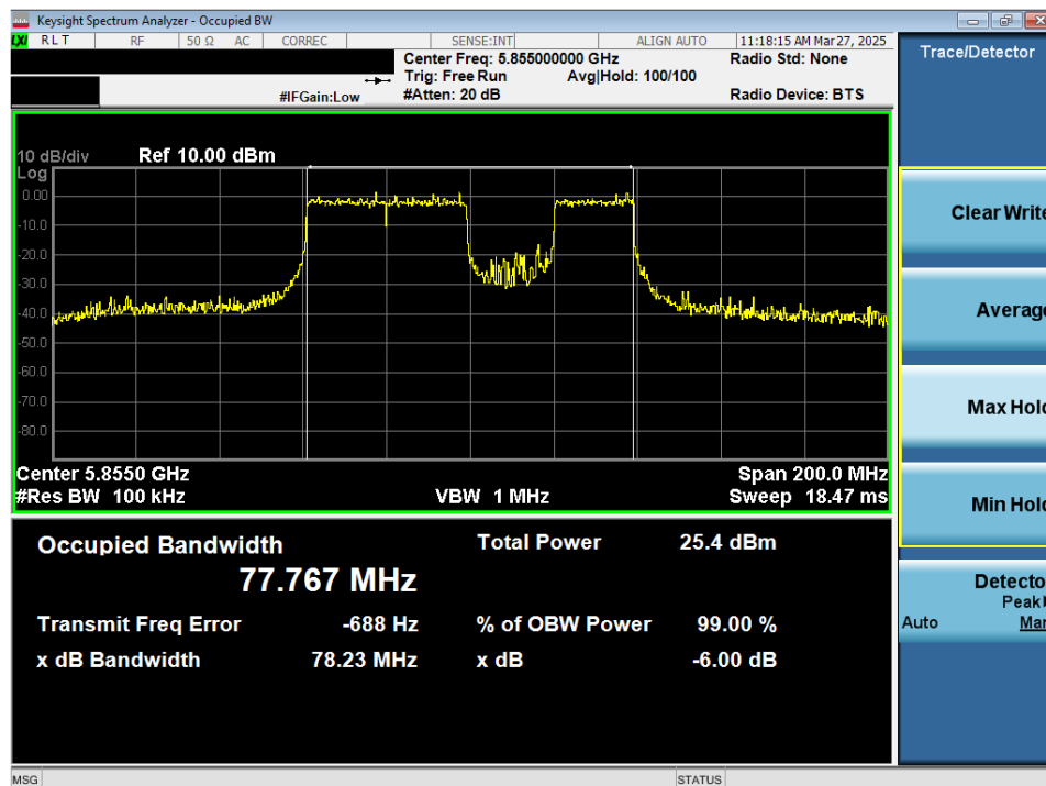
Plot 7-62. 6dB Bandwidth Plot MIMO ANT2 (80MHz 802.11be (20MHz Puncture) (UNII Band 3/4) – Ch. 171)
