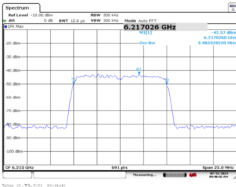
Plot 7-73. AWGN Signal (Demonstration)
