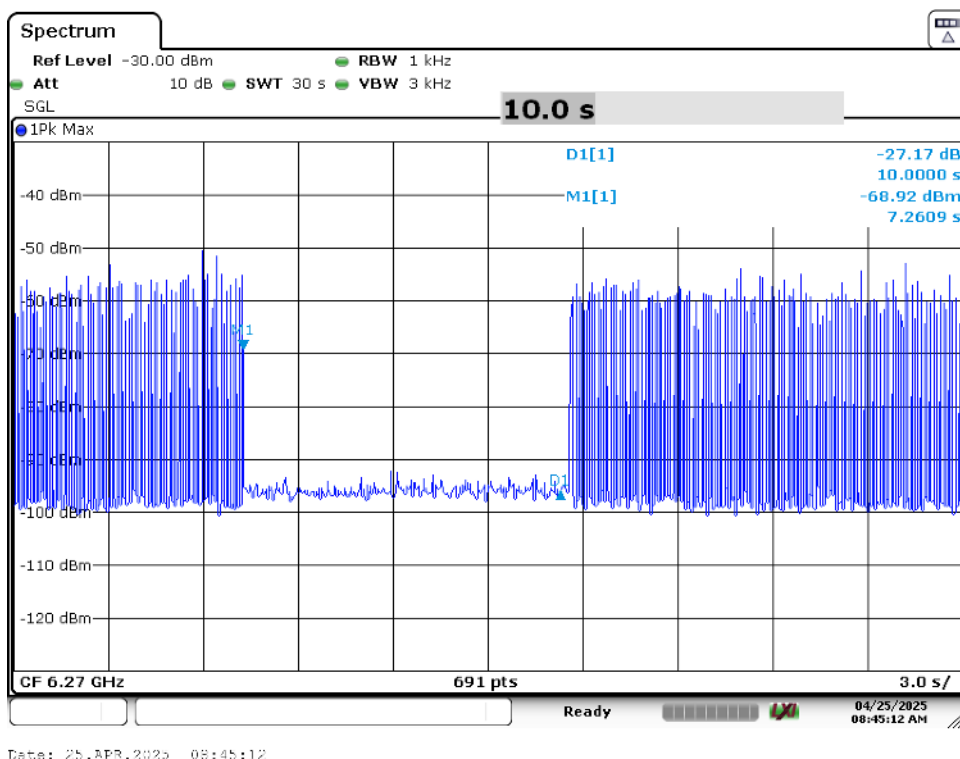
Plot 7-79. Contention Based Protocol Timing Plot (320MHz (UNII Band 6) – Ch. 95 Low)
