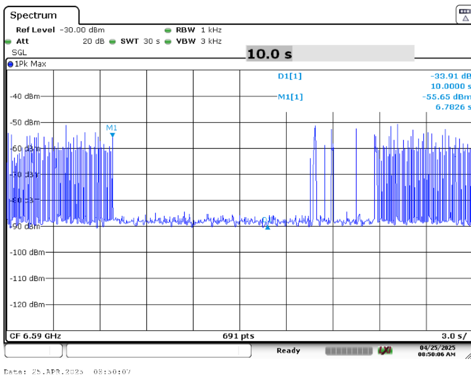
Plot 7-83. Contention Based Protocol Timing Plot (320MHz (UNII Band 7) – Ch. 159 Low)
