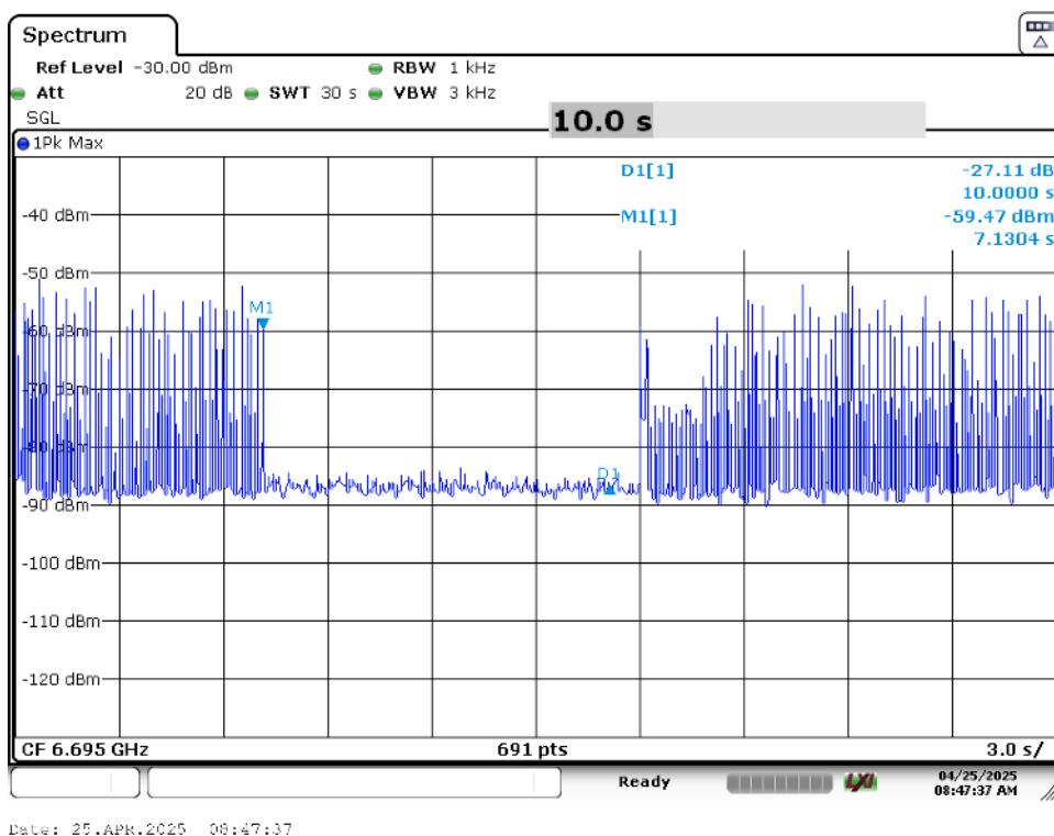
Plot 7-82. Contention Based Protocol Timing Plot (20MHz (UNII Band 7) – Ch. 149)
