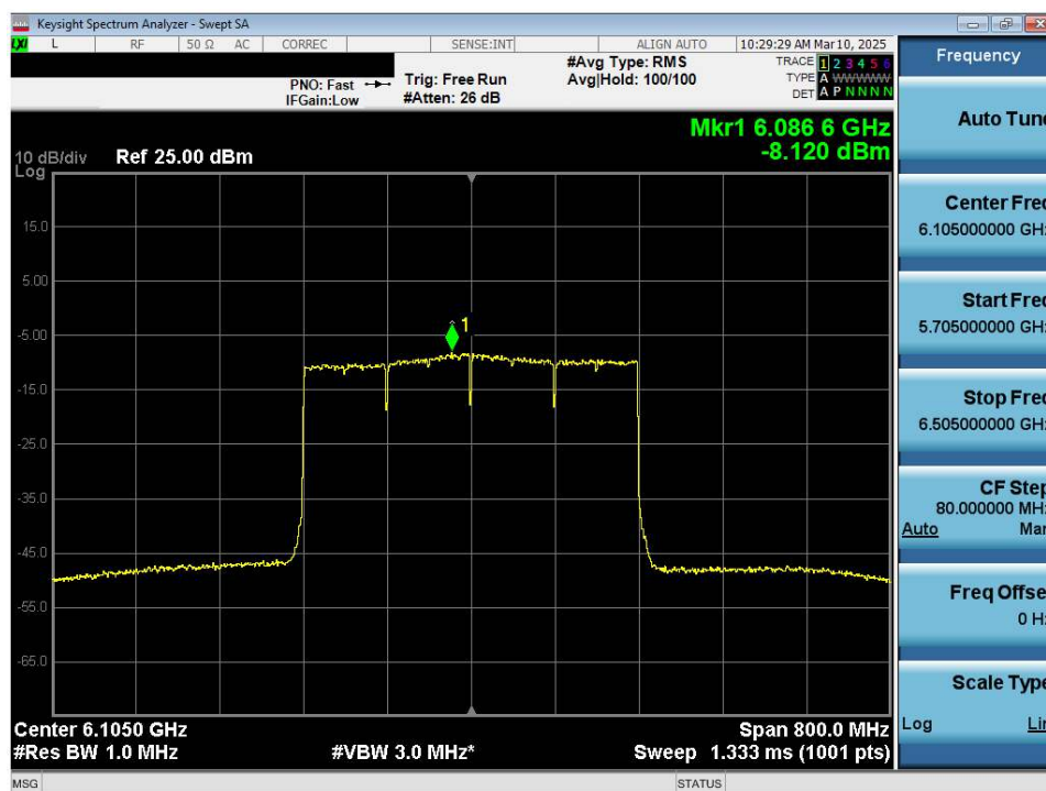
Plot 7-42. Power Spectral Density Plot MIMO ANT2 (320MHz 802.11ax/be (UNII Band 5) – Ch. 31) - LPI/SP
