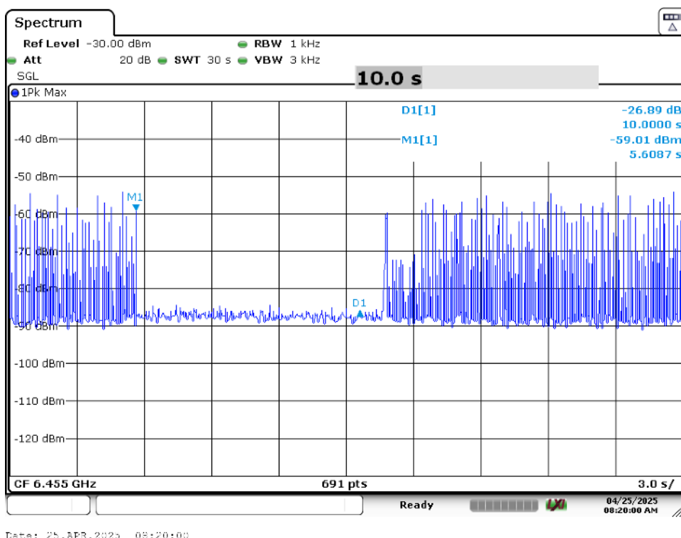
Plot 7-78. Contention Based Protocol Timing Plot (20MHz (UNII Band 6) – Ch. 101)
