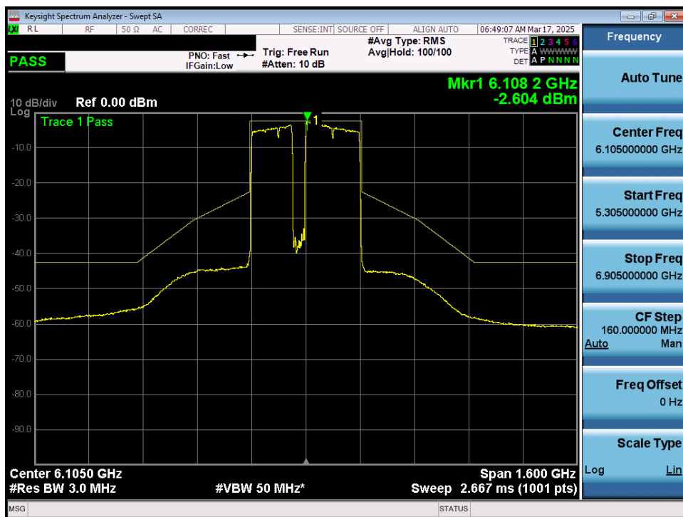
Plot 7-57. In Band Emissions Plot MIMO ANT1 (320MHz 802.11be (UNII Band 5) – Ch. 31) – 40MHz Punctured – LPI/SP
