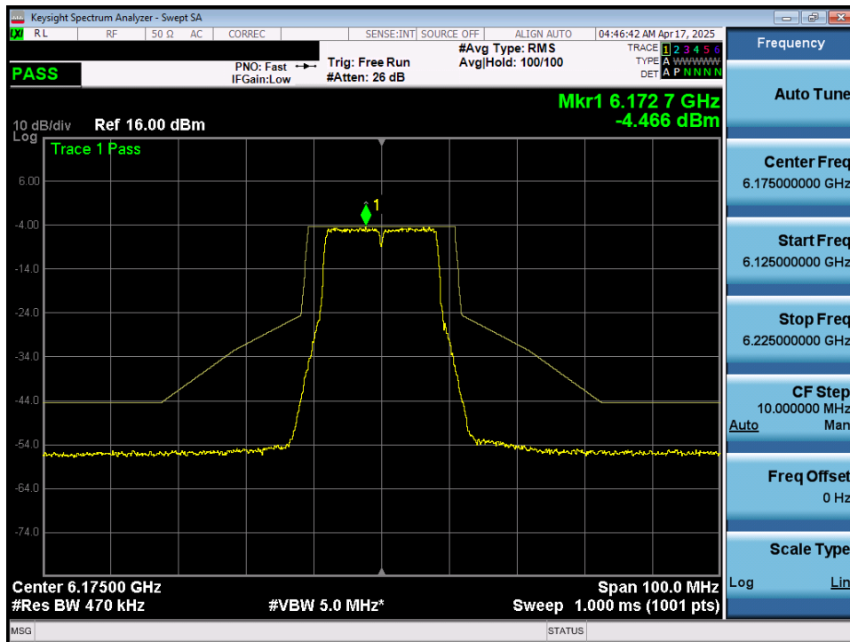
Plot 7-49. In Band Emissions Plot MIMO ANT1 (20MHz 802.11a (UNII Band 5) – Ch. 45) - LPI
