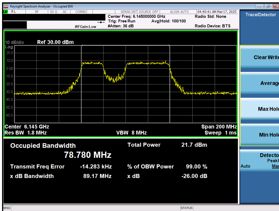
Plot 7-7. 26dB Bandwidth Plot MIMO ANT1 (80MHz 802.11be (UNII Band 5) – Ch. 39) – 20MHz Punctured - LPI/SP
