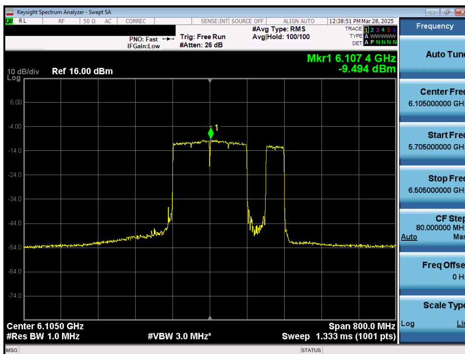
Plot 7-37. Power Spectral Density Plot MIMO ANT1 (320MHz 802.11be (UNII Band 5) – Ch. 31) VLP
