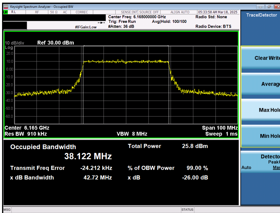
Plot 7-22. 26dB Bandwidth Plot MIMO ANT1 (40MHz 802.11ax/be (Full Tones) (UNII Band 5) – Ch. 43) - SP
