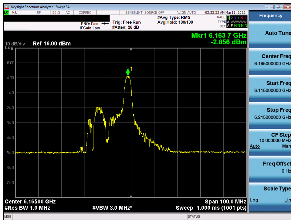
Plot 7-46. Power Spectral Density Plot MIMO ANT1 (40MHz 802.11ax/be (26 Tones) (UNII Band 5) – Ch. 43) - LPI
