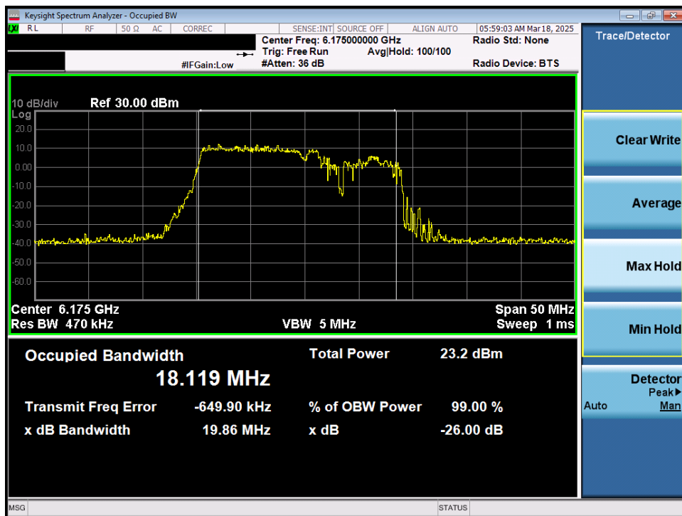
Plot 7-15. 26dB Bandwidth Plot MIMO ANT1 (20MHz 802.11be (106+26 Tones) (UNII Band 5) – Ch. 45) - SP
