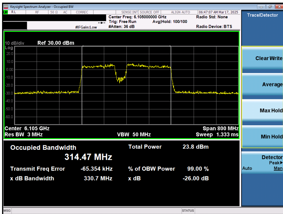
Plot 7-9. 26dB Bandwidth Plot MIMO ANT1 (320MHz 802.11be (3*996+484 Tones) (UNII Band 5) – Ch. 31) LPI/SP
