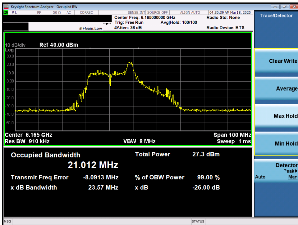
Plot 7-11. 26dB Bandwidth Plot MIMO ANT1 (40MHz 802.11ax/be (26 Tones) (UNII Band 5) – Ch. 43) – SP
