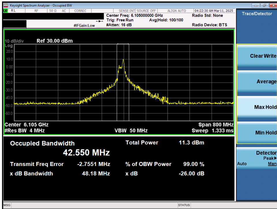
Plot 7-5. 26dB Bandwidth Plot MIMO ANT1 (320MHz 802.11ax/be (26 Tones) (UNII Band 5) – Ch. 31) - LPI
