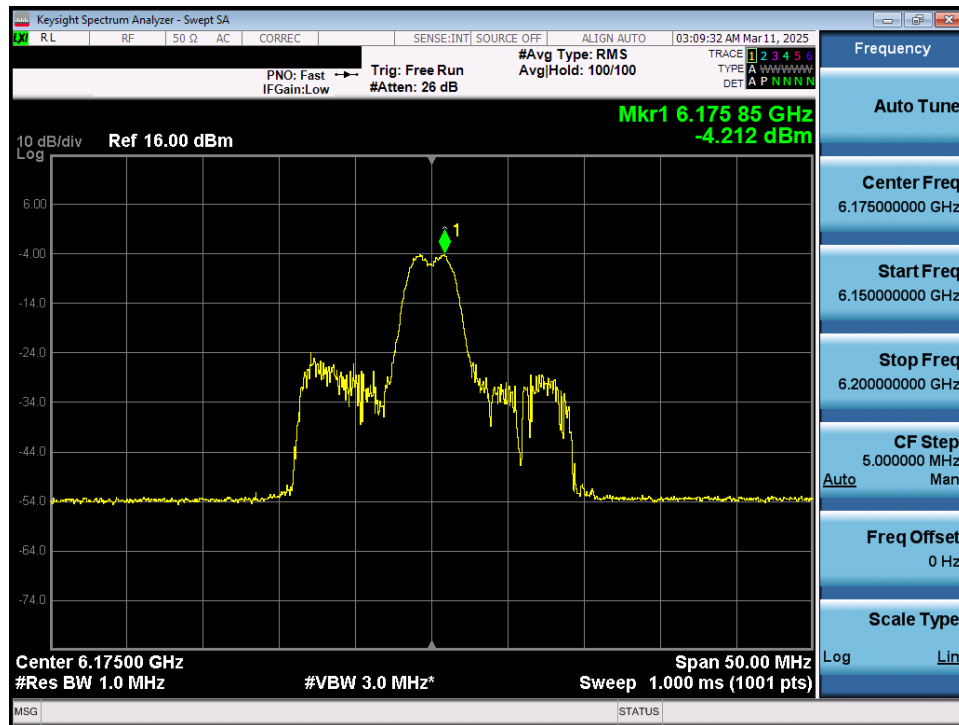
Plot 7-45. Power Spectral Density Plot MIMO ANT1 (20MHz 802.11ax/be (26 Tones) (UNII Band 5) – Ch. 45) - LPI
