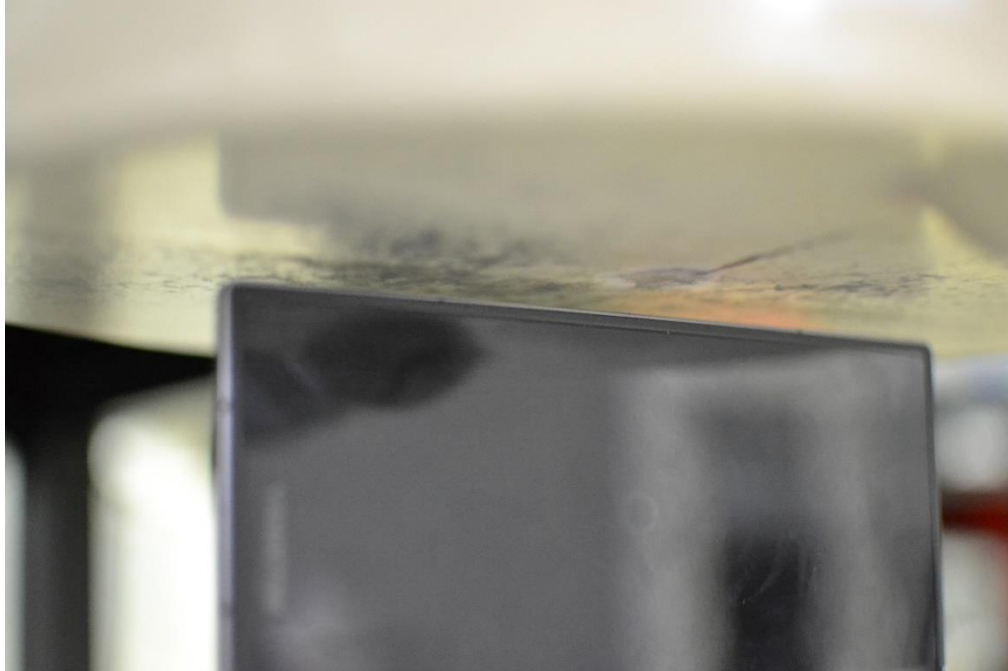
SAR Test Setup Photo 25 – Tablet, Folder Open, Left Edge at 5mm
