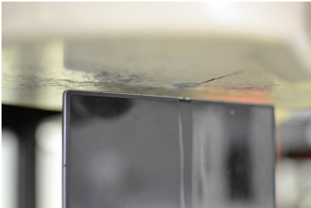
SAR Test Setup Photo 22 – Tablet, Folder Open, Top Edge at 5mm
