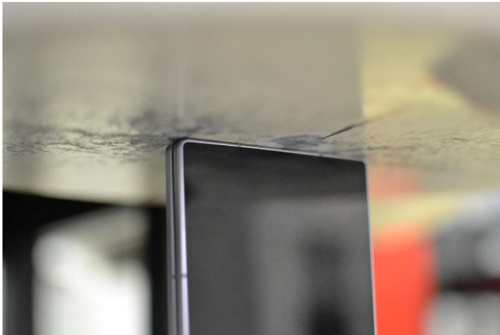
SAR Test Setup Photo 14 – Phablet, Folder Closed, Bottom Edge at 0mm
