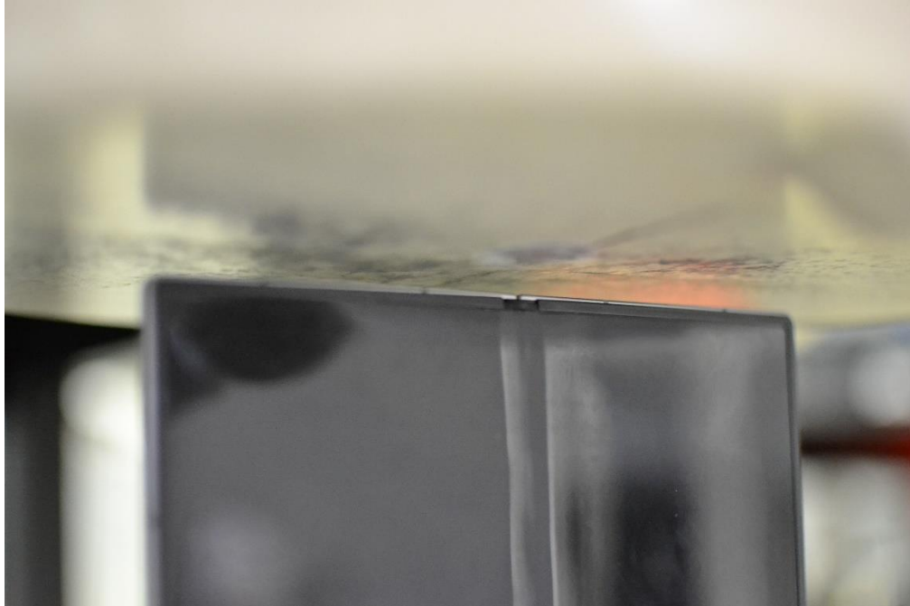
SAR Test Setup Photo 23 – Tablet, Folder Open, Bottom Edge at 5mm
