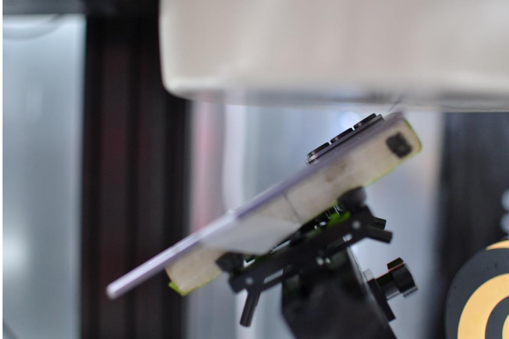
SAR Test Setup Photo 21 – Tablet, Folder Open, Back Side at 5mm (for AG1)
