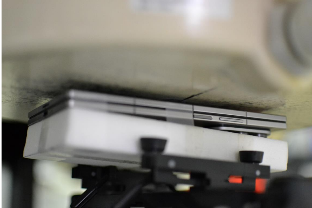
SAR Test Setup Photo 11 – Hotspot, Folder Closed, Front Side at 5mm
