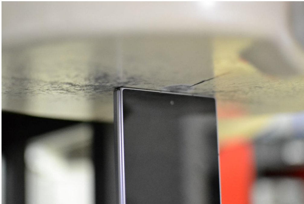
SAR Test Setup Photo 16 – Phablet, Folder Closed, Top Edge at 0mm
