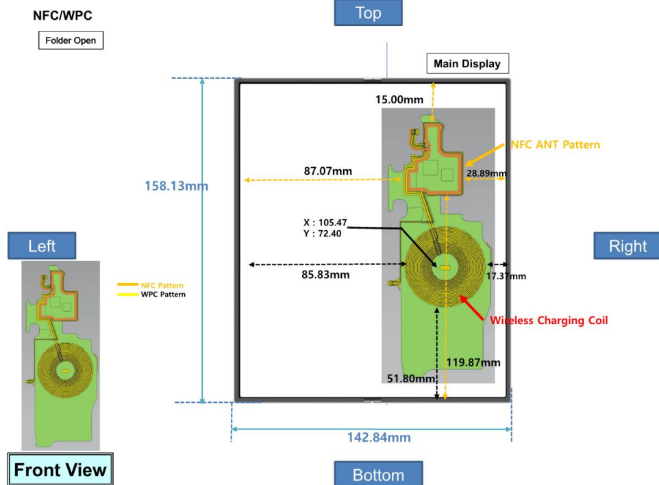
Figure H-4 NFC Antenna Locations – Folder Open
