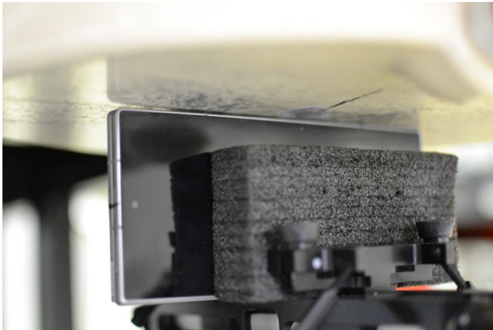
SAR Test Setup Photo 18 – Phablet, Folder Closed, Right Edge at 0mm
