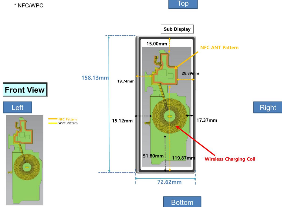
Figure H-3 NFC Antenna Locations – Folder Closed
