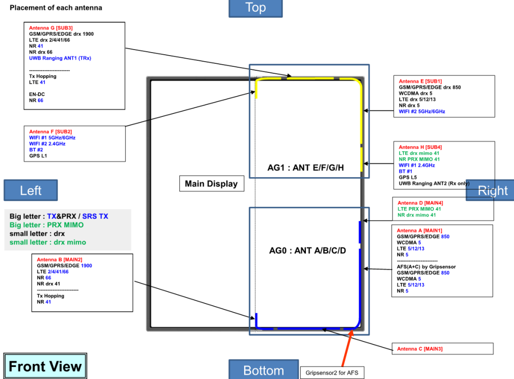
Figure H-1 DUT Antenna Locations – Folder Closed
