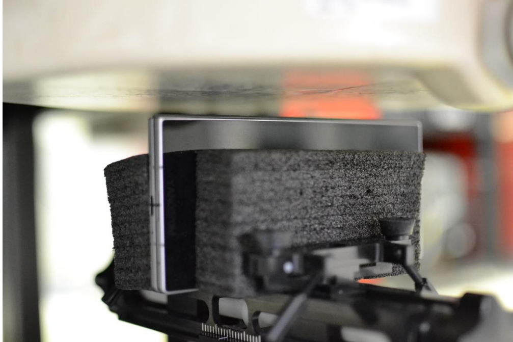
SAR Test Setup Photo 19 – Hotspot, Folder Closed, Left Edge at 10mm
