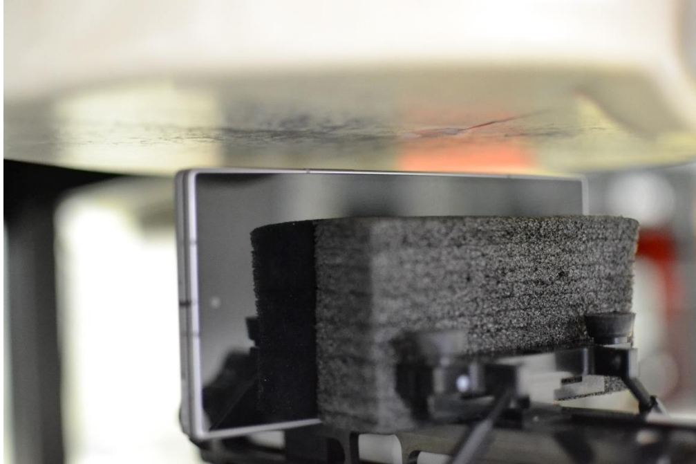
SAR Test Setup Photo 17 – Hotspot, Folder Closed, Right Edge at 10mm
