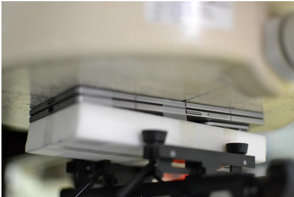
SAR Test Setup Photo 12 – Phablet, Folder Closed, Front Side at 0mm
