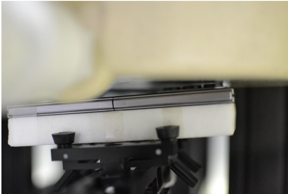
SAR Test Setup Photo 9 – Body-worn/Hotspot, Folder Closed, Back Side at 5mm (for AG1)
