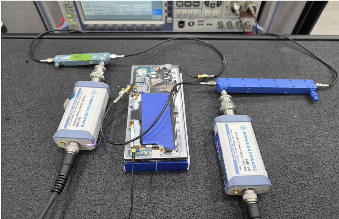
Test Setup Photo 9 – Conducted Test Setup (Figure 6-1e)
