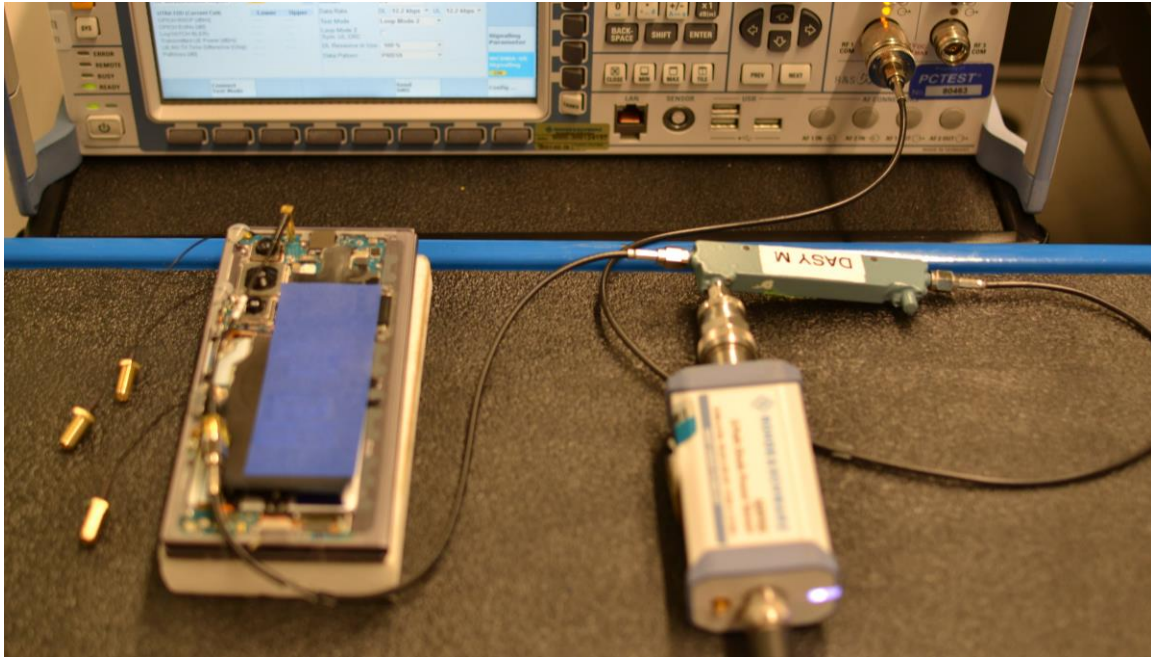
Test Setup Photo 3 – Conducted Test Setup (Figure 6-1a)
