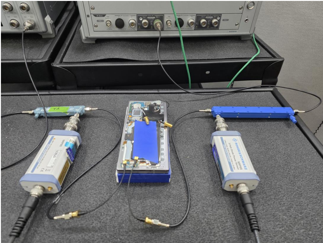
Test Setup Photo 6 – Conducted Test Setup (Figure 6-1c)
