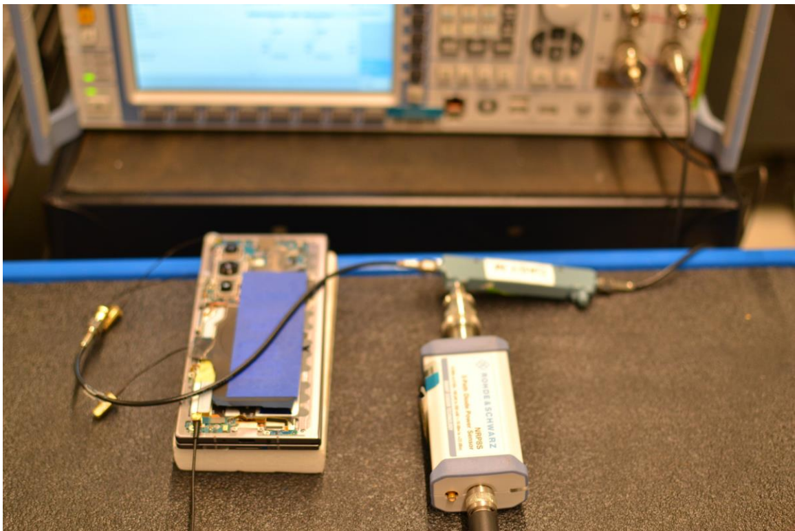
Test Setup Photo 8 – Conducted Test Setup (Figure 6-1d)
