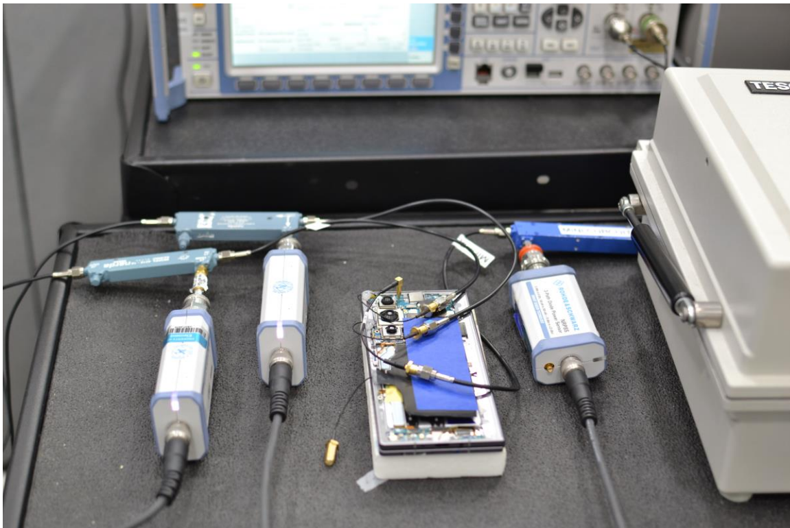
Test Setup Photo 10 – Conducted Test Setup (Figure 6-1f)
