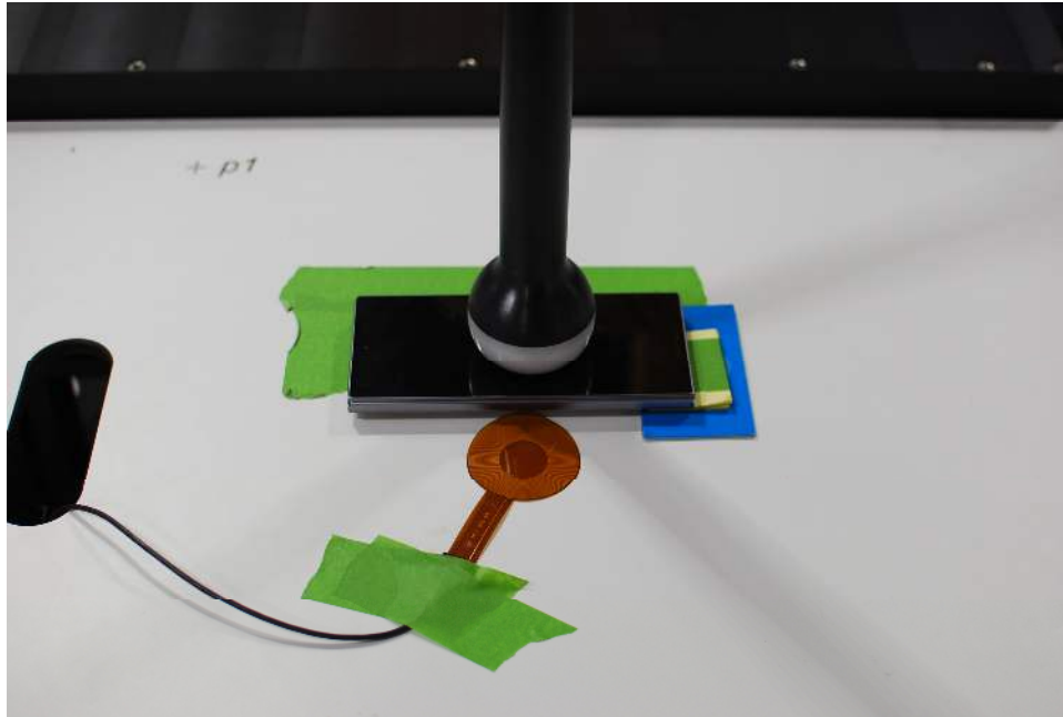
Test Setup Photo 1 Standby (Ping) Signal, Folder Closed, Front side, 0mm
