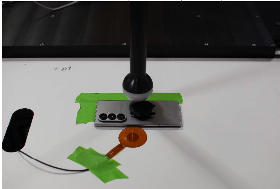
Test Setup Photo 10 Device to Watch, Folder Closed, Back Side, 0mm
