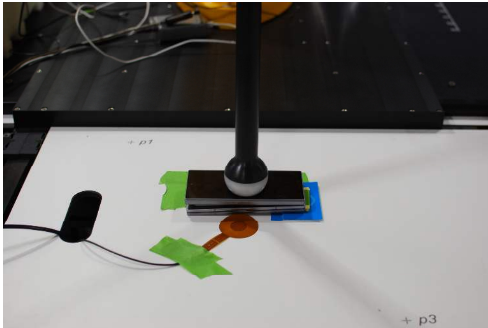
Test Setup Photo 8 Device to Device - Inline, Folder Closed, Back Side, 0mm
