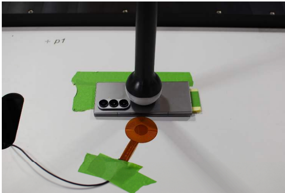
Test Setup Photo 2 Standby (Ping) Signal, Folder Closed, Back side, 0mm
