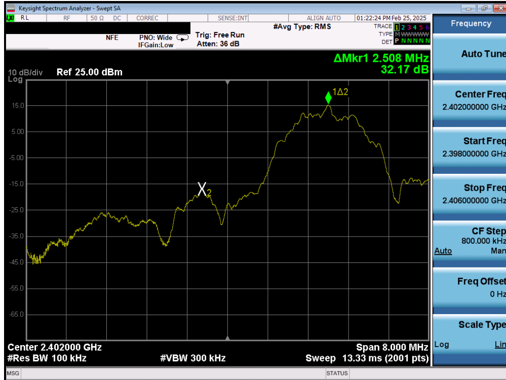
Plot 7-131. Band Edge Plot (Bluetooth (LE), 2Mbps – Ch. 0) – Dual Ant 2
