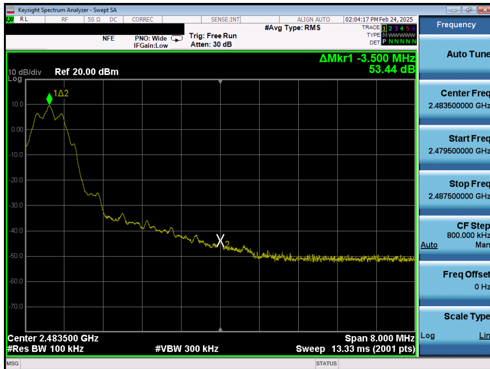
Plot 7-110. Band Edge Plot (Bluetooth (LE), 125kbps - Ch. 39) - Ant 1
