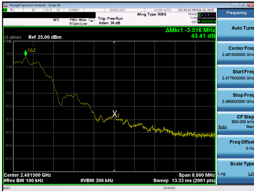
Plot 7-128. Band Edge Plot (Bluetooth (LE), 2Mbps – Ch. 39) – Dual Ant 1
