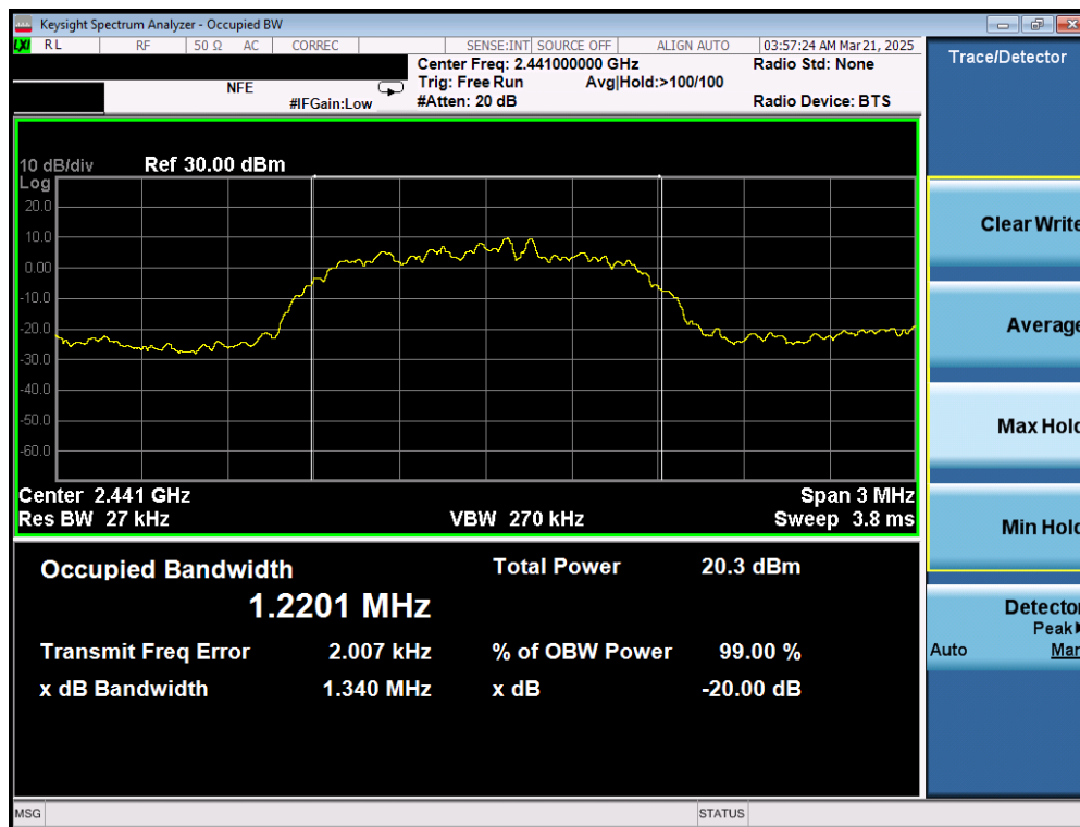
Plot 7-23. 20dB Bandwidth Plot (Bluetooth, 2Mbps – Ch. 39) – Dual Ant 1
