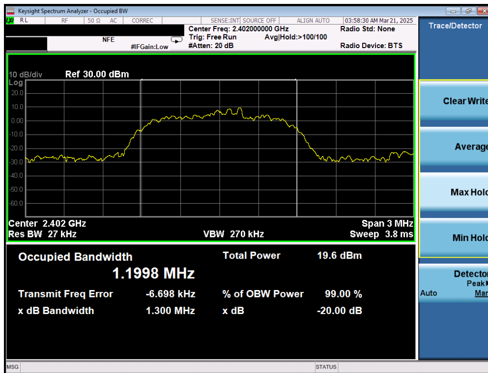
Plot 7-25. 20dB Bandwidth Plot (Bluetooth, 3Mbps – Ch. 0) – Dual Ant 1
