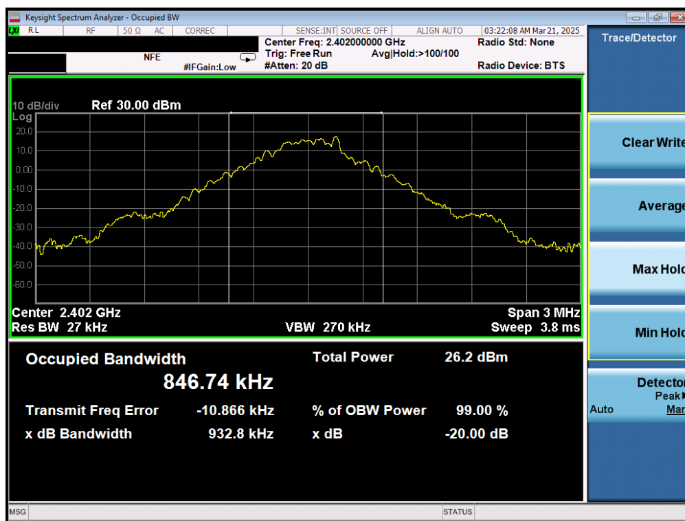
Plot 7-10. 20dB Bandwidth Plot (Bluetooth, 1Mbps – Ch. 0) – Ant 2
