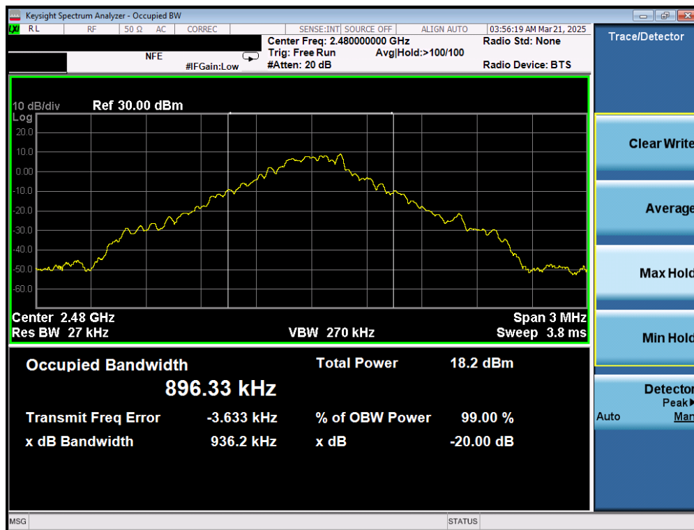
Plot 7-21. 20dB Bandwidth Plot (Bluetooth, 1Mbps – Ch. 78) – Dual Ant 1
